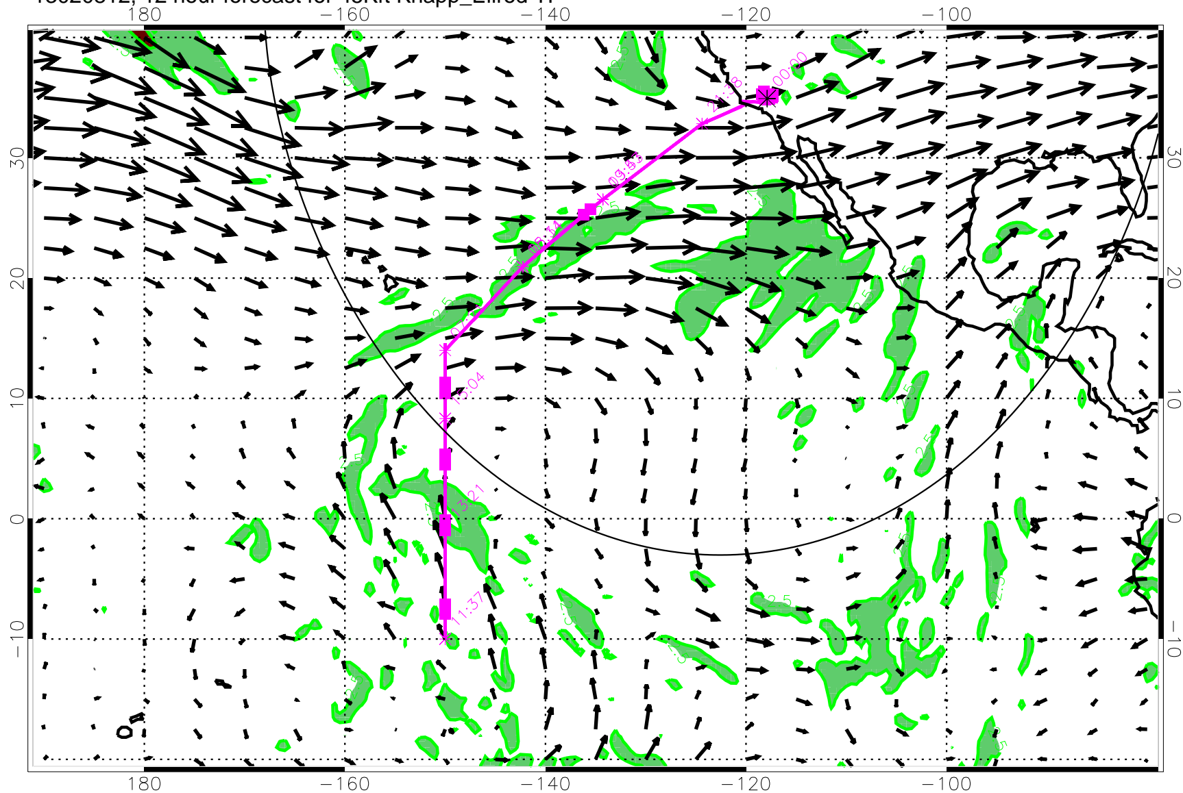
13020812, 12 hour forecast for 45Kft Knapp_Ellrod TI
