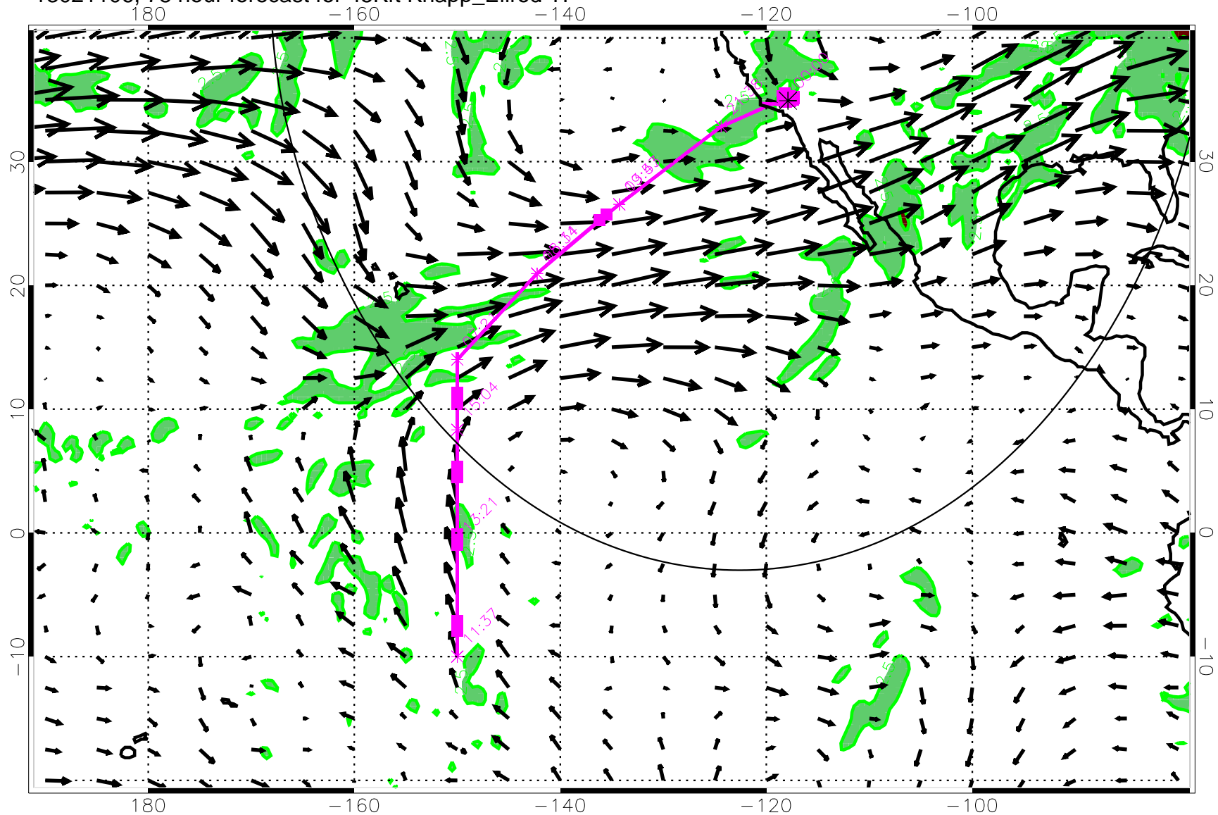
13021106, 78 hour forecast for 45Kft Knapp_Ellrod TI
