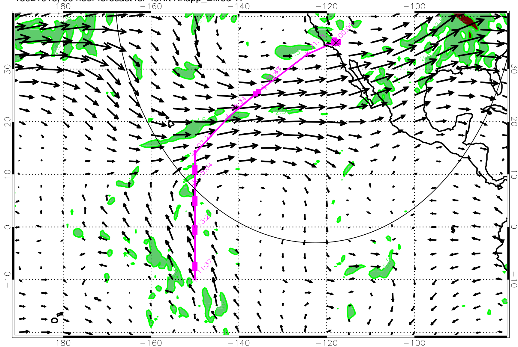
13021018, 66 hour forecast for 45Kft Knapp_Ellrod TI
