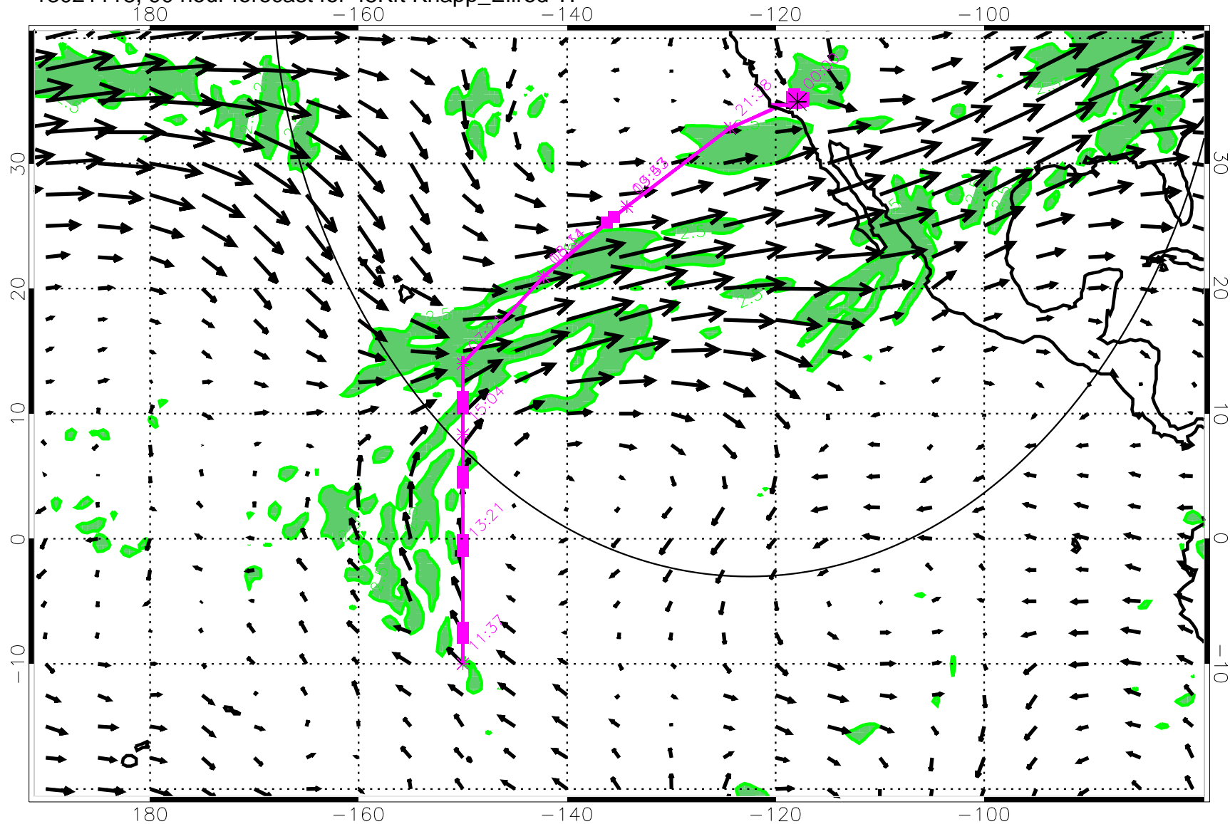
13021118, 90 hour forecast for 45Kft Knapp_Ellrod TI
