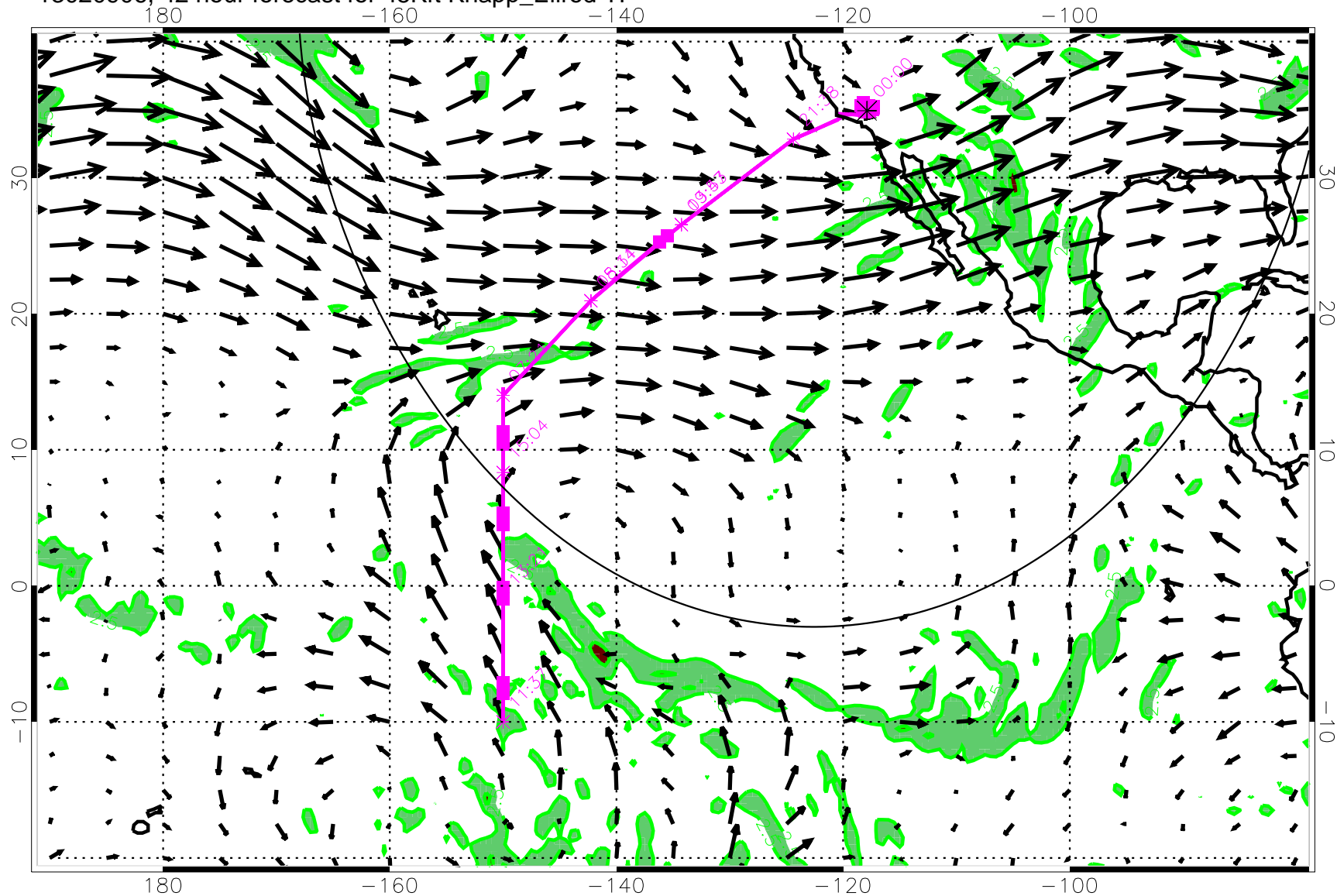
13020906, 42 hour forecast for 45Kft Knapp_Ellrod TI
