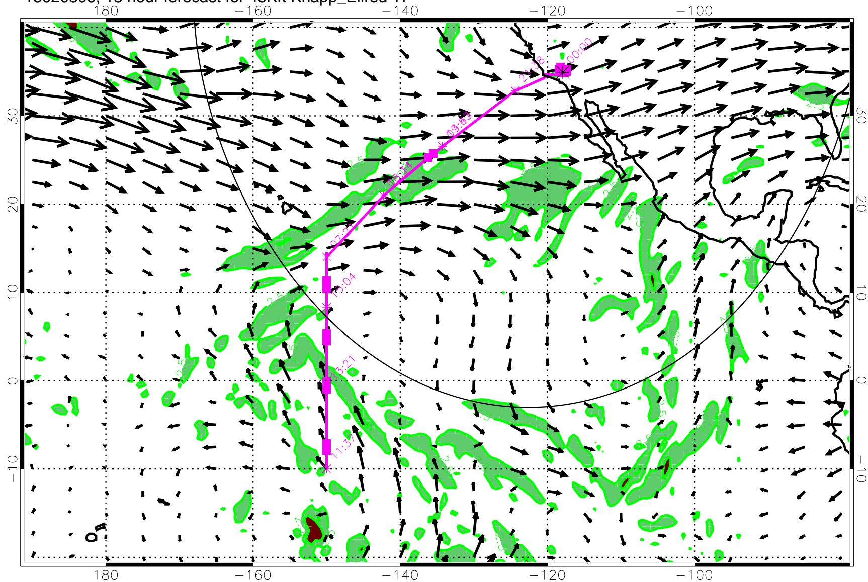
13020806, 18 hour forecast for 45Kft Knapp_Ellrod TI
