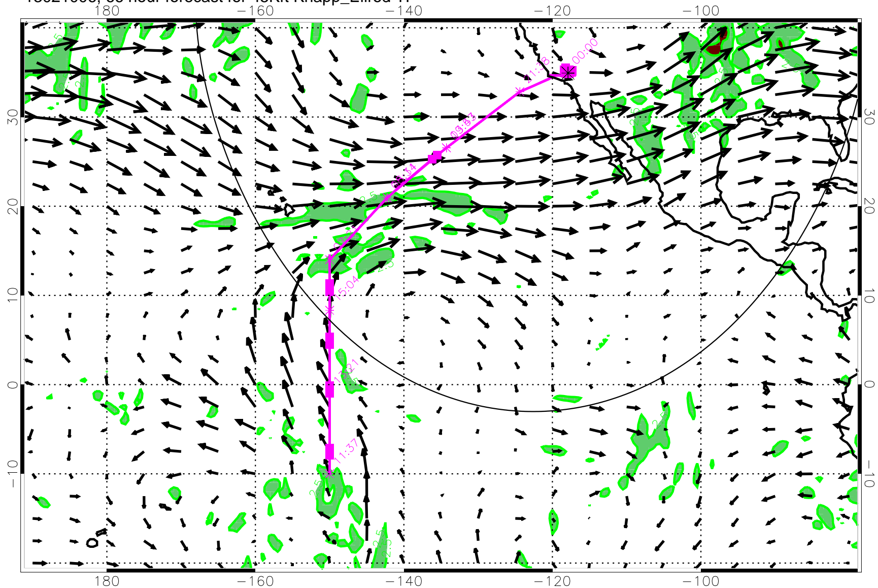
13021006, 66 hour forecast for 45Kft Knapp_Ellrod TI
