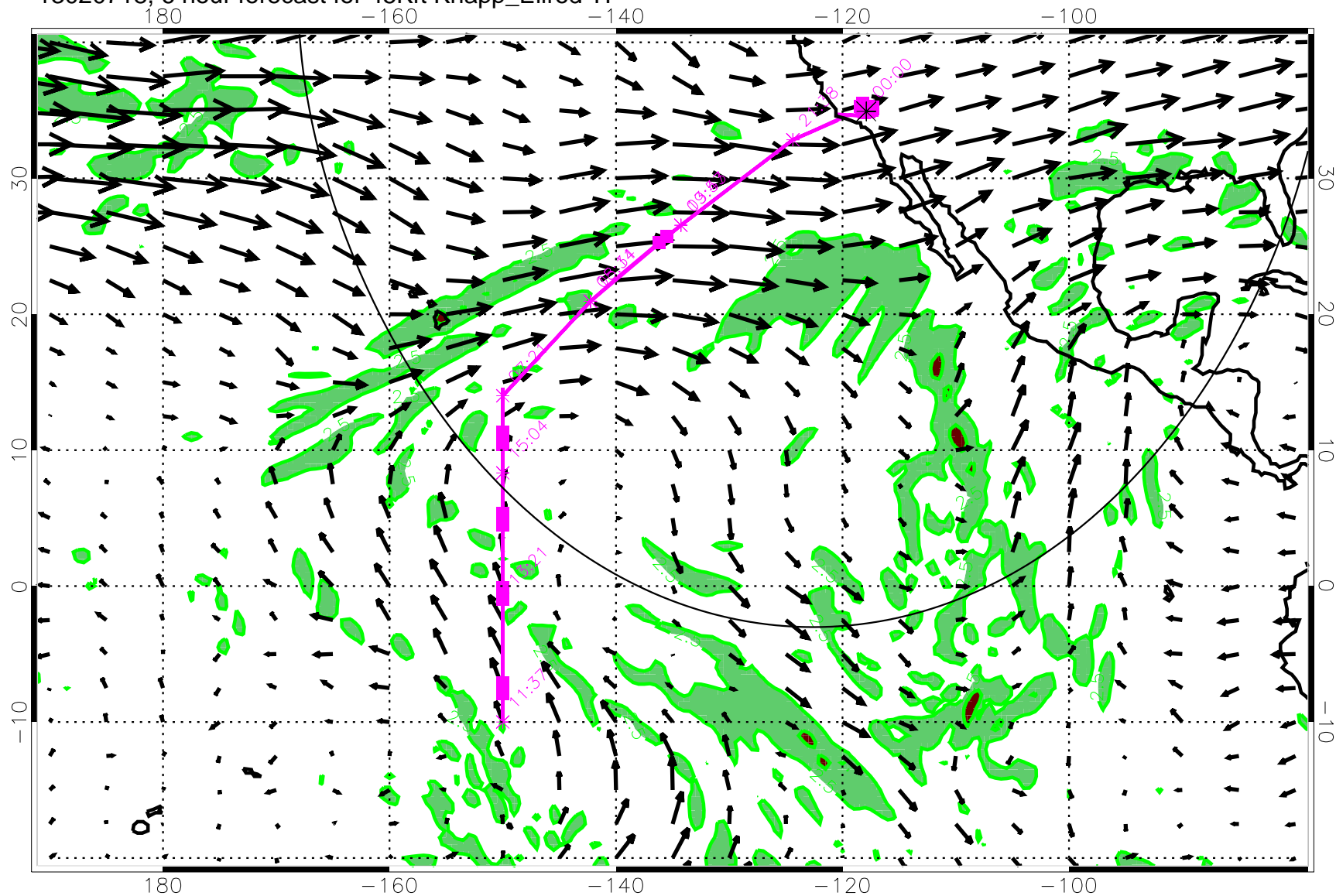
13020718, 6 hour forecast for 45Kft Knapp_Ellrod TI
