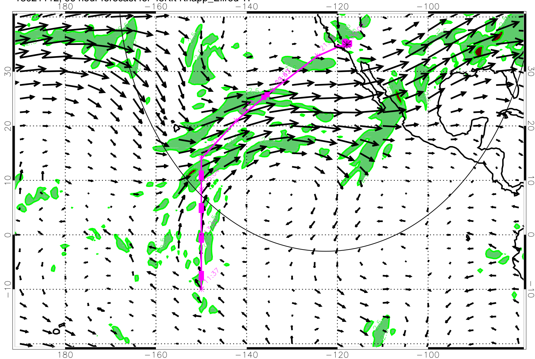
13021112, 96 hour forecast for 45Kft Knapp_Ellrod TI
