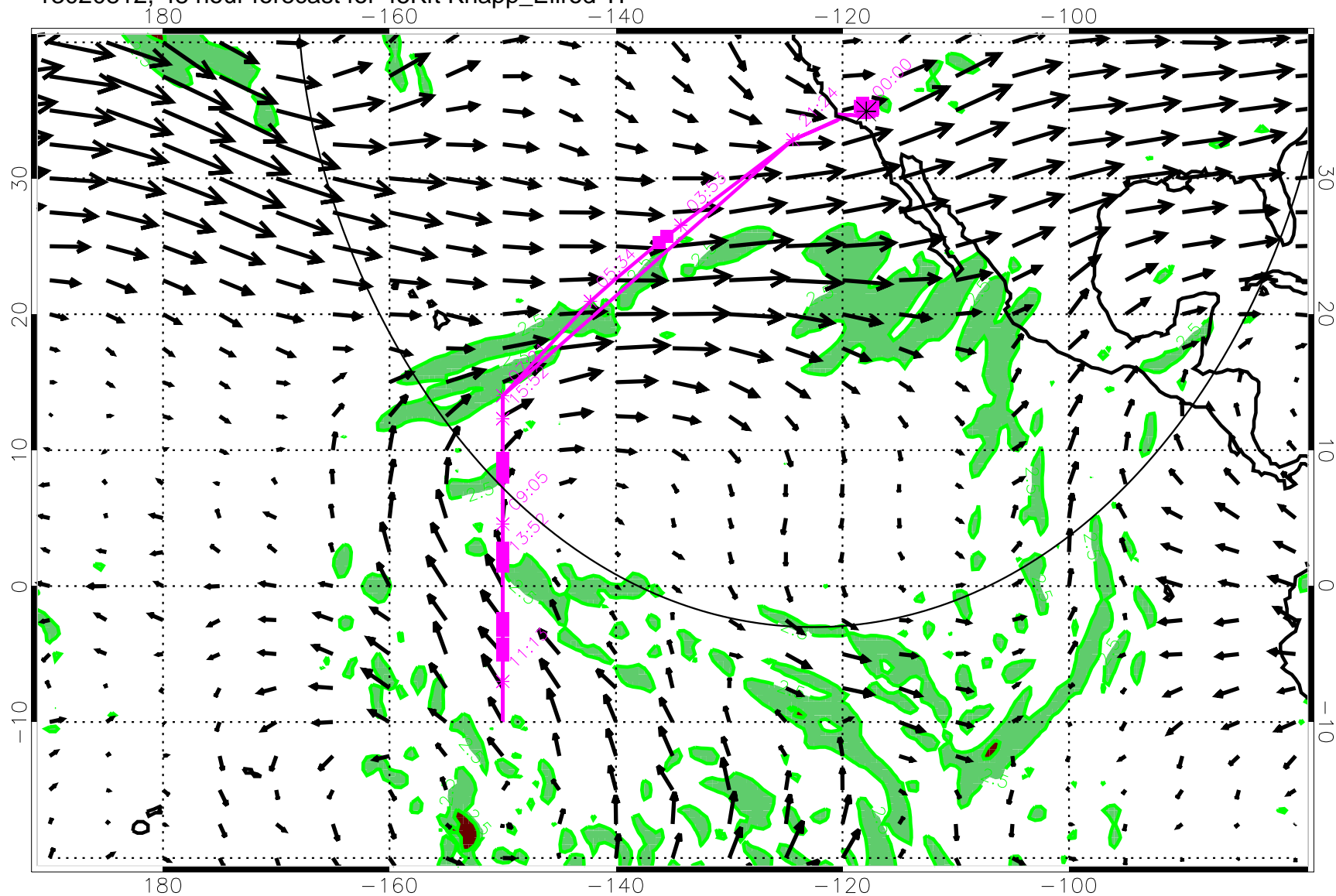
13020812, 48 hour forecast for 45Kft Knapp_Ellrod TI
