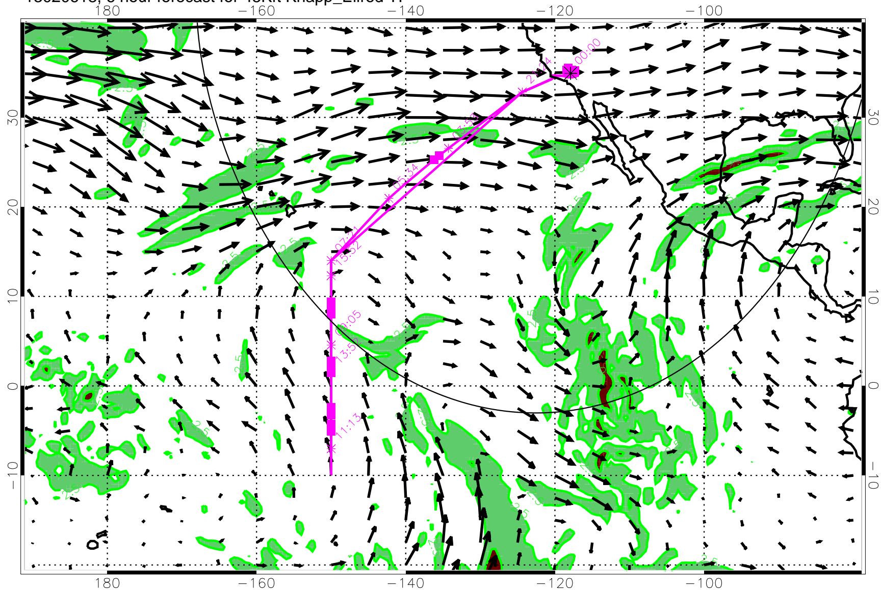
13020618, 6 hour forecast for 45Kft Knapp_Ellrod TI
