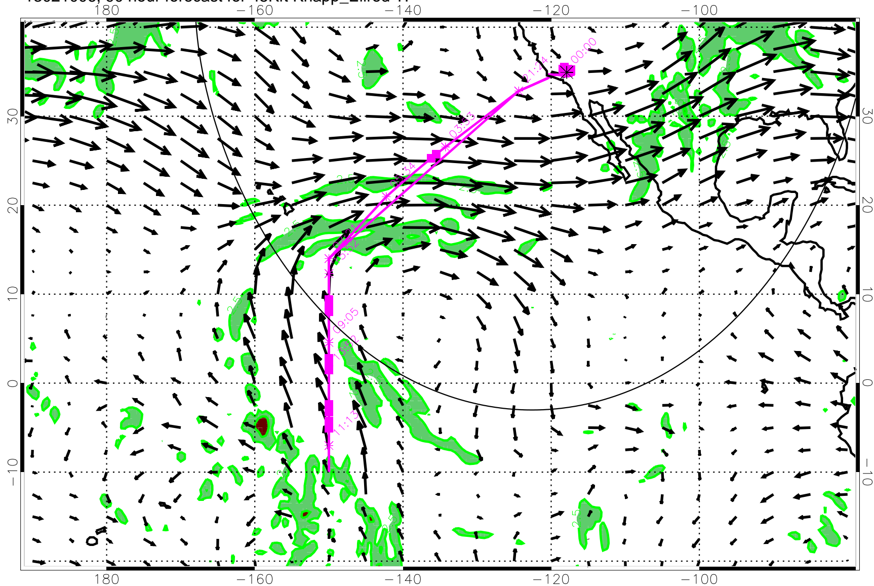
13021006, 90 hour forecast for 45Kft Knapp_Ellrod TI
