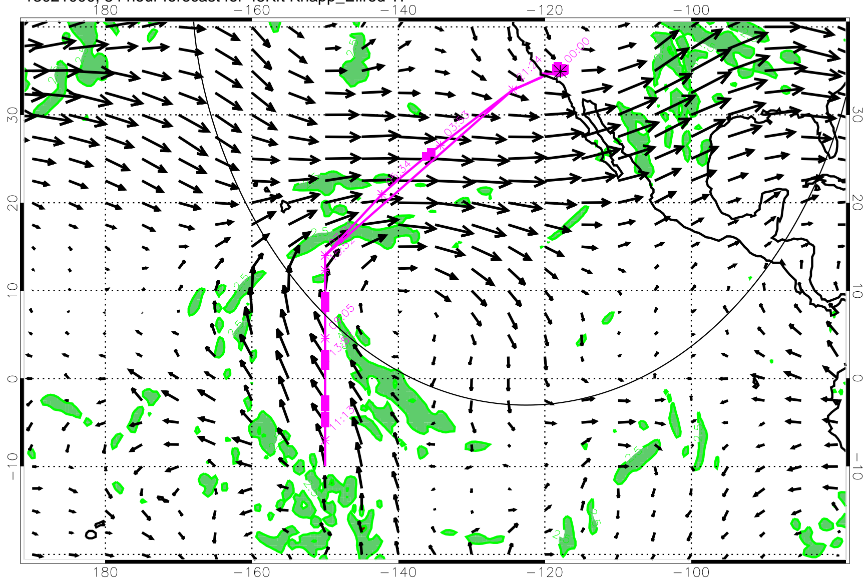
13021000, 84 hour forecast for 45Kft Knapp_Ellrod TI
