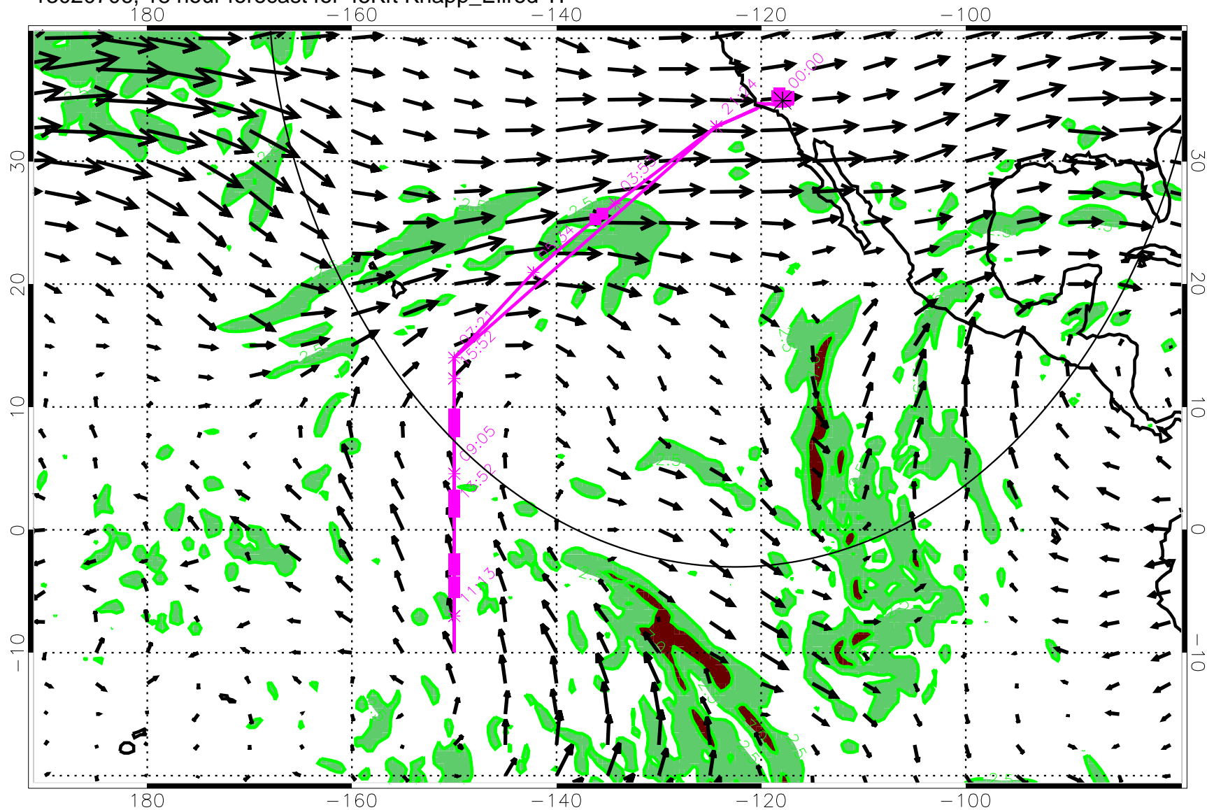
13020706, 18 hour forecast for 45Kft Knapp_Ellrod TI
