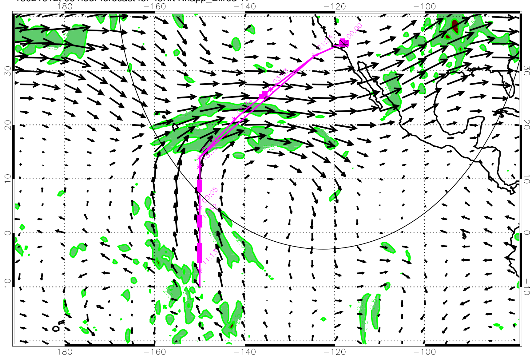
13021012, 96 hour forecast for 45Kft Knapp_Ellrod TI
