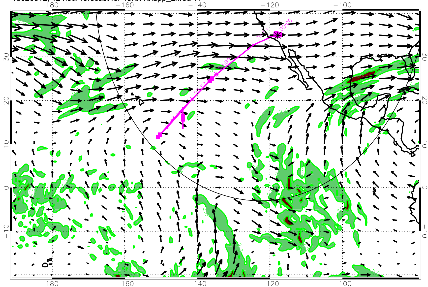
13020612, 12 hour forecast for 45Kft Knapp_Ellrod TI
