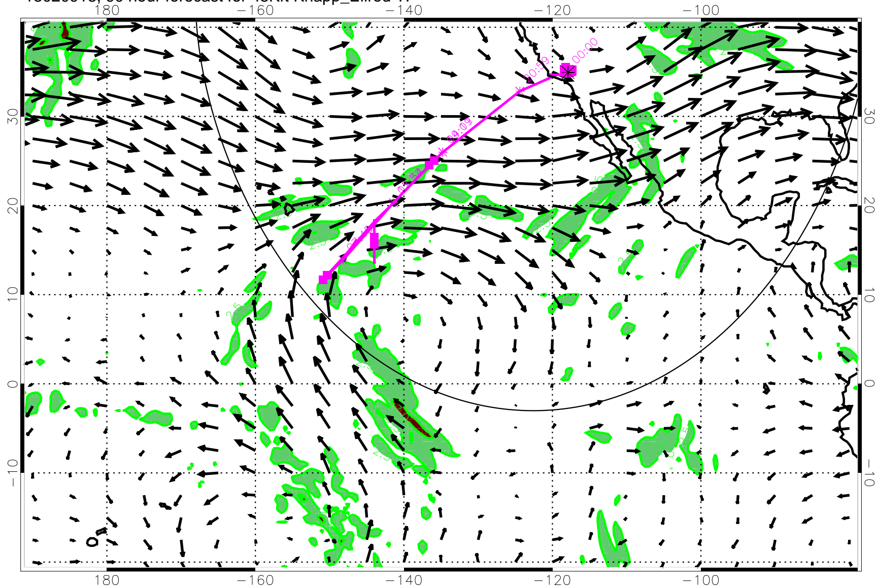
13020918, 90 hour forecast for 45Kft Knapp_Ellrod TI
