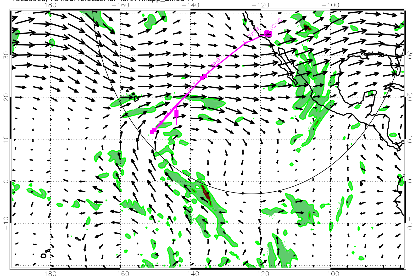
13020906, 78 hour forecast for 45Kft Knapp_Ellrod TI
