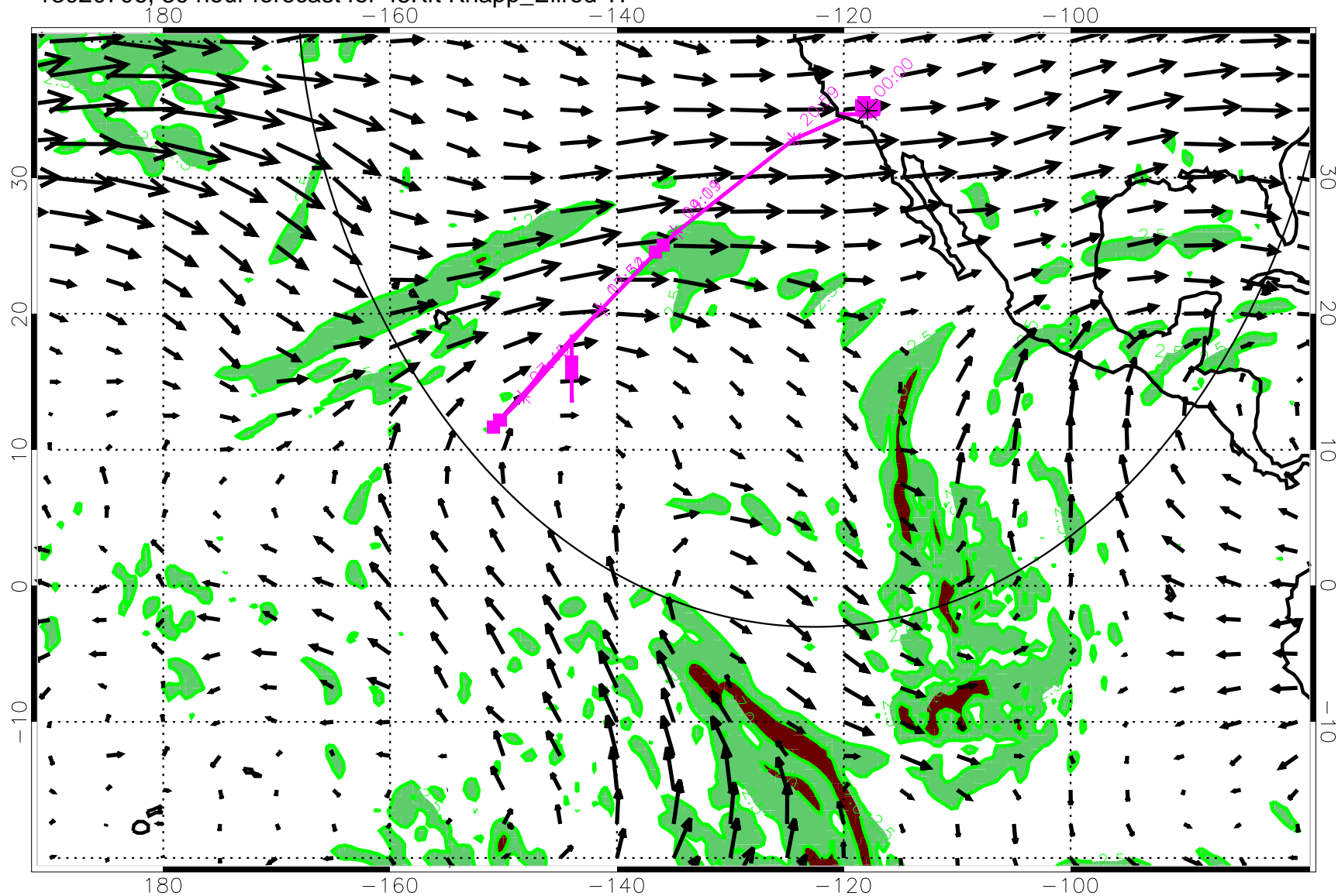
13020706, 30 hour forecast for 45Kft Knapp_Ellrod TI
