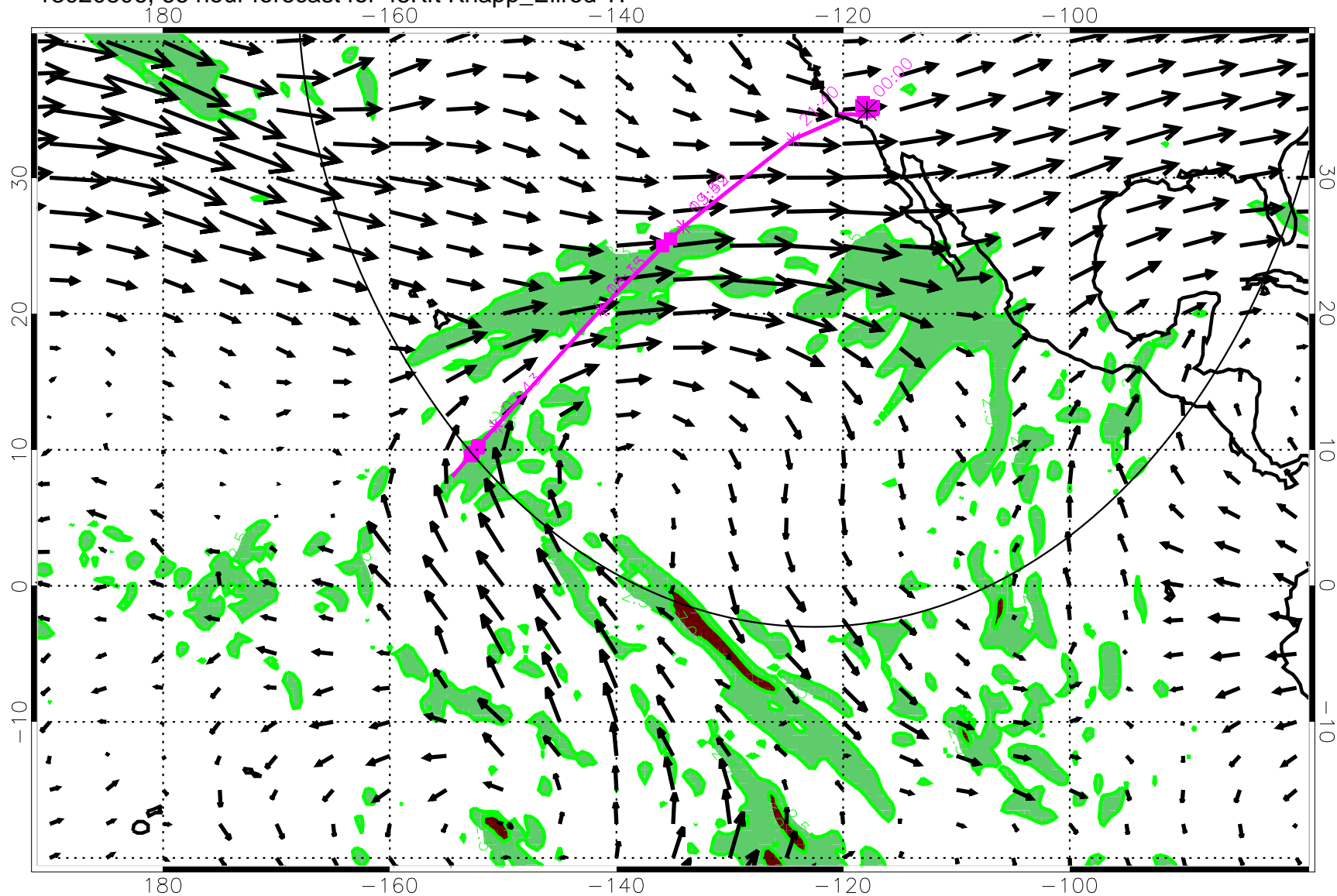
13020806, 66 hour forecast for 45Kft Knapp_Ellrod TI
