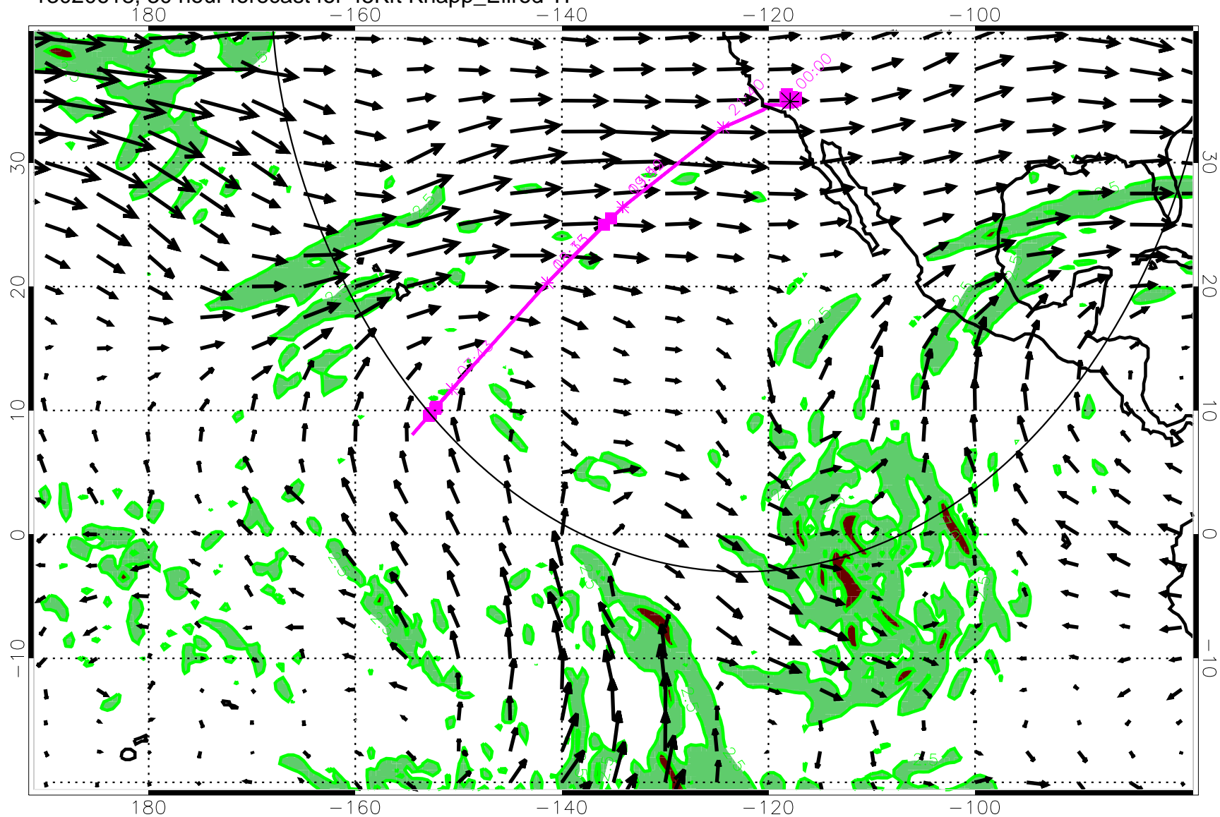
13020618, 30 hour forecast for 45Kft Knapp_Ellrod TI
