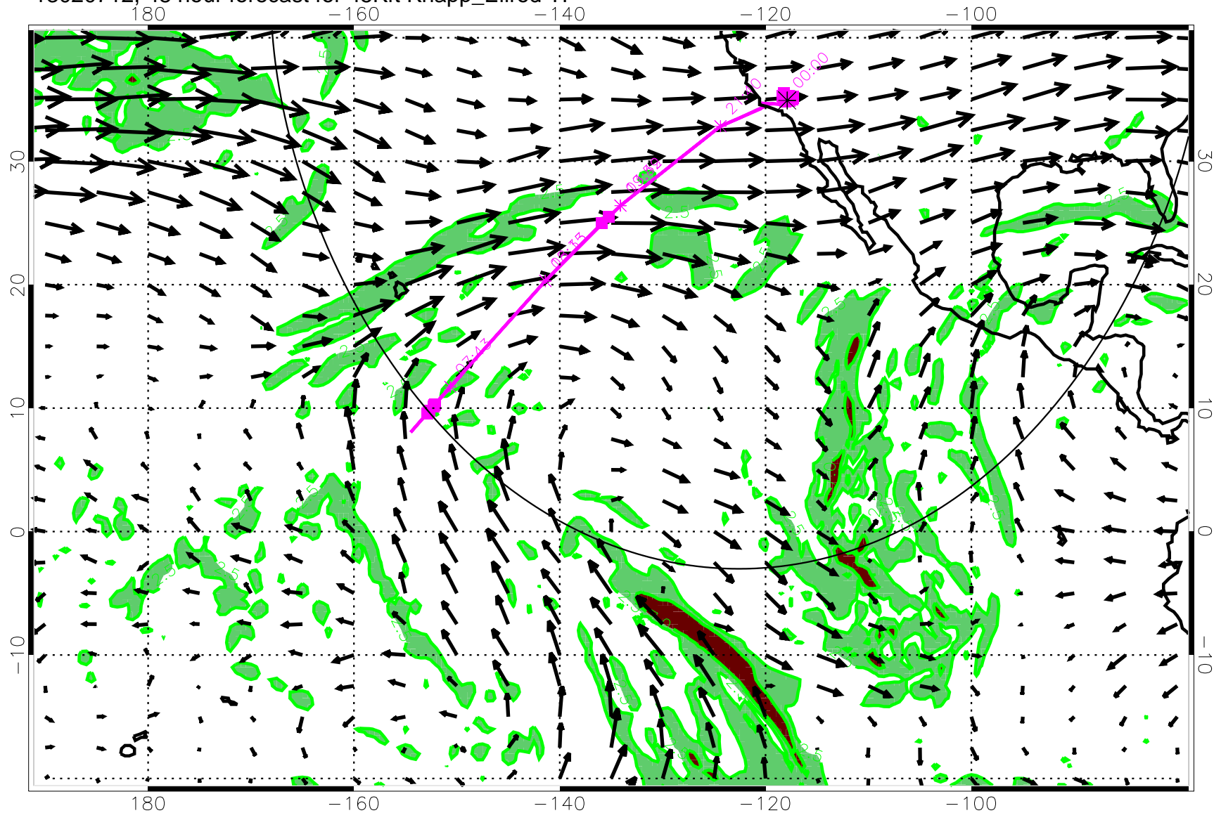
13020712, 48 hour forecast for 45Kft Knapp_Ellrod TI
