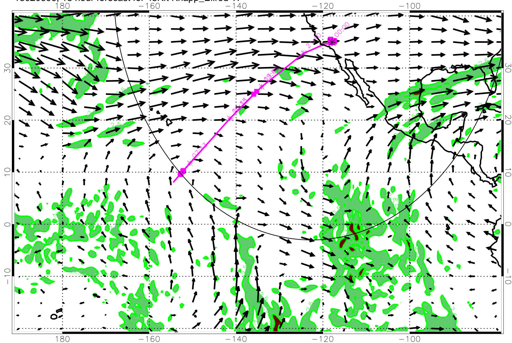
13020606, 18 hour forecast for 45Kft Knapp_Ellrod TI
