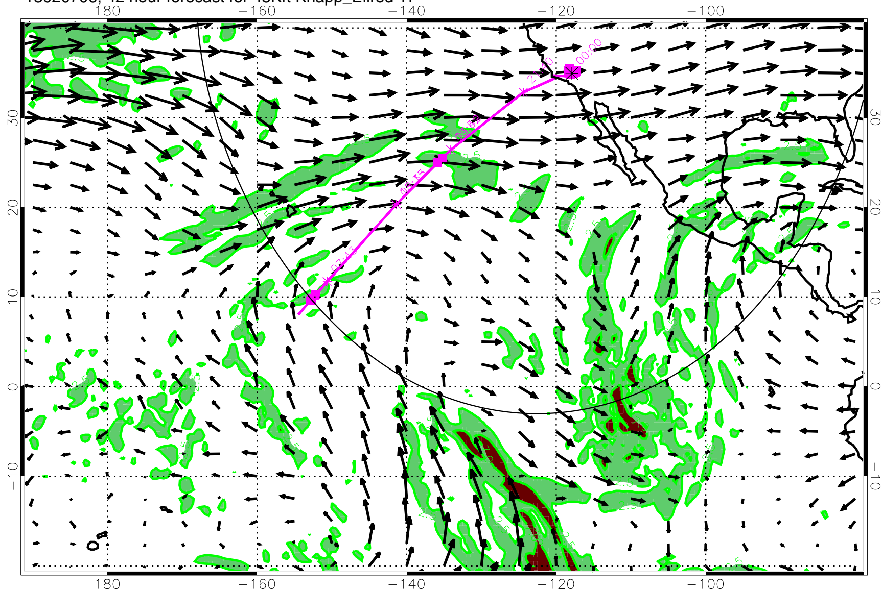
13020706, 42 hour forecast for 45Kft Knapp_Ellrod TI
