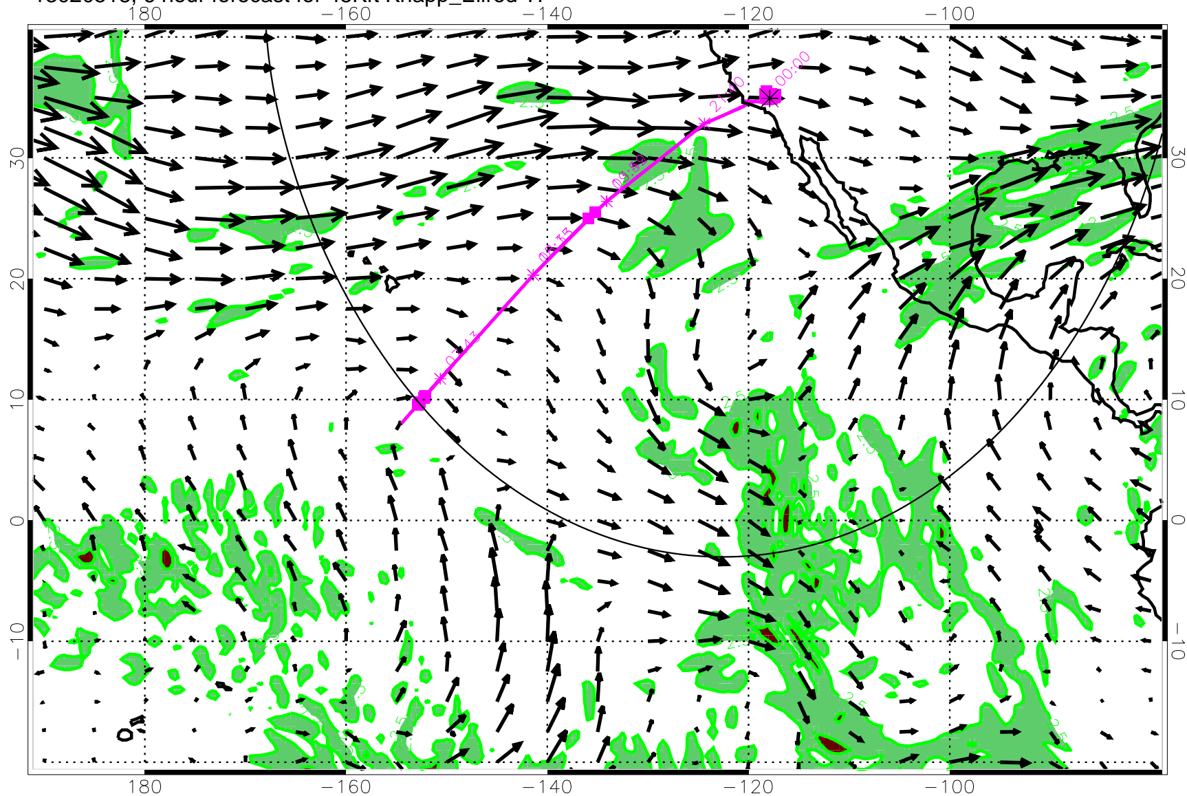
13020518, 6 hour forecast for 45Kft Knapp_Ellrod TI
