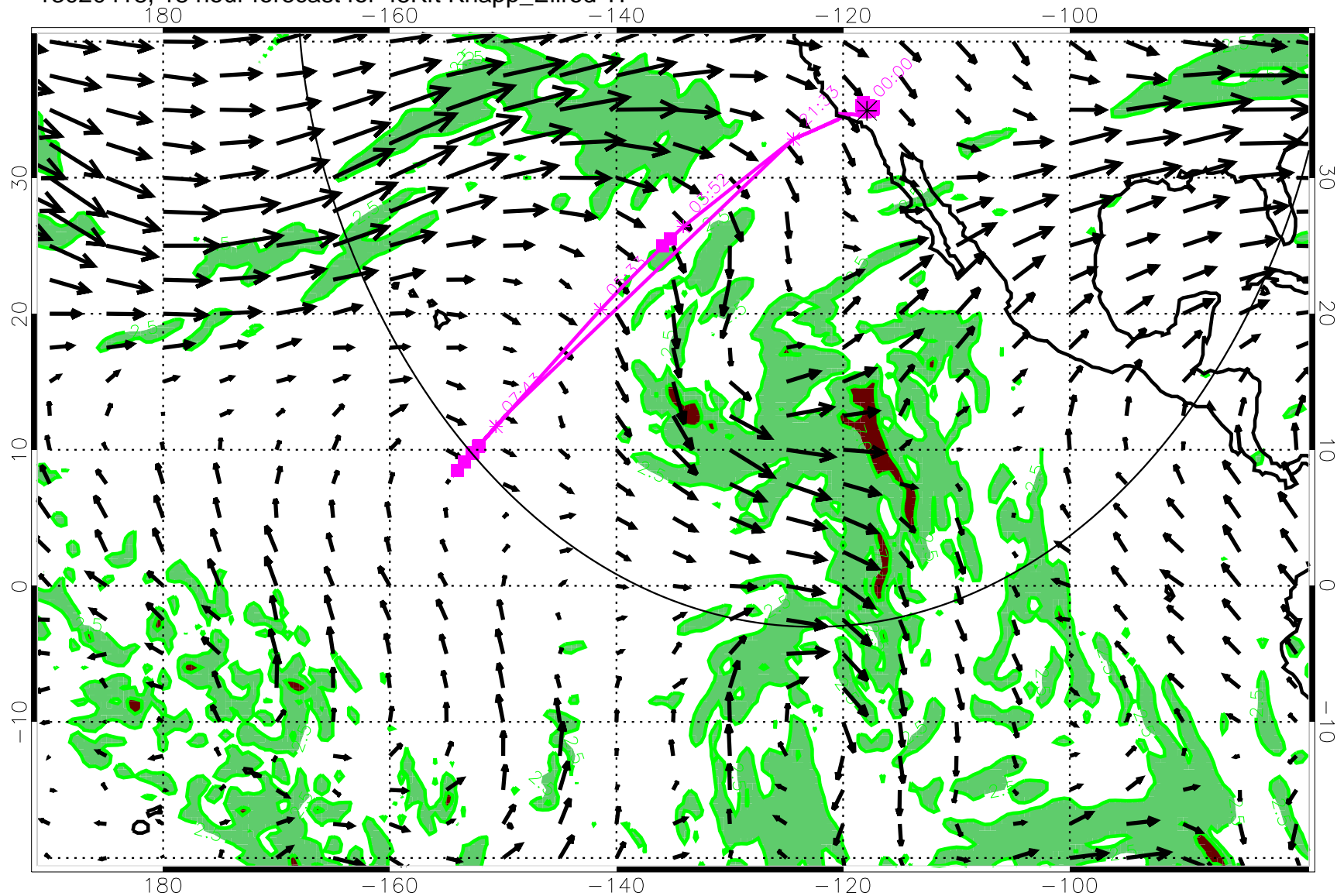
13020418, 18 hour forecast for 45Kft Knapp_Ellrod TI
