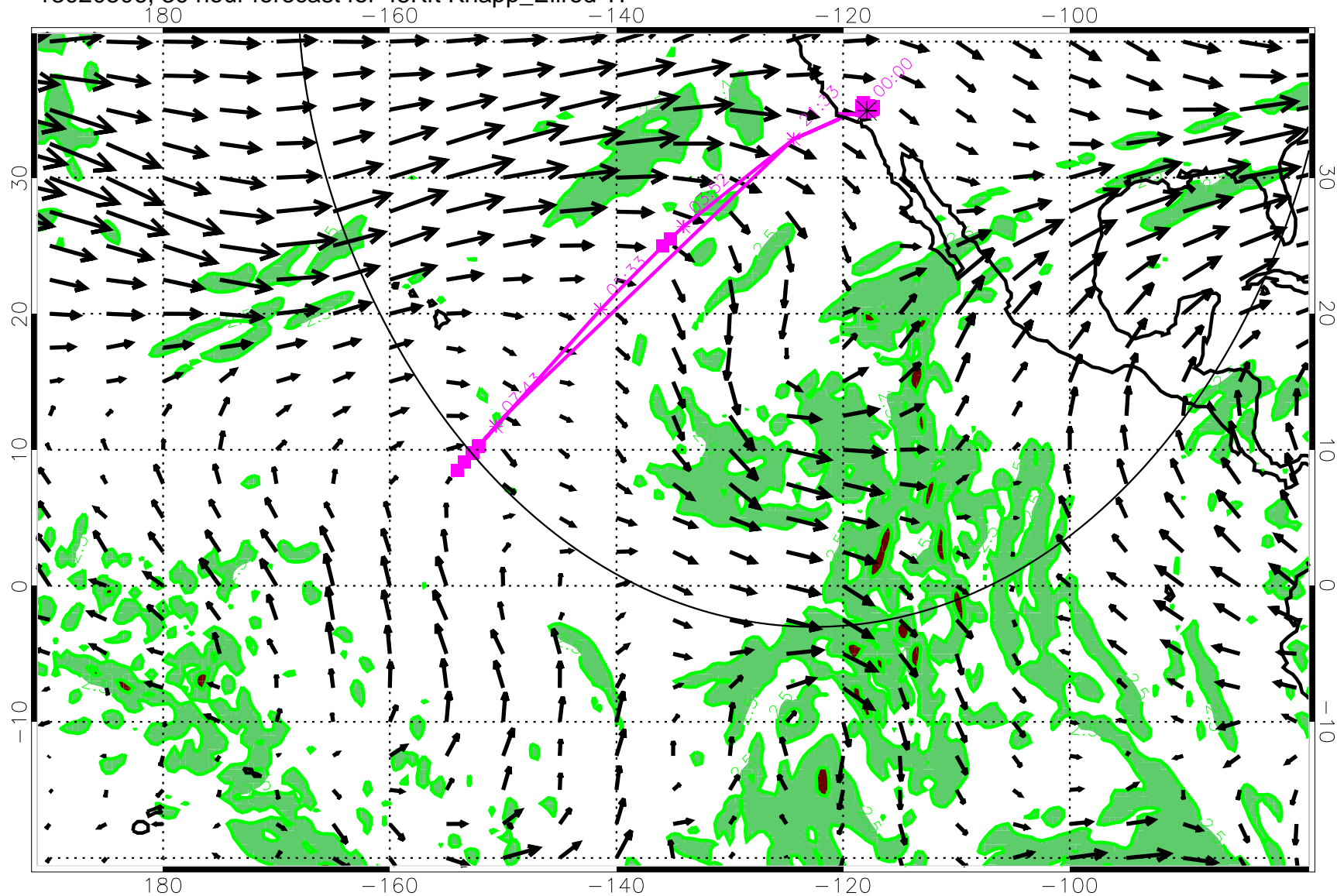
13020506, 30 hour forecast for 45Kft Knapp_Ellrod TI
