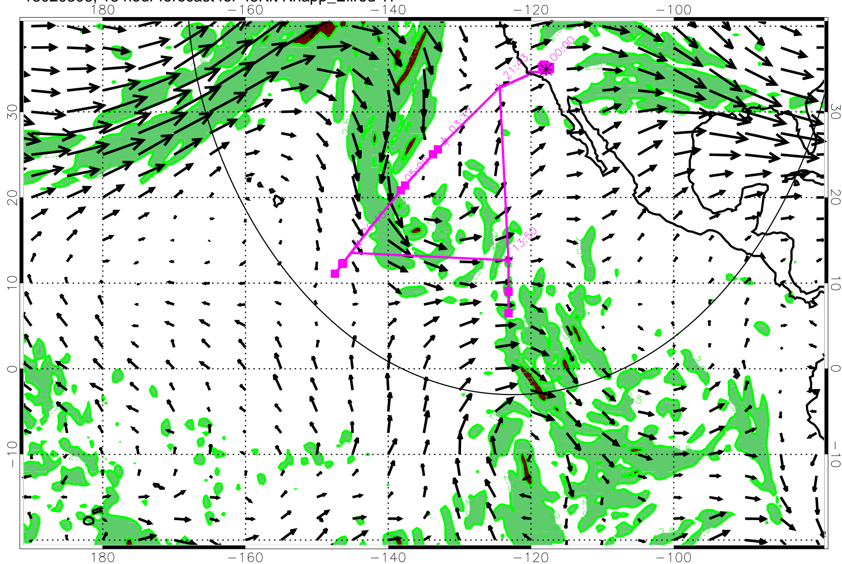
13020306, 18 hour forecast for 45Kft Knapp_Ellrod TI
