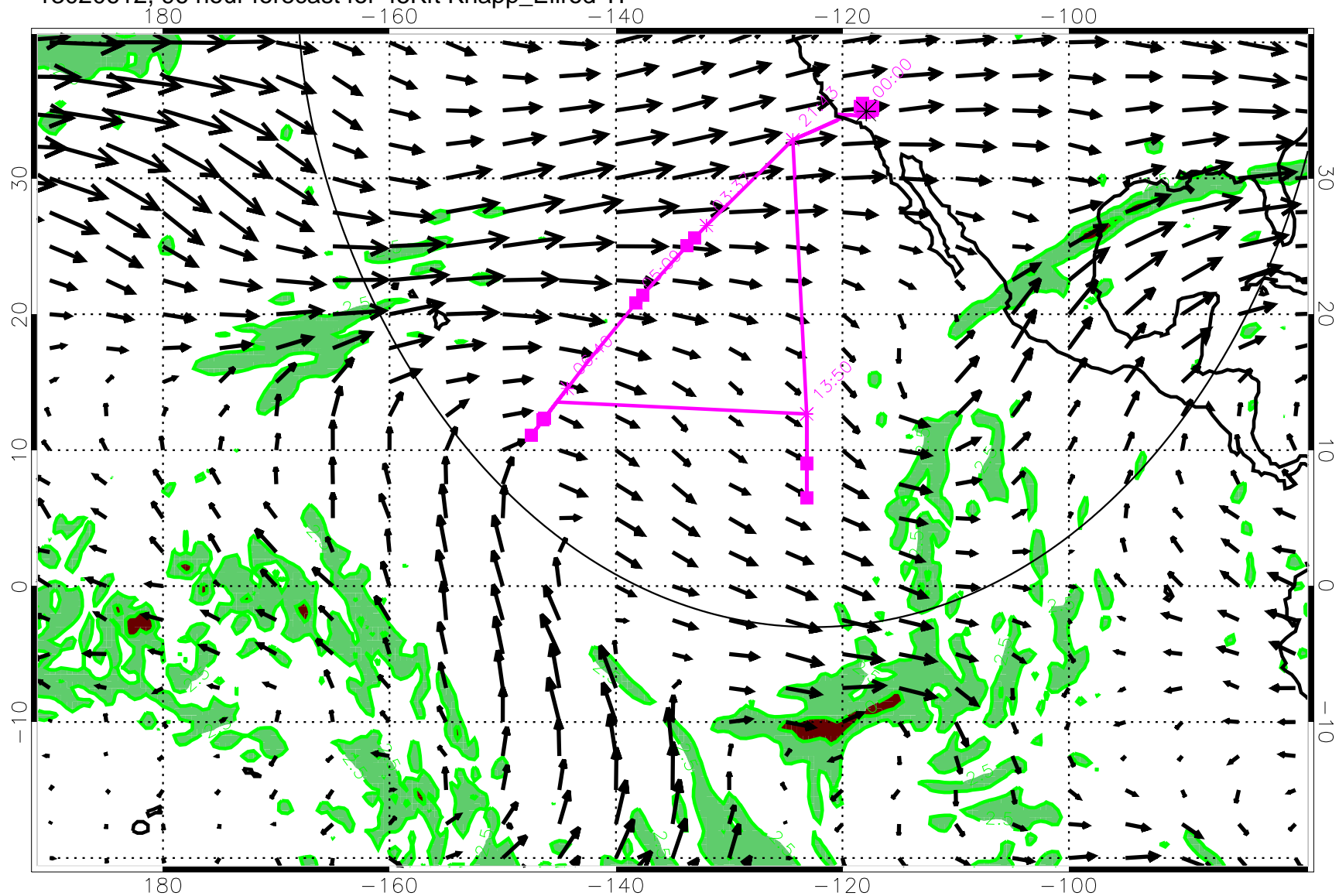
13020612, 96 hour forecast for 45Kft Knapp_Ellrod TI
