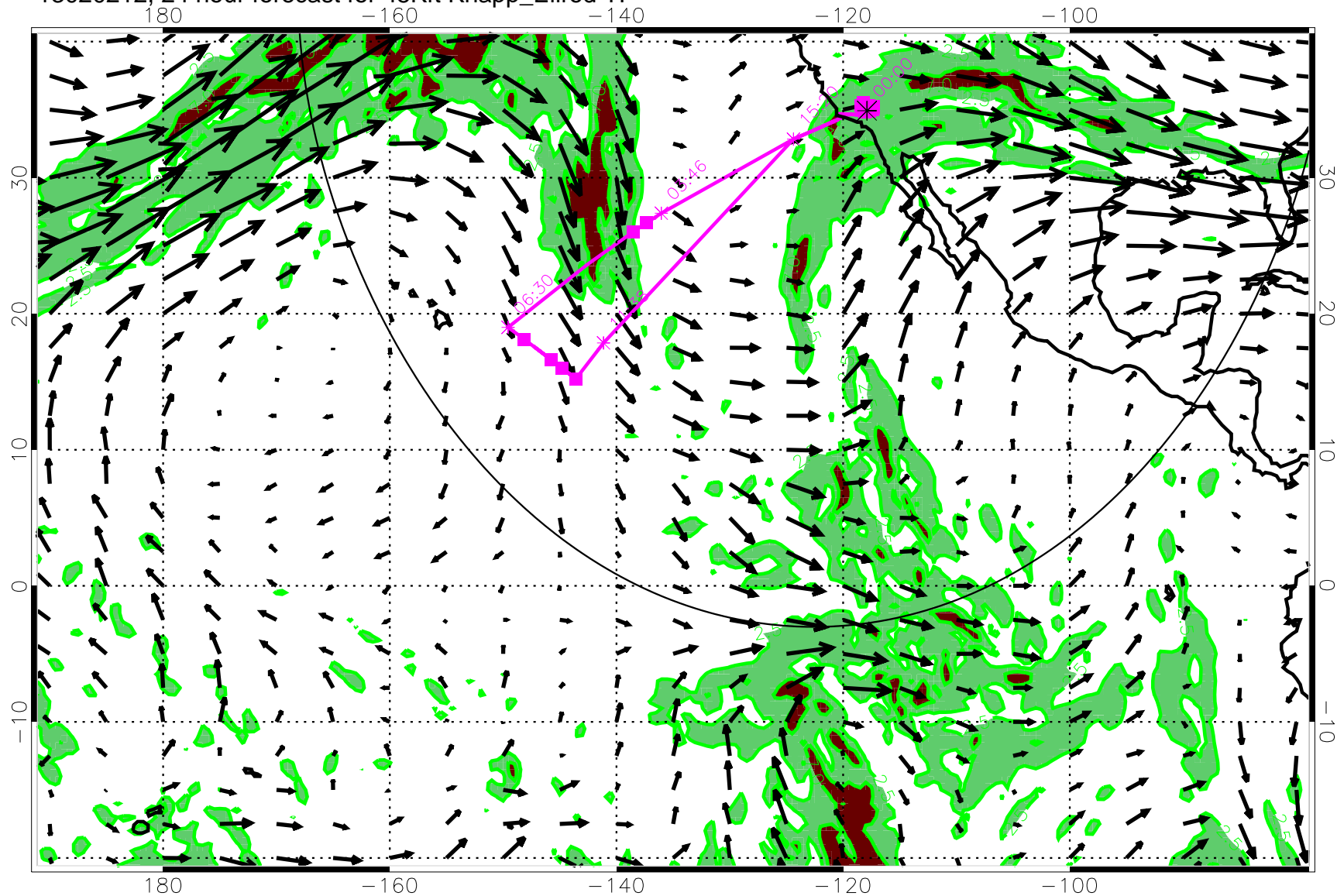
13020212, 24 hour forecast for 45Kft Knapp_Ellrod TI
