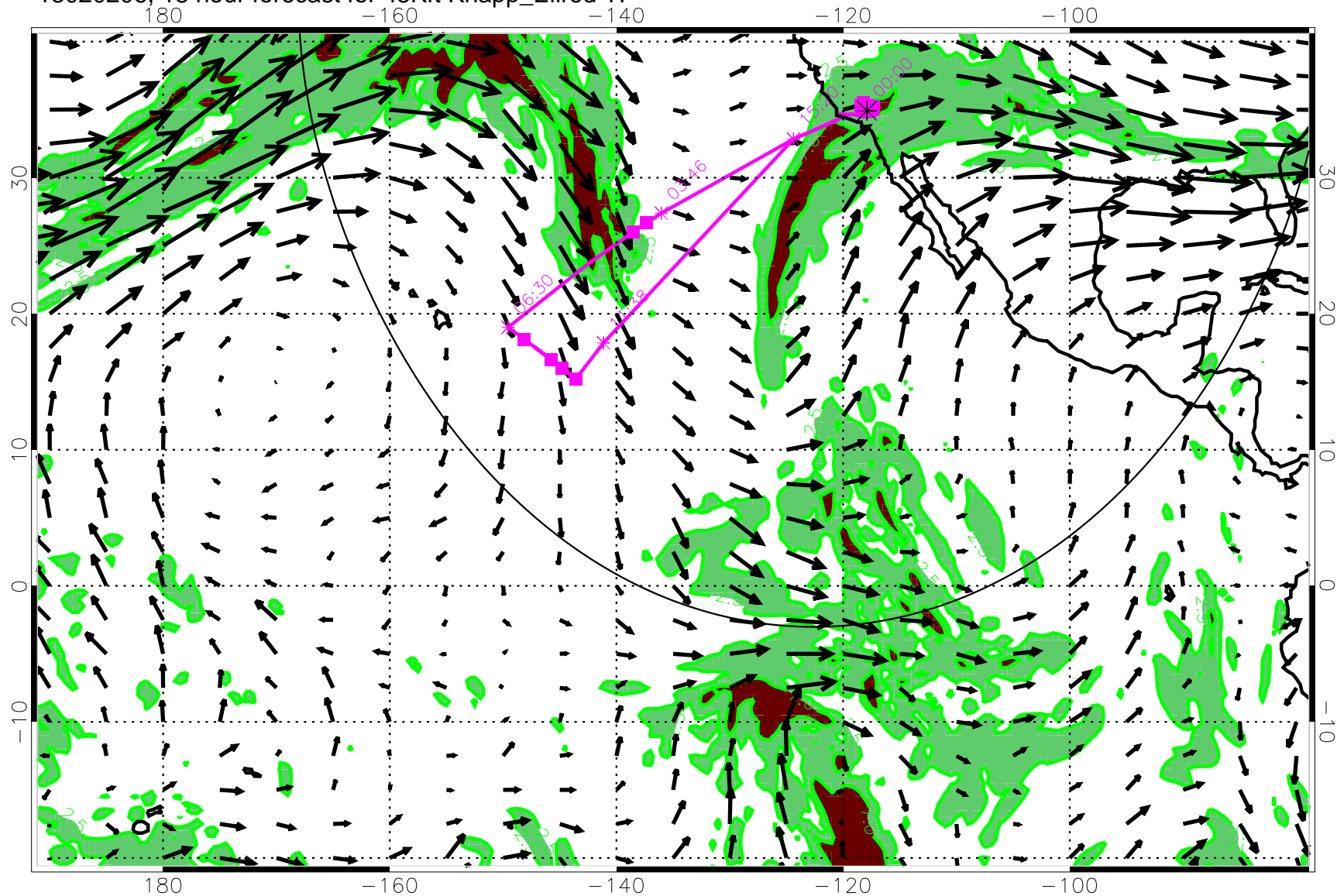
13020206, 18 hour forecast for 45Kft Knapp_Ellrod TI
