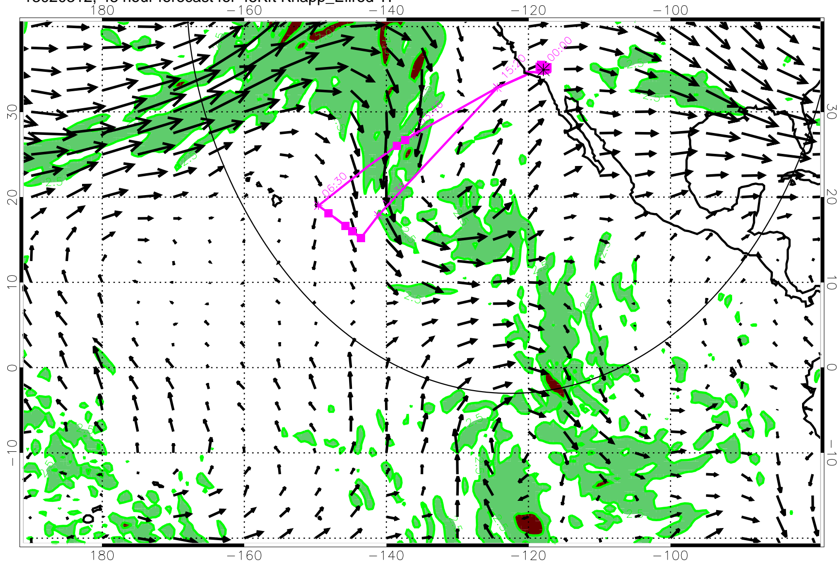
13020312, 48 hour forecast for 45Kft Knapp_Ellrod TI
