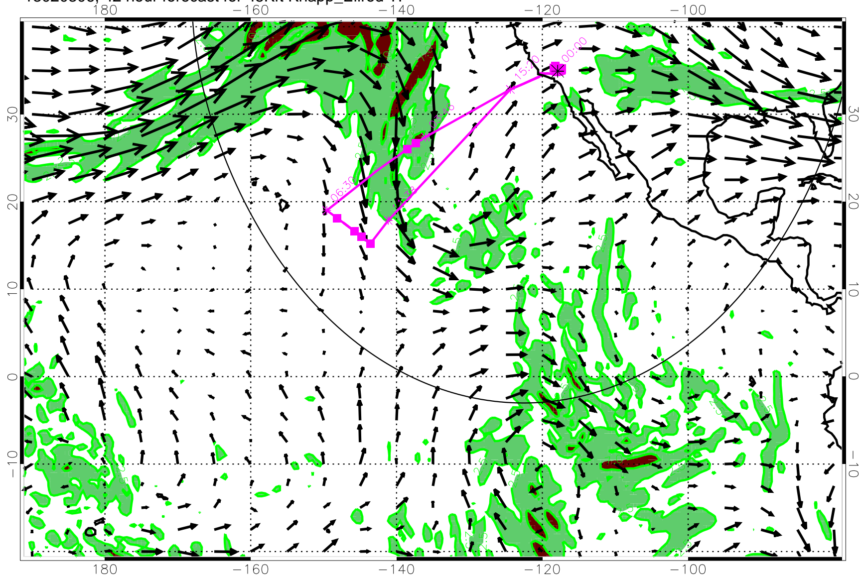
13020306, 42 hour forecast for 45Kft Knapp_Ellrod TI
