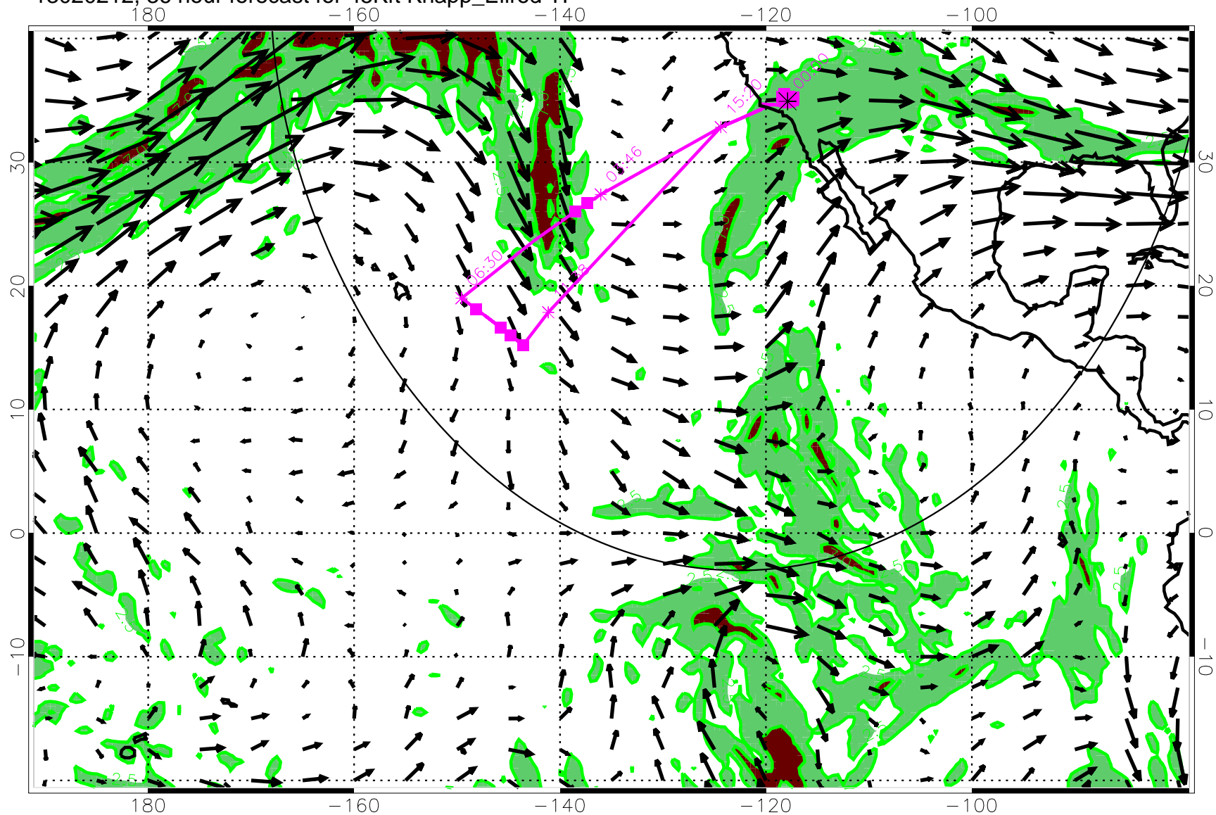
13020212, 36 hour forecast for 45Kft Knapp_Ellrod TI
