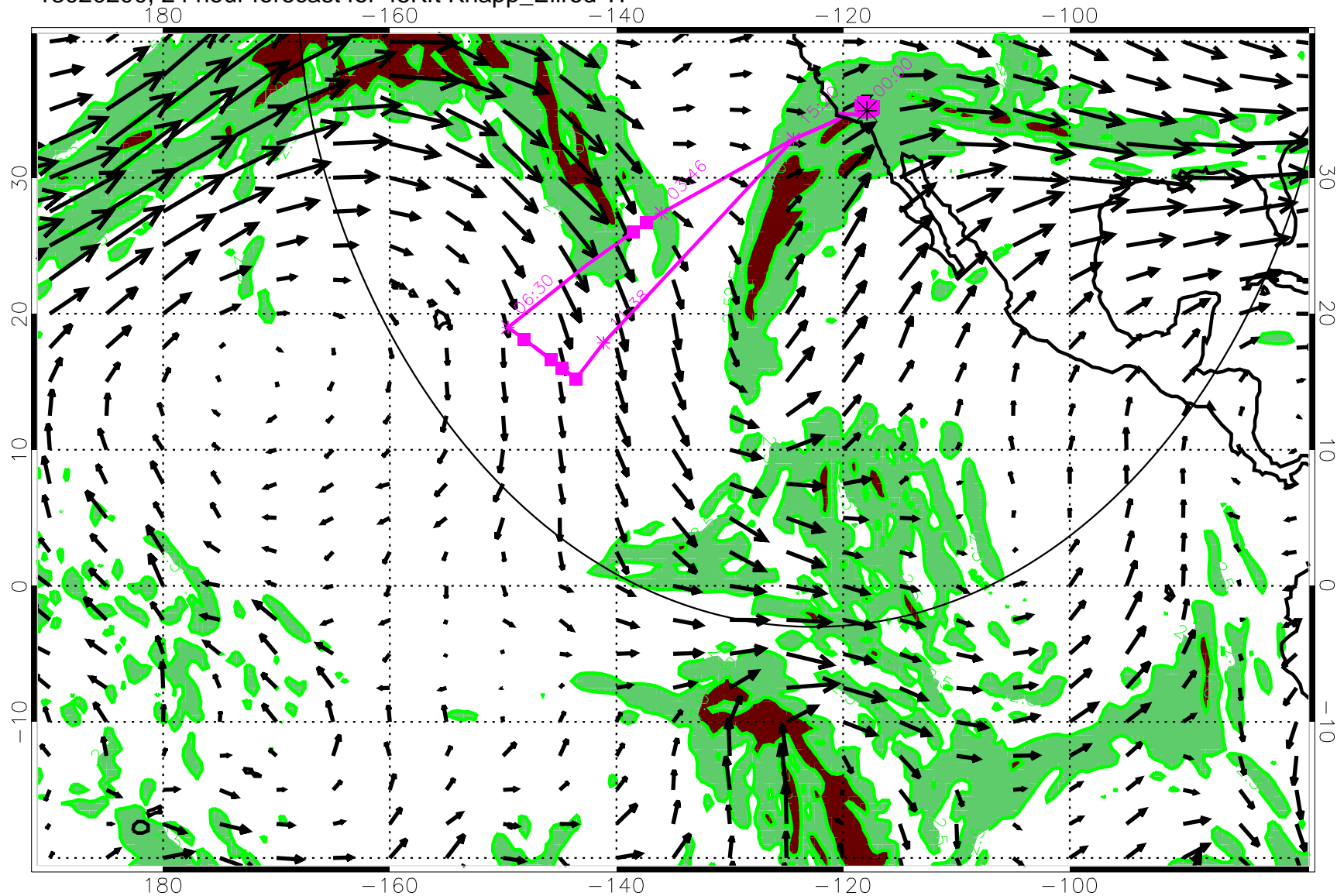
13020200, 24 hour forecast for 45Kft Knapp_Ellrod TI
