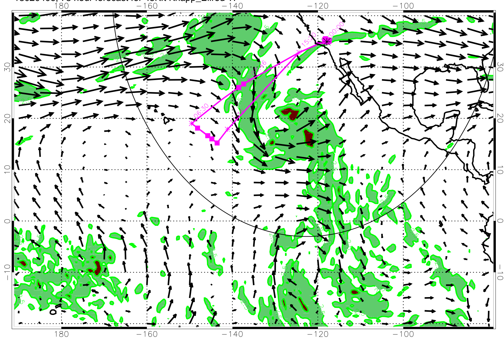
13020406, 78 hour forecast for 45Kft Knapp_Ellrod TI
