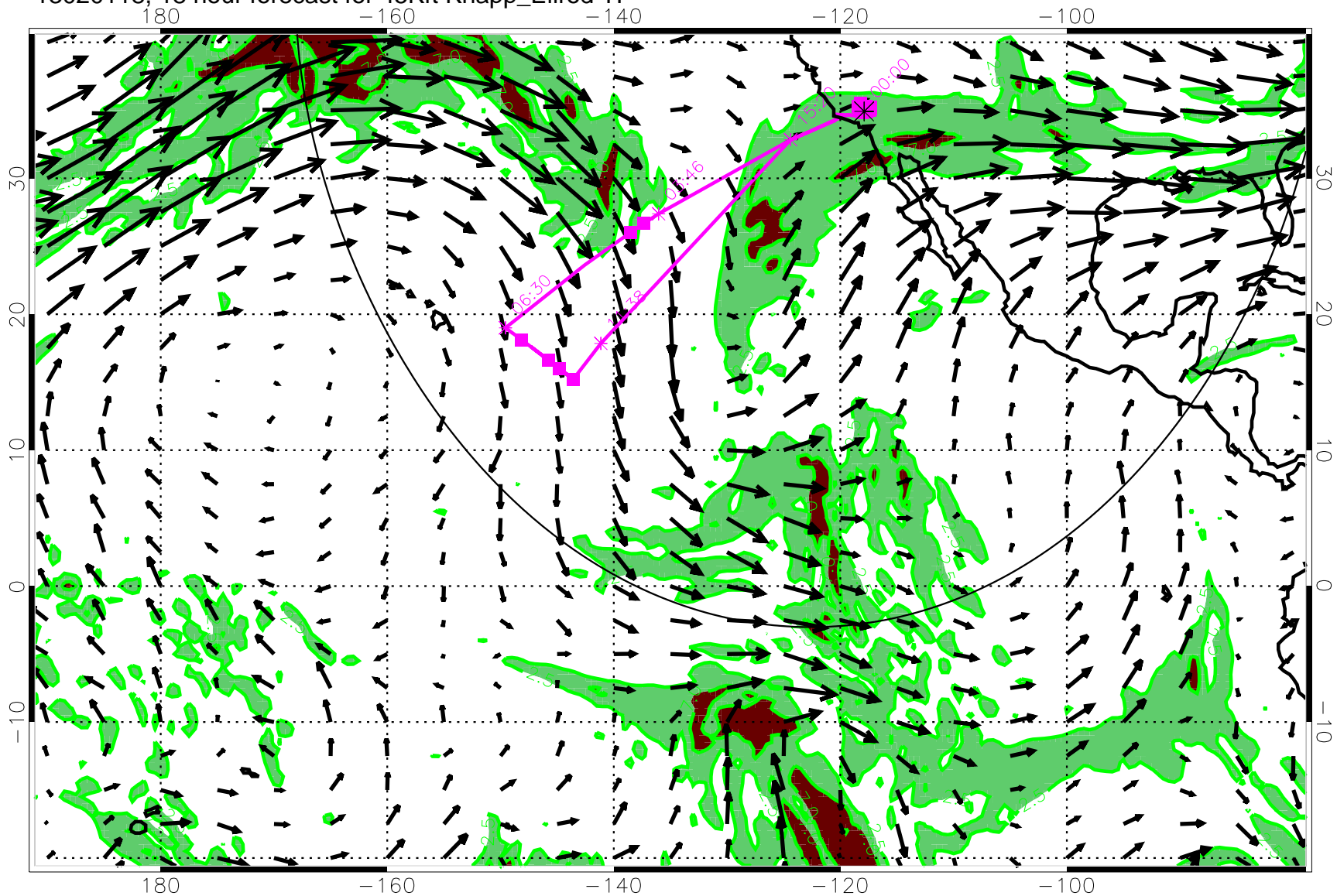
13020118, 18 hour forecast for 45Kft Knapp_Ellrod TI
