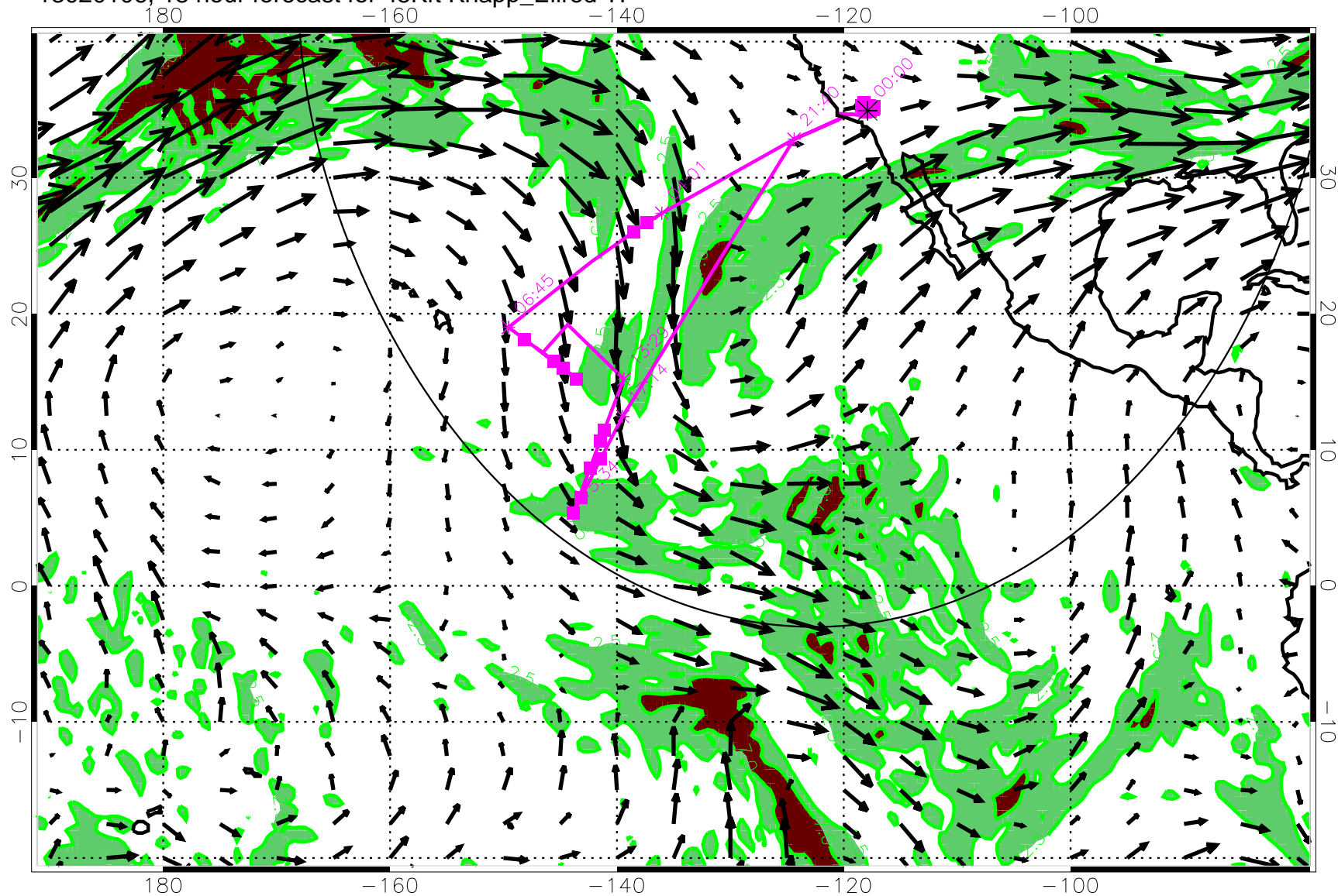
13020106, 18 hour forecast for 45Kft Knapp_Ellrod TI
