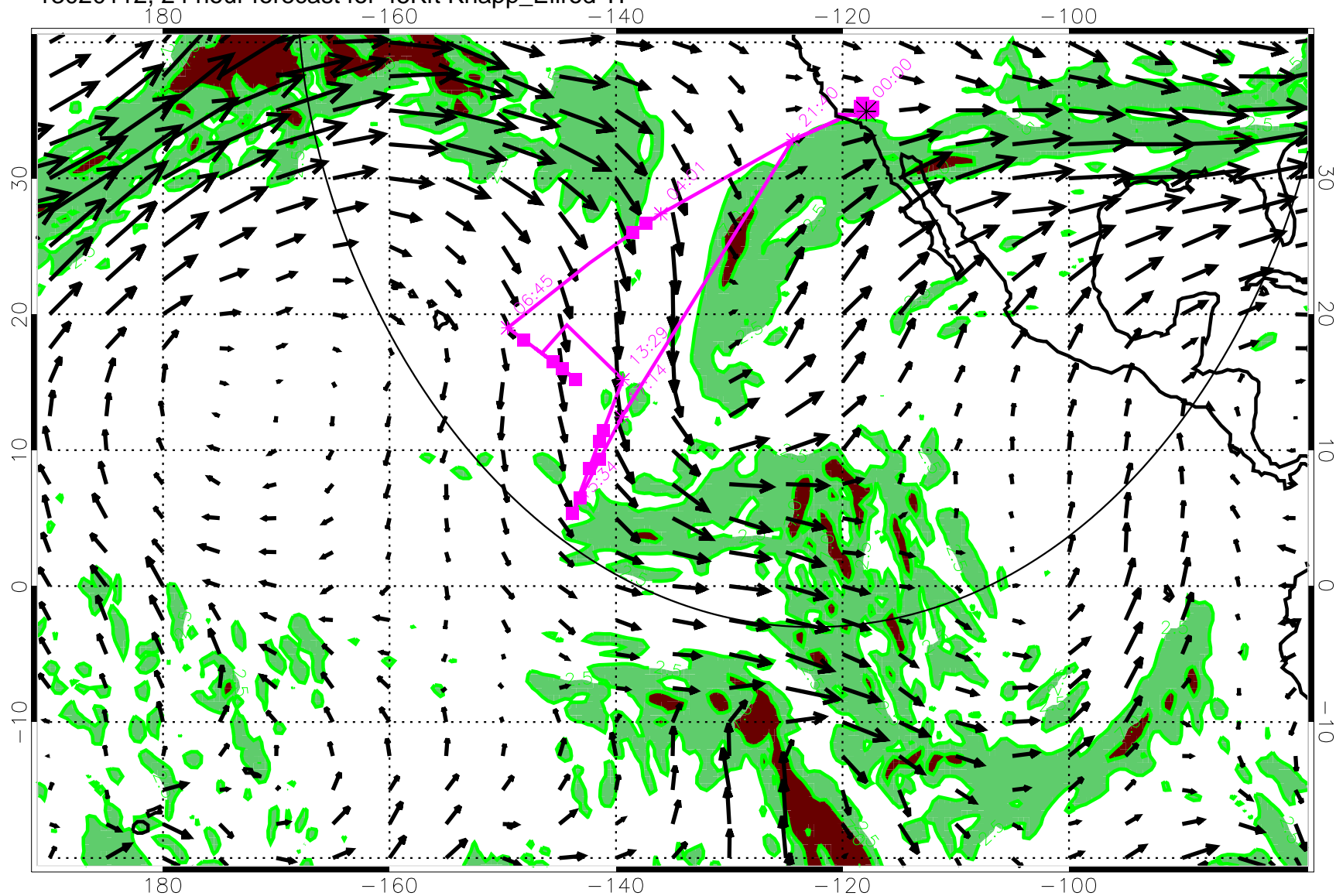
13020112, 24 hour forecast for 45Kft Knapp_Ellrod TI
