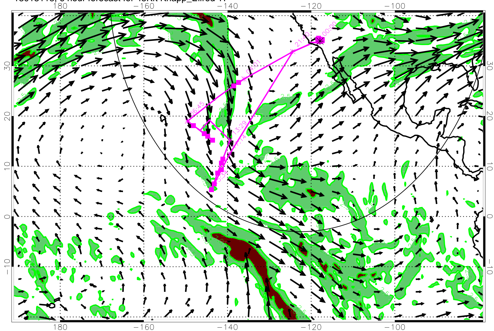
13013118, 6 hour forecast for 45Kft Knapp_Ellrod TI
