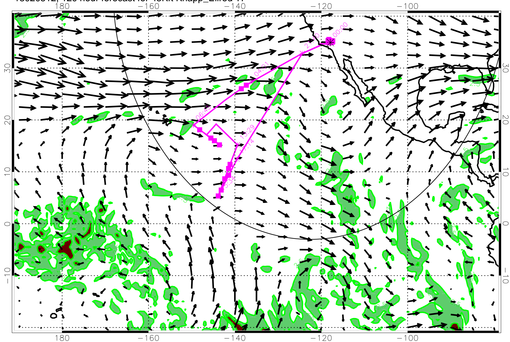
13020512, 120 hour forecast for 45Kft Knapp_Ellrod TI
