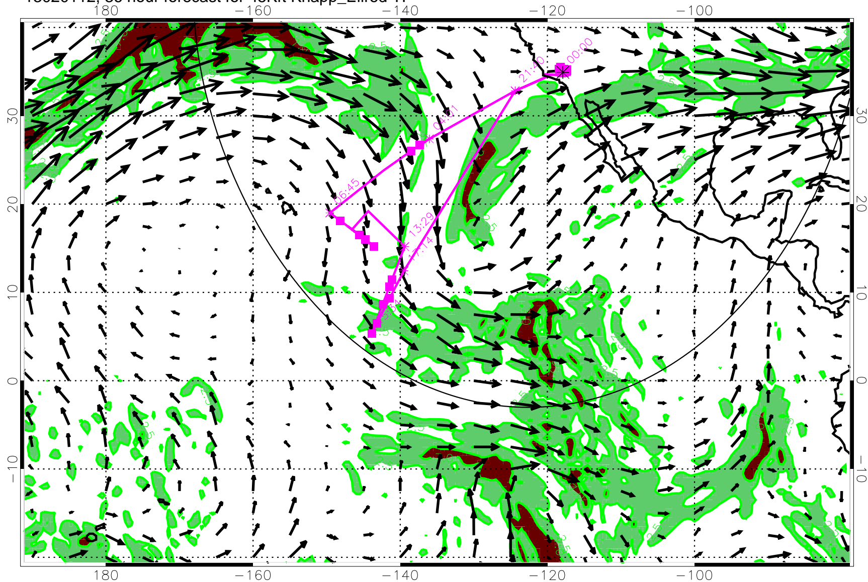
13020112, 36 hour forecast for 45Kft Knapp_Ellrod TI
