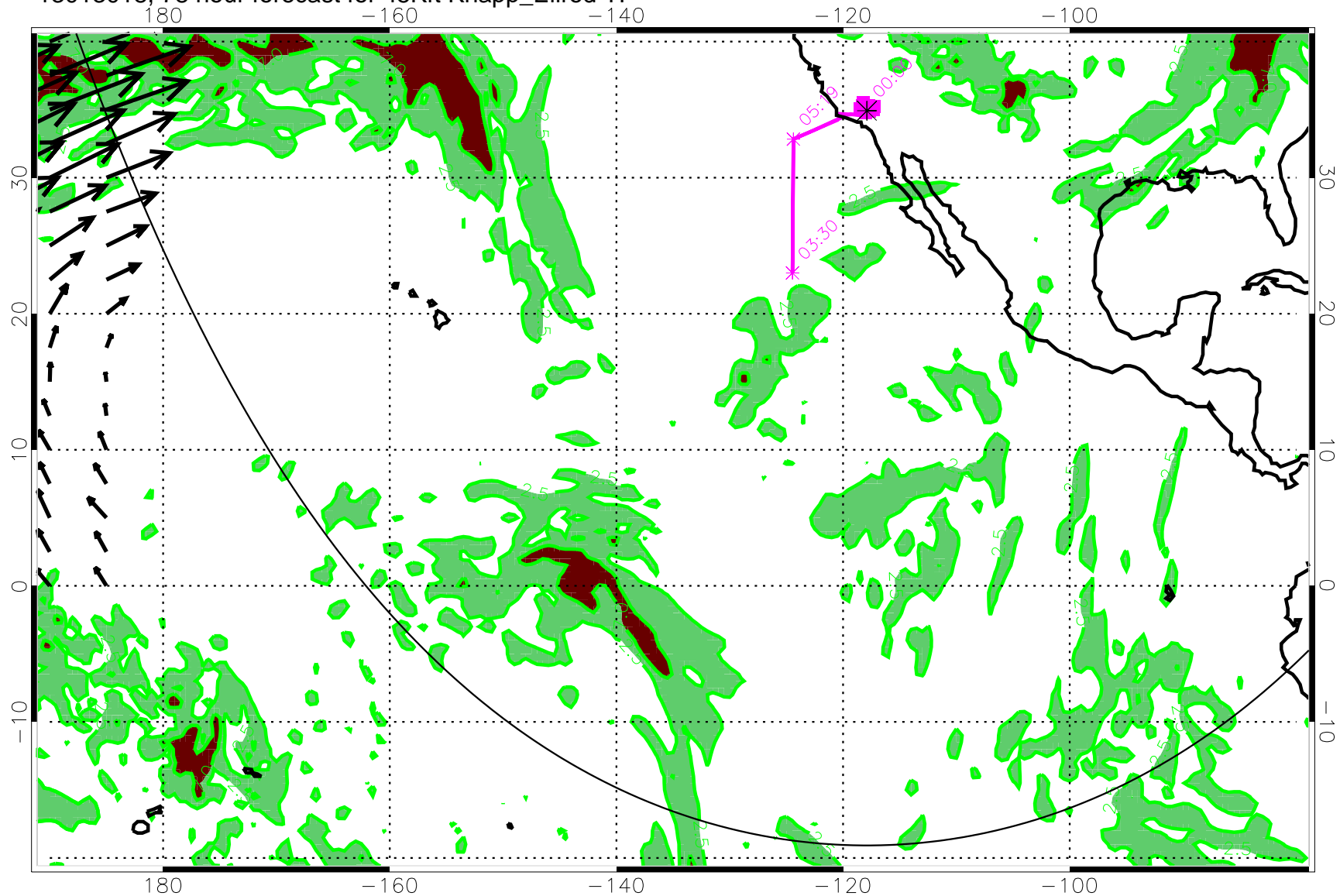
13013018, 78 hour forecast for 45Kft Knapp_Ellrod TI
