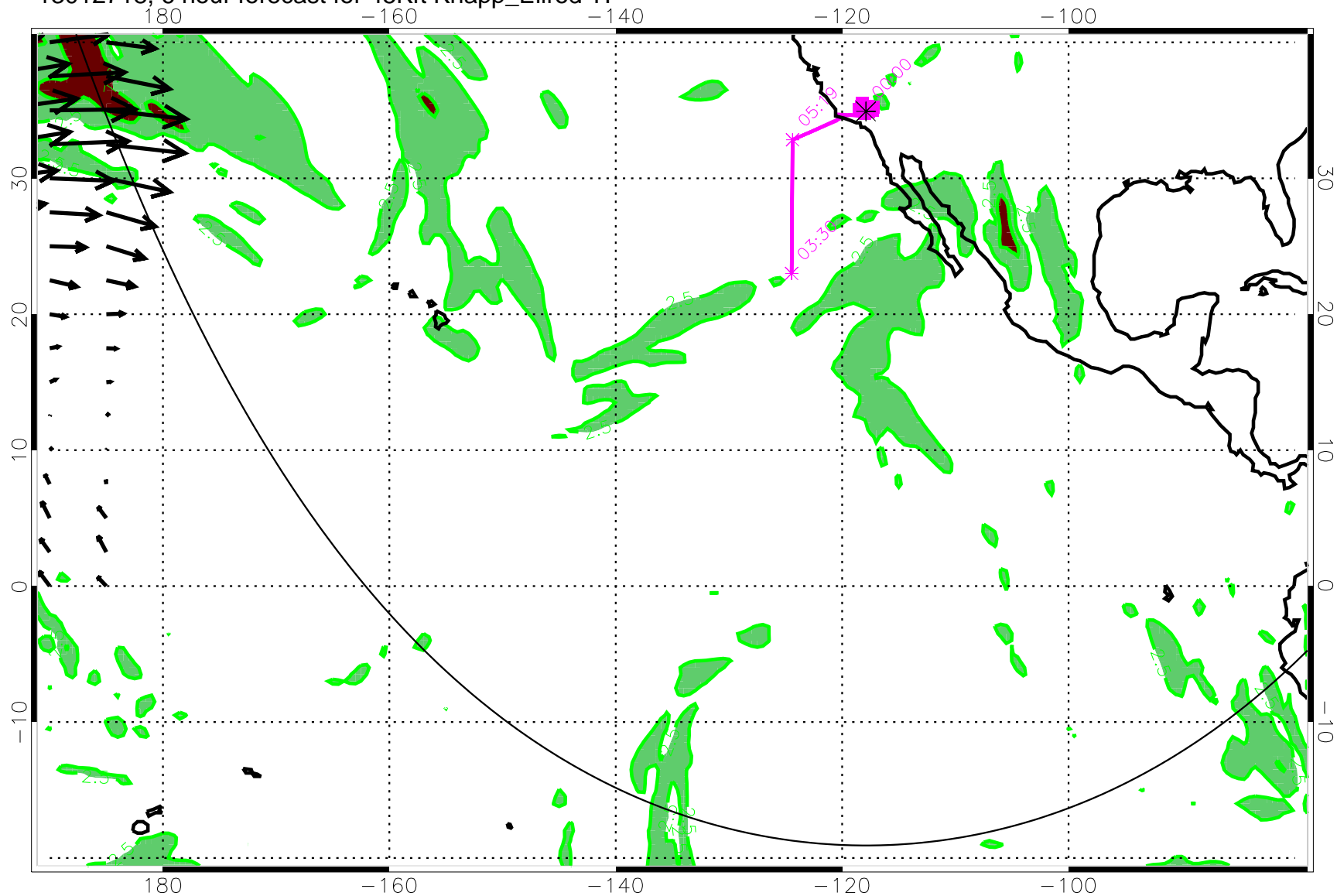
13012718, 6 hour forecast for 45Kft Knapp_Ellrod TI
