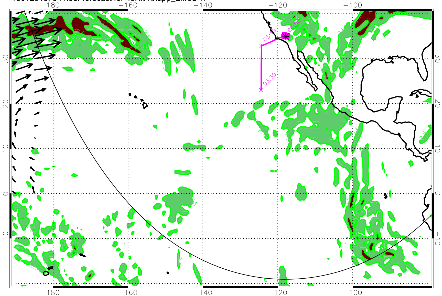
13012918, 54 hour forecast for 45Kft Knapp_Ellrod TI
