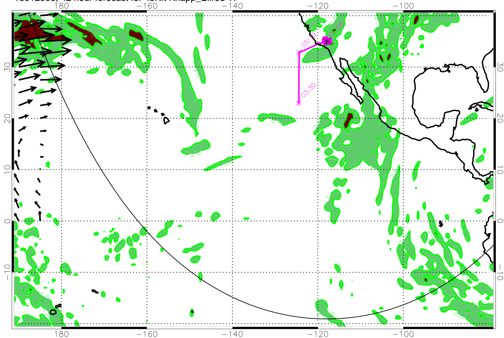
13012906, 42 hour forecast for 45Kft Knapp_Ellrod TI
