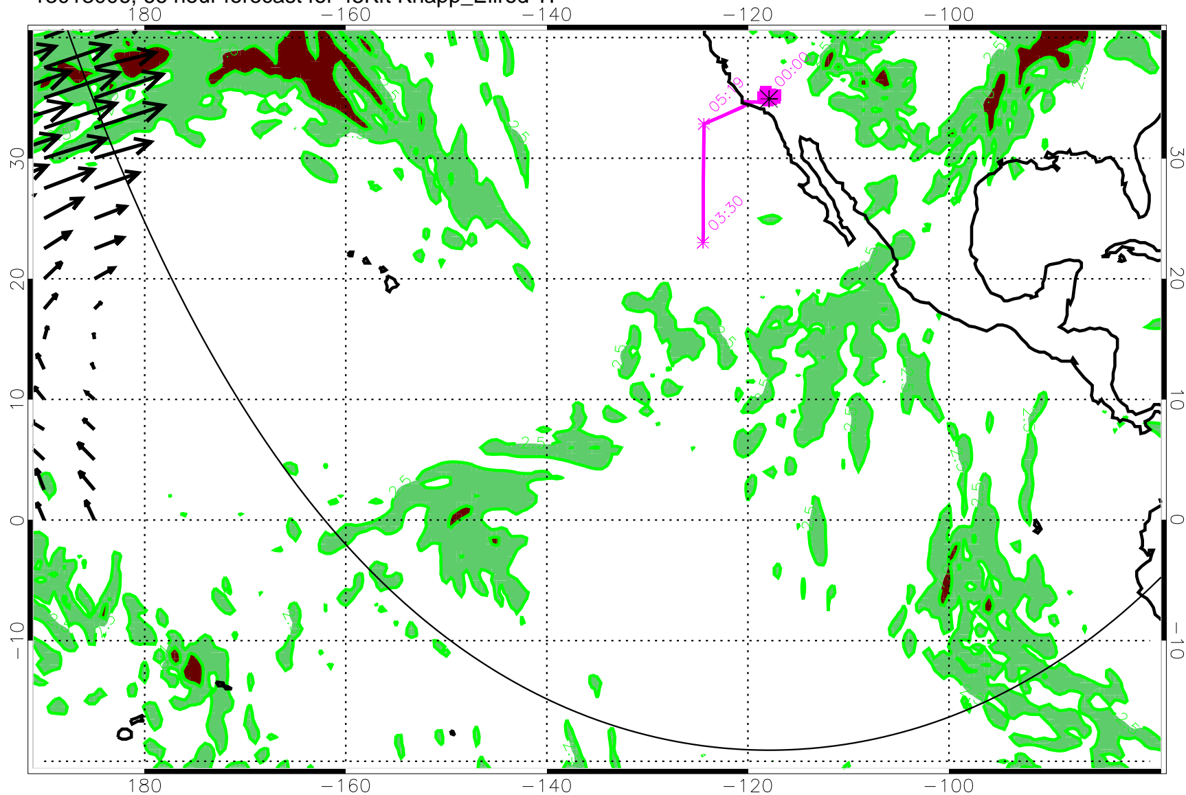
13013006, 66 hour forecast for 45Kft Knapp_Ellrod TI
