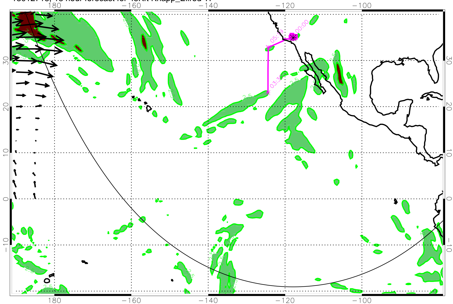
13012718, 18 hour forecast for 45Kft Knapp_Ellrod TI
