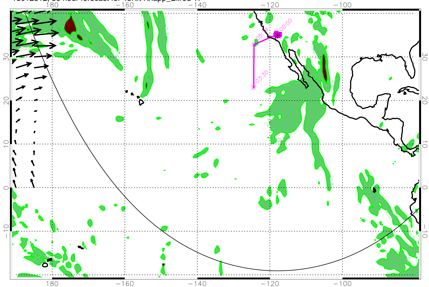
13012812, 36 hour forecast for 45Kft Knapp_Ellrod TI
