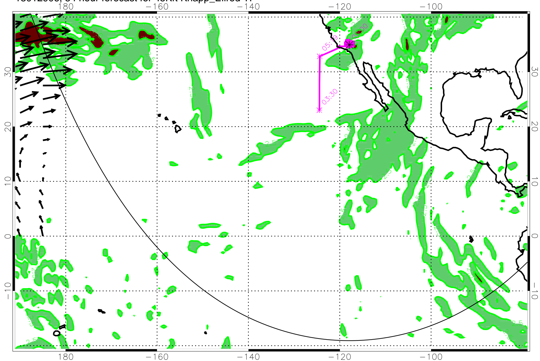
13012906, 54 hour forecast for 45Kft Knapp_Ellrod TI
