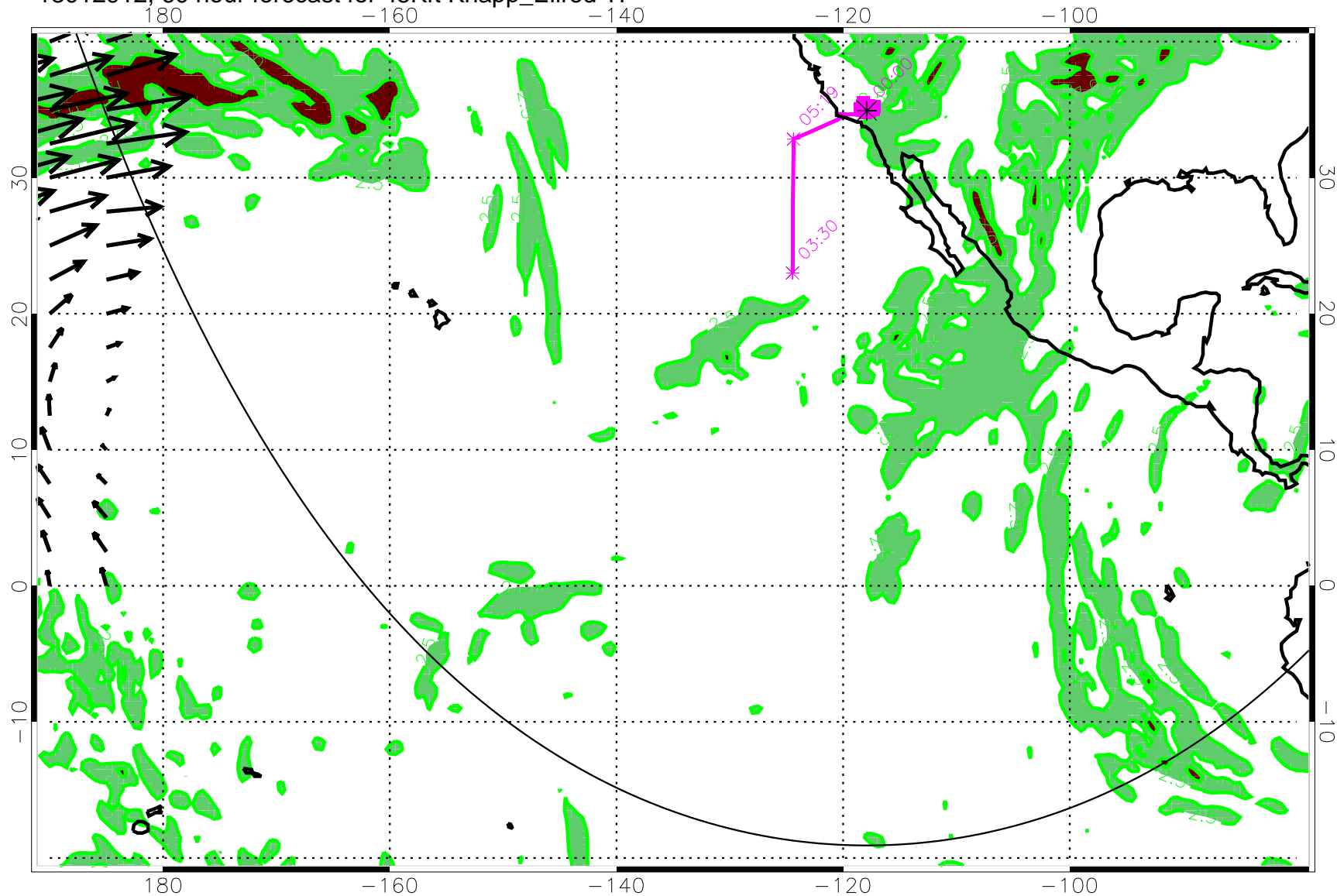
13012912, 60 hour forecast for 45Kft Knapp_Ellrod TI
