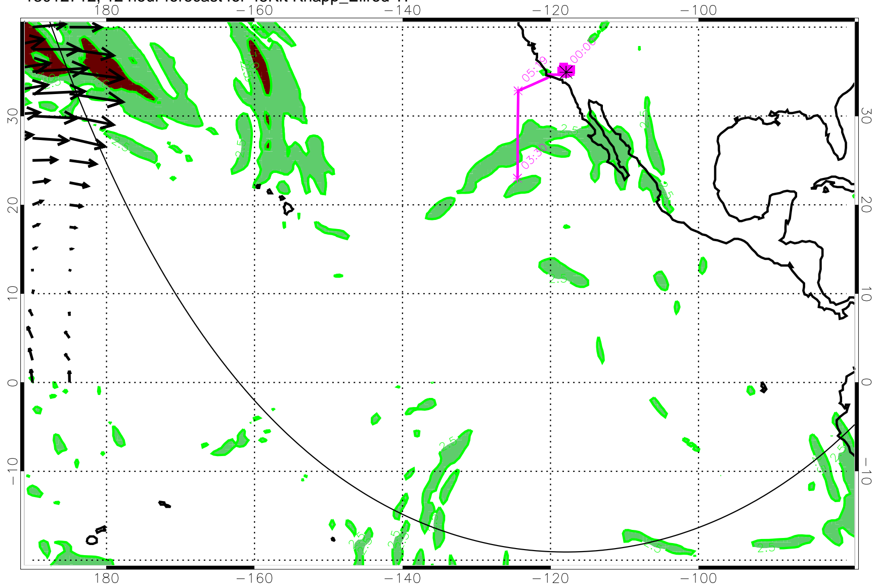
13012712, 12 hour forecast for 45Kft Knapp_Ellrod TI
