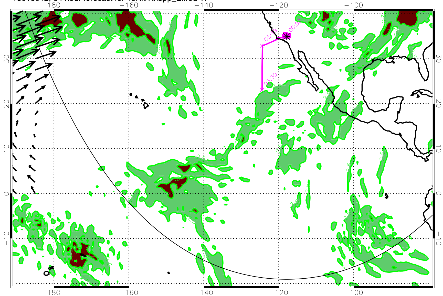
13013012, 84 hour forecast for 45Kft Knapp_Ellrod TI
