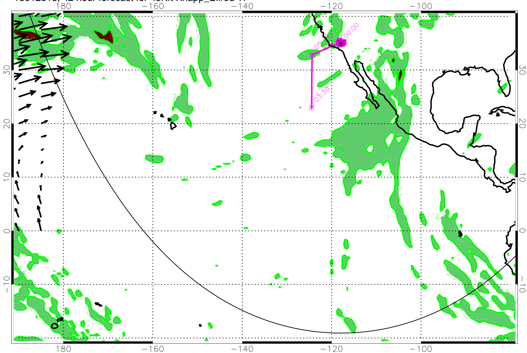
13012818, 42 hour forecast for 45Kft Knapp_Ellrod TI
