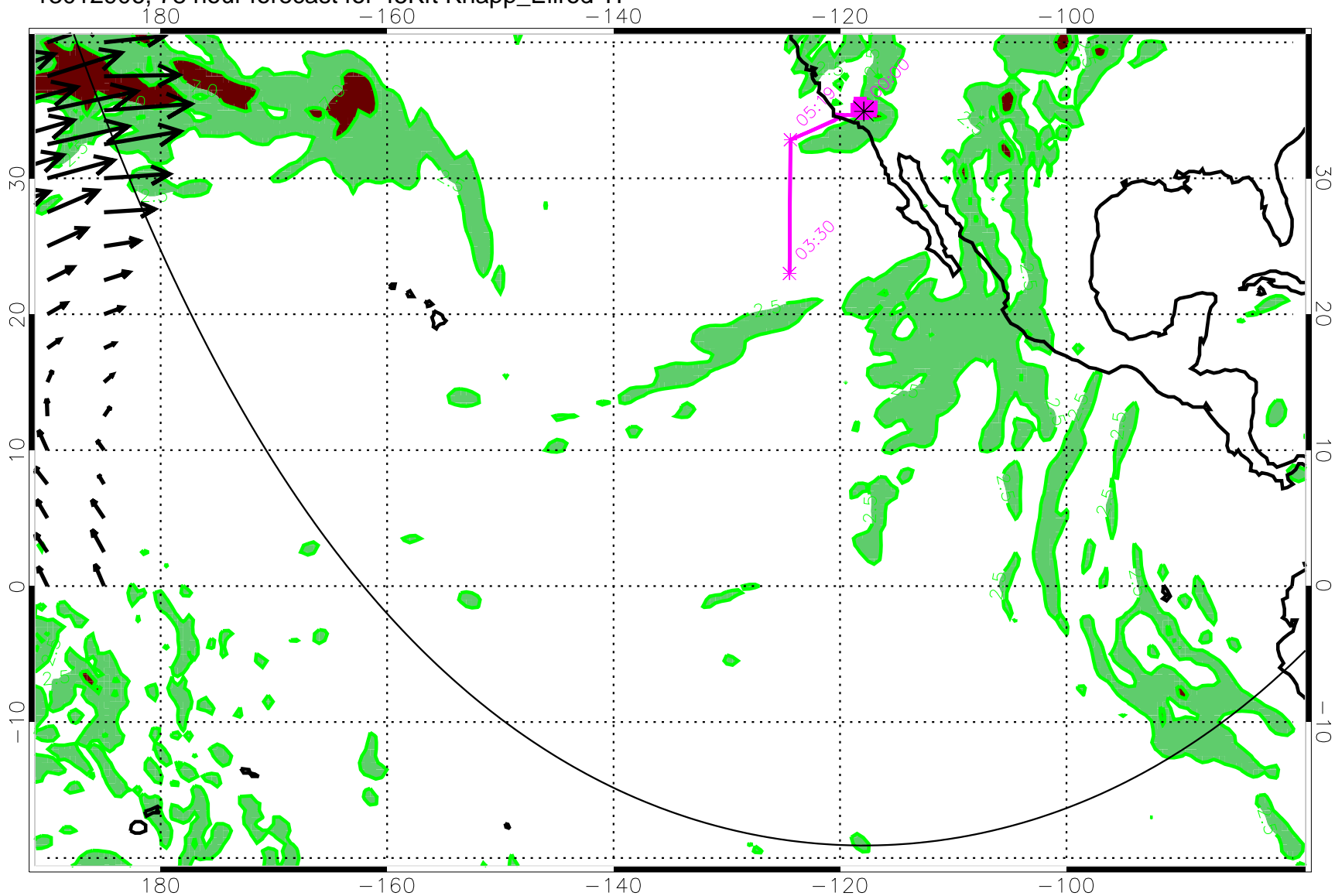
13012906, 78 hour forecast for 45Kft Knapp_Ellrod TI
