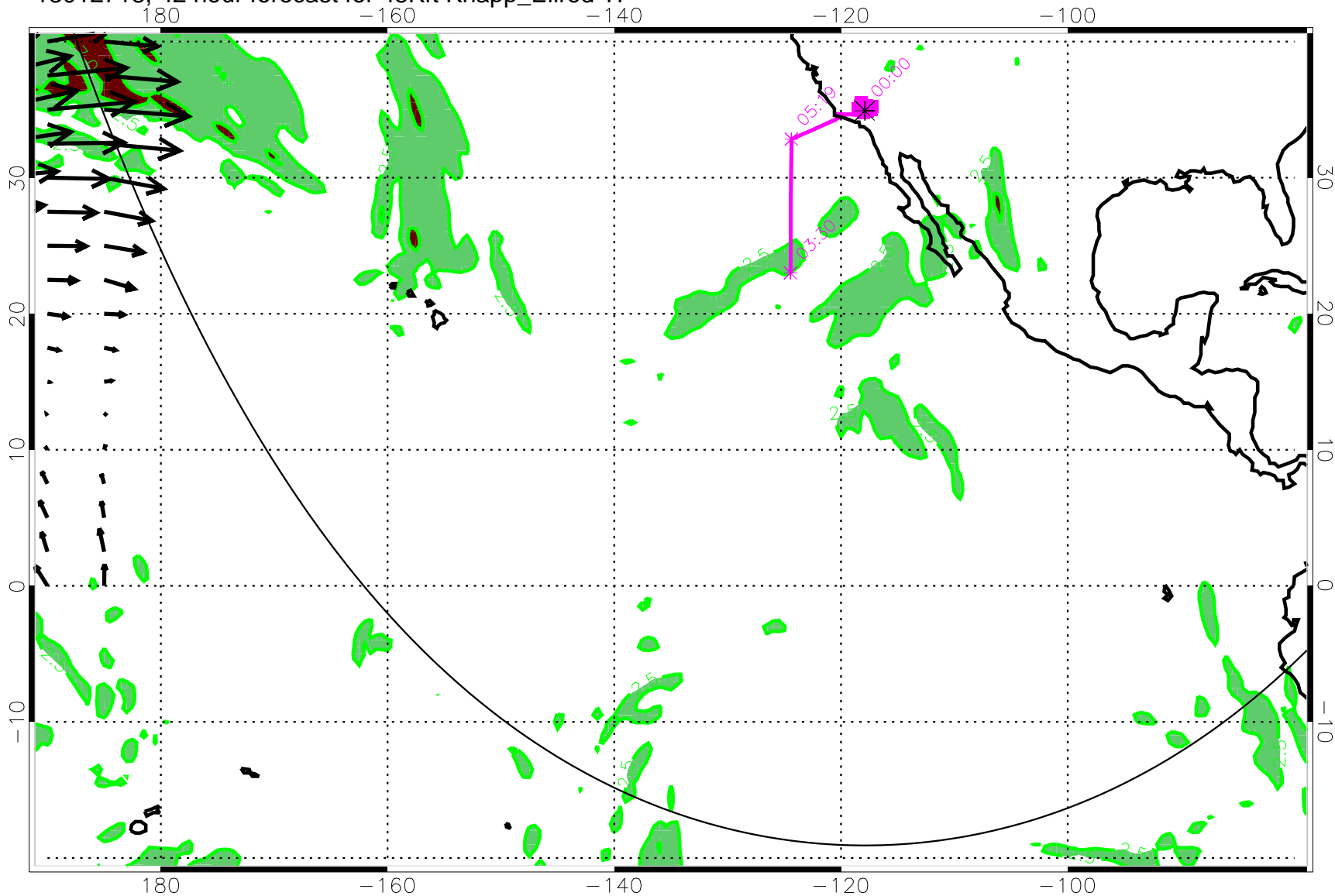
13012718, 42 hour forecast for 45Kft Knapp_Ellrod TI
