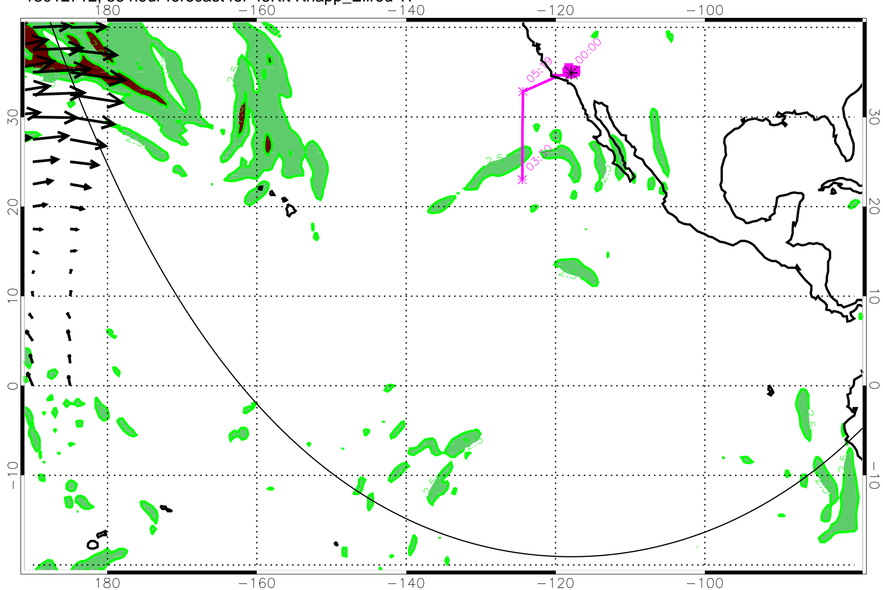
13012712, 36 hour forecast for 45Kft Knapp_Ellrod TI
