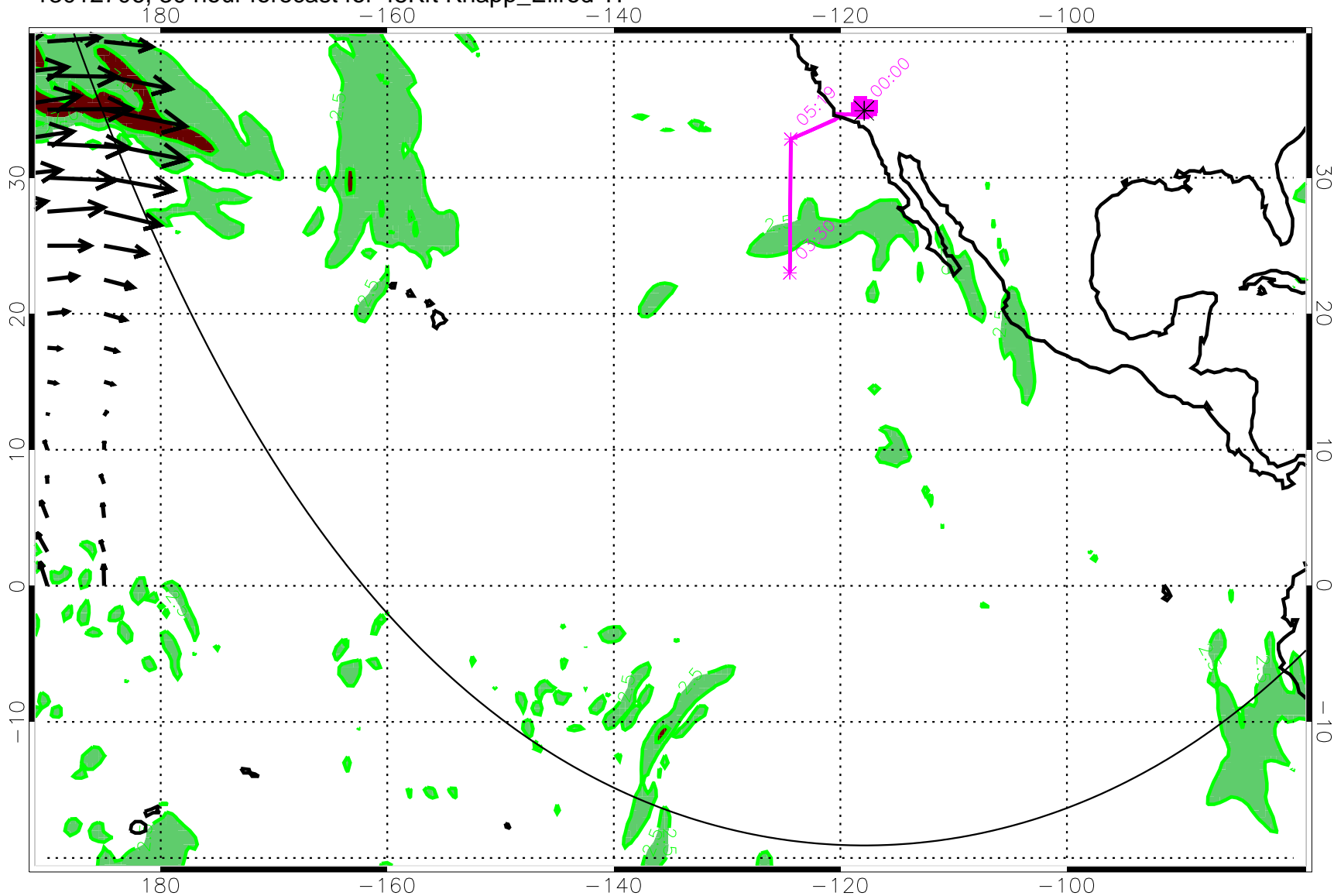
13012706, 30 hour forecast for 45Kft Knapp_Ellrod TI
