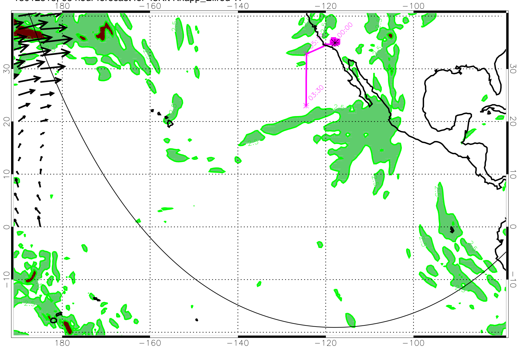
13012818, 66 hour forecast for 45Kft Knapp_Ellrod TI
