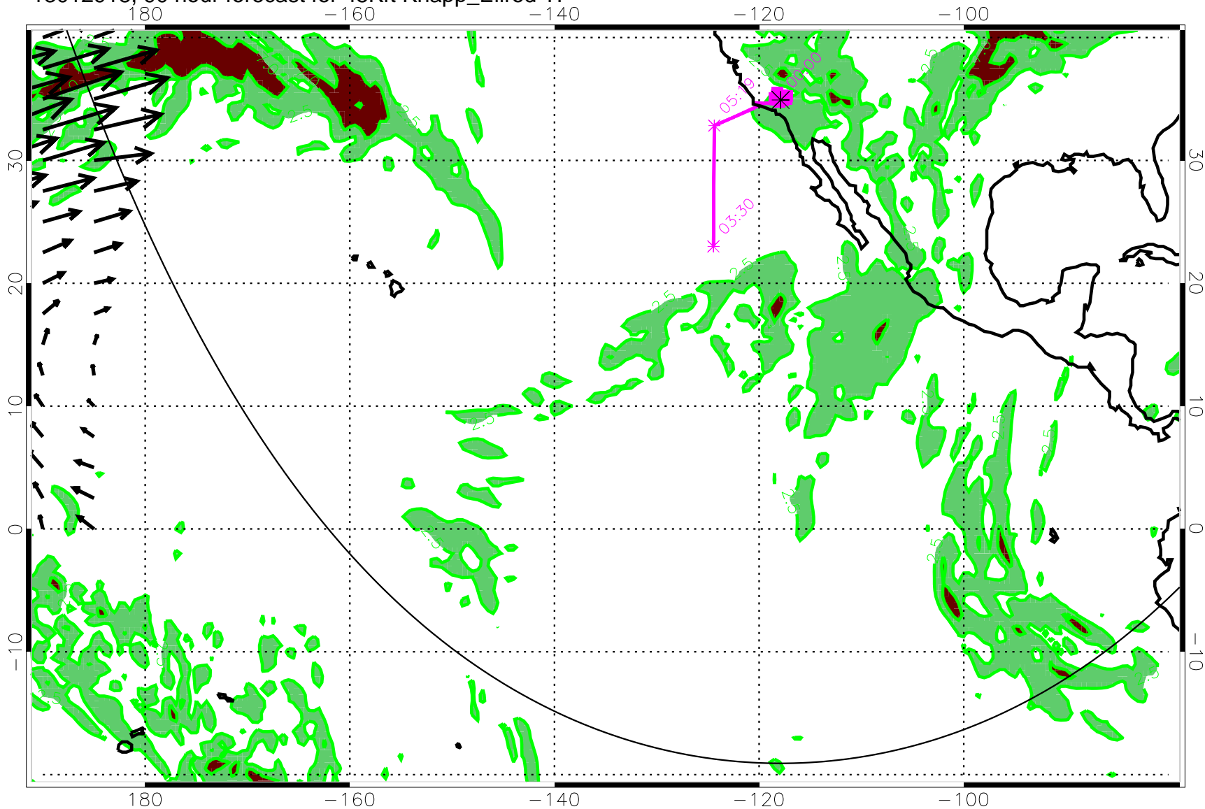
13012918, 90 hour forecast for 45Kft Knapp_Ellrod TI
