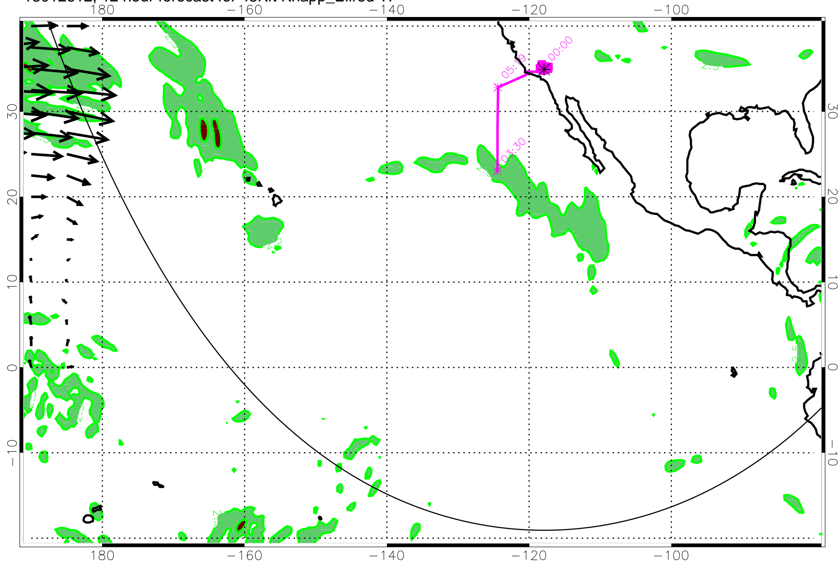
13012612, 12 hour forecast for 45Kft Knapp_Ellrod TI
