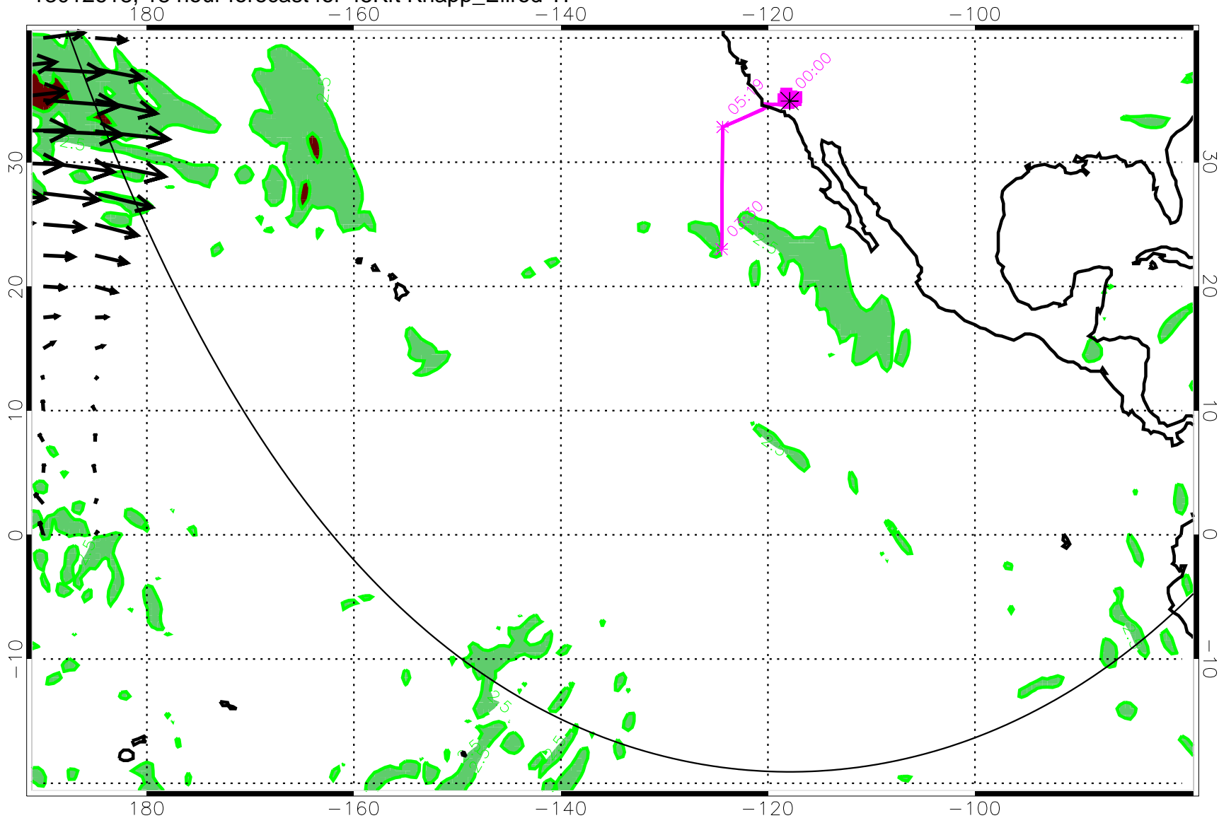
13012618, 18 hour forecast for 45Kft Knapp_Ellrod TI
