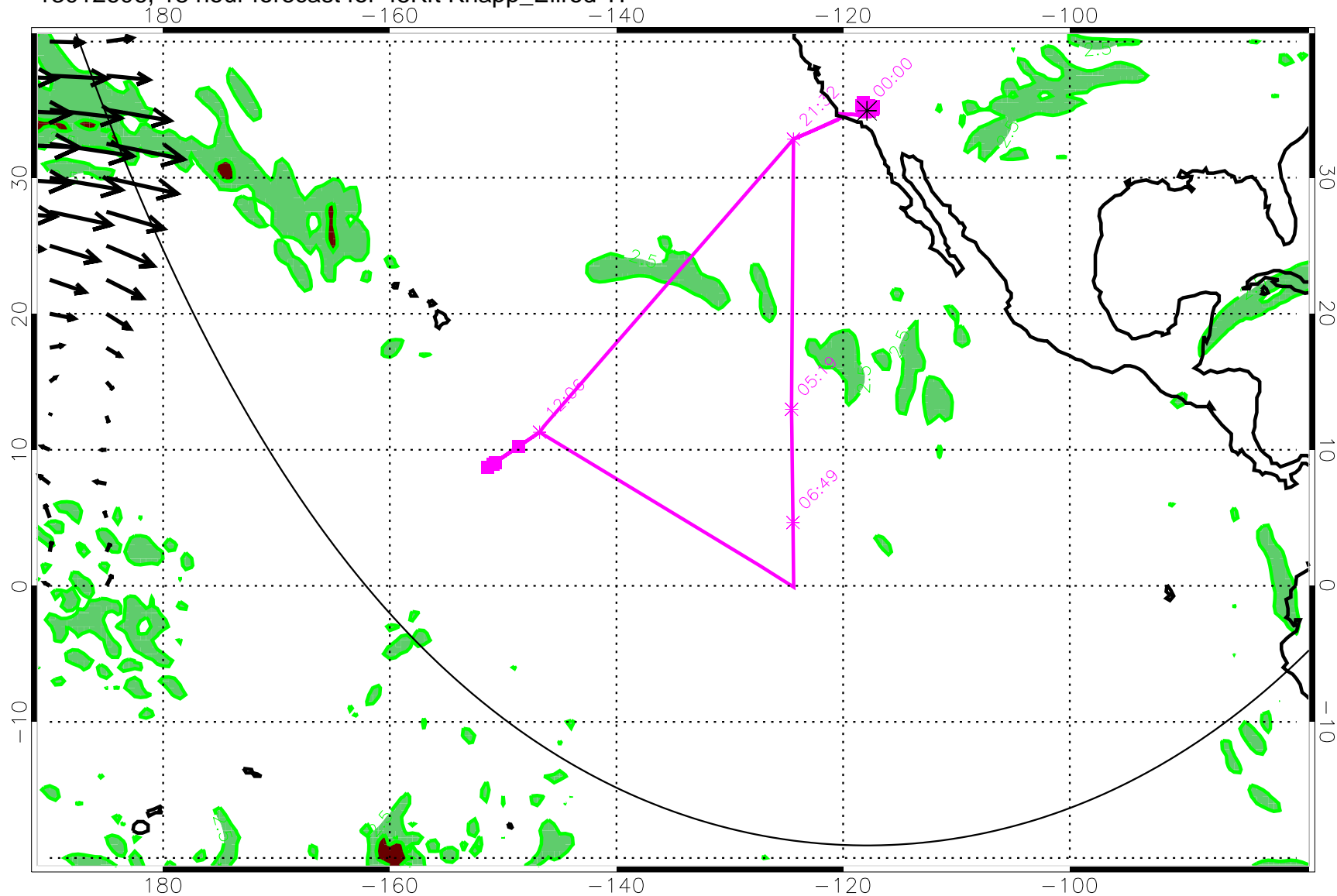
13012606, 18 hour forecast for 45Kft Knapp_Ellrod TI
