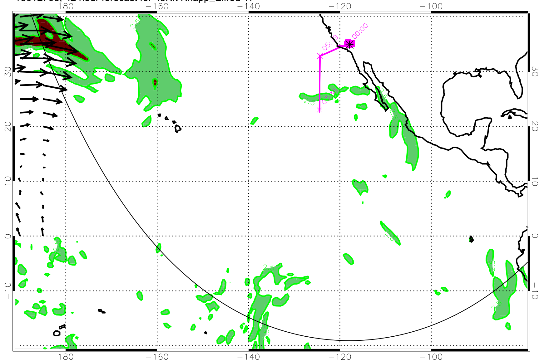
13012706, 42 hour forecast for 45Kft Knapp_Ellrod TI
