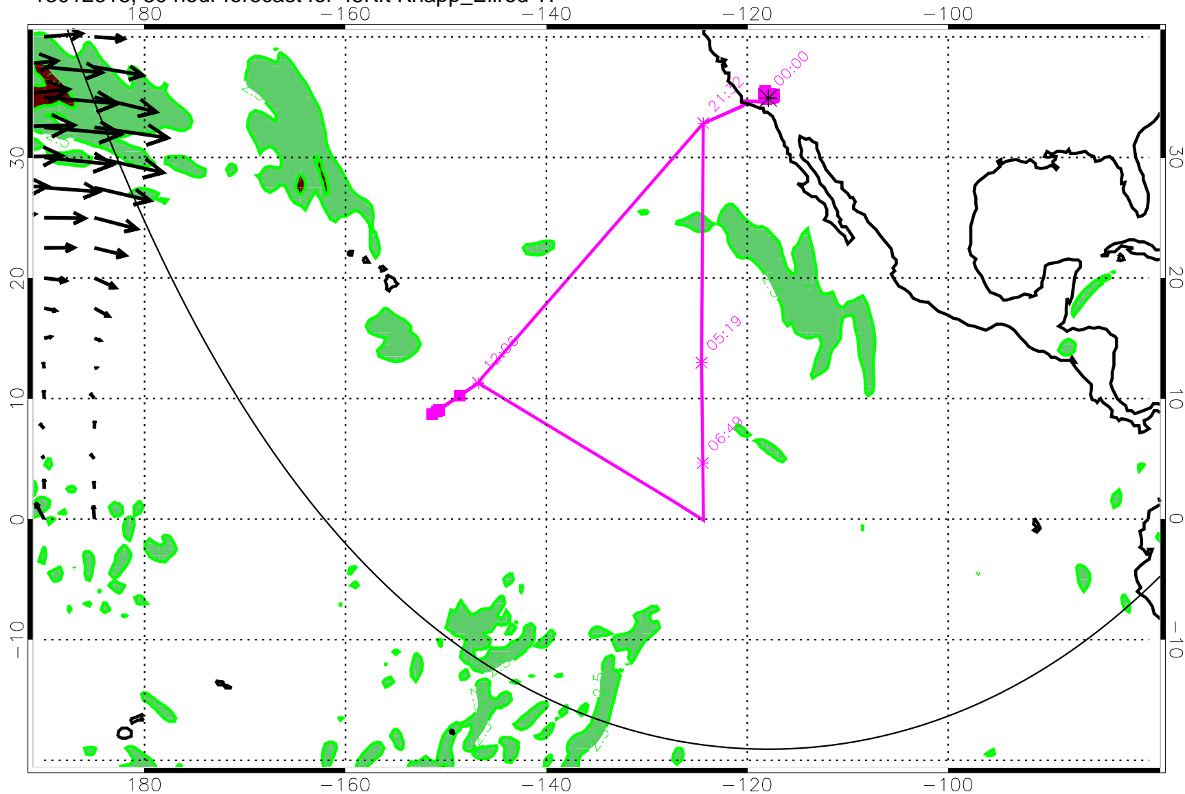
13012618, 30 hour forecast for 45Kft Knapp_Ellrod TI
