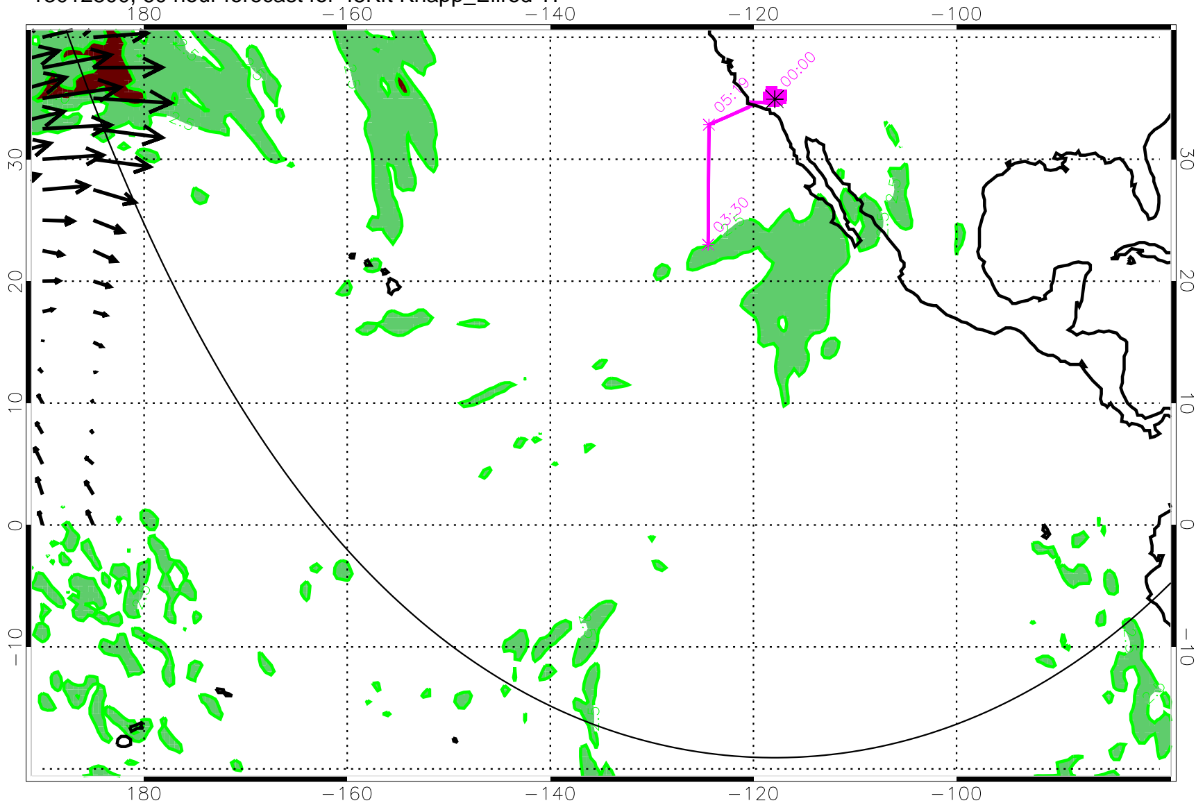
13012800, 60 hour forecast for 45Kft Knapp_Ellrod TI
