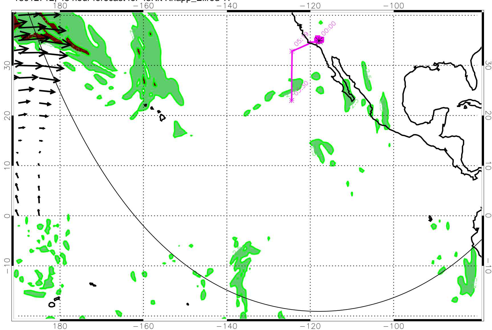
13012712, 48 hour forecast for 45Kft Knapp_Ellrod TI
