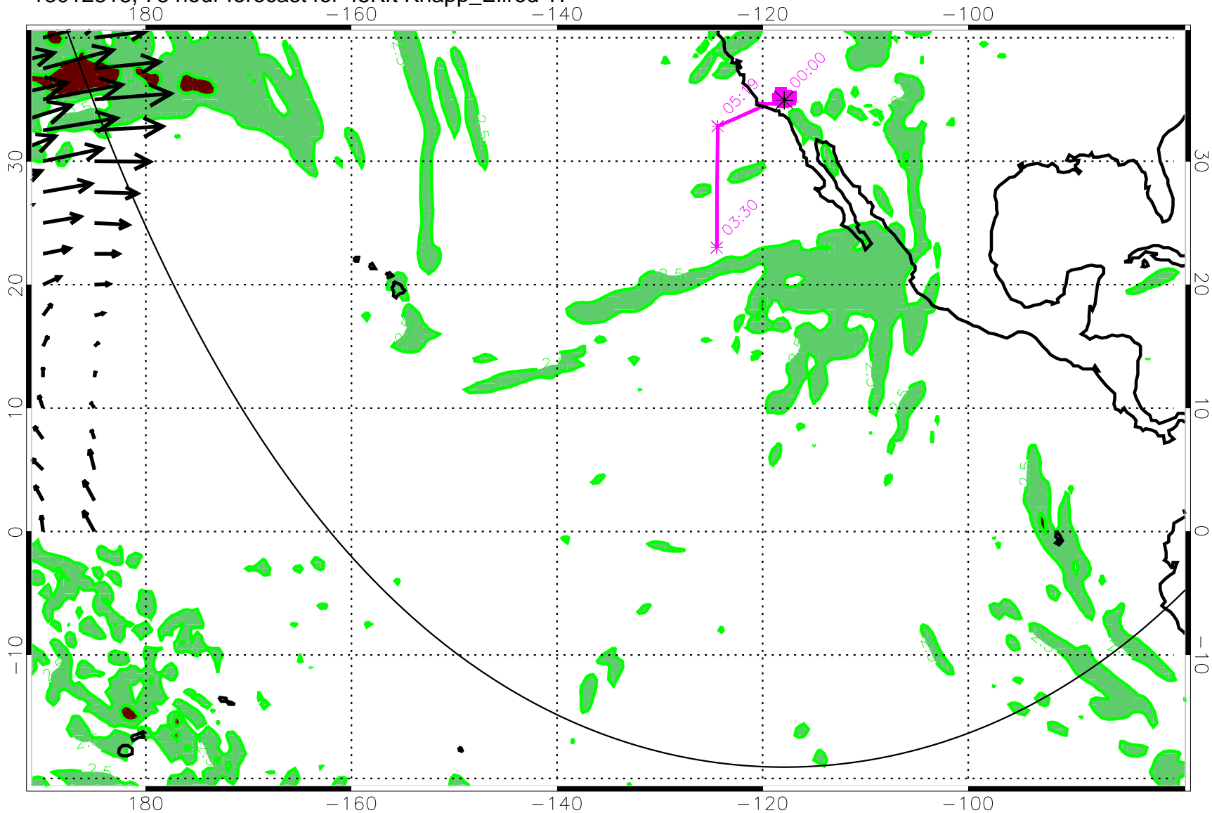
13012818, 78 hour forecast for 45Kft Knapp_Ellrod TI
