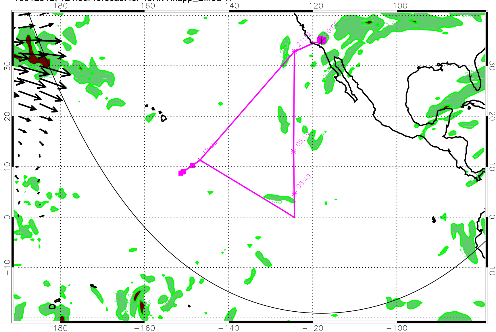
13012512, 12 hour forecast for 45Kft Knapp_Ellrod TI
