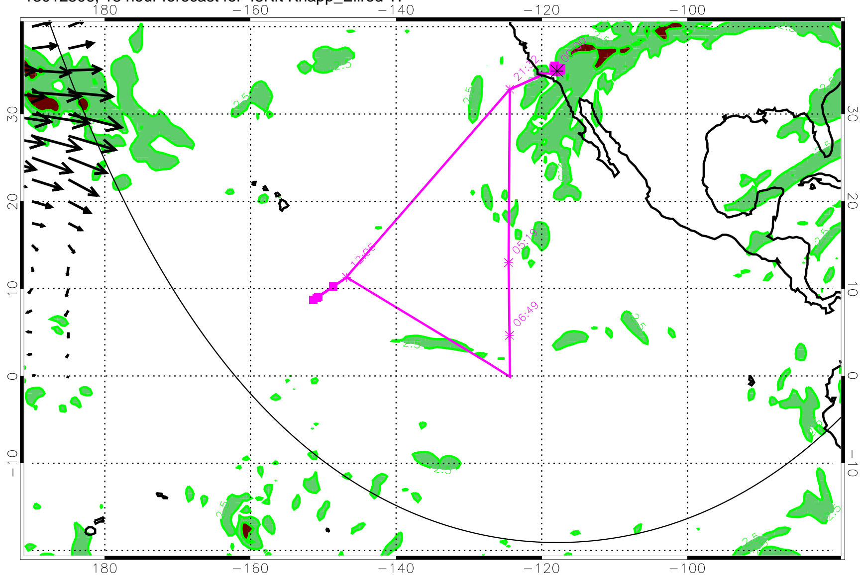
13012506, 18 hour forecast for 45Kft Knapp_Ellrod TI
