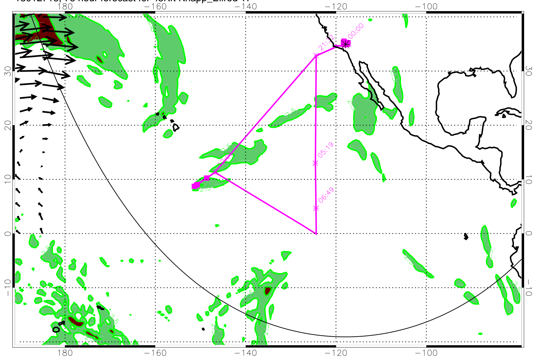
13012718, 78 hour forecast for 45Kft Knapp_Ellrod TI
