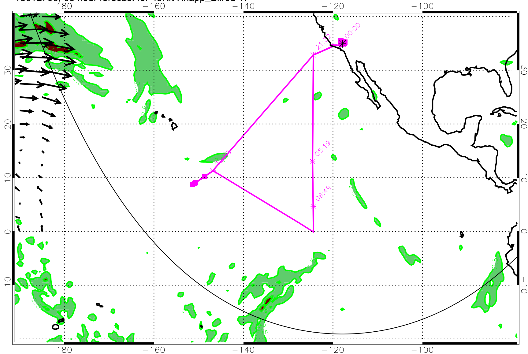
13012706, 66 hour forecast for 45Kft Knapp_Ellrod TI
