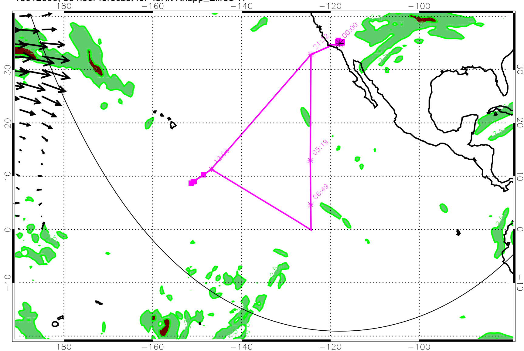
13012600, 36 hour forecast for 45Kft Knapp_Ellrod TI
