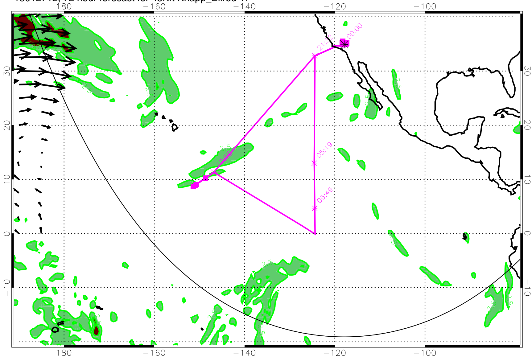
13012712, 72 hour forecast for 45Kft Knapp_Ellrod TI
