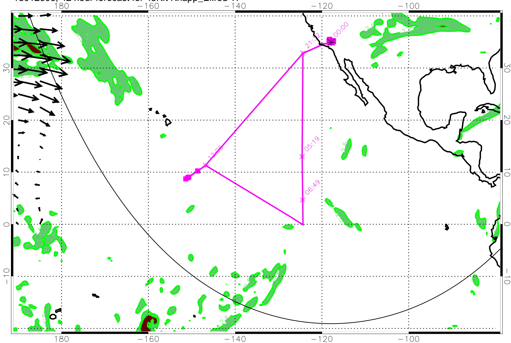
13012606, 42 hour forecast for 45Kft Knapp_Ellrod TI
