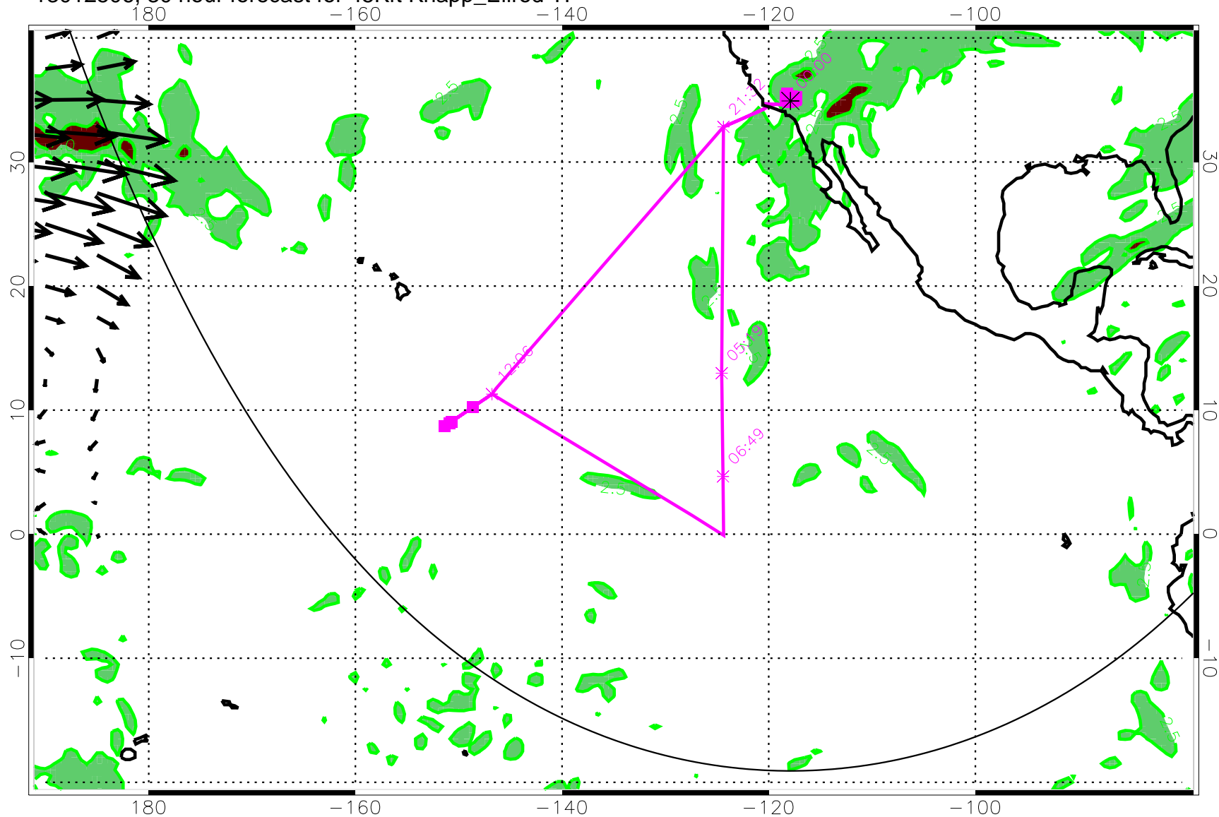
13012506, 30 hour forecast for 45Kft Knapp_Ellrod TI
