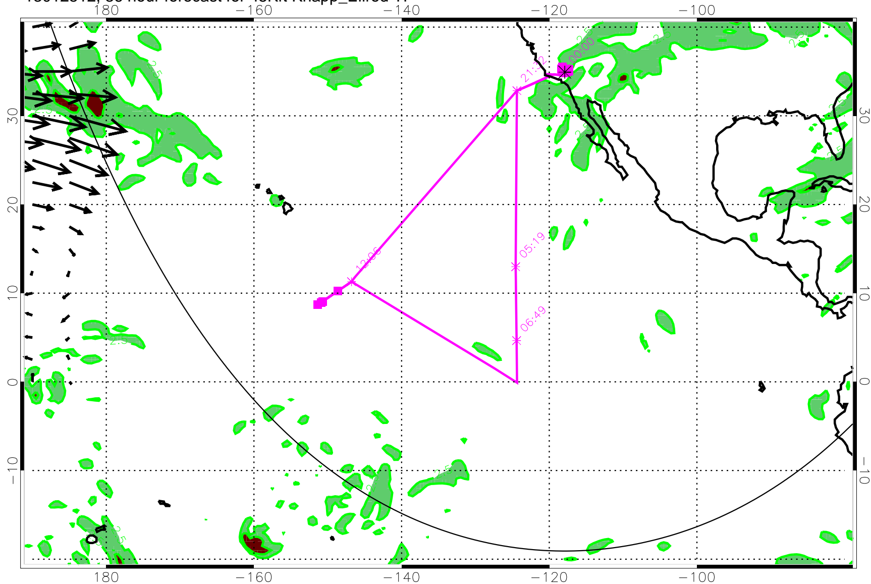
13012512, 36 hour forecast for 45Kft Knapp_Ellrod TI
