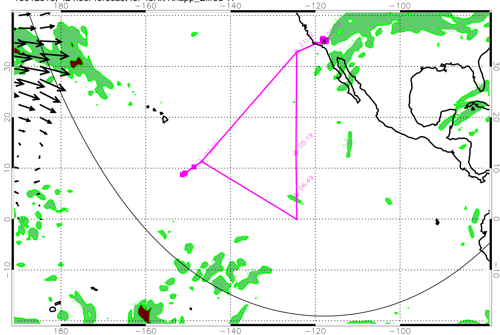
13012518, 42 hour forecast for 45Kft Knapp_Ellrod TI
