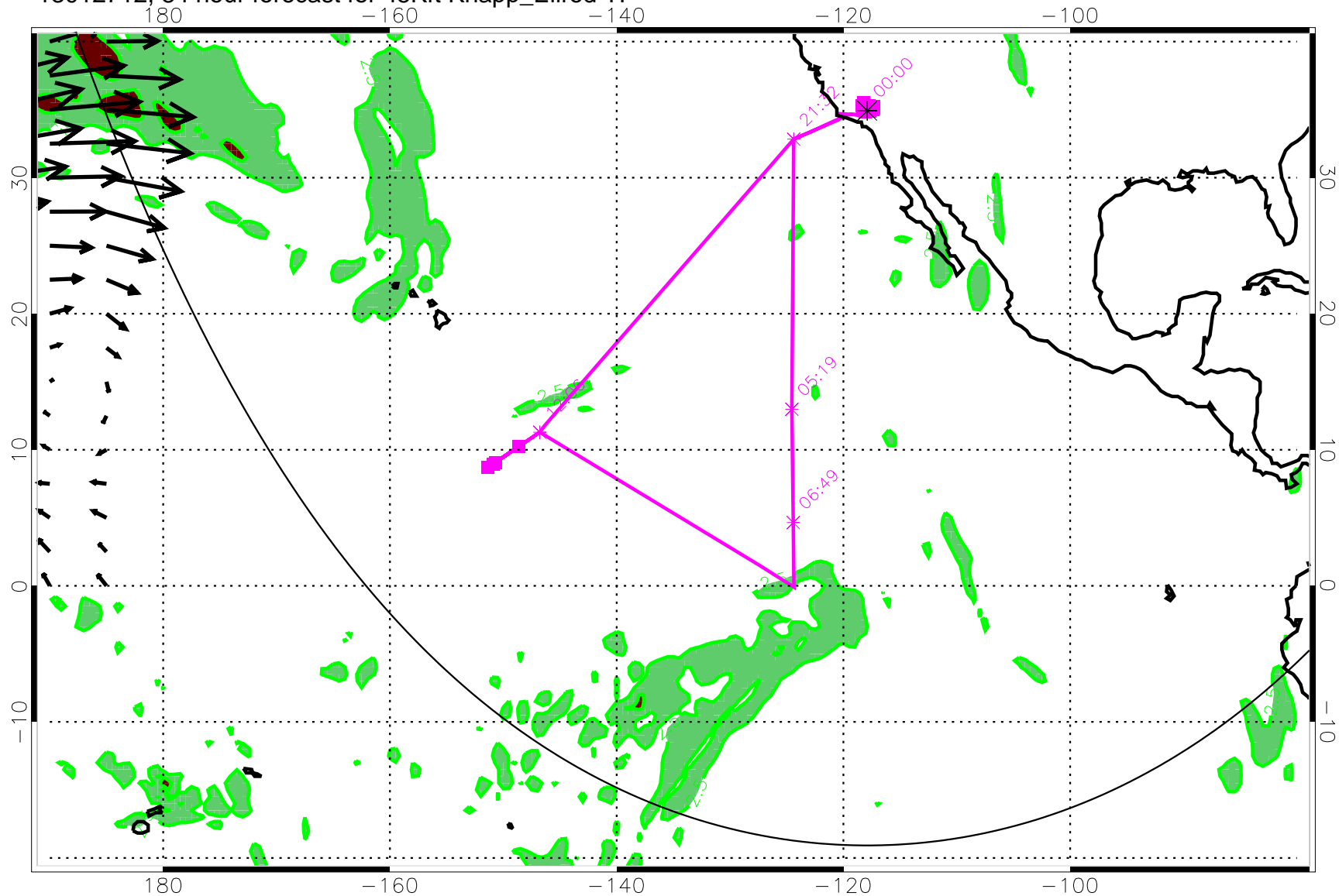
13012712, 84 hour forecast for 45Kft Knapp_Ellrod TI
