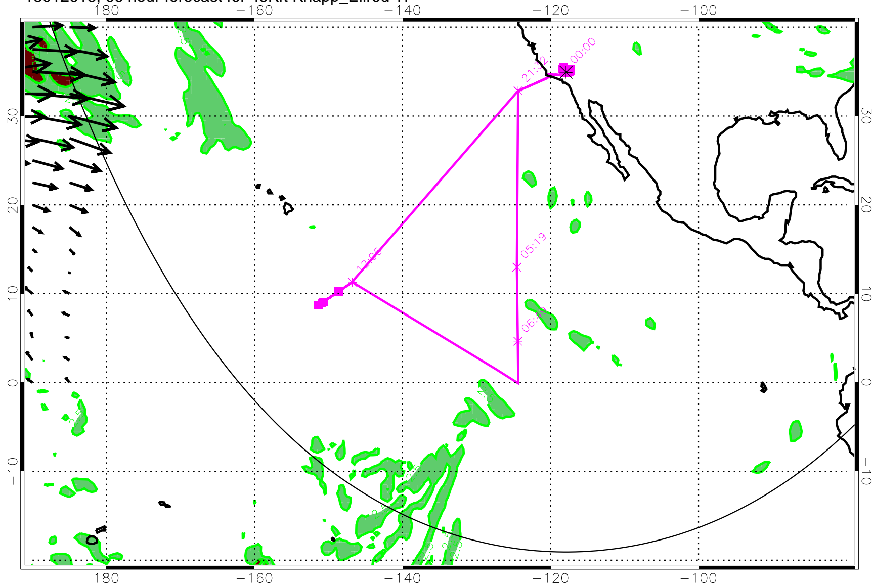
13012618, 66 hour forecast for 45Kft Knapp_Ellrod TI
