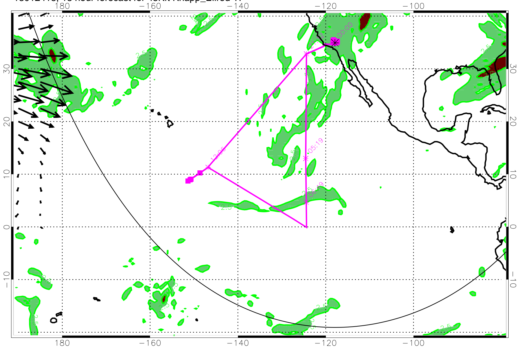
13012418, 18 hour forecast for 45Kft Knapp_Ellrod TI
