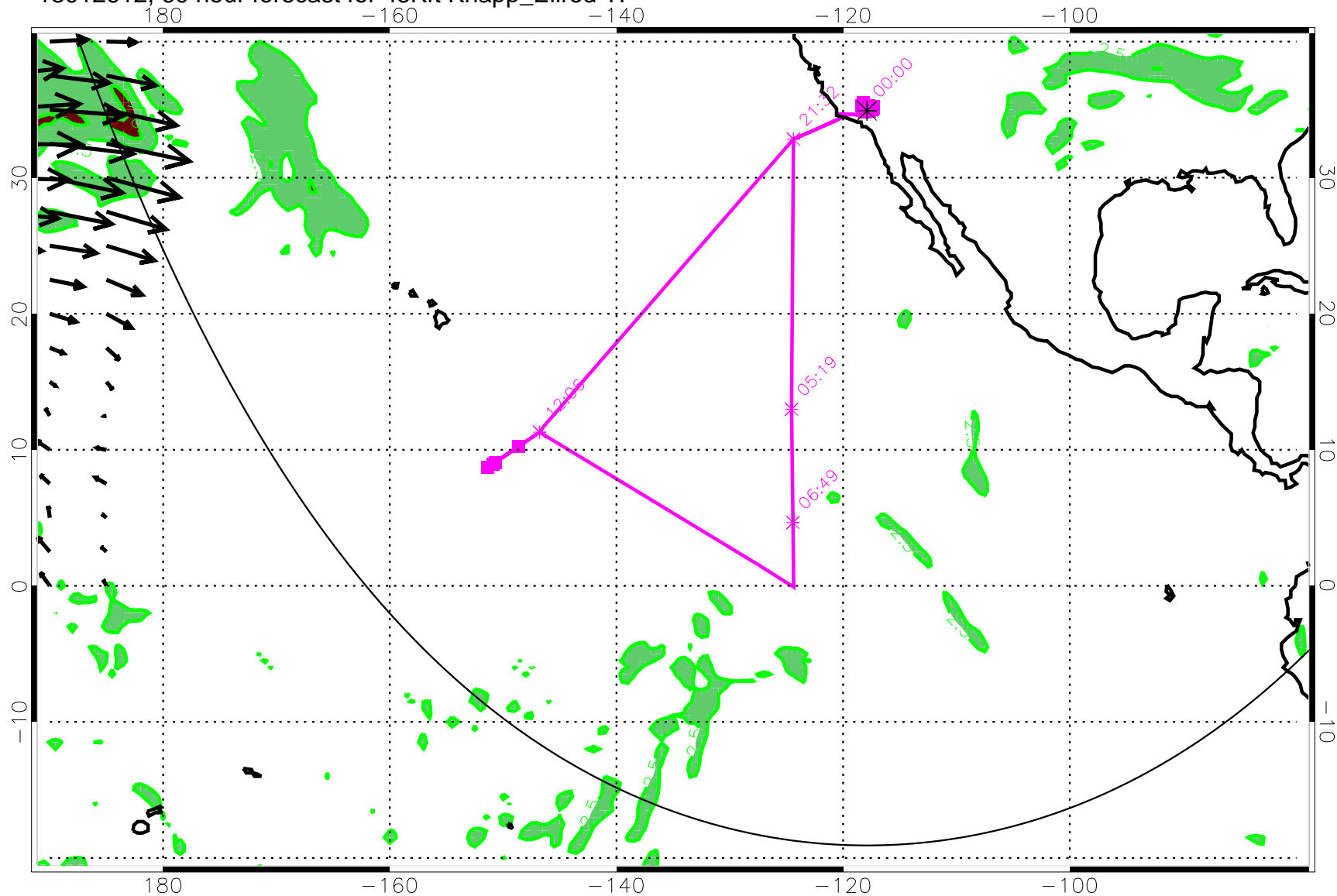
13012612, 60 hour forecast for 45Kft Knapp_Ellrod TI
