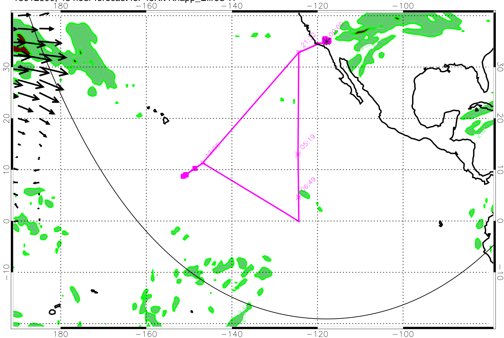
13012600, 48 hour forecast for 45Kft Knapp_Ellrod TI
