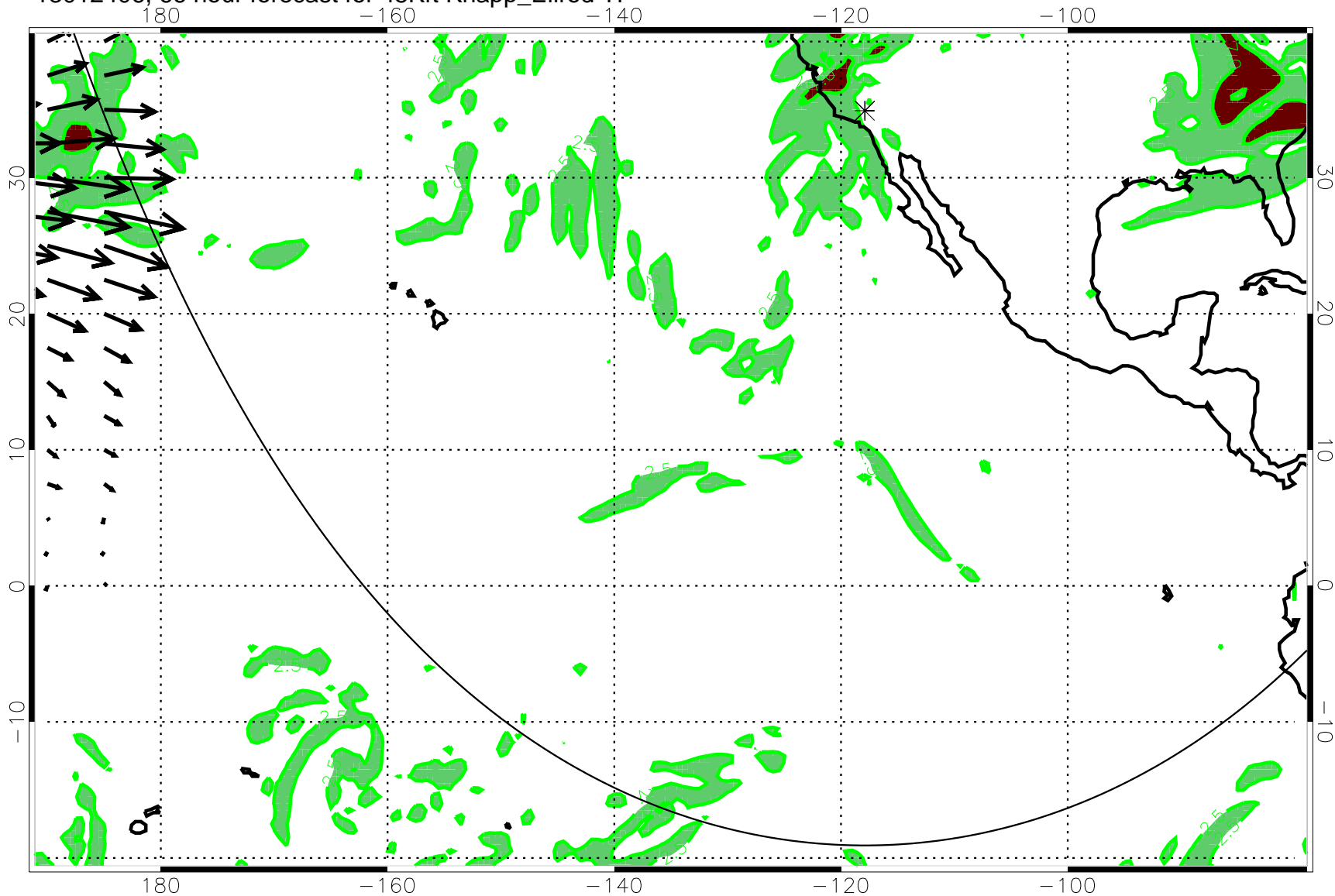
13012406, 66 hour forecast for 45Kft Knapp_Ellrod TI
