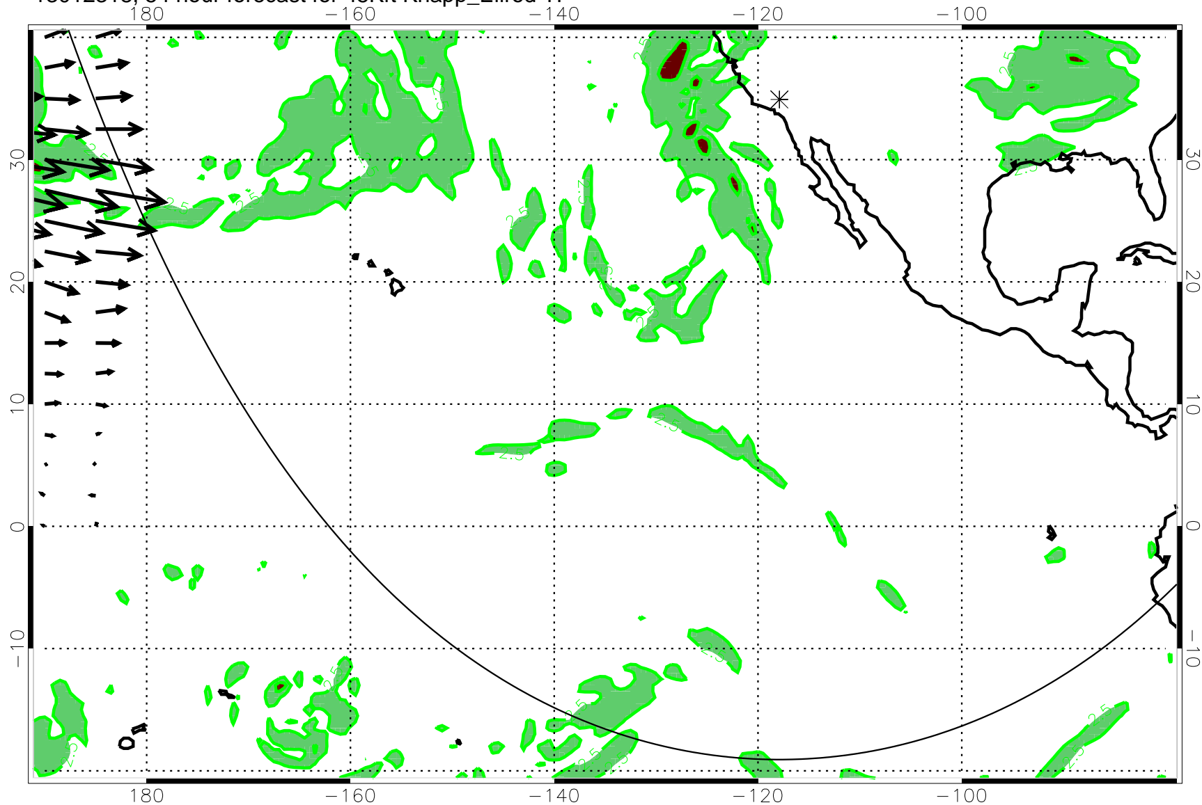
13012318, 54 hour forecast for 45Kft Knapp_Ellrod TI
