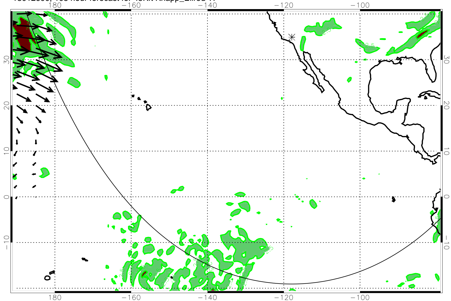
13012600, 108 hour forecast for 45Kft Knapp_Ellrod TI
