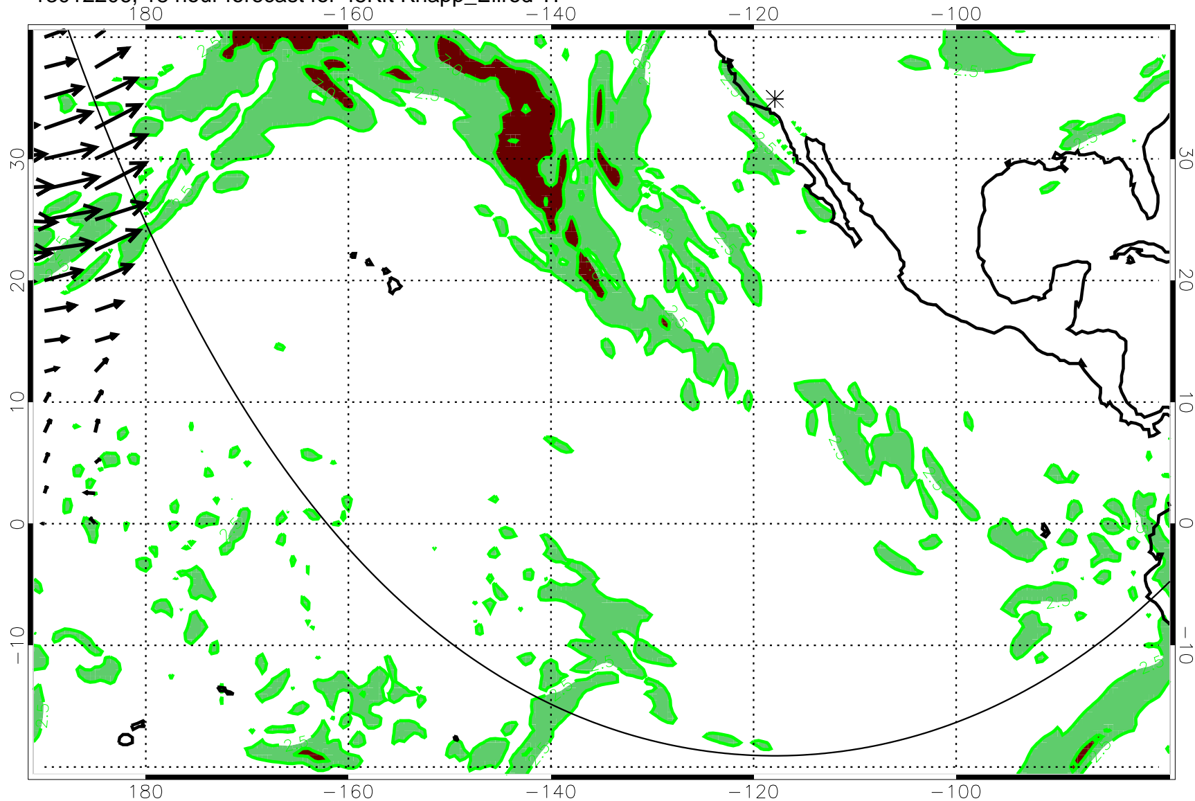
13012206, 18 hour forecast for 45Kft Knapp_Ellrod TI
