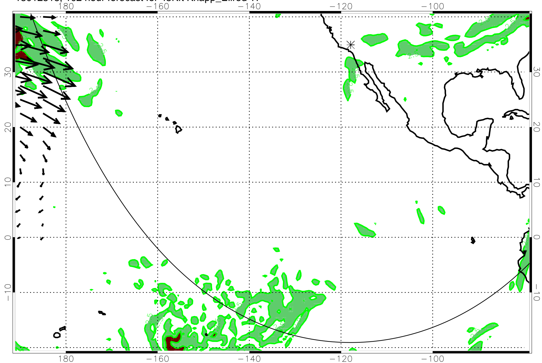
13012518, 102 hour forecast for 45Kft Knapp_Ellrod T1
