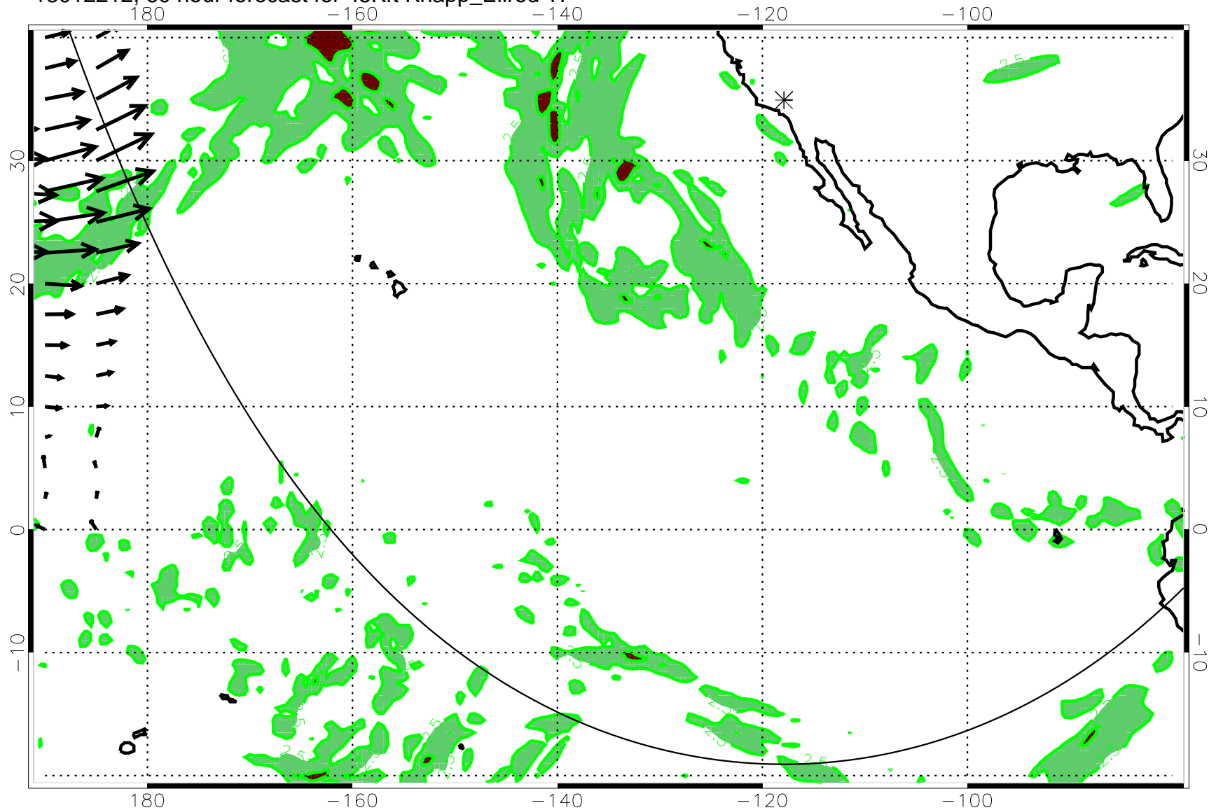
13012212, 60 hour forecast for 45Kft Knapp_Ellrod TI
