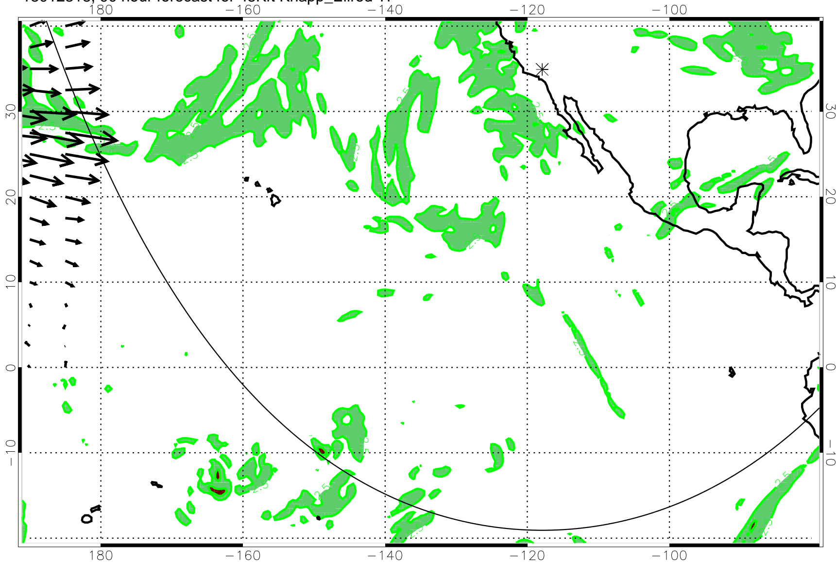
13012318, 90 hour forecast for 45Kft Knapp_Ellrod TI
