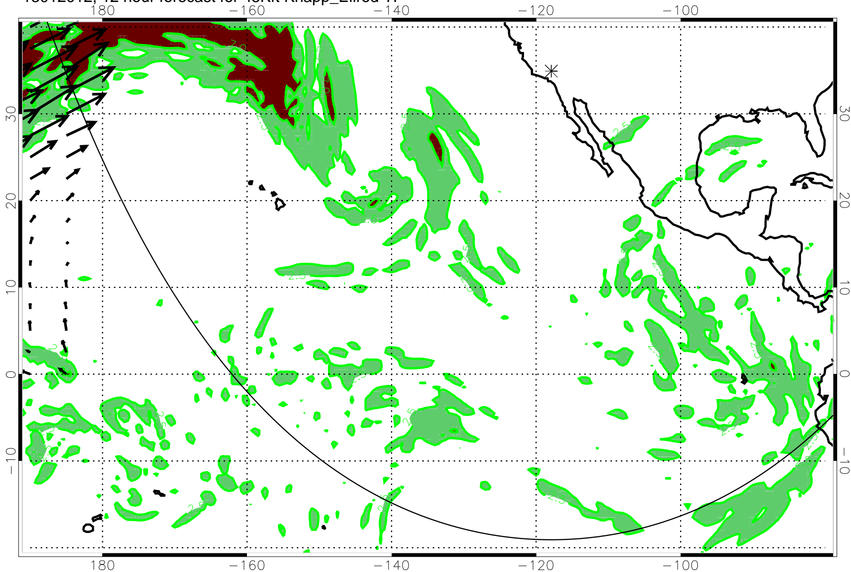
13012012, 12 hour forecast for 45Kft Knapp_Ellrod TI
