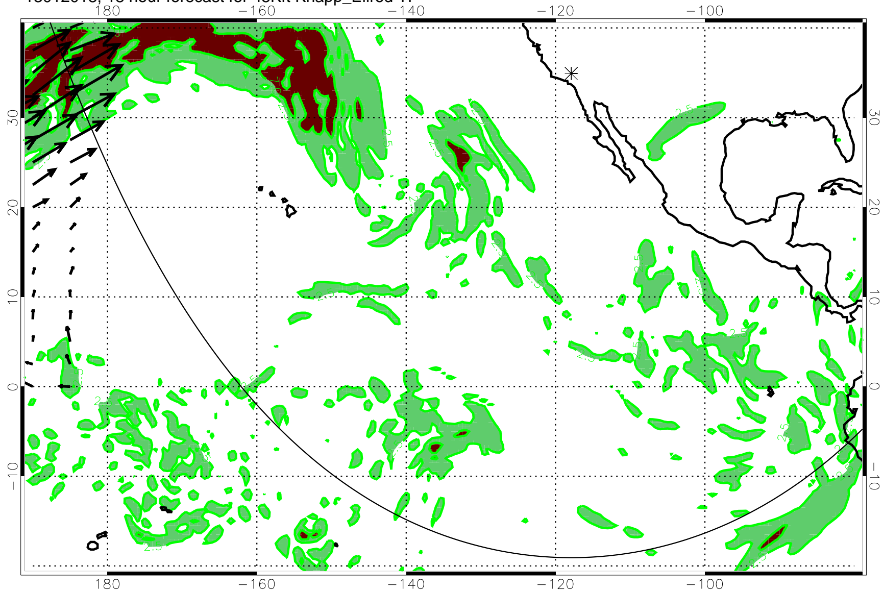
13012018, 18 hour forecast for 45Kft Knapp_Ellrod TI
