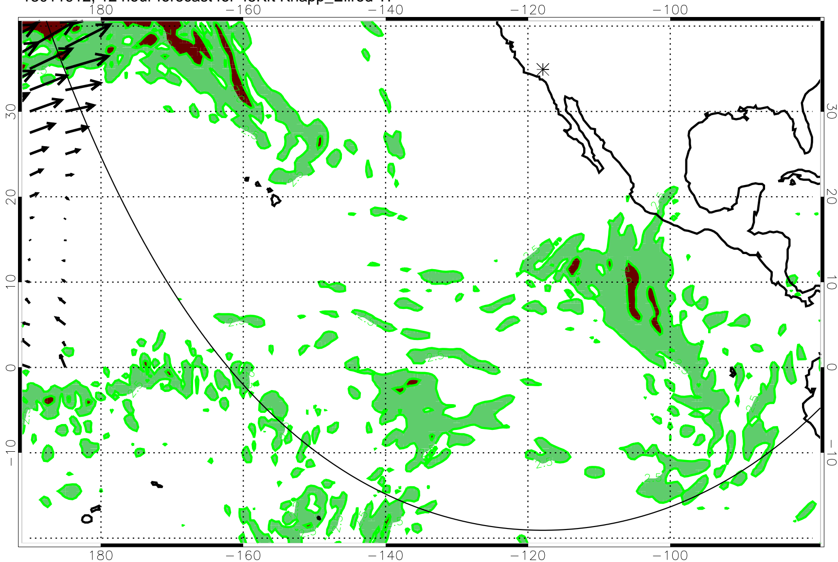
13011912, 12 hour forecast for 45Kft Knapp_Ellrod TI
