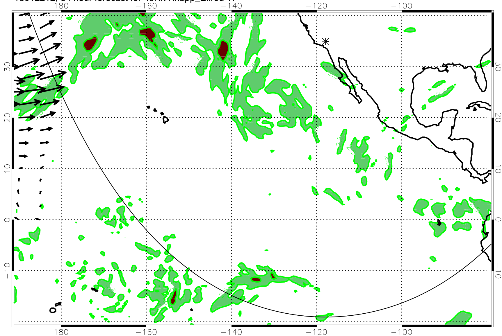
13012212, 84 hour forecast for 45Kft Knapp_Ellrod TI
