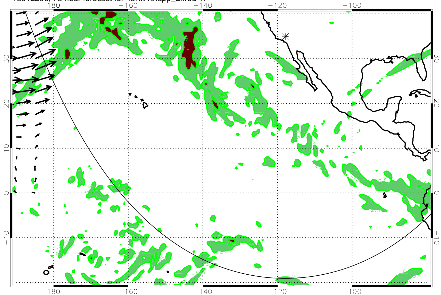
13012206, 78 hour forecast for 45Kft Knapp_Ellrod TI
