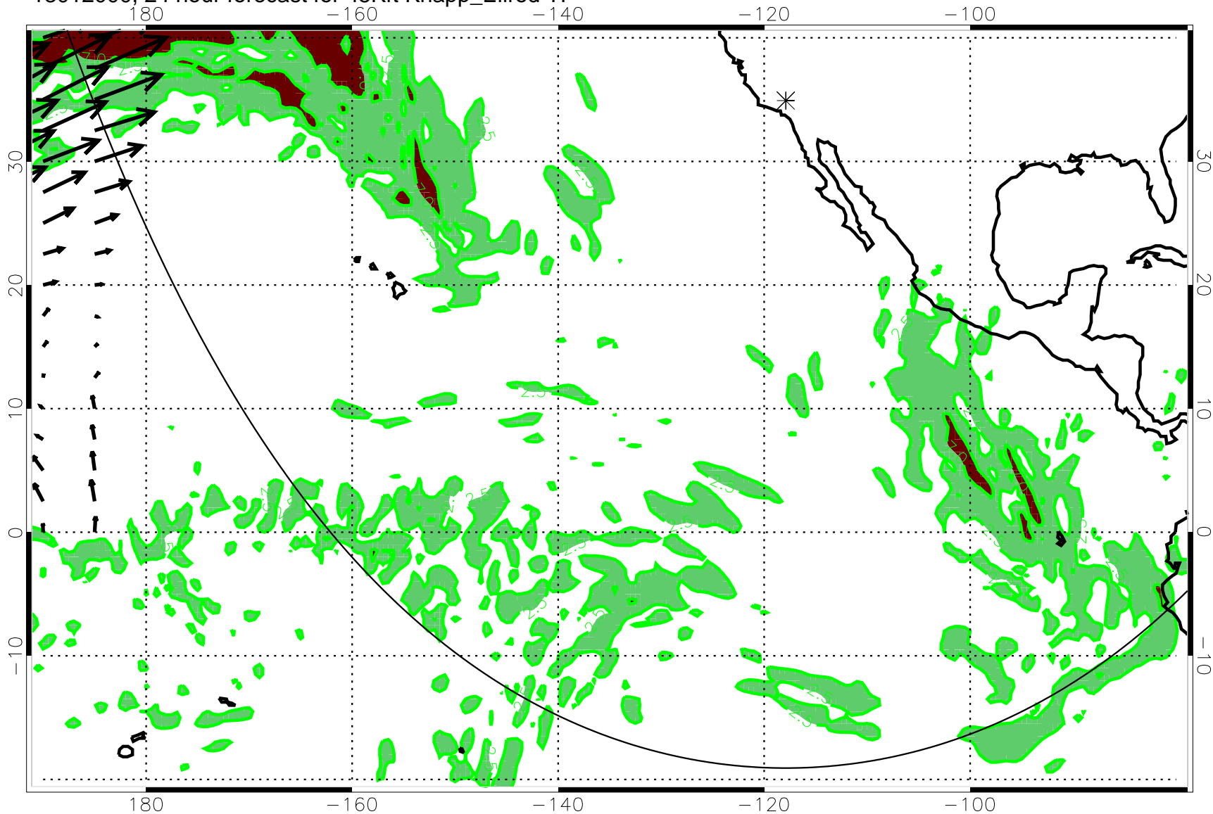
13012000, 24 hour forecast for 45Kft Knapp_Ellrod TI
