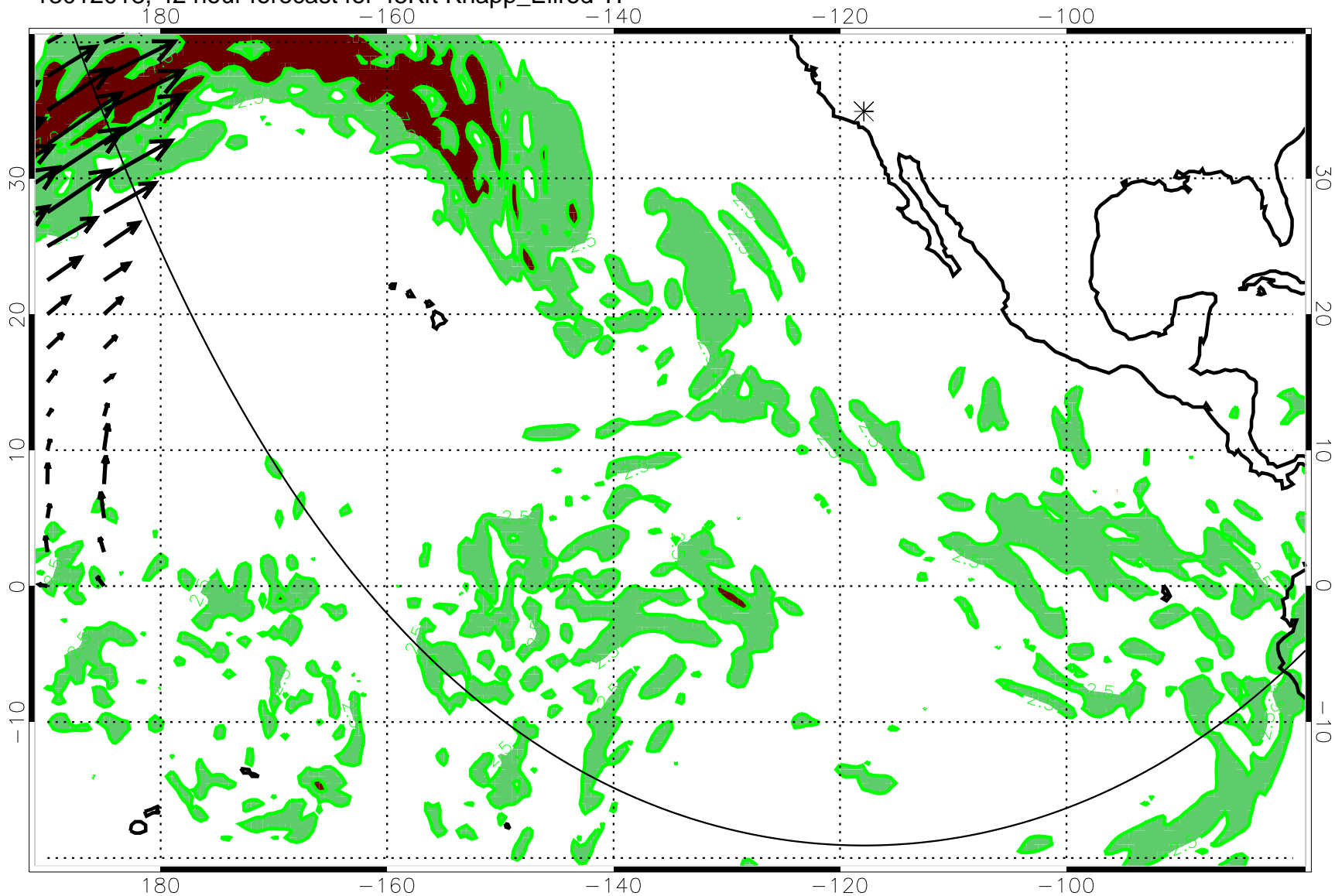
13012018, 42 hour forecast for 45Kft Knapp_Ellrod TI
