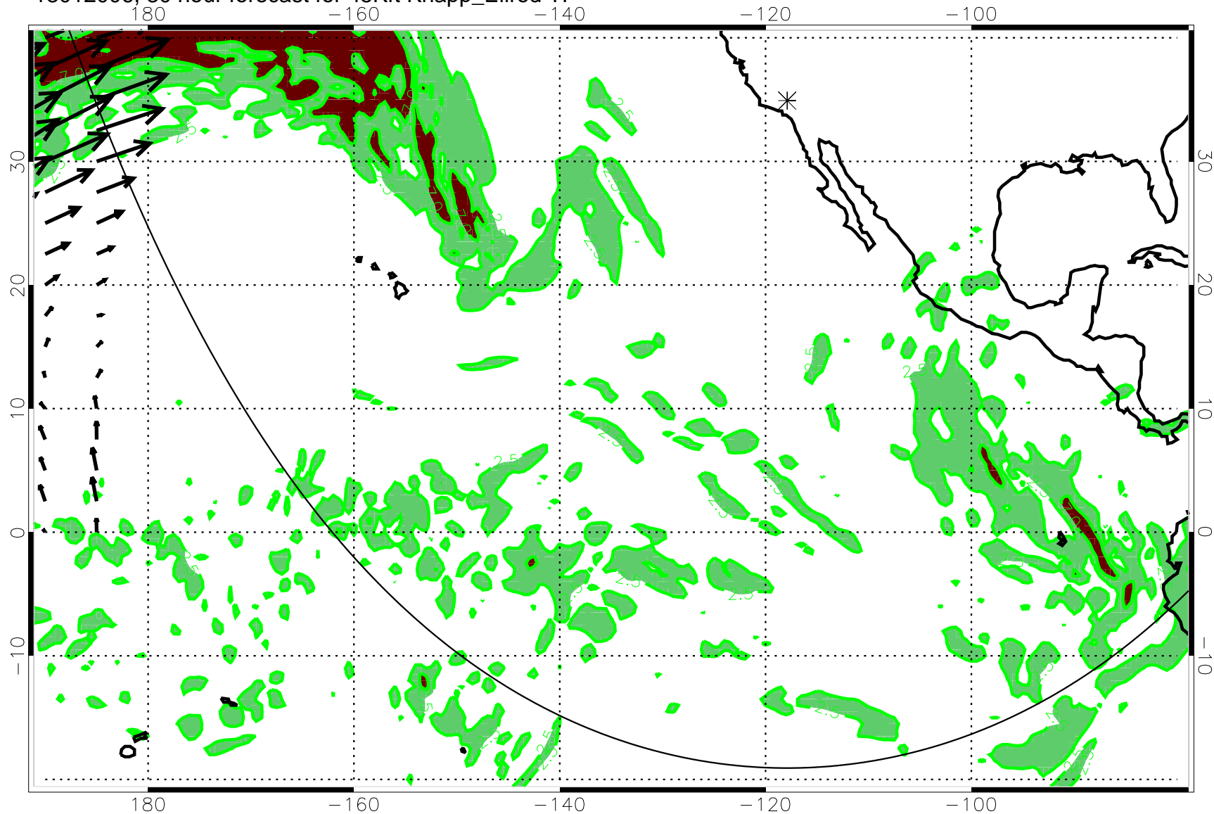
13012006, 30 hour forecast for 45Kft Knapp_Ellrod TI
