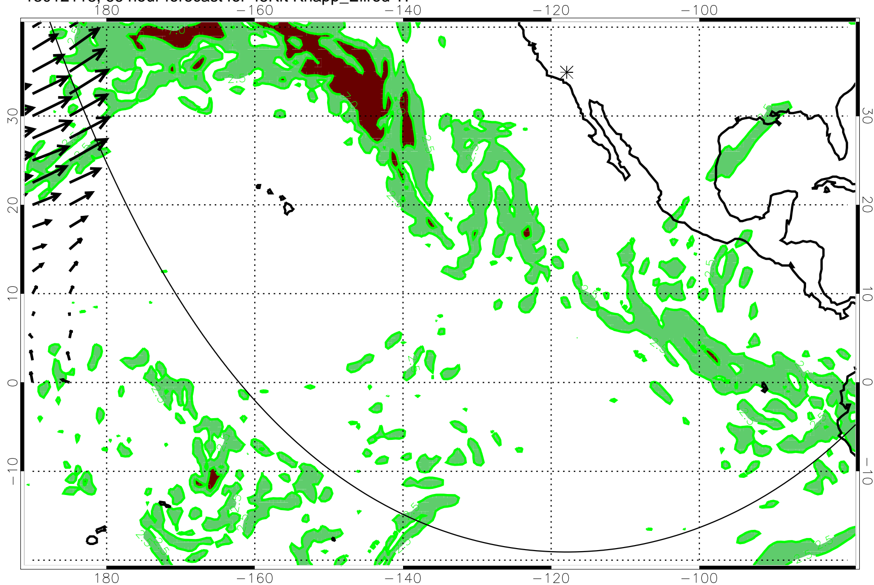
13012118, 66 hour forecast for 45Kft Knapp_Ellrod TI
