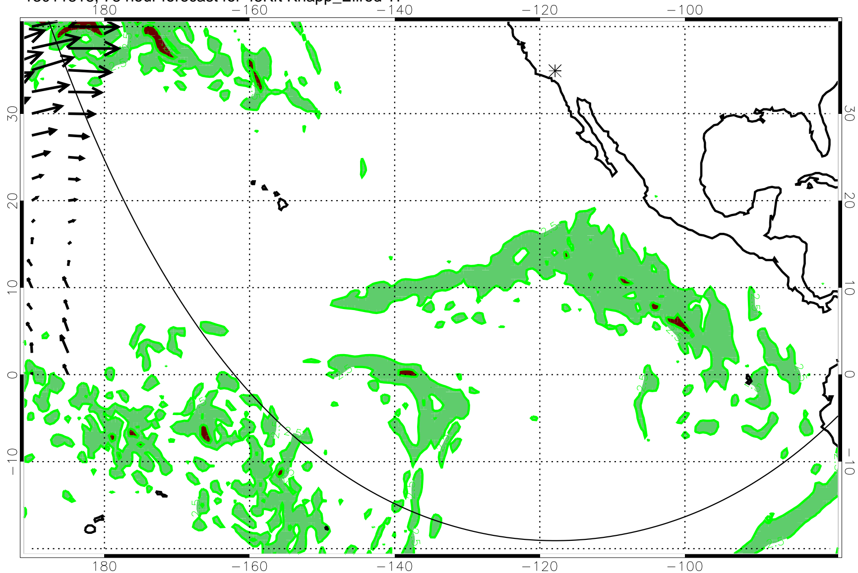
13011818, 78 hour forecast for 45Kft Knapp_Ellrod TI
