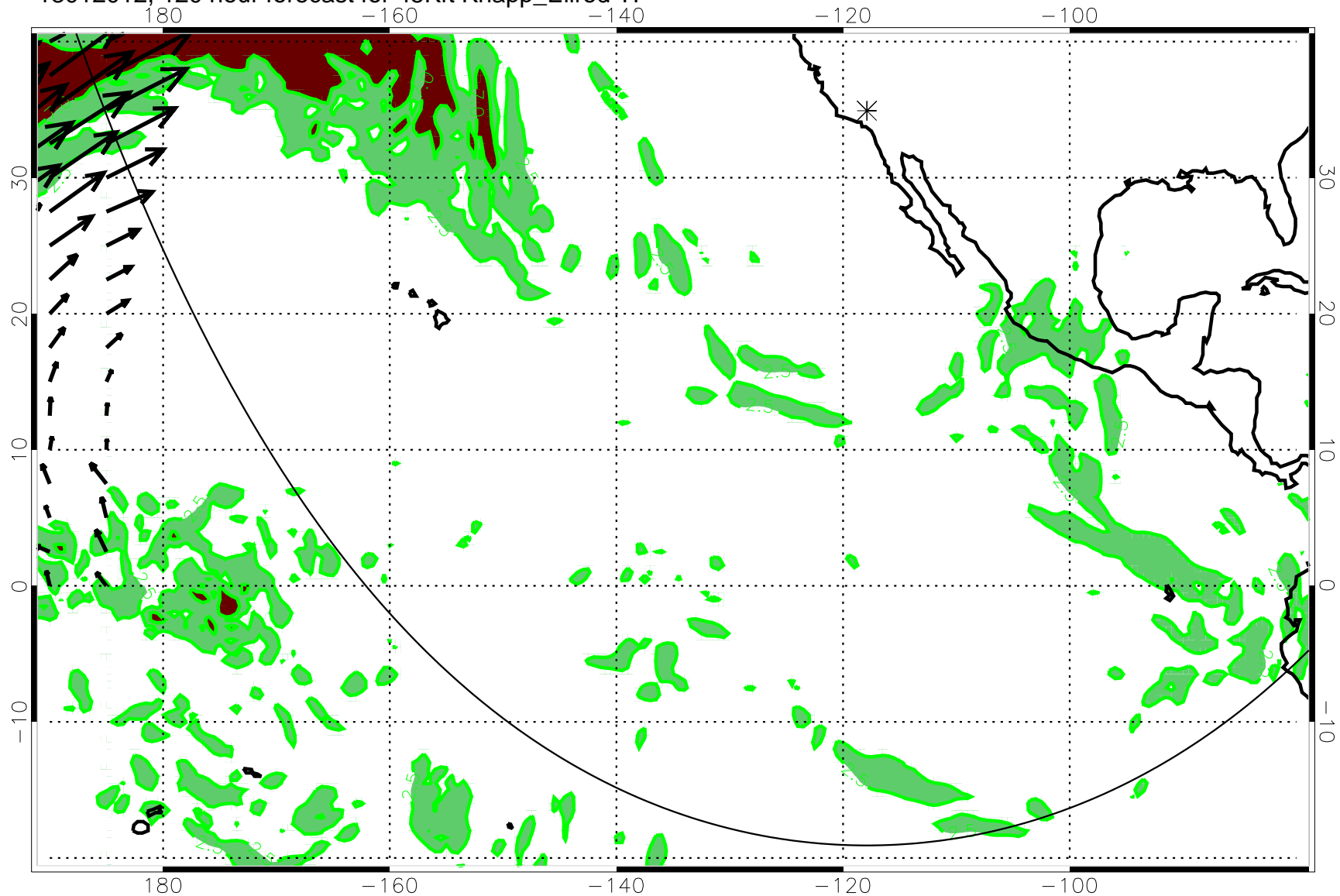
13012012, 120 hour forecast for 45Kft Knapp_Ellrod TI
