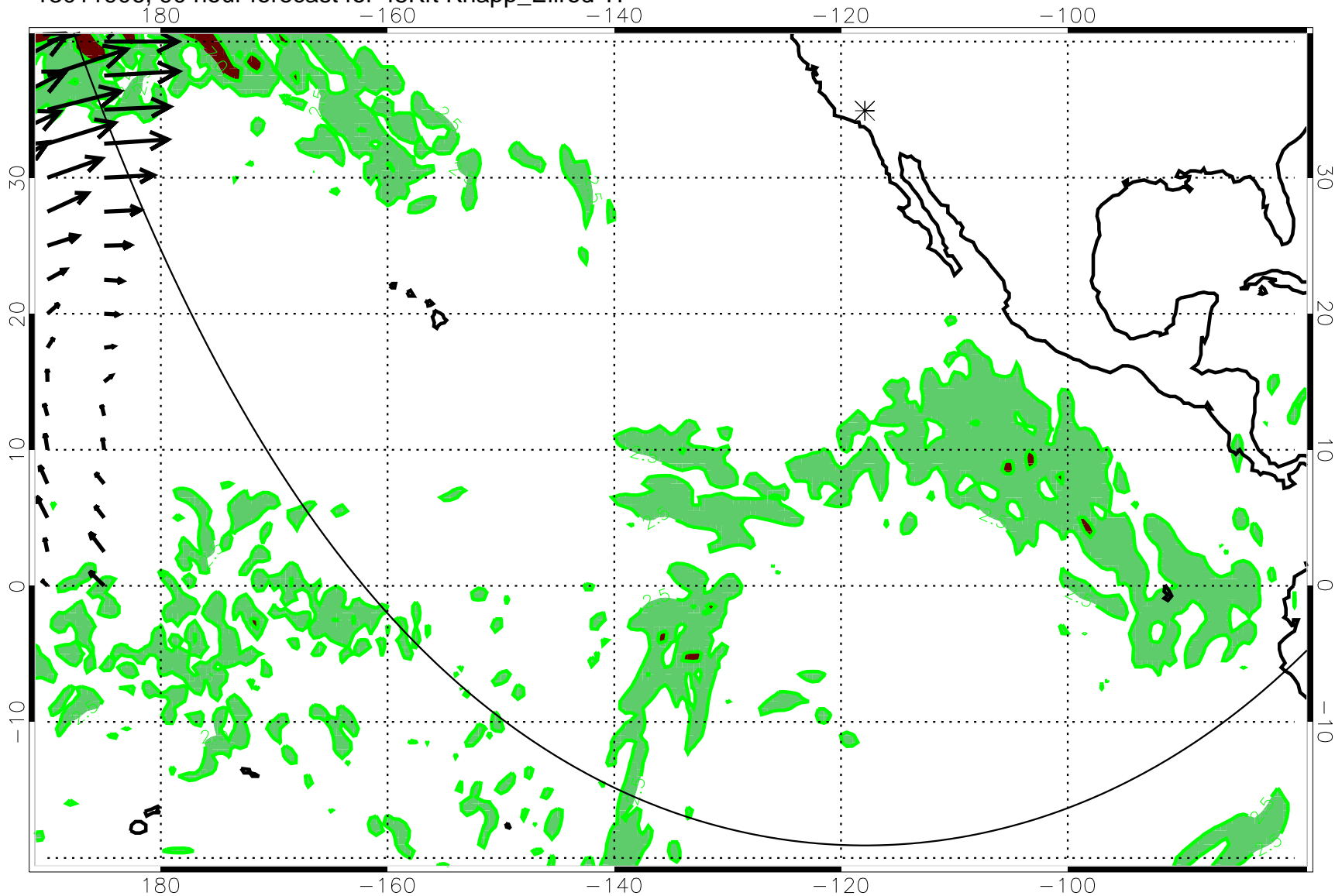
13011906, 90 hour forecast for 45Kft Knapp_Ellrod TI
