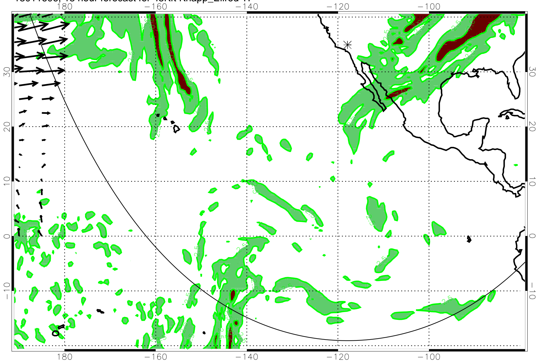
13011606, 18 hour forecast for 45Kft Knapp_Ellrod TI
