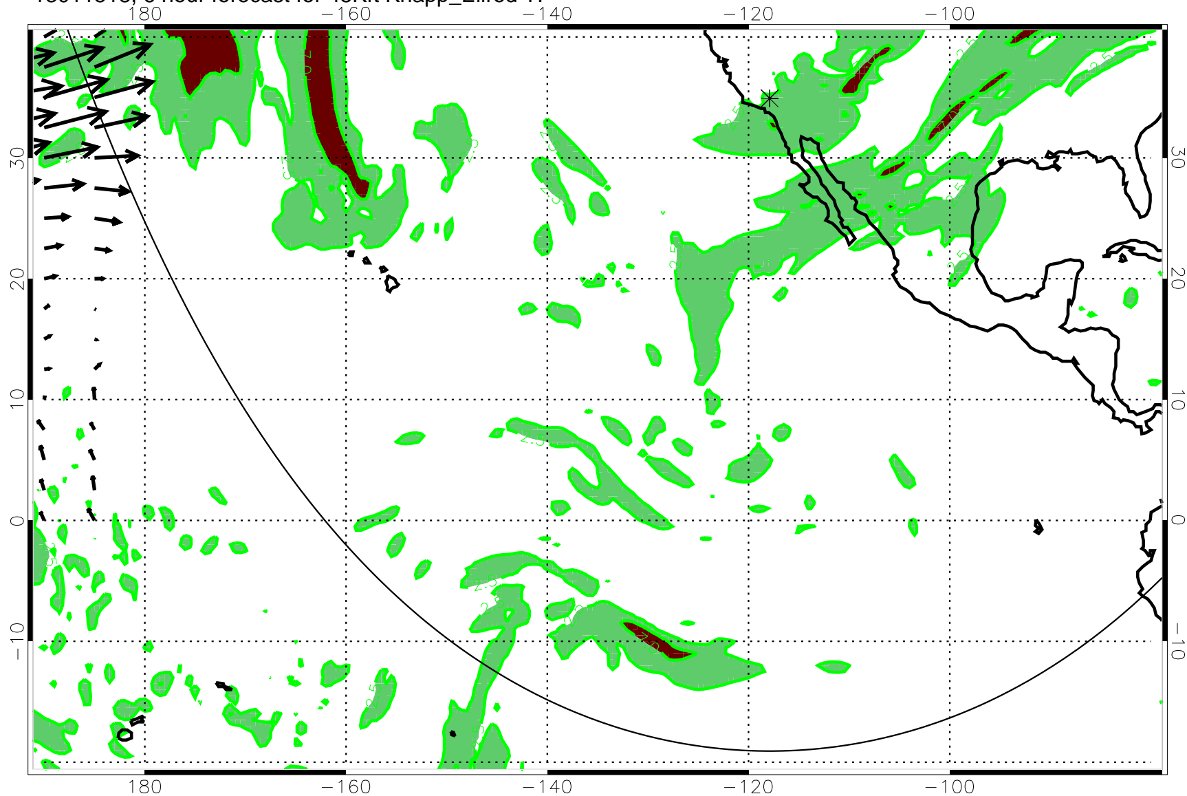
13011518, 6 hour forecast for 45Kft Knapp_Ellrod TI
