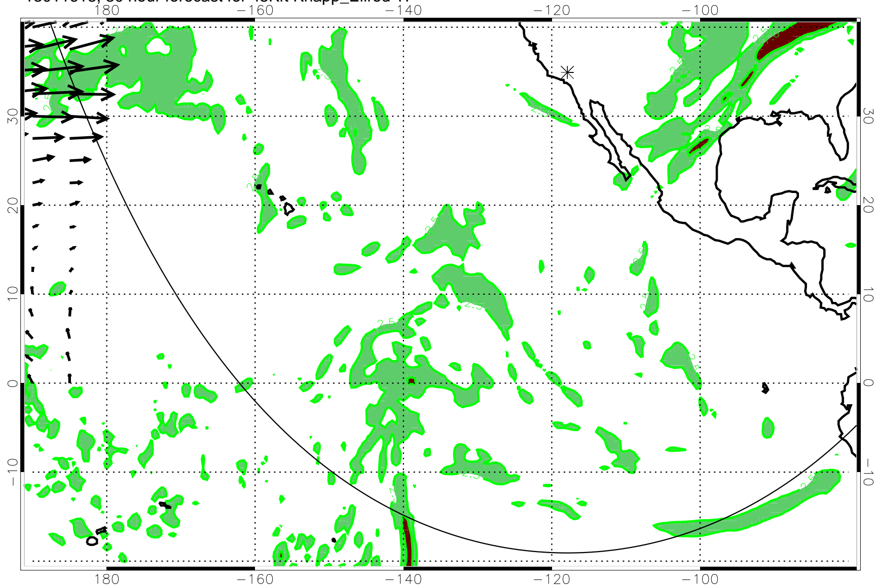
13011618, 30 hour forecast for 45Kft Knapp_Ellrod TI
