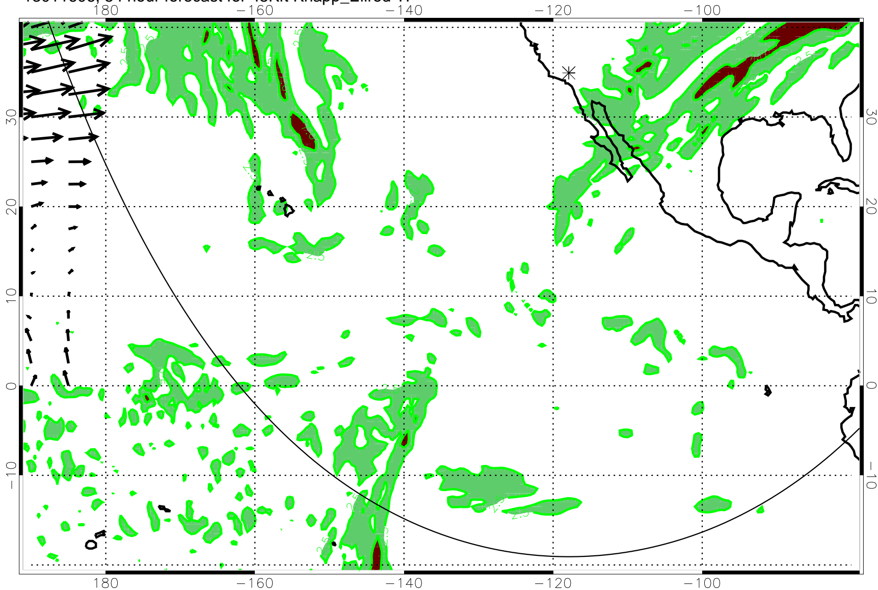
13011606, 54 hour forecast for 45Kft Knapp_Ellrod TI
