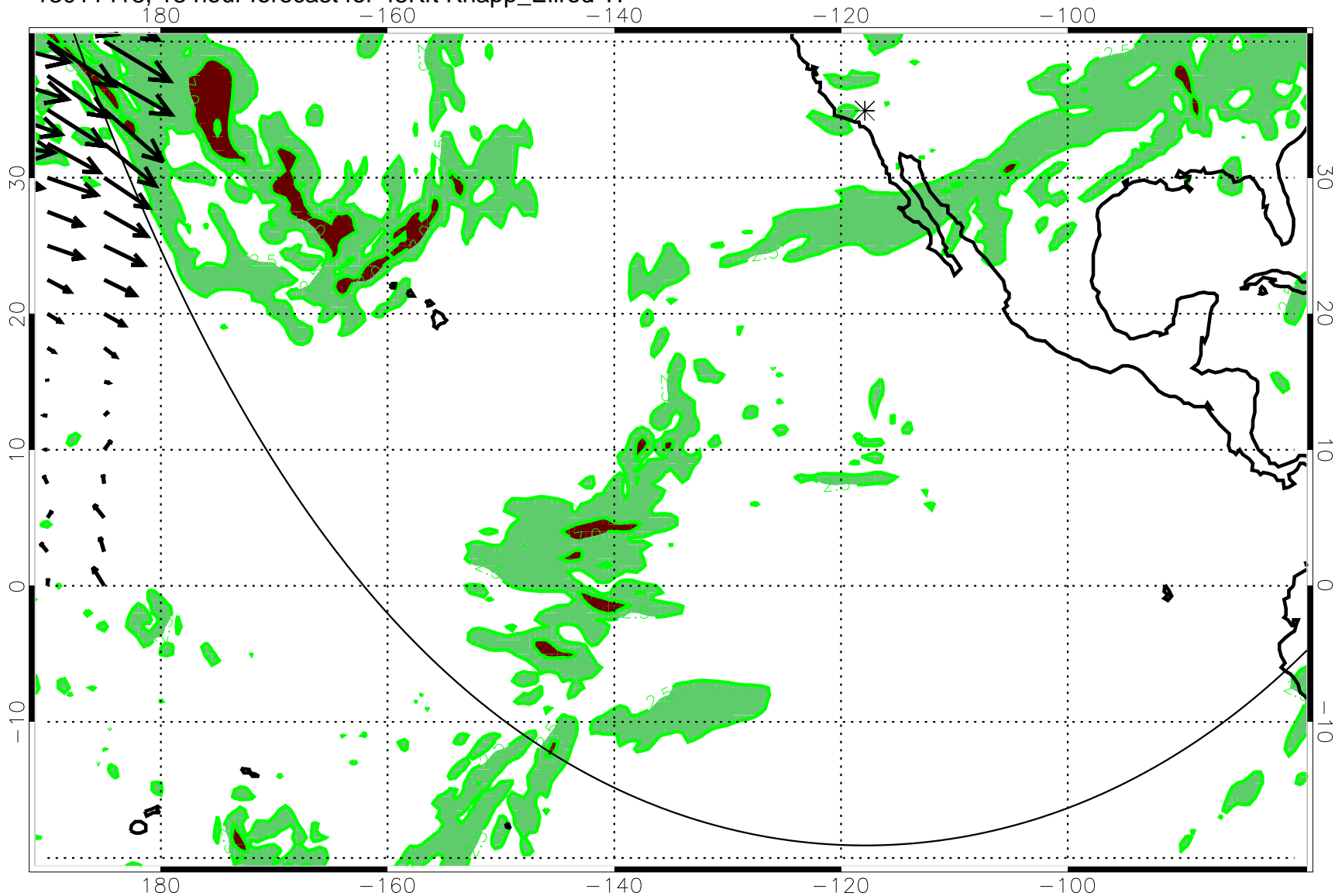
13011418, 18 hour forecast for 45Kft Knapp_Ellrod TI
