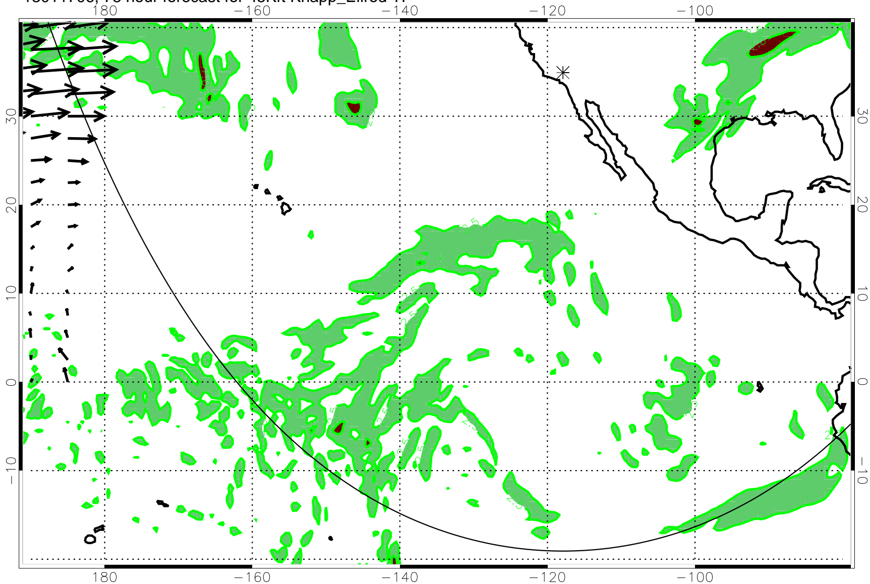
13011706, 78 hour forecast for 45Kft Knapp_Ellrod TI
