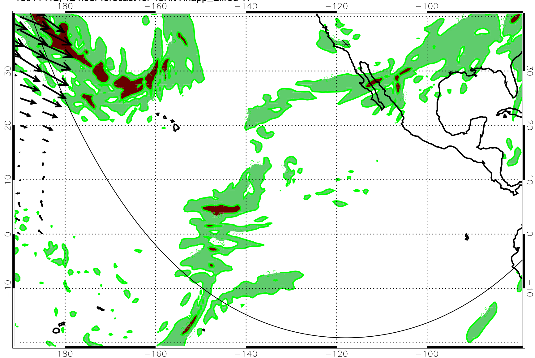
13011412, 12 hour forecast for 45Kft Knapp_Ellrod TI
