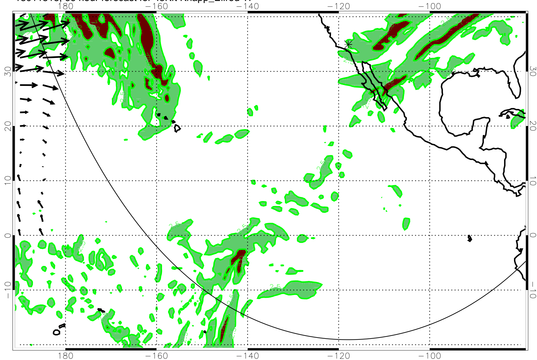
13011518, 66 hour forecast for 45Kft Knapp_Ellrod TI
