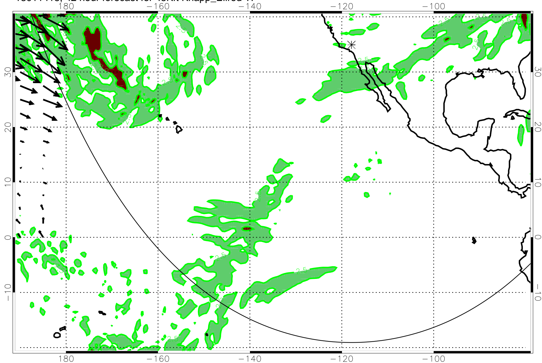
13011418, 42 hour forecast for 45Kft Knapp_Ellrod TI
