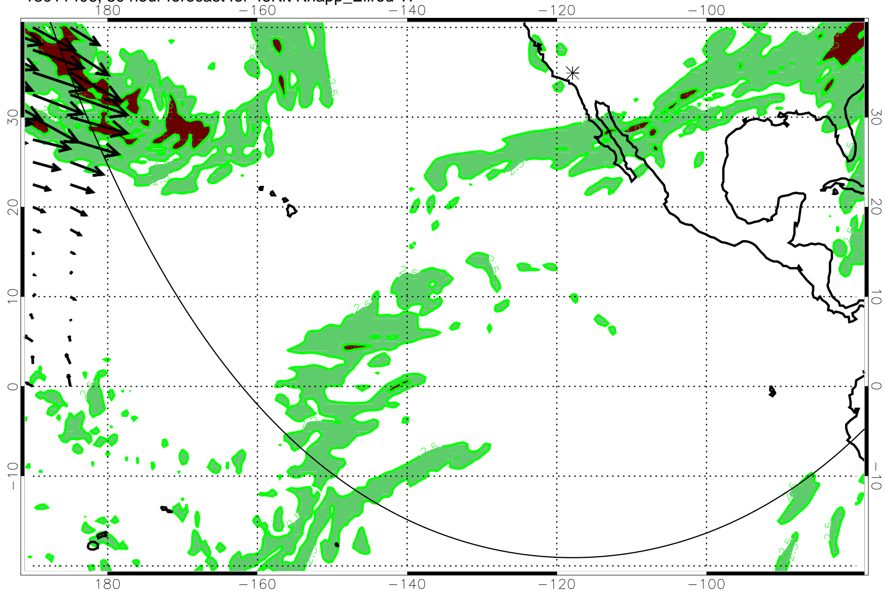
13011406, 30 hour forecast for 45Kft Knapp_Ellrod TI
