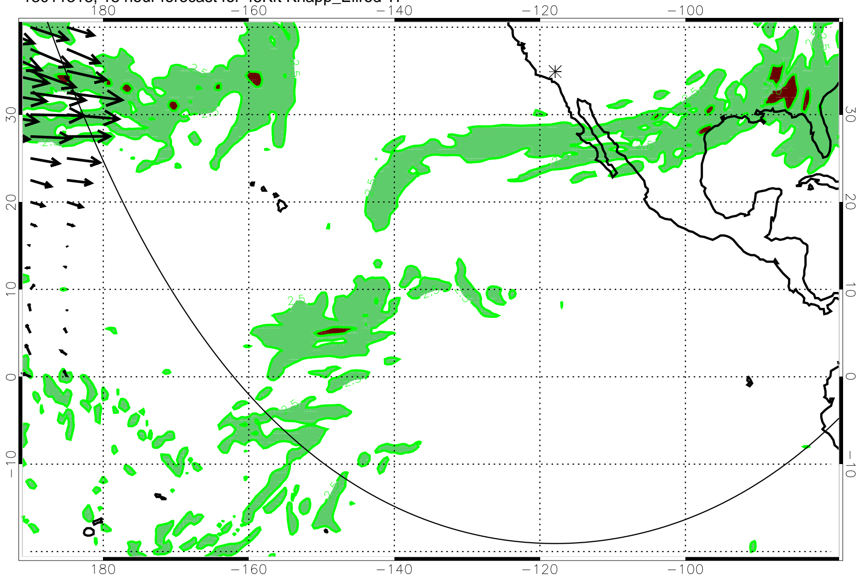
13011318, 18 hour forecast for 45Kft Knapp_Ellrod TI
