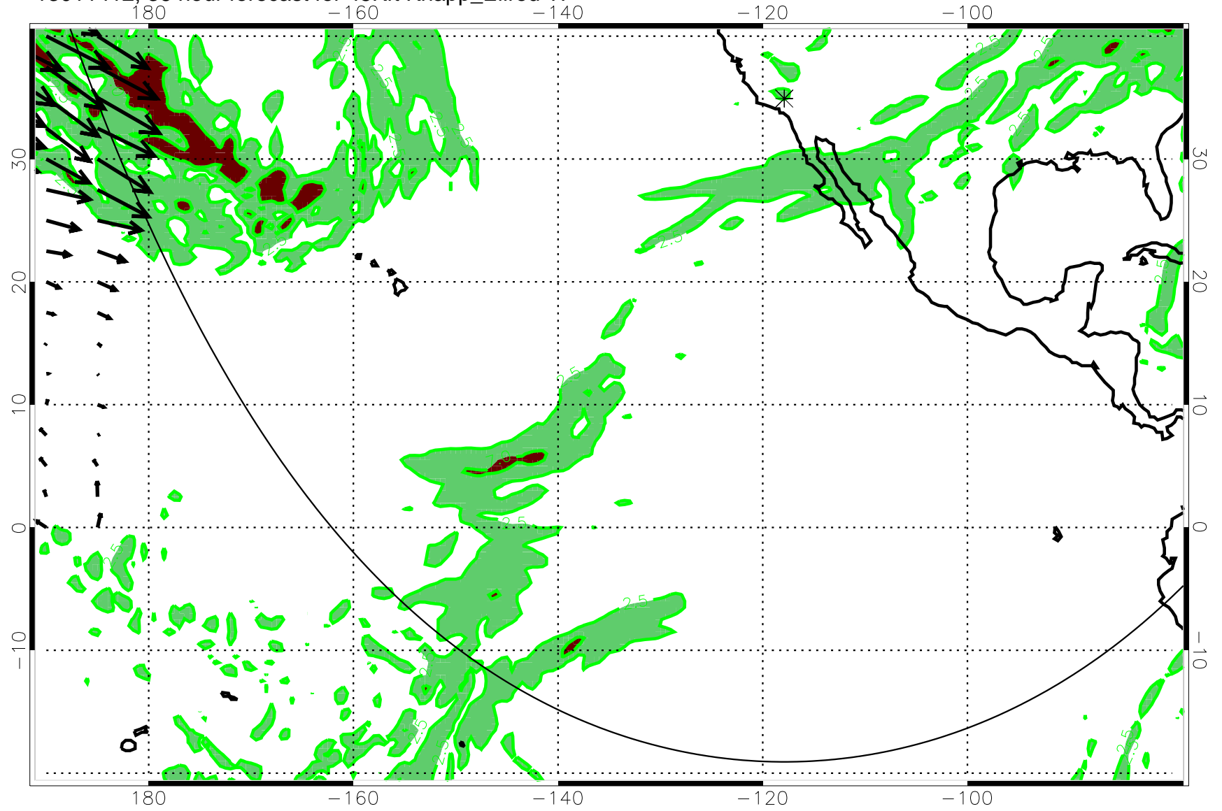
13011412, 36 hour forecast for 45Kft Knapp_Ellrod TI
