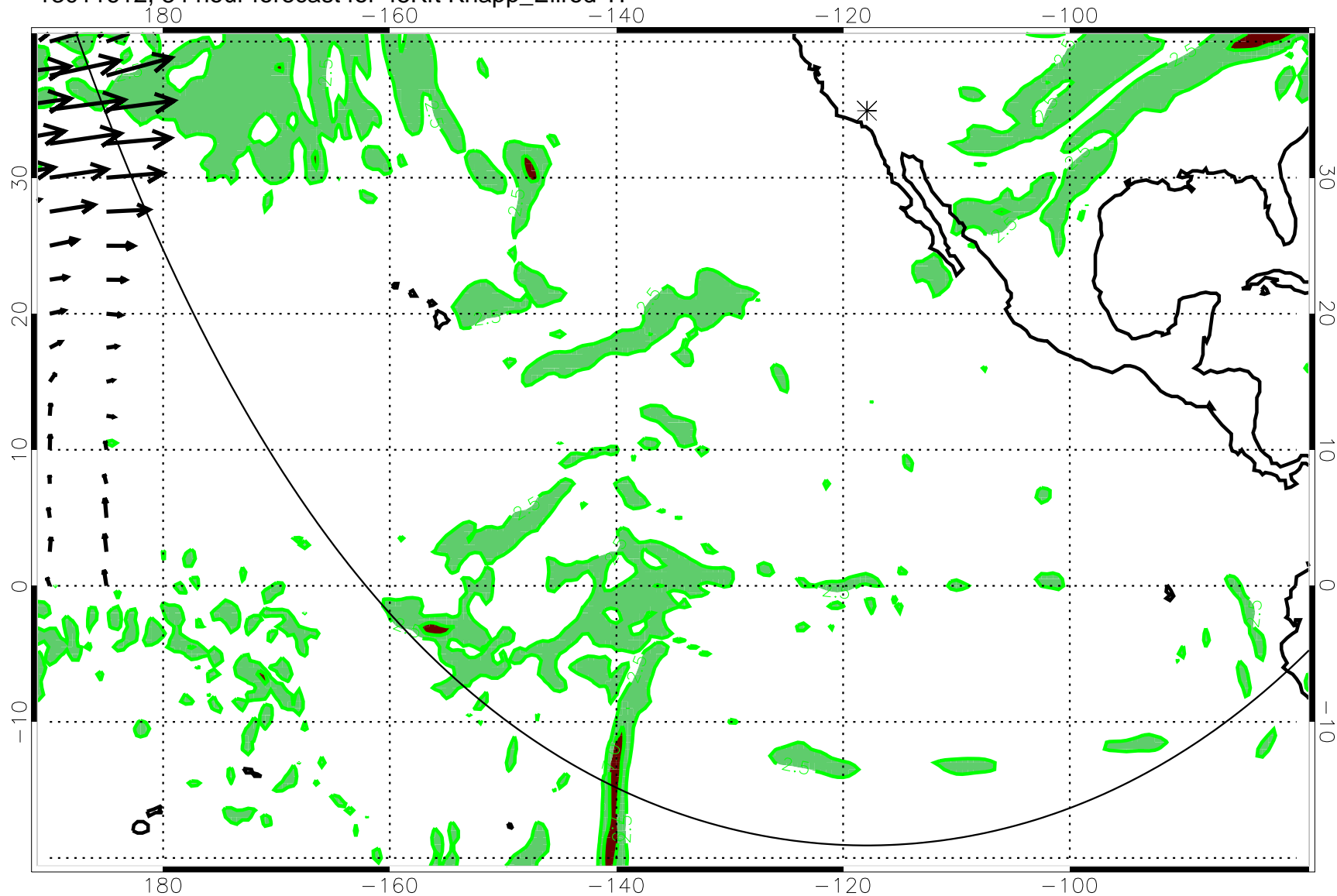
13011612, 84 hour forecast for 45Kft Knapp_Ellrod TI
