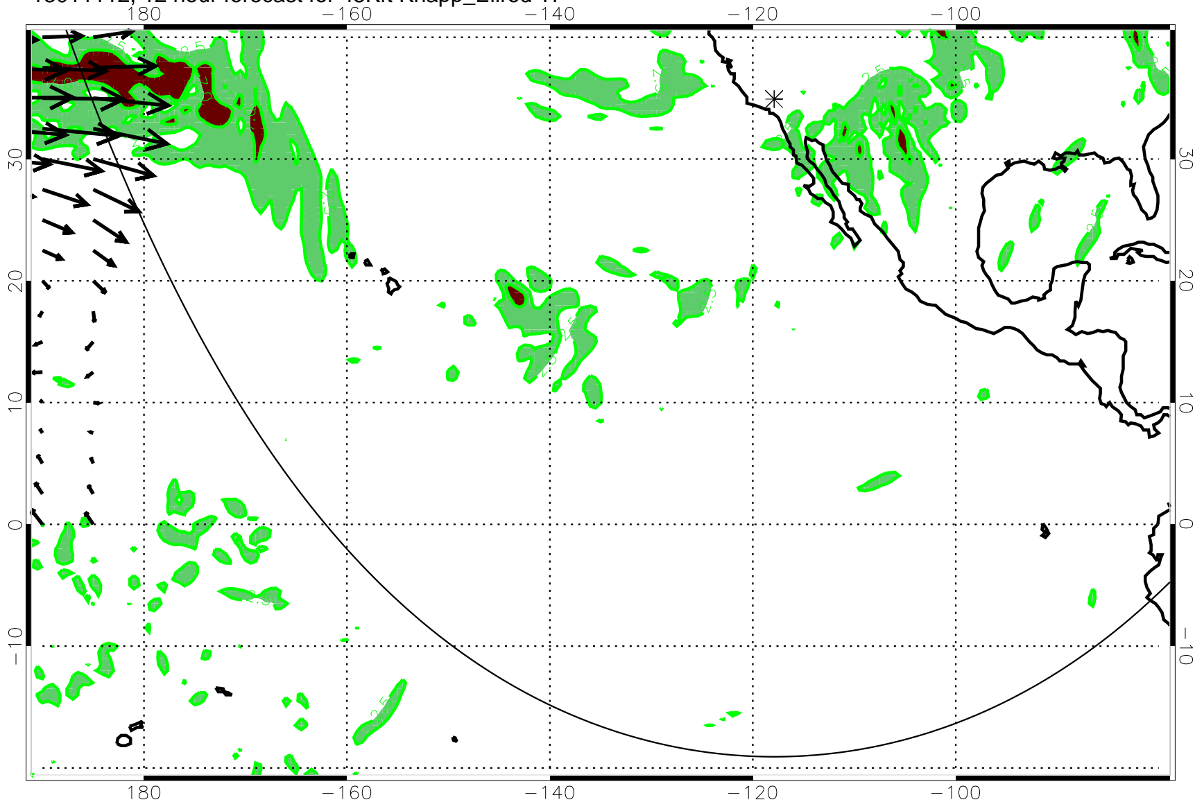
13011112, 12 hour forecast for 45Kft Knapp_Ellrod TI
