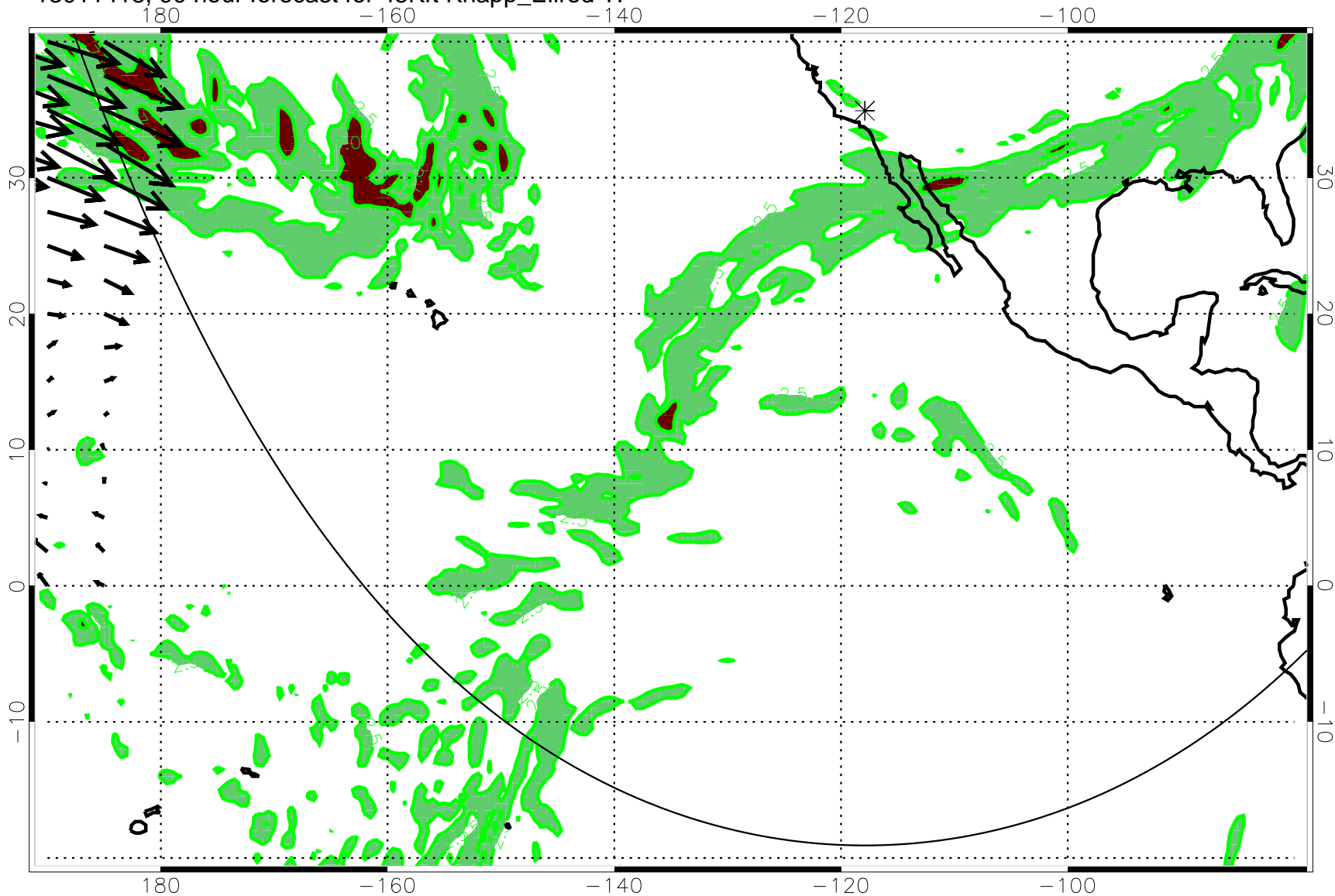
13011418, 90 hour forecast for 45Kft Knapp_Ellrod TI
