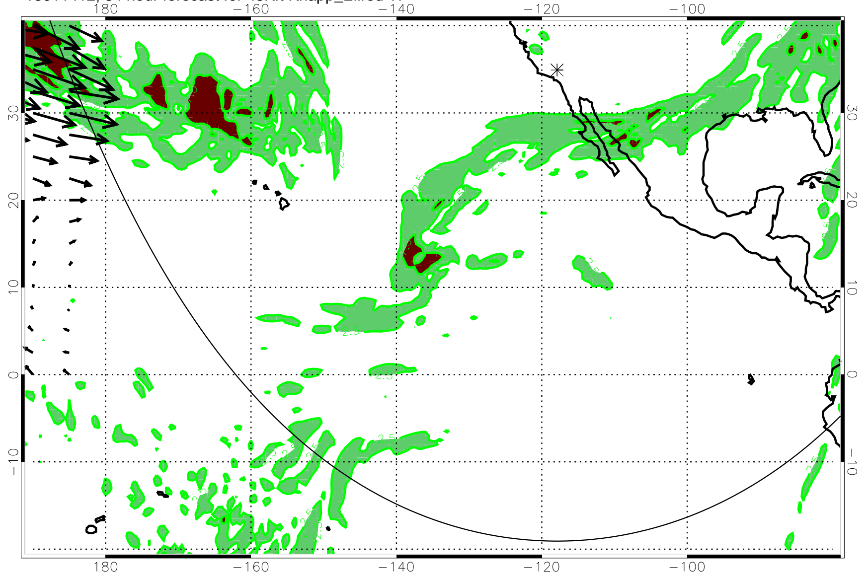
13011412, 84 hour forecast for 45Kft Knapp_Ellrod TI
