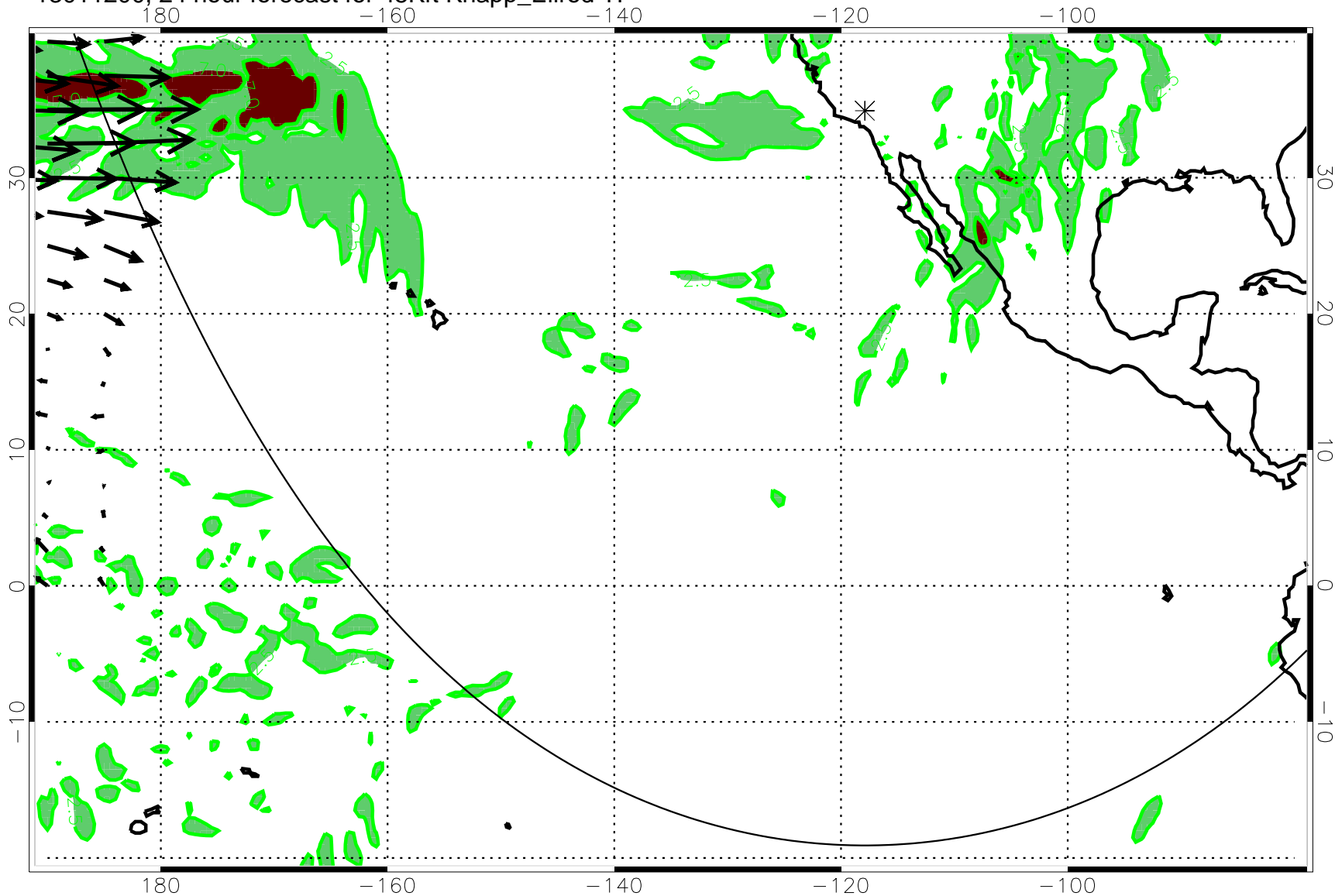
13011200, 24 hour forecast for 45Kft Knapp_Ellrod TI
