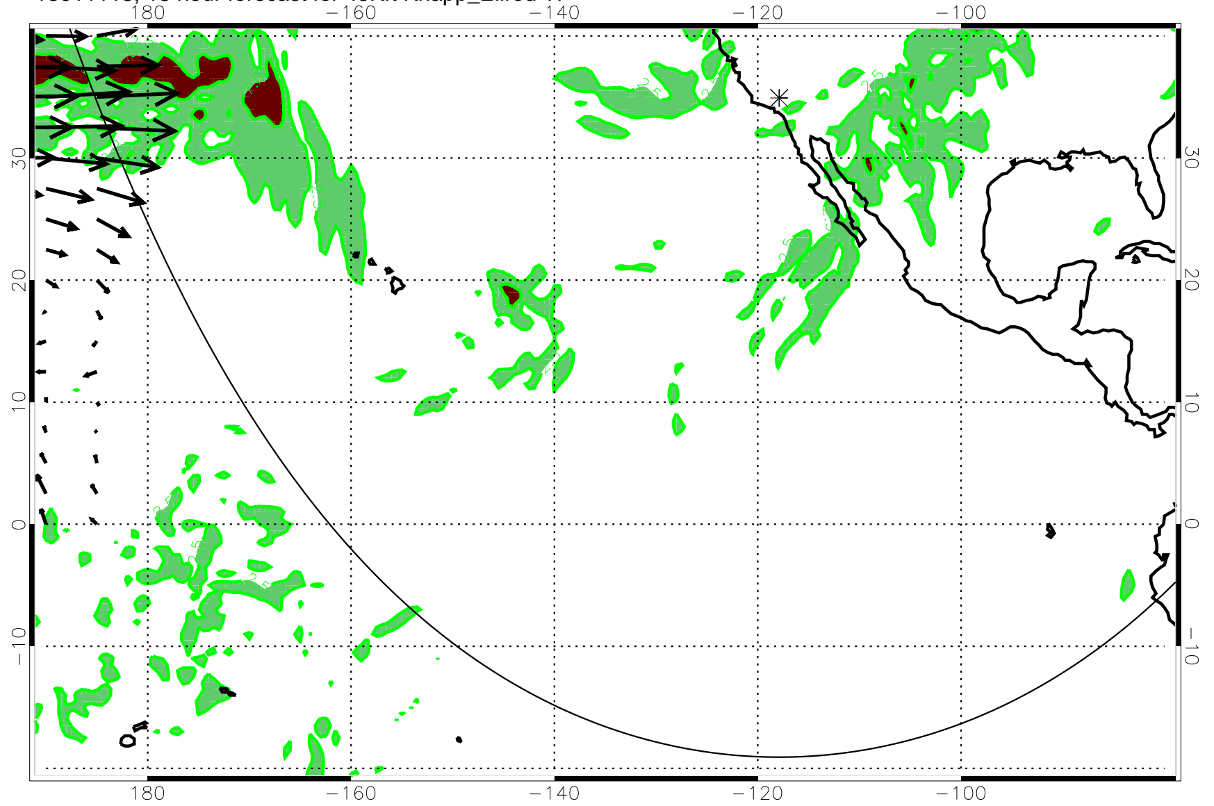
13011118, 18 hour forecast for 45Kft Knapp_Ellrod TI
