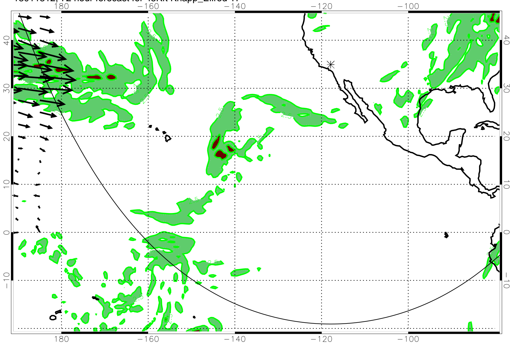
13011312, 72 hour forecast for 45Kft Knapp_Ellrod TI
