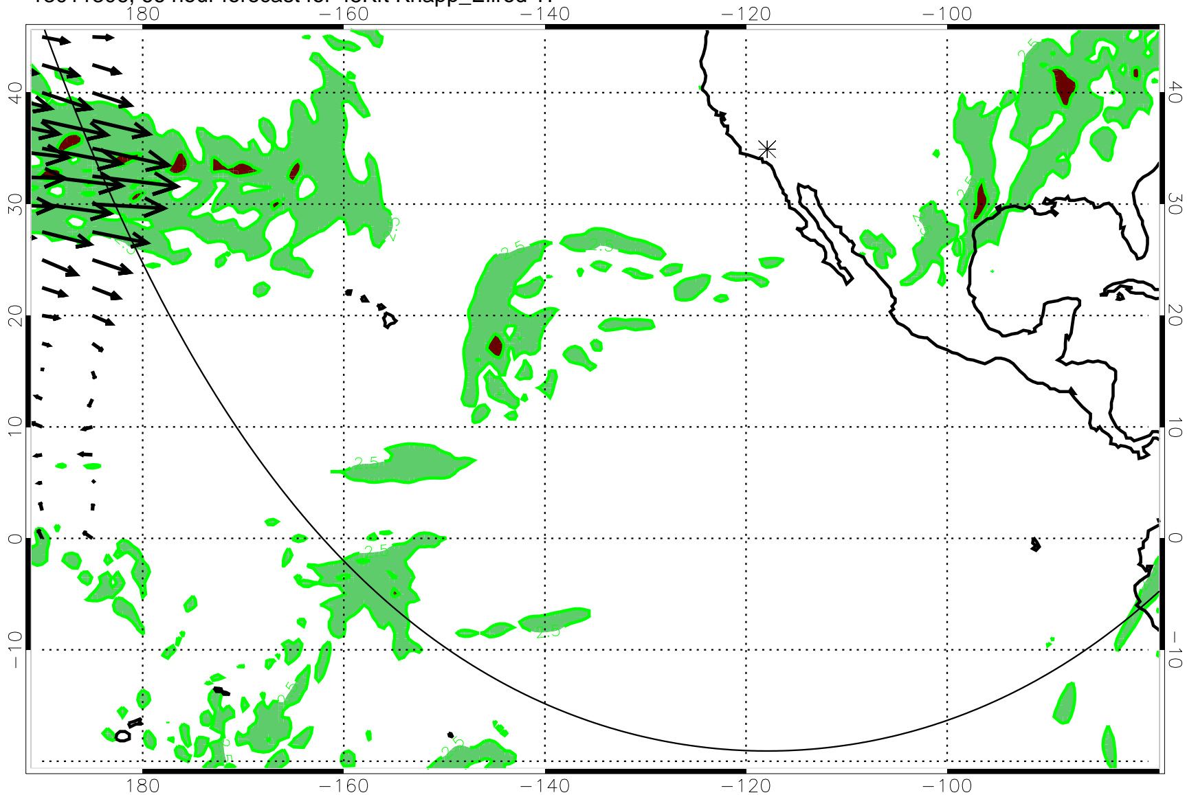
13011306, 66 hour forecast for 45Kft Knapp_Ellrod TI
