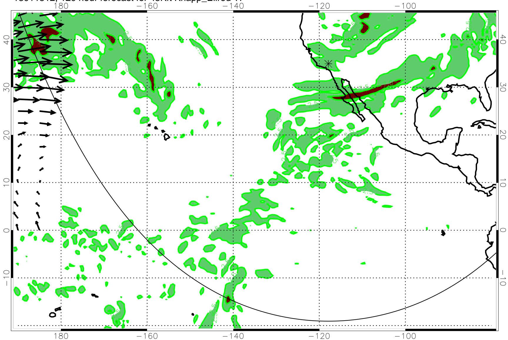
13011512, 120 hour forecast for 45Kft Knapp_Ellrod TI
