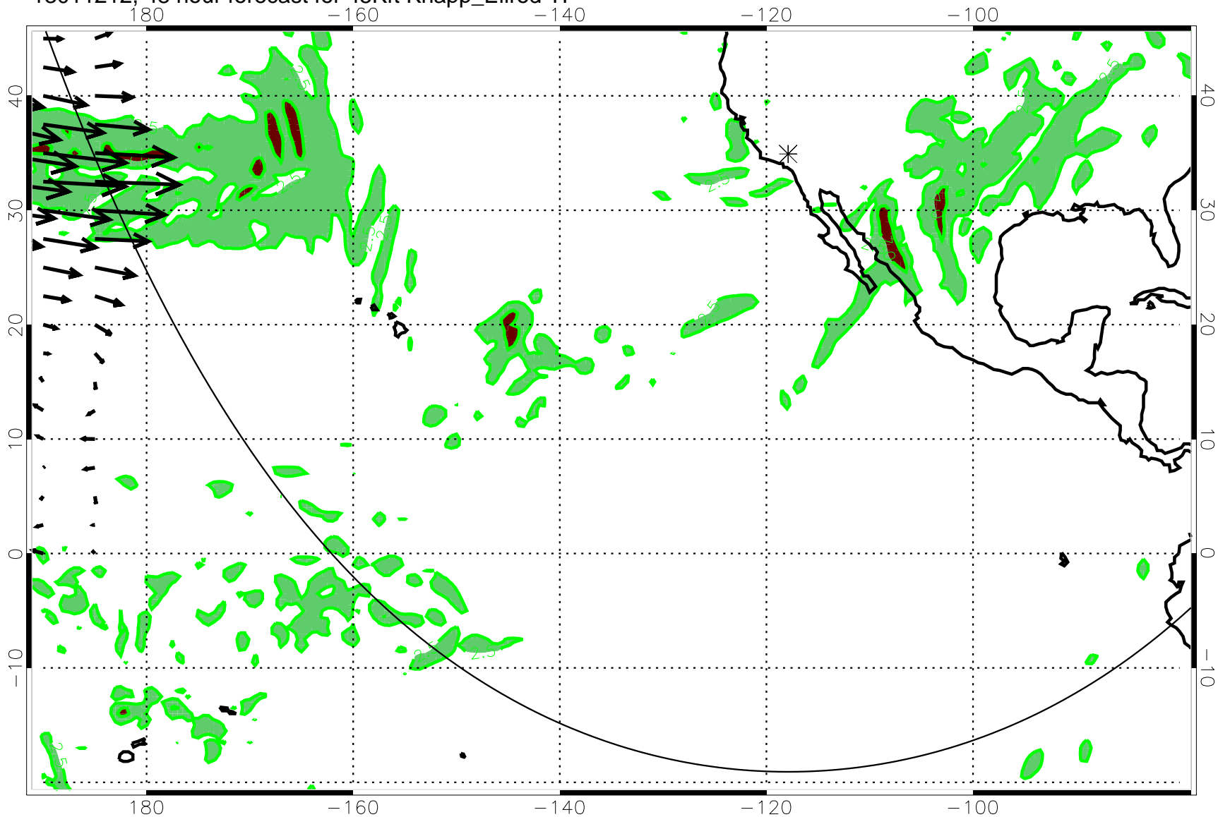
13011212, 48 hour forecast for 45Kft Knapp_Ellrod TI
