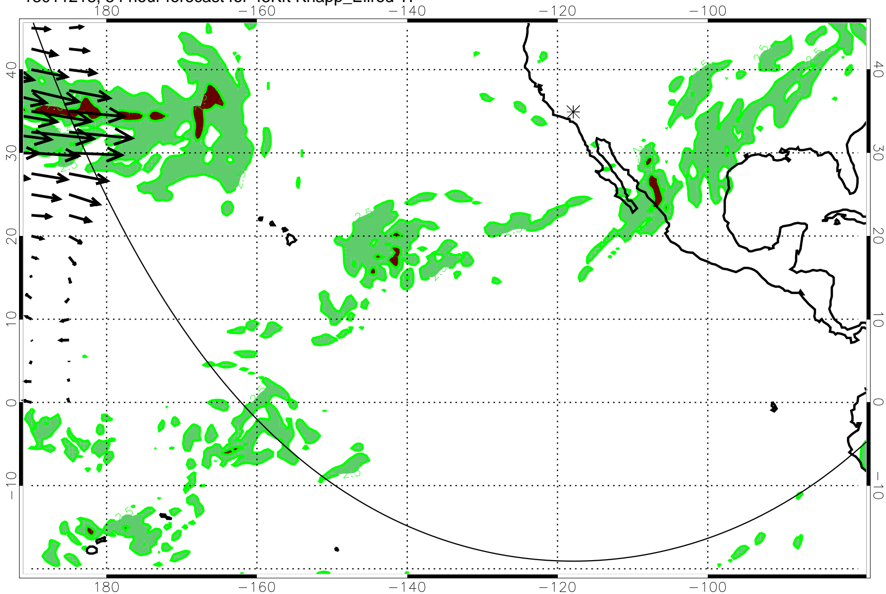
13011218, 54 hour forecast for 45Kft Knapp_Ellrod TI
