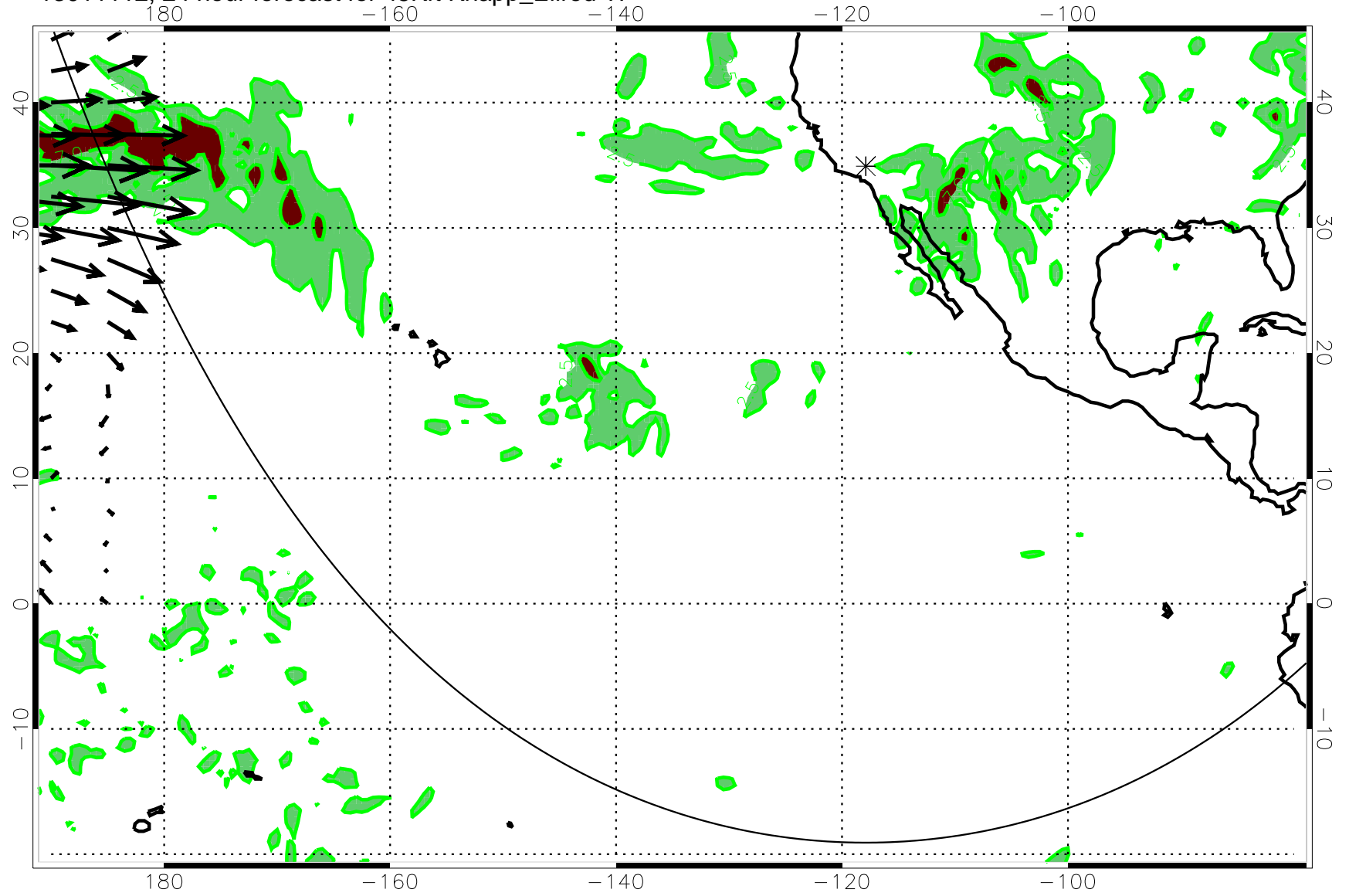
13011112, 24 hour forecast for 45Kft Knapp_Ellrod TI
