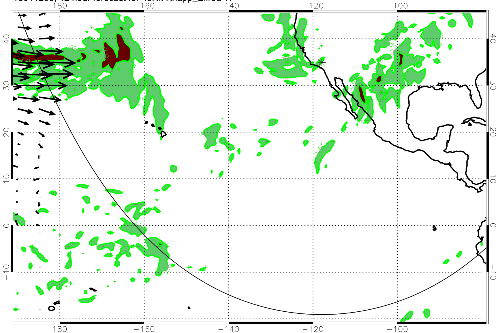
13011206, 42 hour forecast for 45Kft Knapp_Ellrod TI
