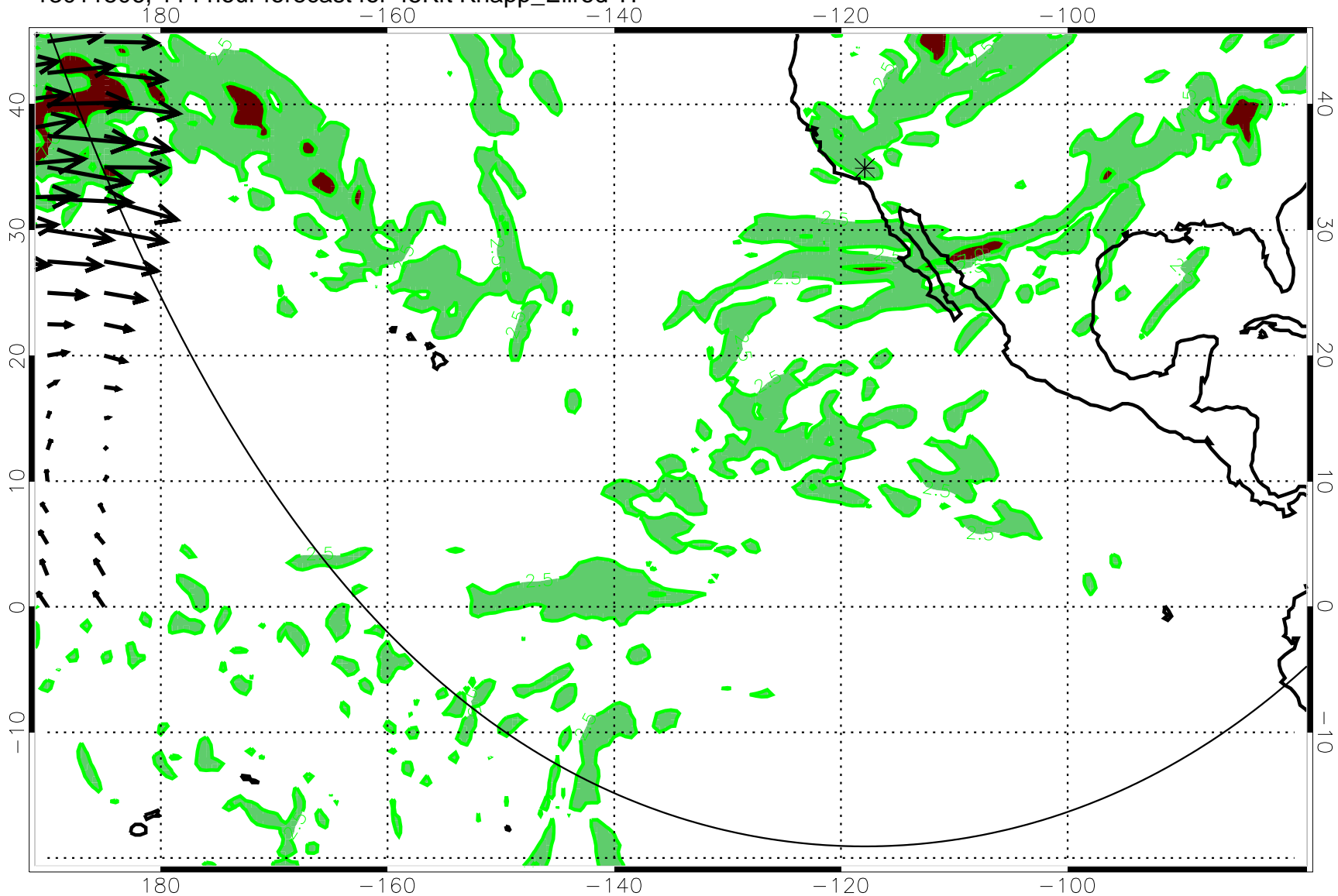
13011506, 114 hour forecast for 45Kft Knapp_Ellrod T1
