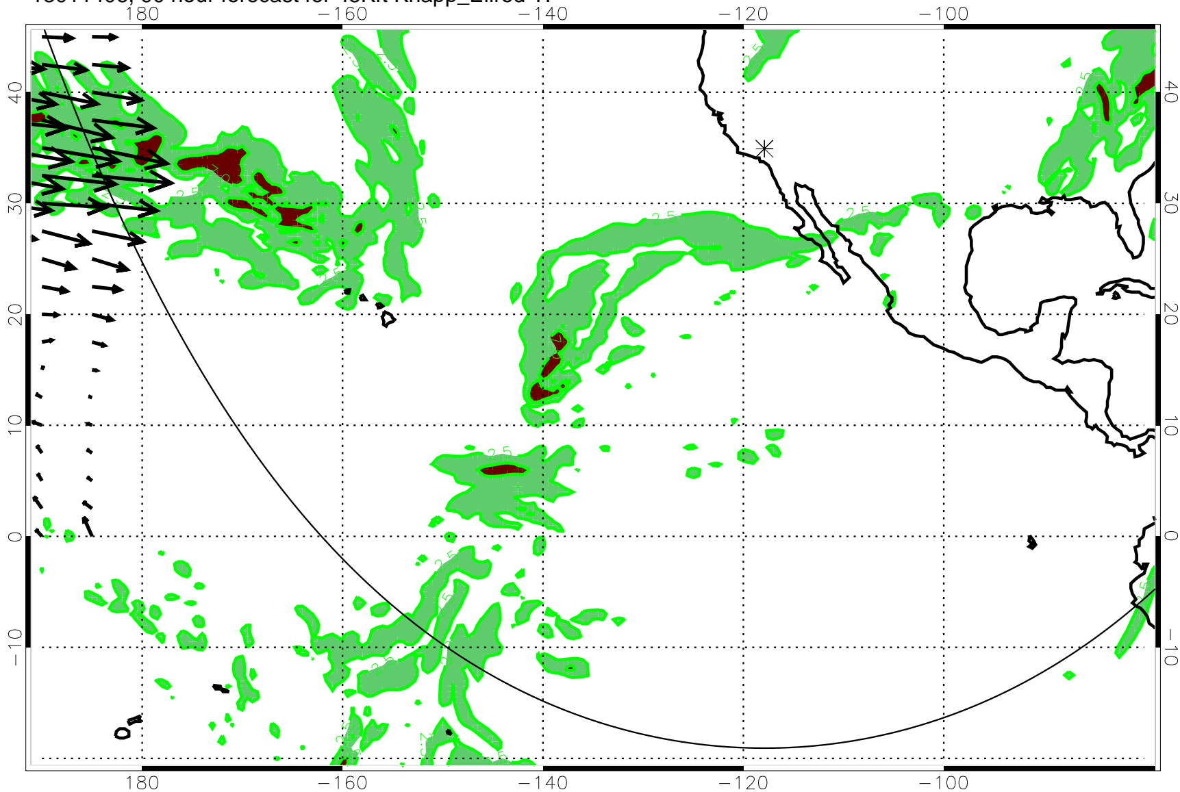
13011406, 90 hour forecast for 45Kft Knapp_Ellrod TI
