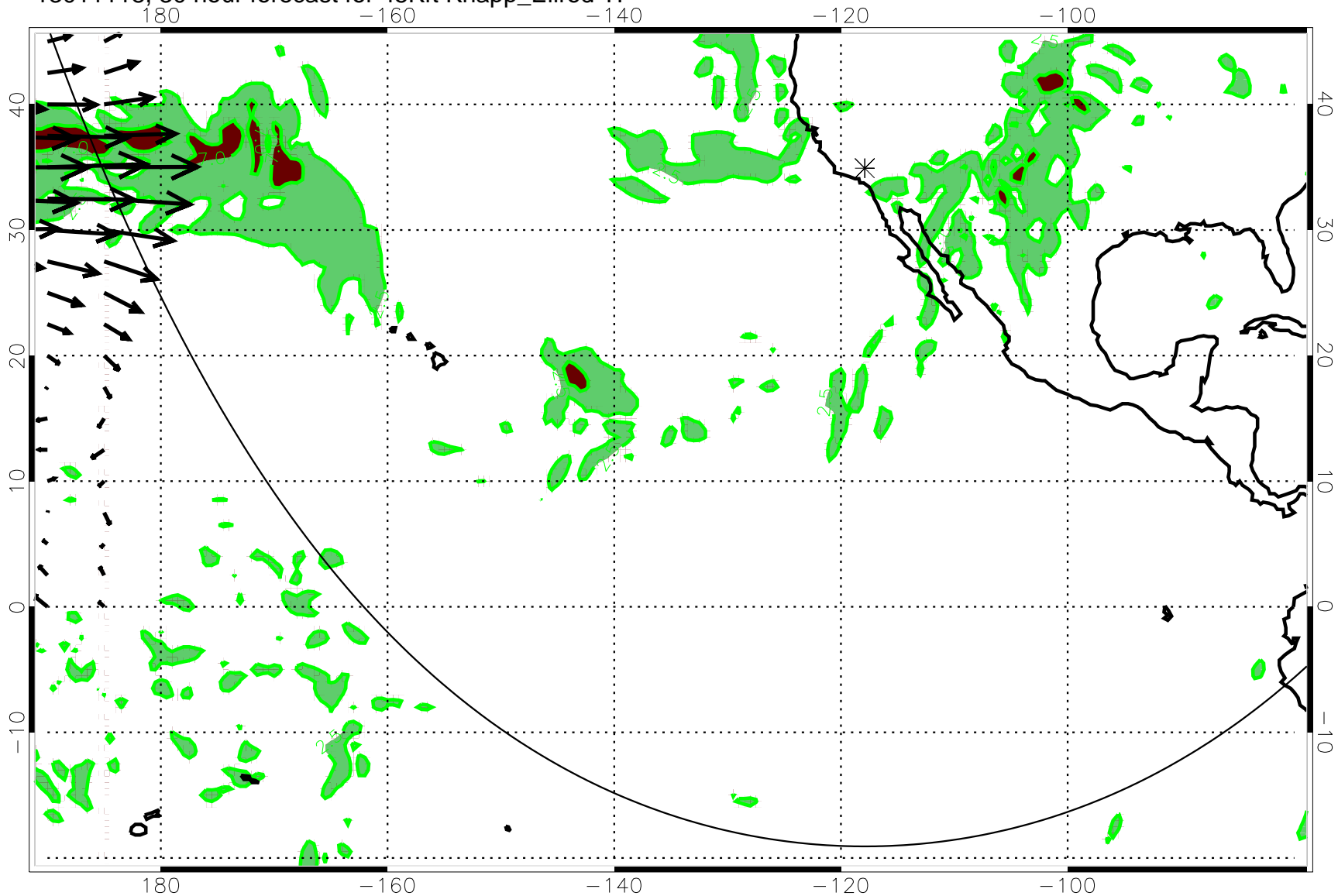
13011118, 30 hour forecast for 45Kft Knapp_Ellrod TI
