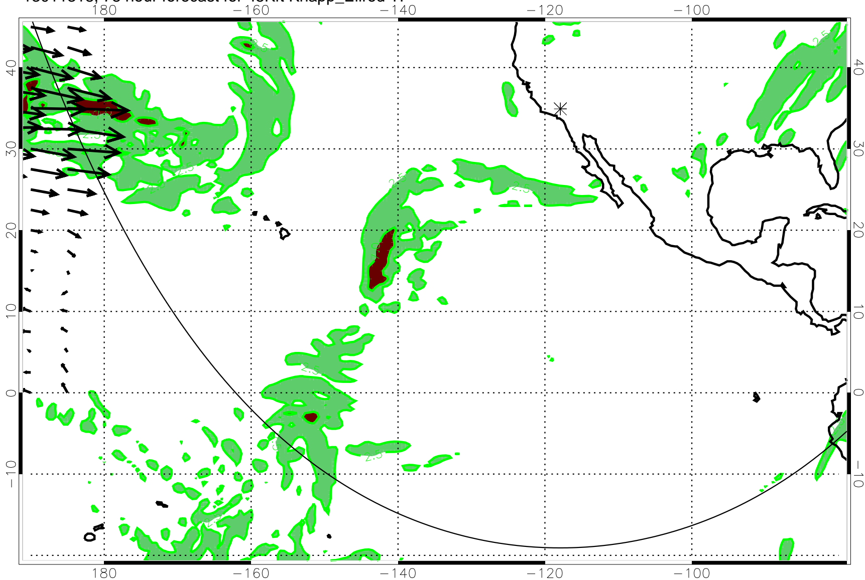
13011318, 78 hour forecast for 45Kft Knapp_Ellrod TI
