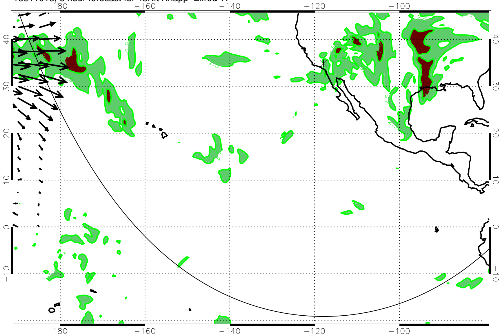
13011018, 6 hour forecast for 45Kft Knapp_Ellrod TI
