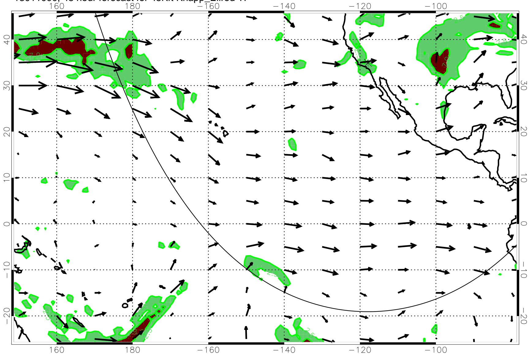
13011000, 48 hour forecast for 45Kft Knapp_Ellrod T1
