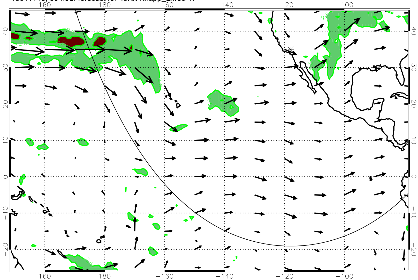
13011118, 90 hour forecast for 45Kft Knapp_Ellrod TI
