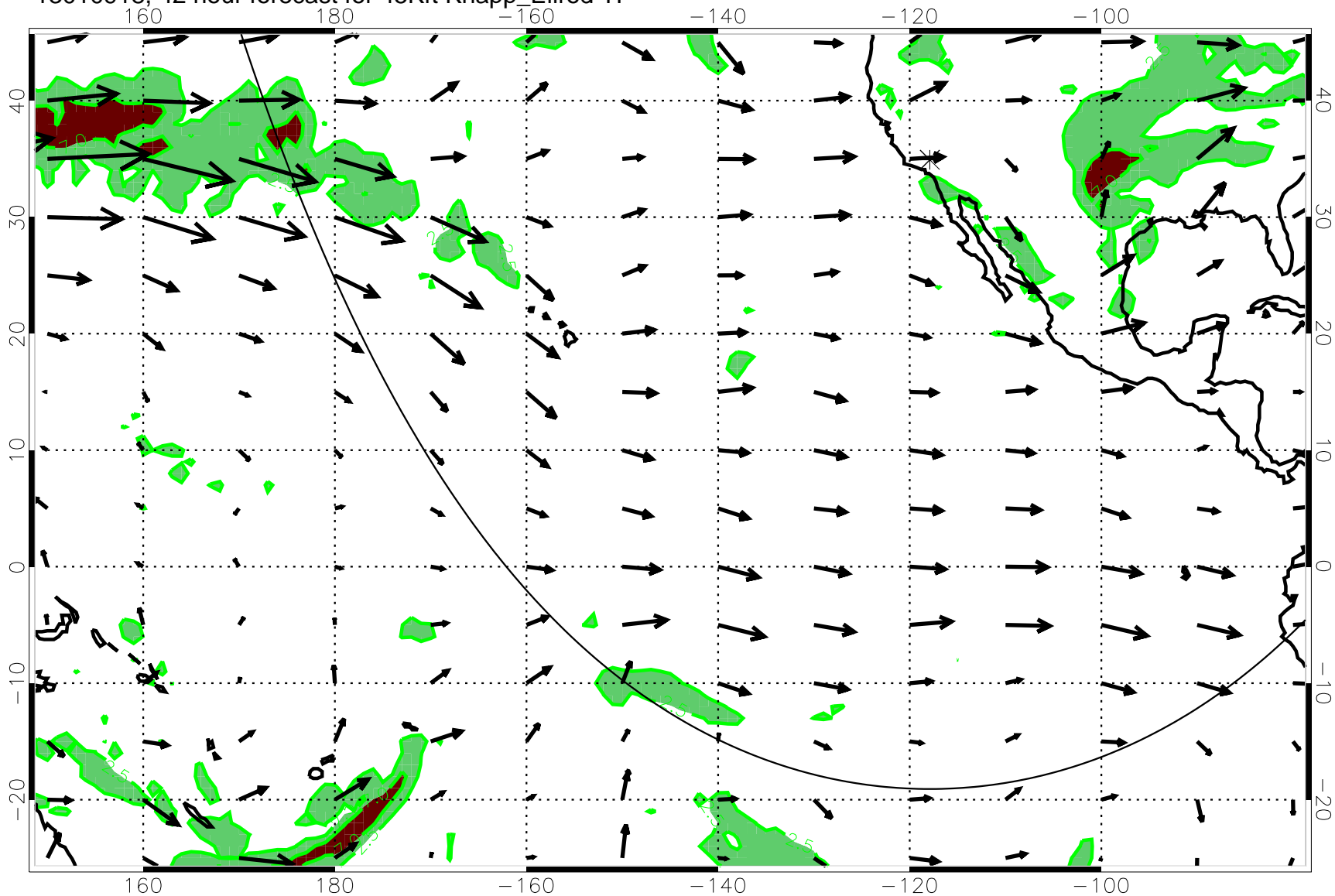
13010918, 42 hour forecast for 45Kft Knapp_Ellrod T1
