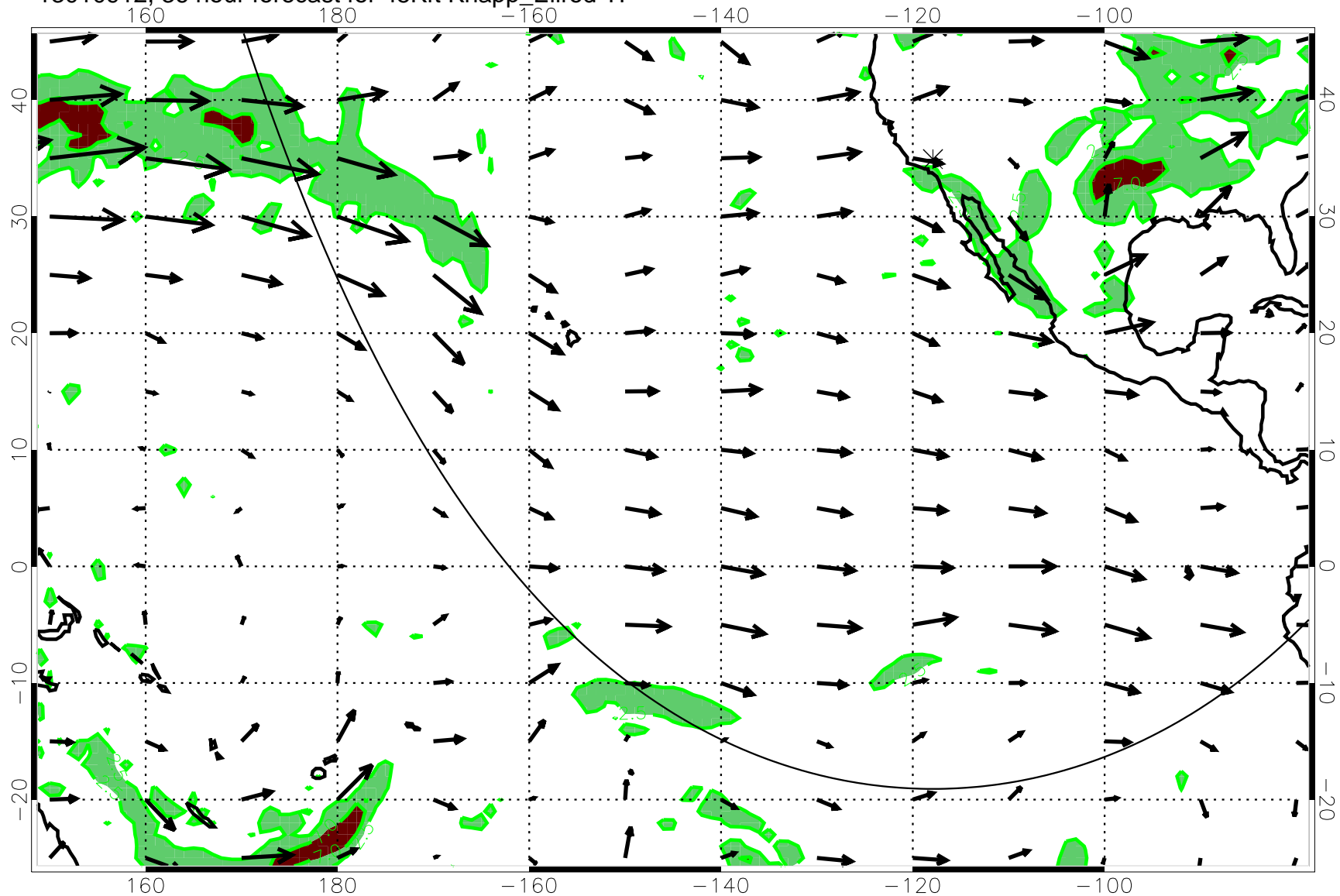
13010912, 36 hour forecast for 45Kft Knapp_Ellrod TI
