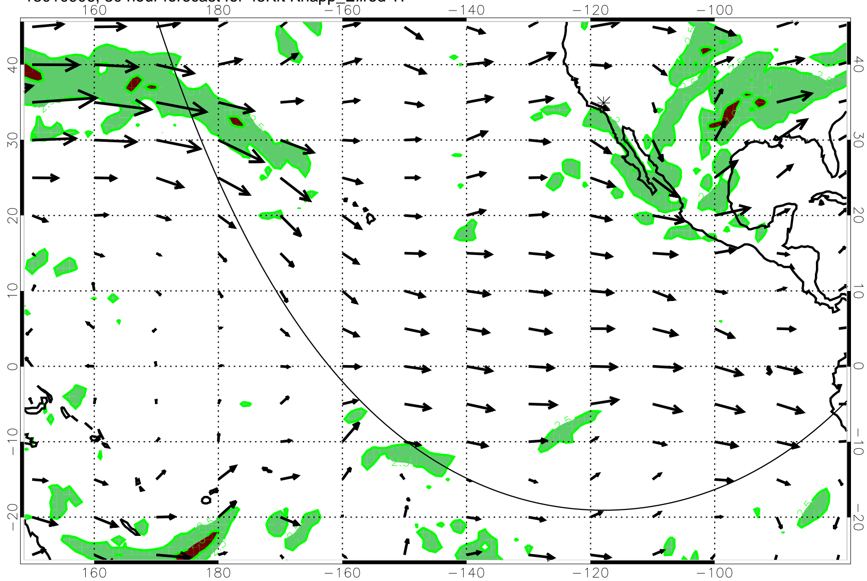
13010906, 30 hour forecast for 45Kft Knapp_Ellrod T1
