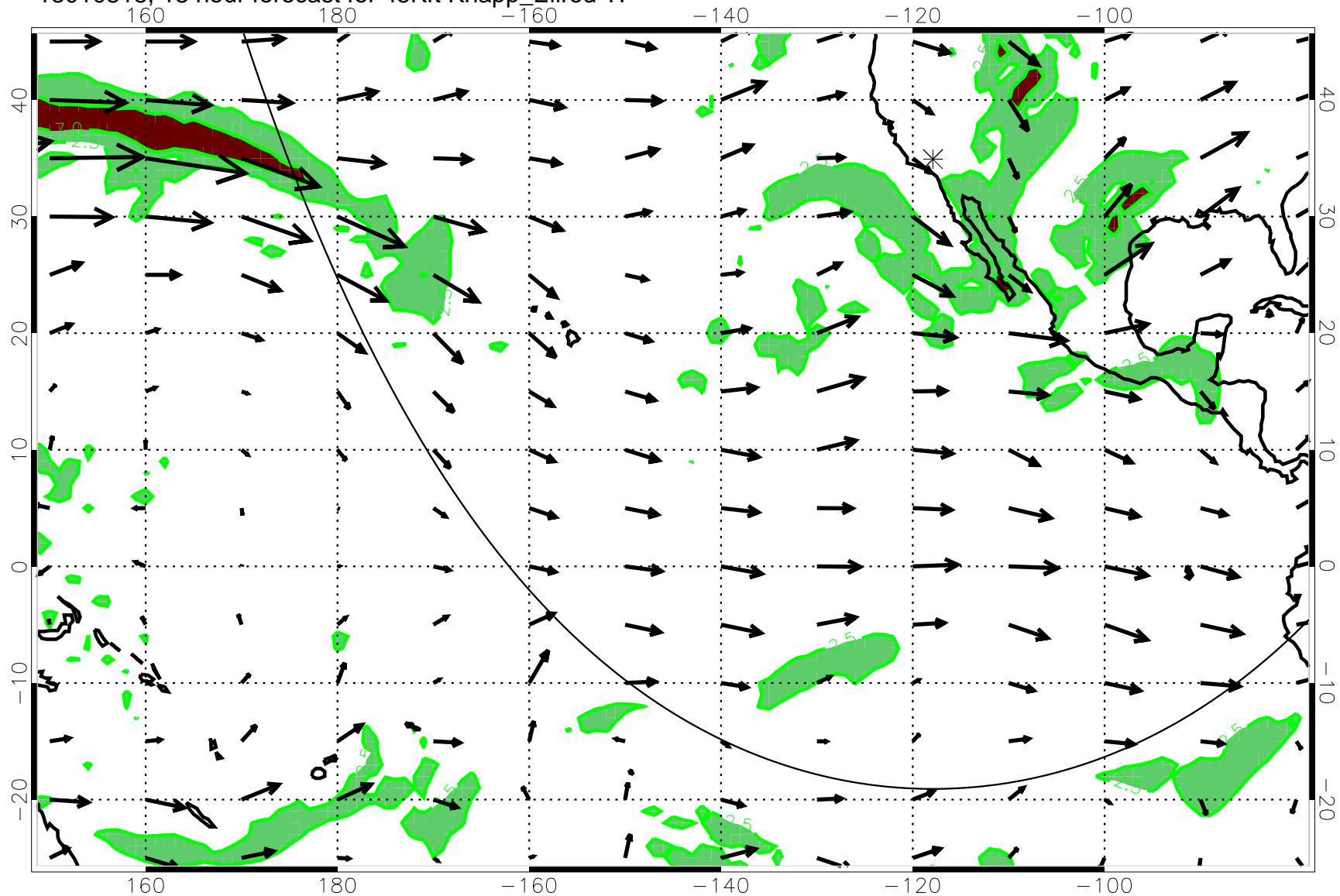
13010818, 18 hour forecast for 45Kft Knapp_Ellrod T1
