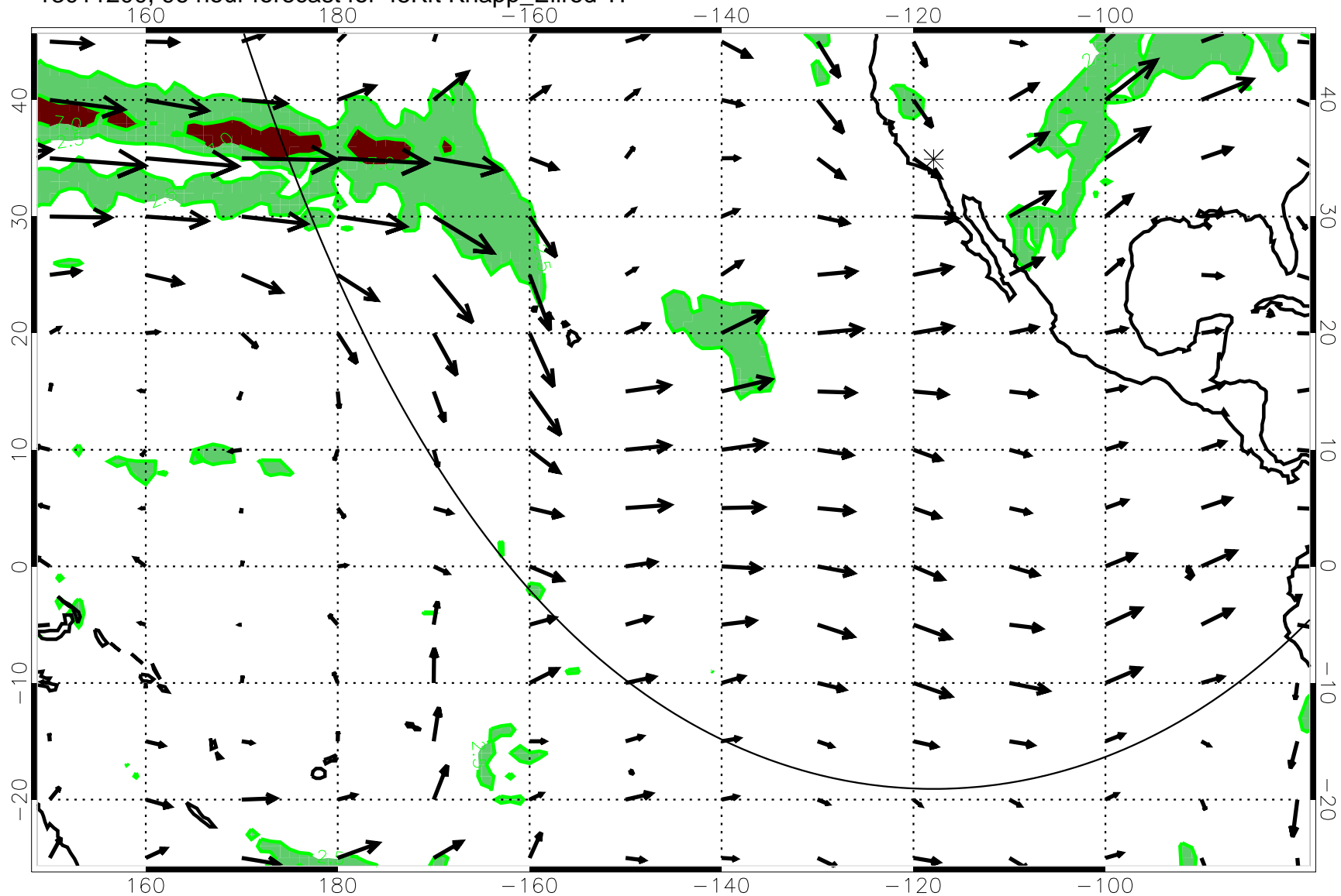
13011200, 96 hour forecast for 45Kft Knapp_Ellrod T1
