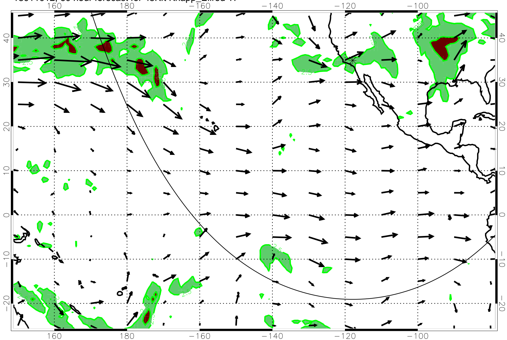
13011012, 60 hour forecast for 45Kft Knapp_Ellrod T1
