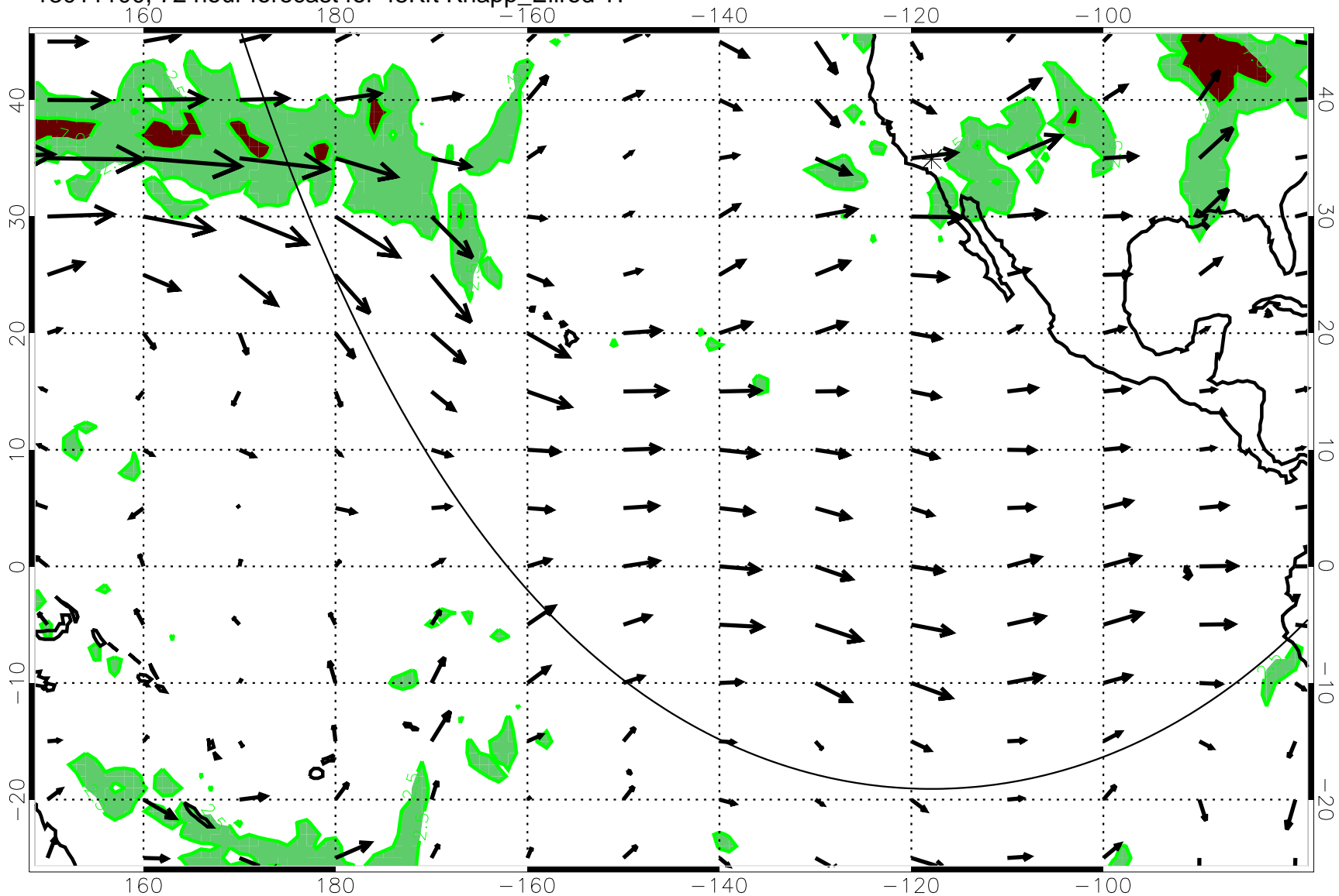
13011100, 72 hour forecast for 45Kft Knapp_Ellrod T1
