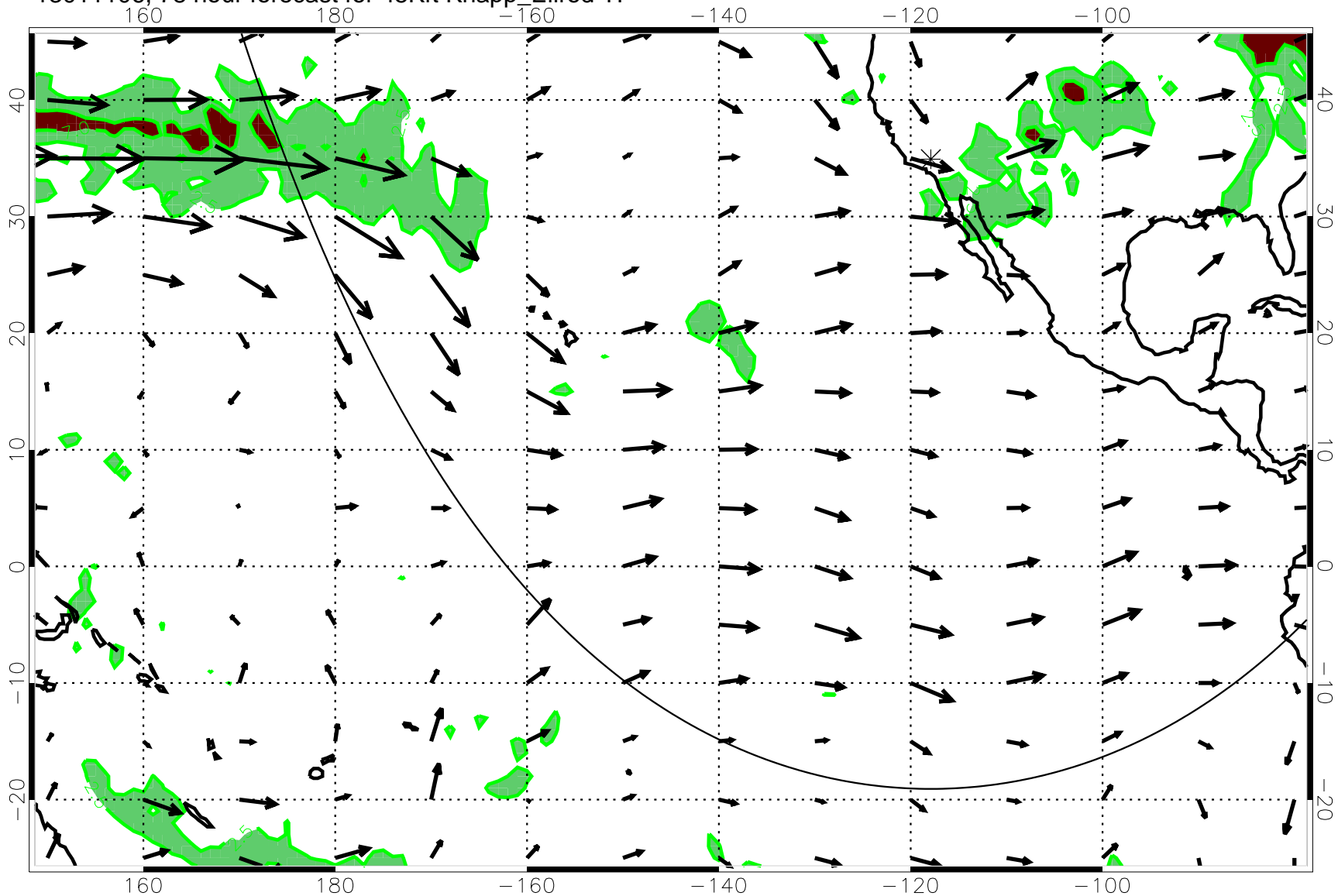
13011106, 78 hour forecast for 45Kft Knapp_Ellrod T1
