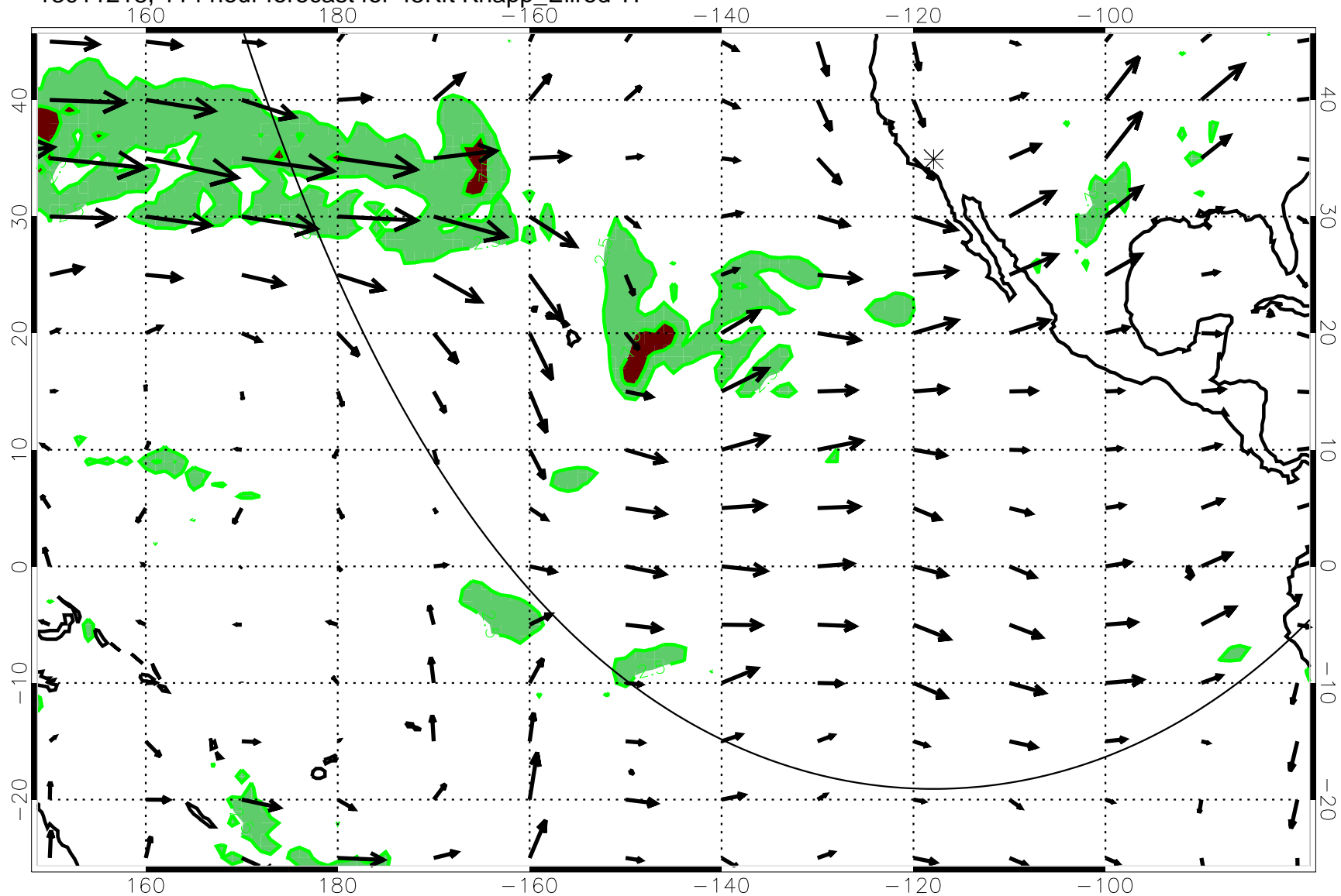
13011218, 114 hour forecast for 45Kft Knapp_Ellrod T1
