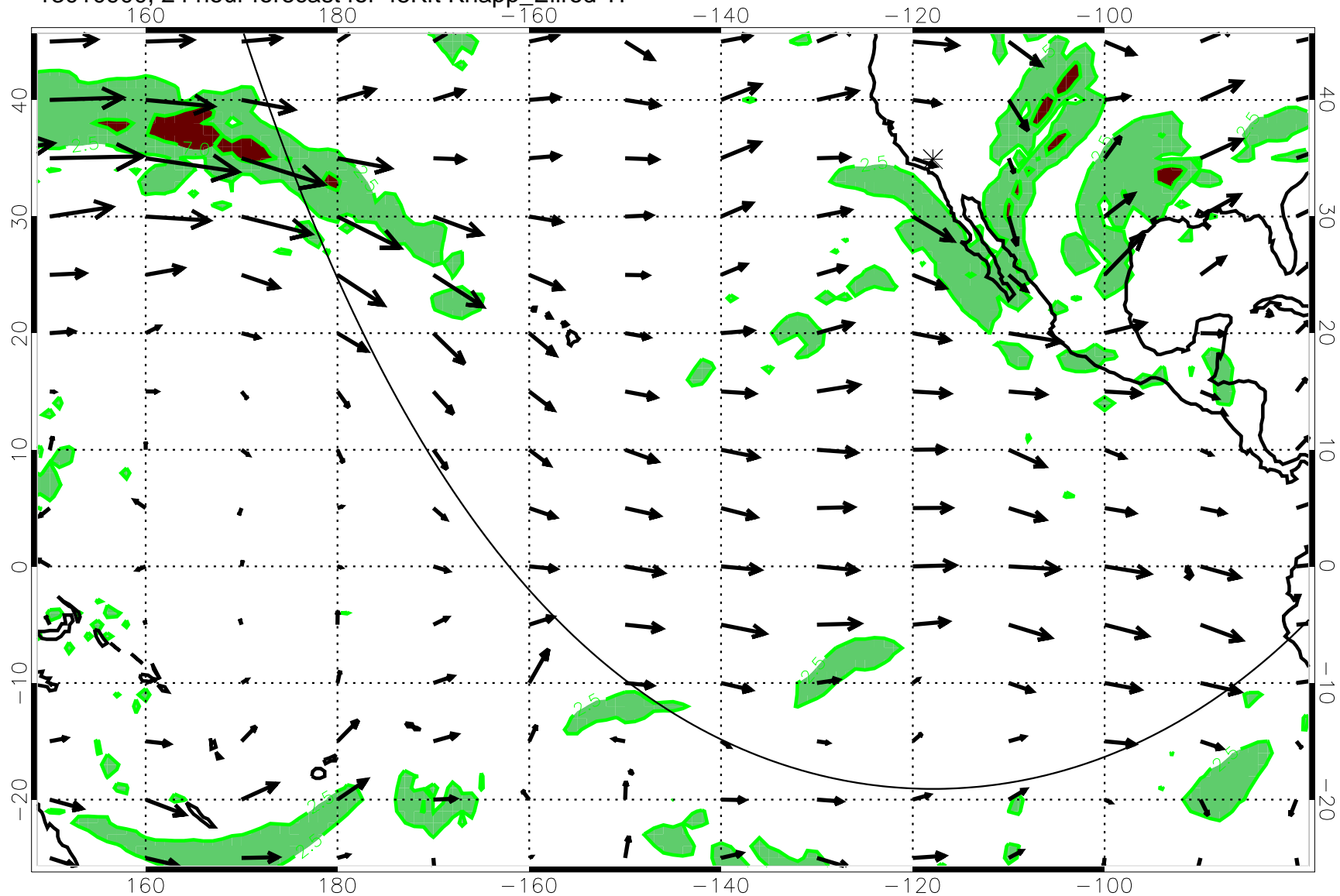
13010900, 24 hour forecast for 45Kft Knapp_Ellrod T1
