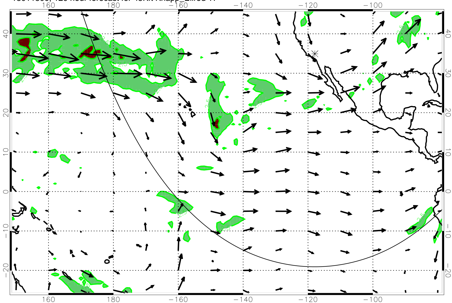
13011300, 120 hour forecast for 45Kft Knapp_Ellrod T1
