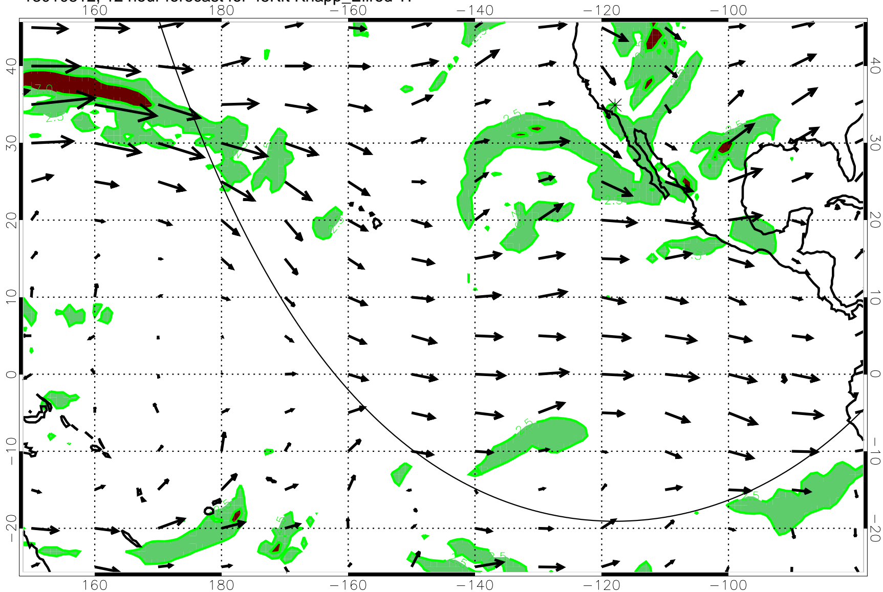
13010812, 12 hour forecast for 45Kft Knapp_Ellrod T1
