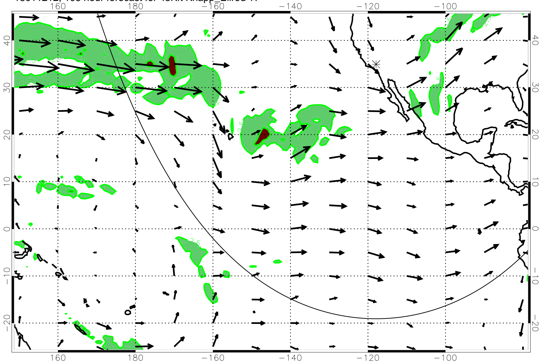
13011212, 108 hour forecast for 45Kft Knapp_Ellrod T1
