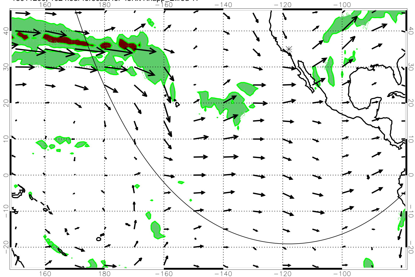
13011206, 102 hour forecast for 45Kft Knapp_Ellrod T1
