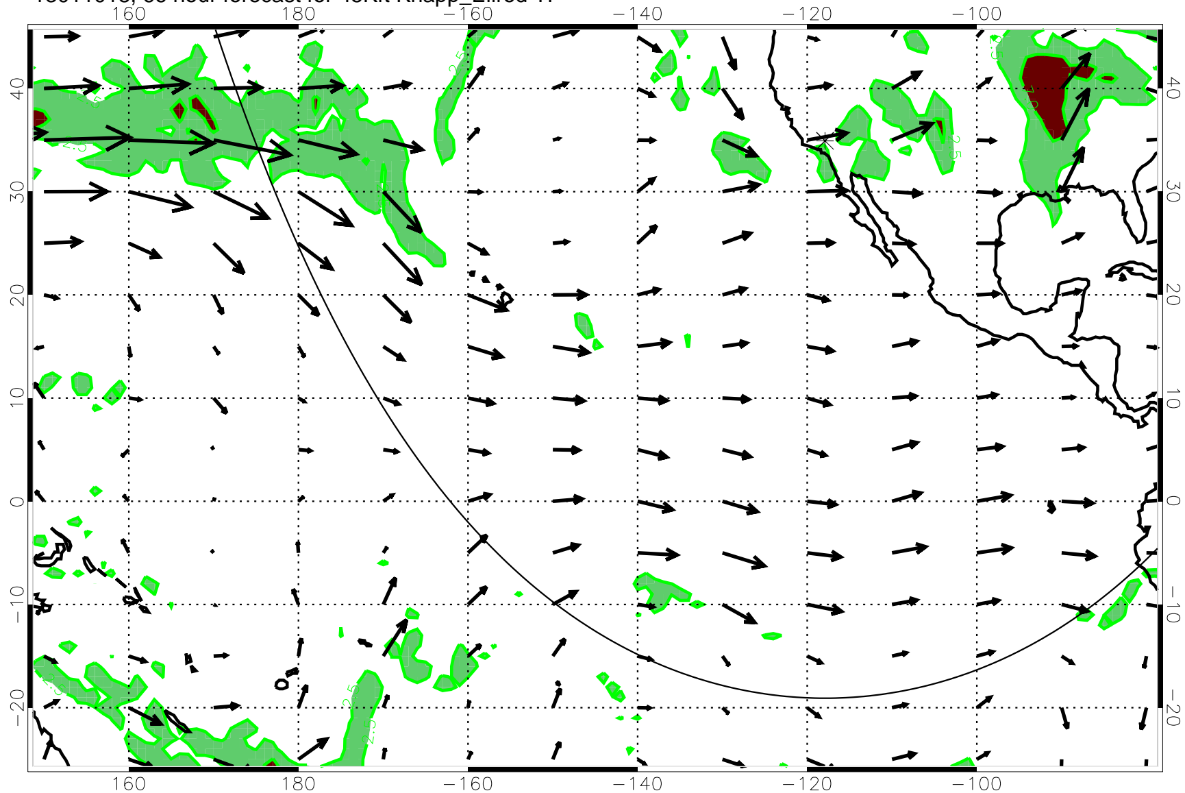
13011018, 66 hour forecast for 45Kft Knapp_Ellrod T1
