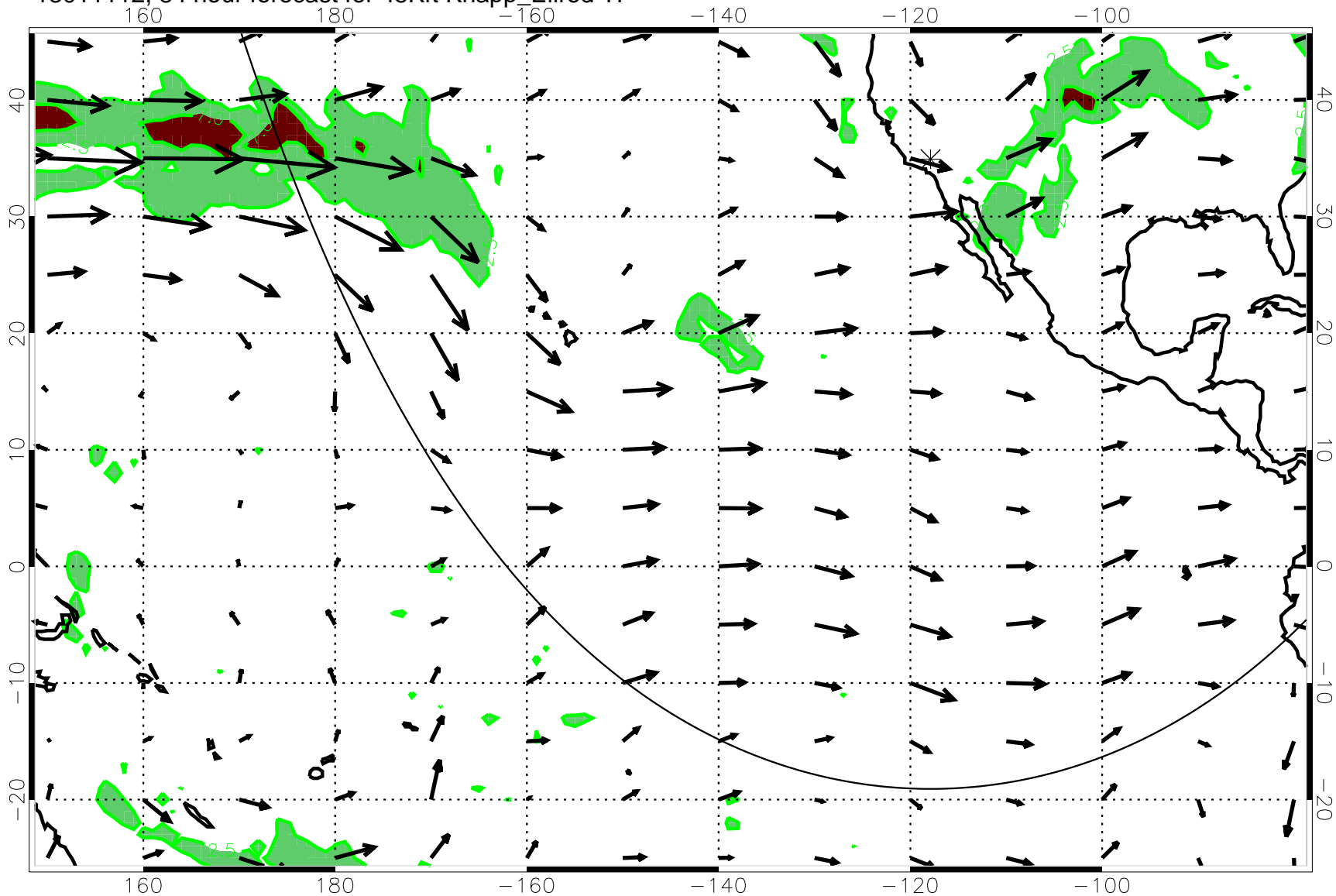
13011112, 84 hour forecast for 45Kft Knapp_Ellrod T1
