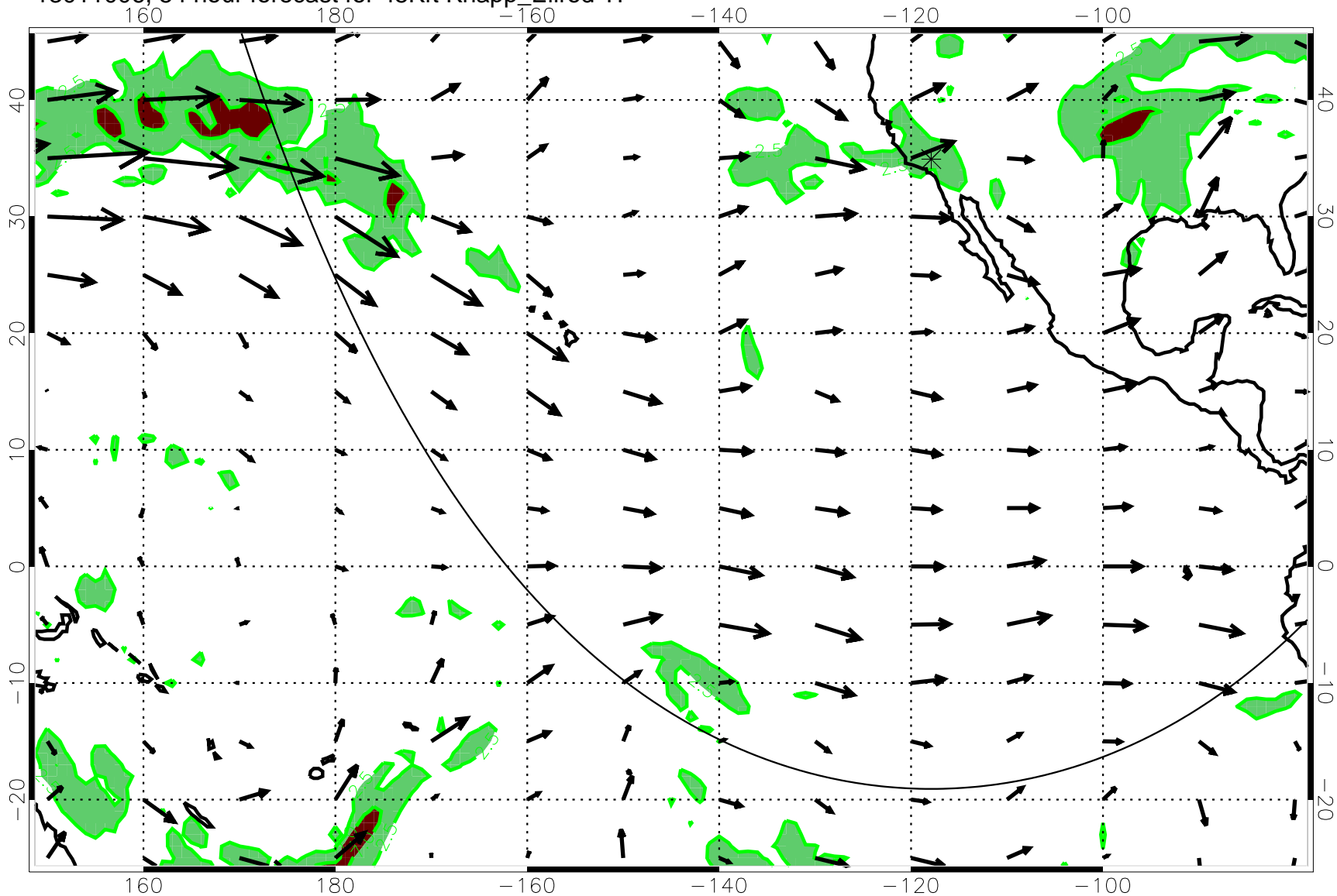
13011006, 54 hour forecast for 45Kft Knapp_Ellrod T1
