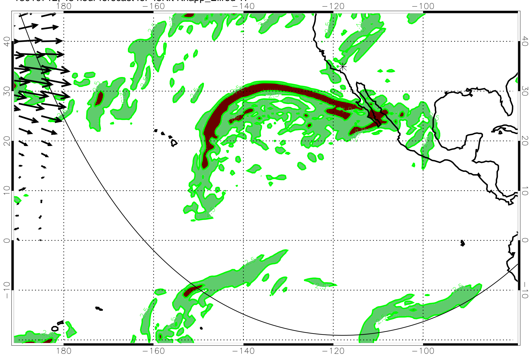
13010712, 48 hour forecast for 45Kft Knapp_Ellrod TI
