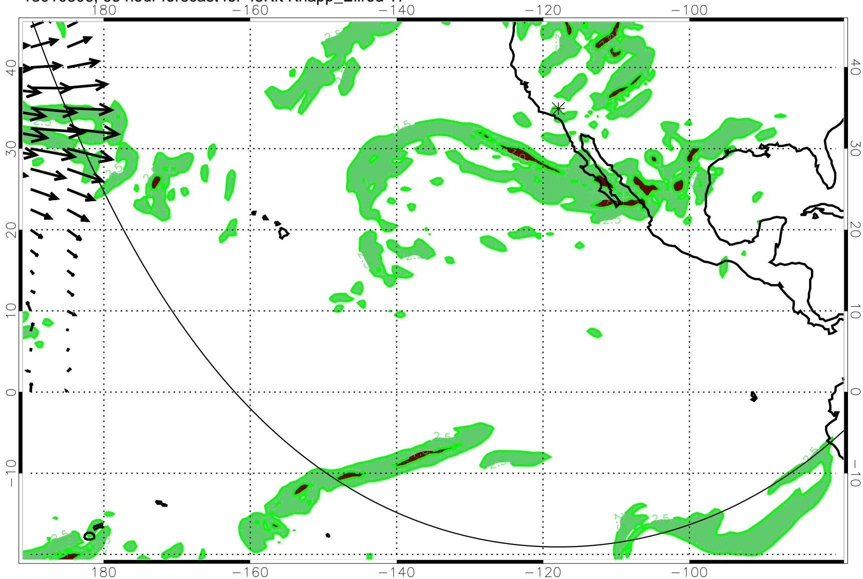
13010806, 66 hour forecast for 45Kft Knapp_Ellrod TI
