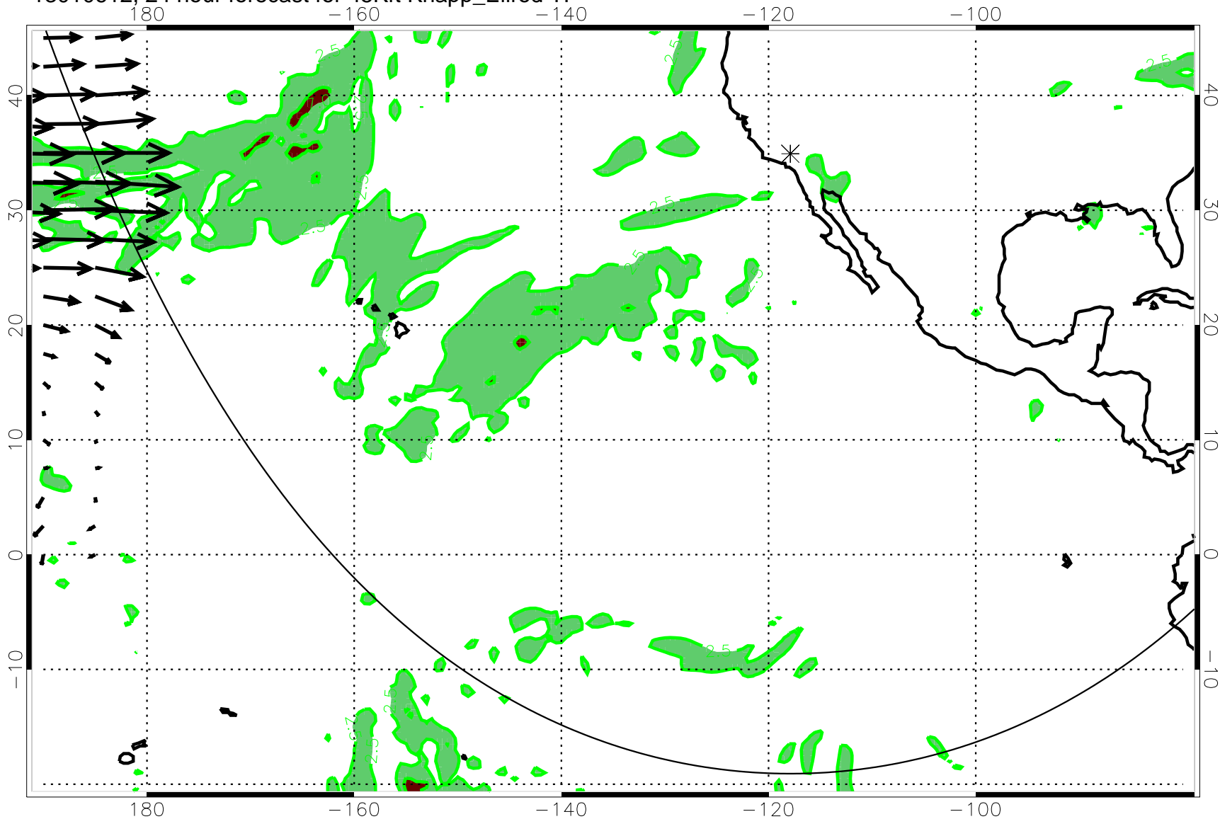
13010612, 24 hour forecast for 45Kft Knapp_Ellrod TI
