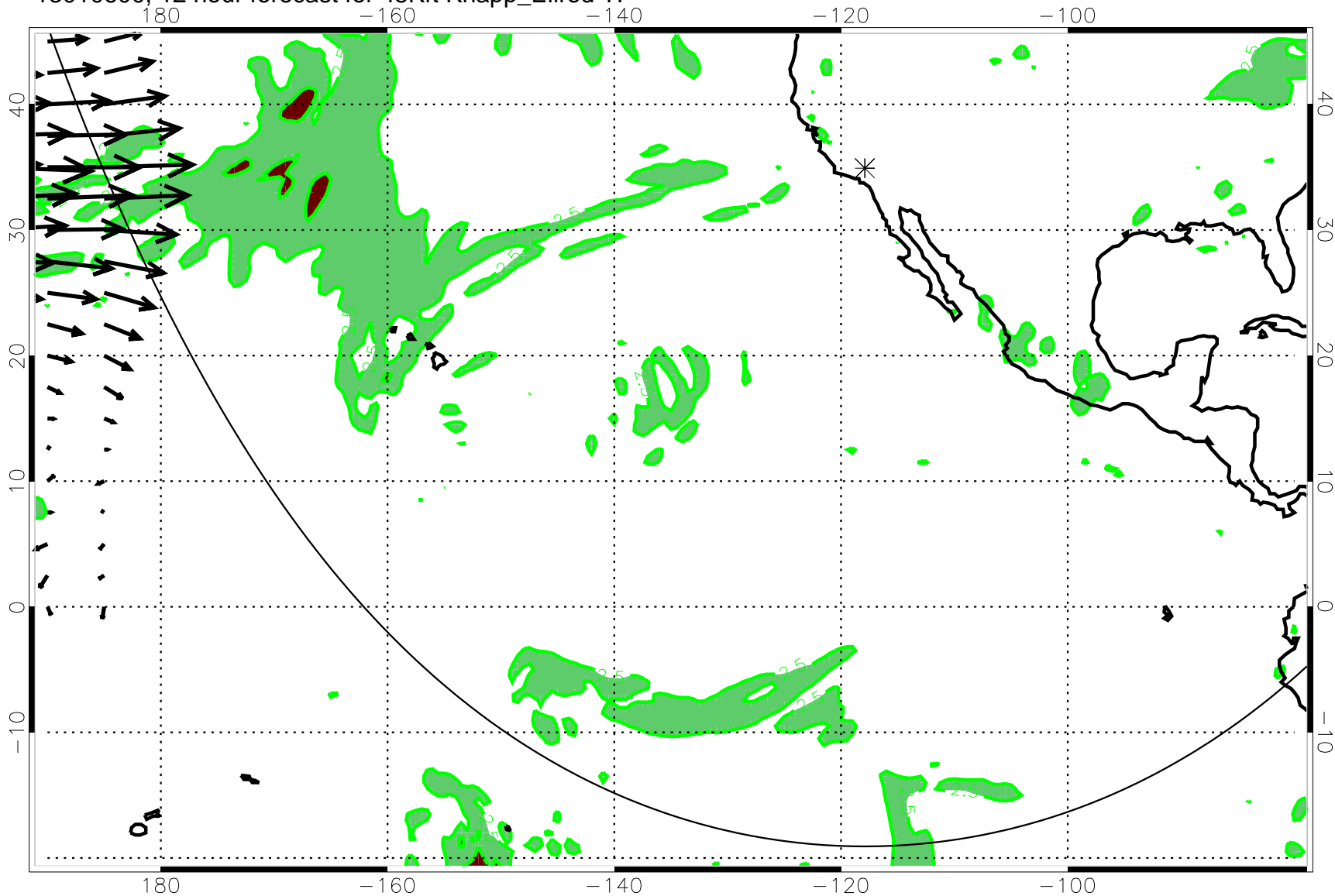
13010600, 12 hour forecast for 45Kft Knapp_Ellrod TI
