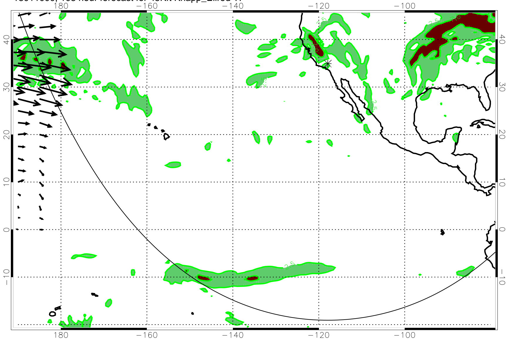
13011000, 108 hour forecast for 45Kft Knapp_Ellrod TI
