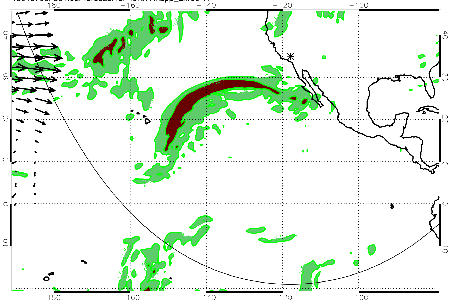
13010700, 36 hour forecast for 45Kft Knapp_Ellrod TI
