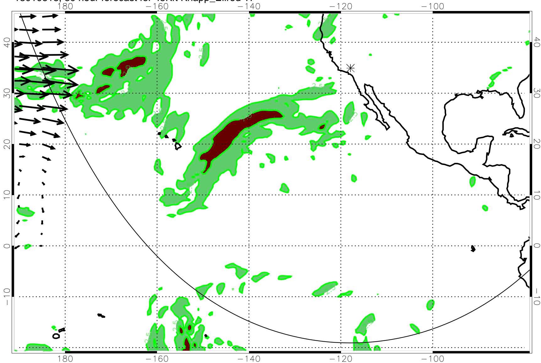
13010618, 30 hour forecast for 45Kft Knapp_Ellrod TI
