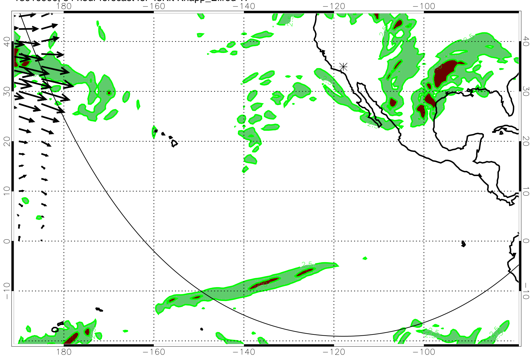
13010900, 84 hour forecast for 45Kft Knapp_Ellrod TI
