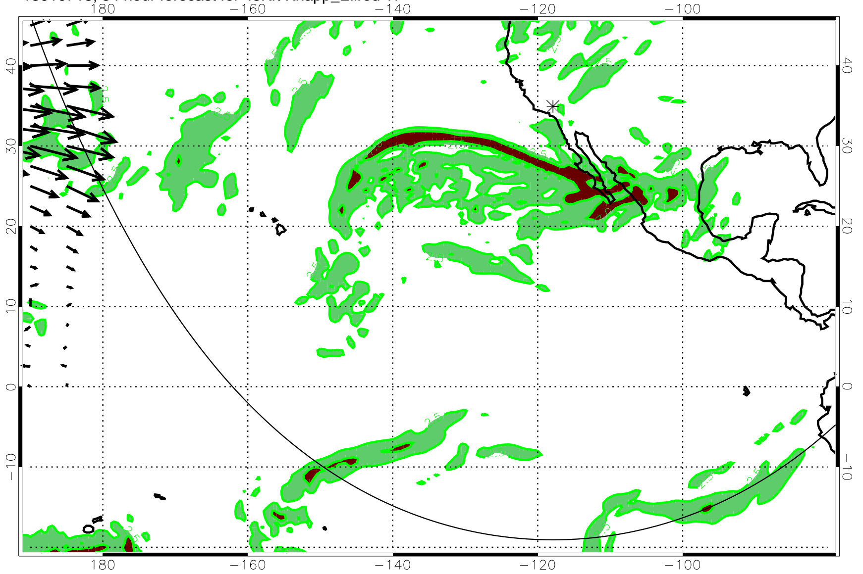
13010718, 54 hour forecast for 45Kft Knapp_Ellrod TI
