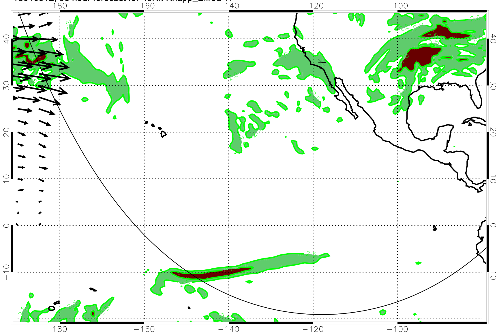
13010912, 96 hour forecast for 45Kft Knapp_Ellrod TI
