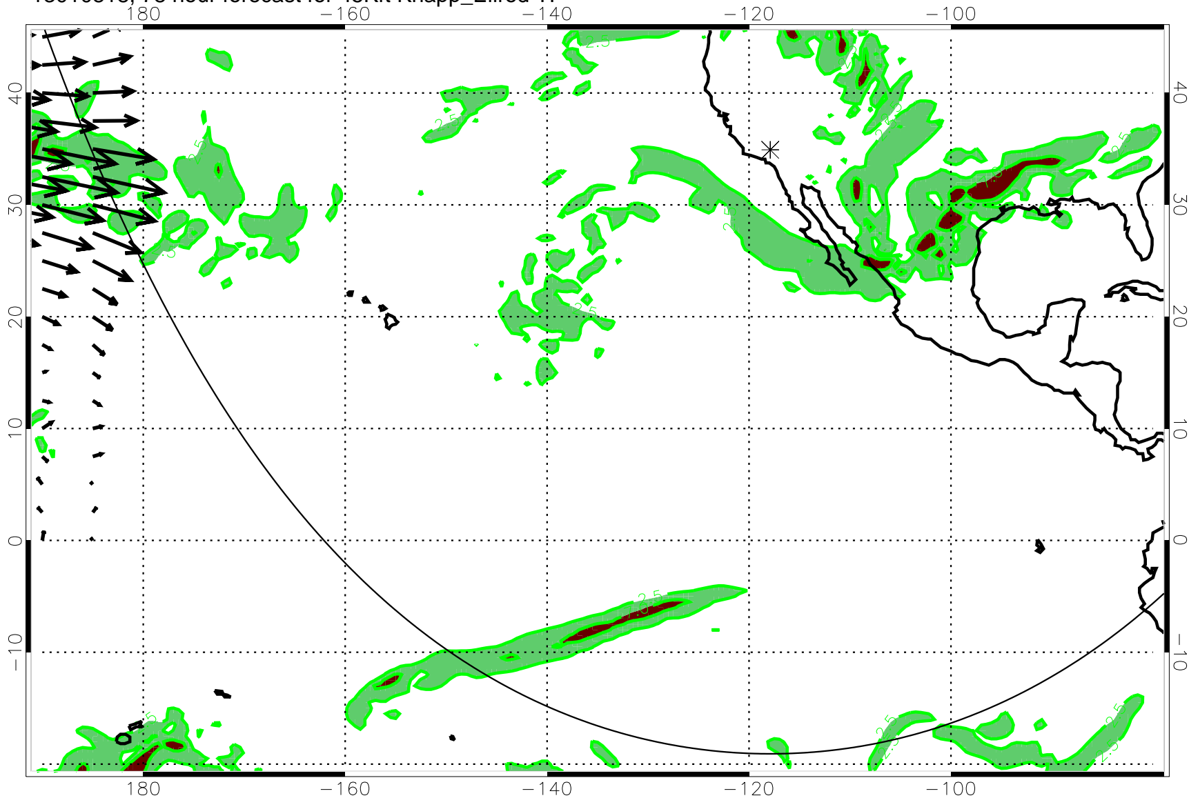
13010818, 78 hour forecast for 45Kft Knapp_Ellrod TI
