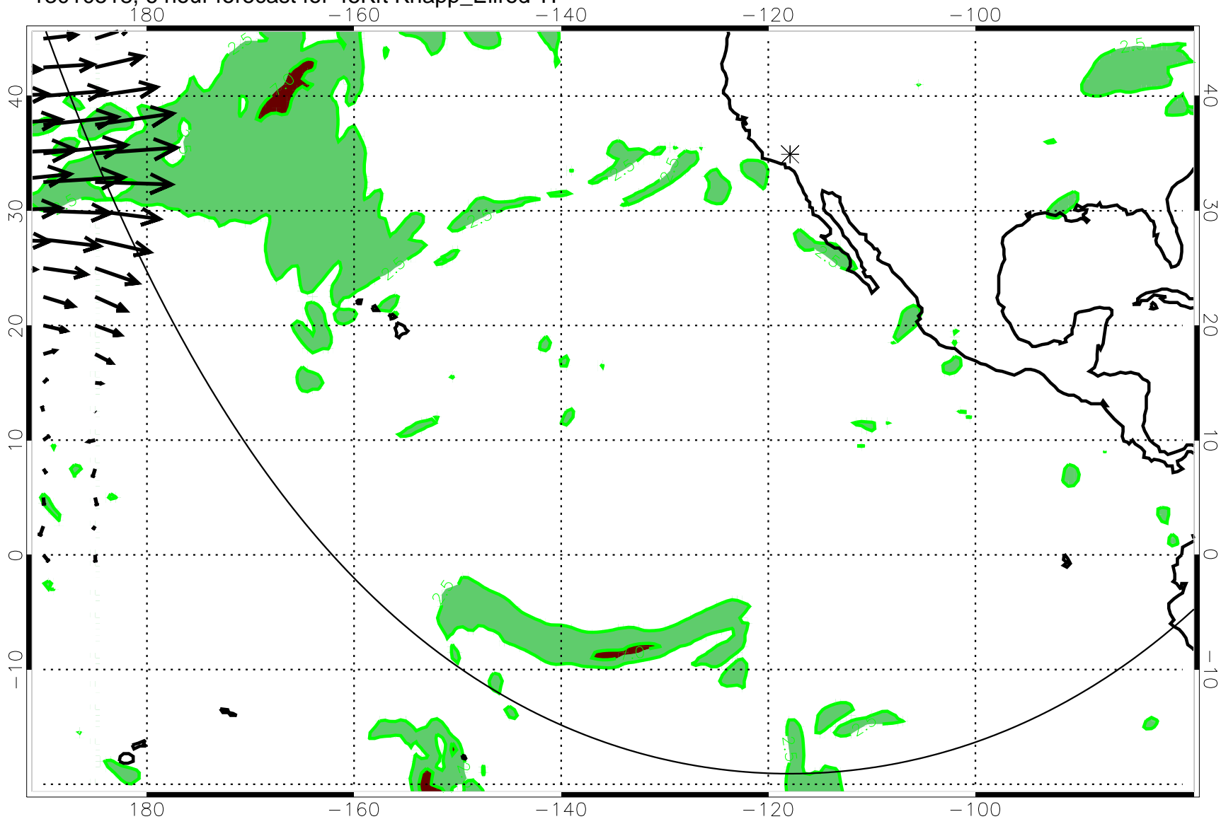
13010518, 6 hour forecast for 45Kft Knapp_Ellrod TI
