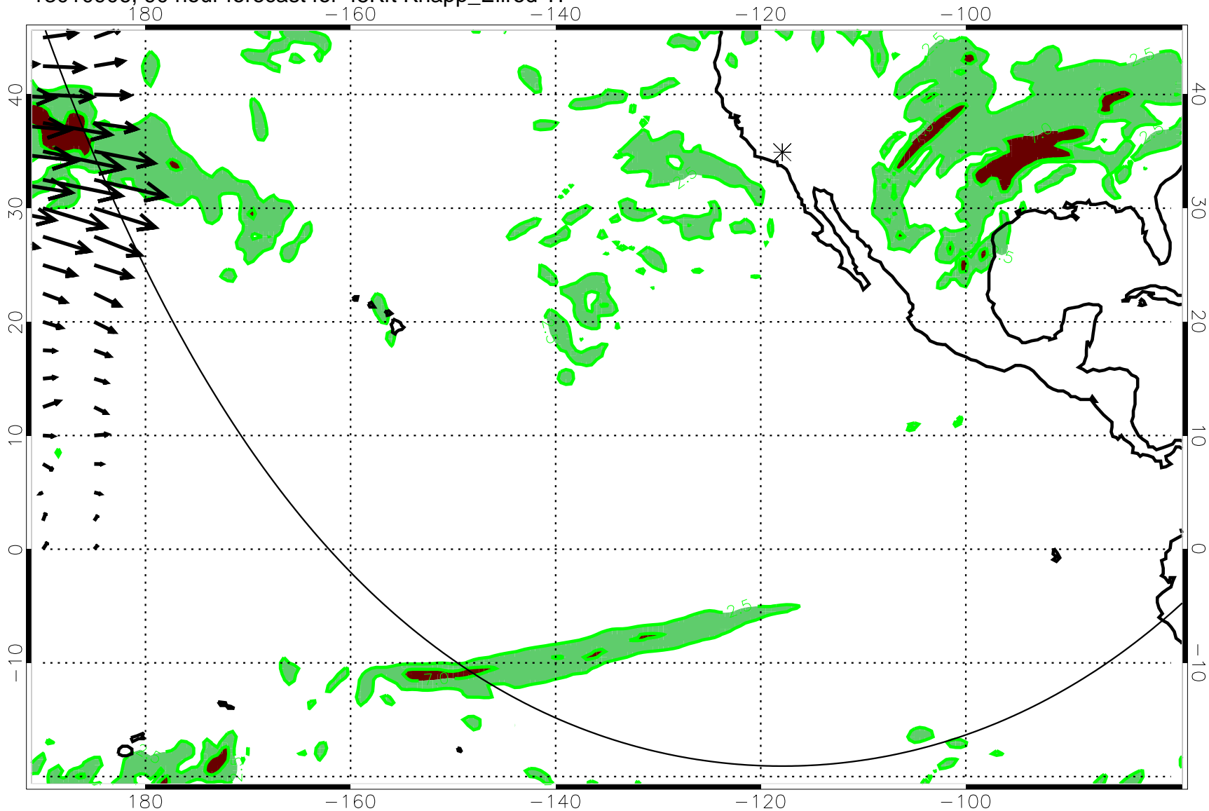
13010906, 90 hour forecast for 45Kft Knapp_Ellrod TI
