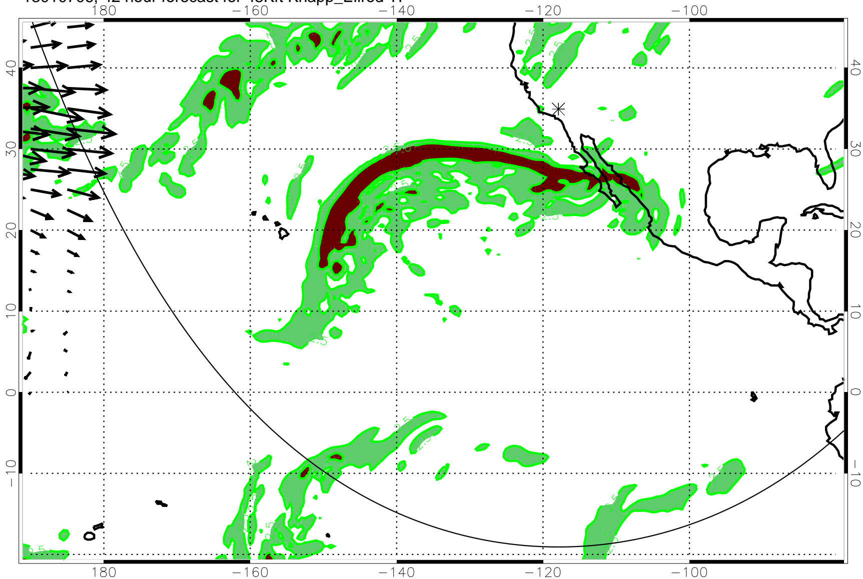
13010706, 42 hour forecast for 45Kft Knapp_Ellrod TI
