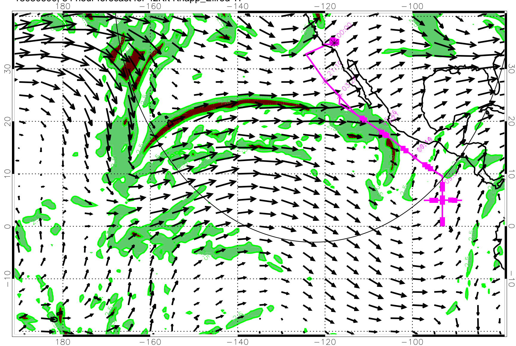
13030600, 84 hour forecast for 42Kft Knapp_Ellrod TI
