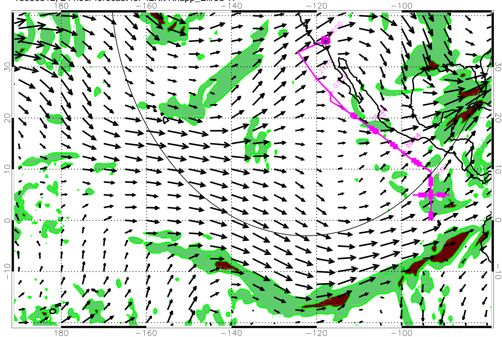
13030312, 24 hour forecast for 42Kft Knapp_Ellrod TI
