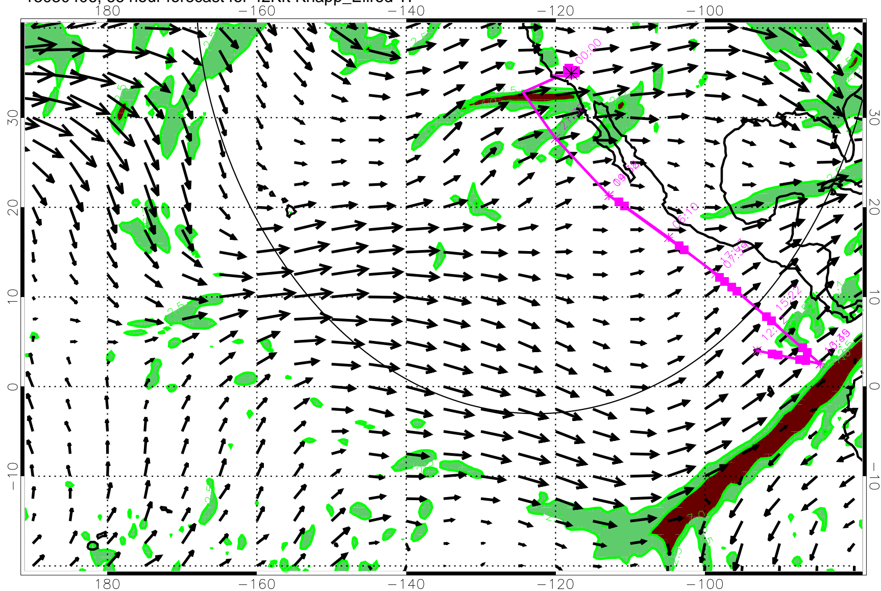
13030406, 66 hour forecast for 42Kft Knapp_Ellrod TI
