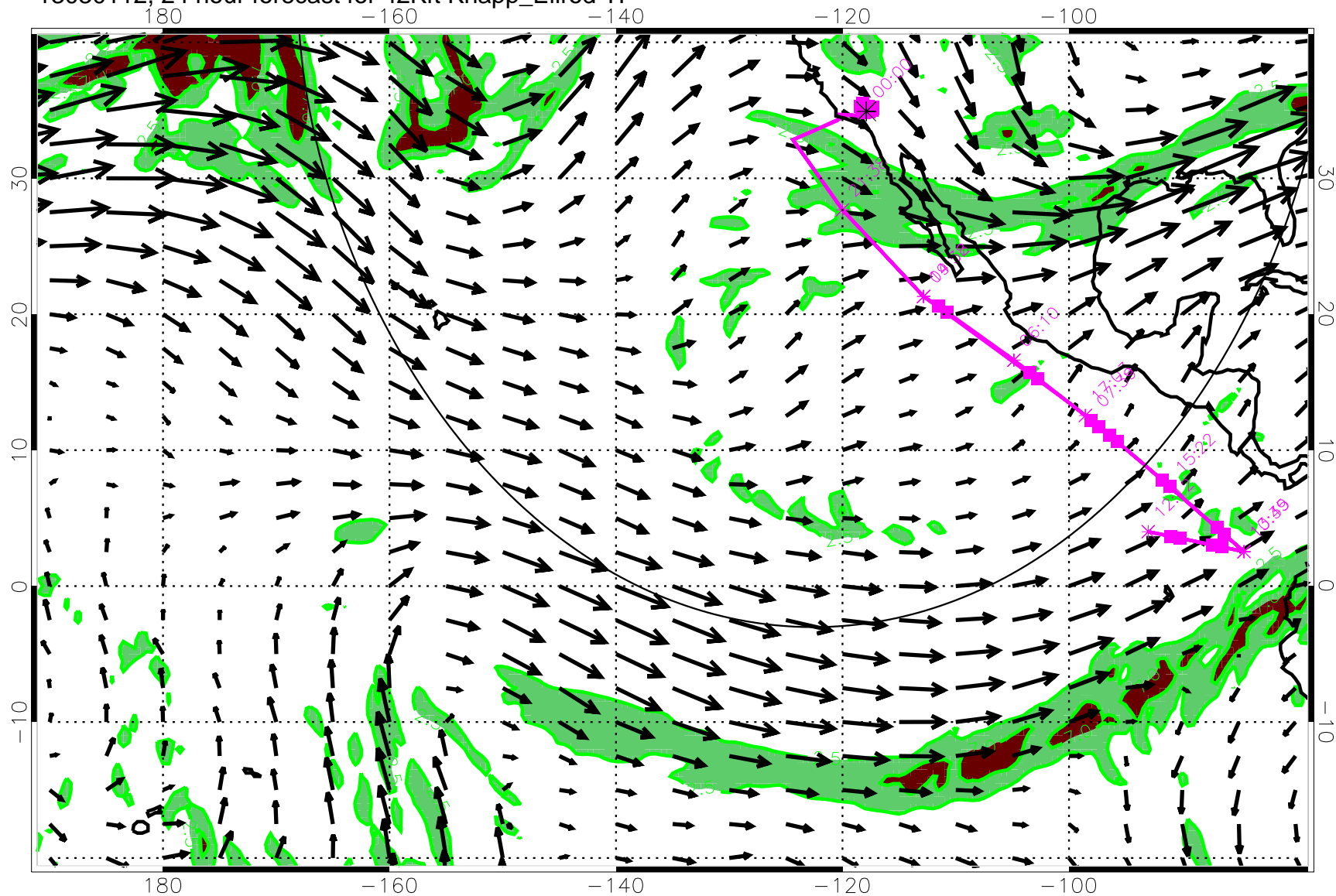
13030112, 24 hour forecast for 42Kft Knapp_Ellrod TI
