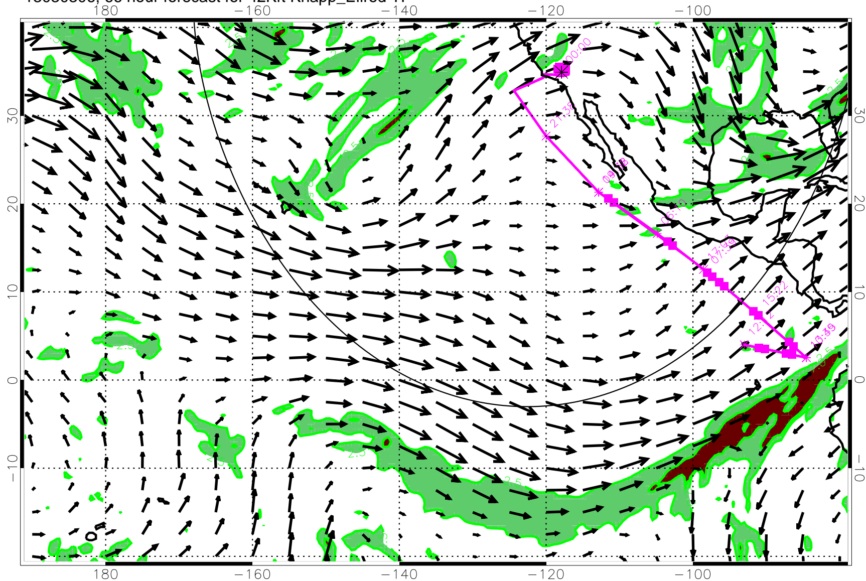
13030306, 66 hour forecast for 42Kft Knapp_Ellrod TI
