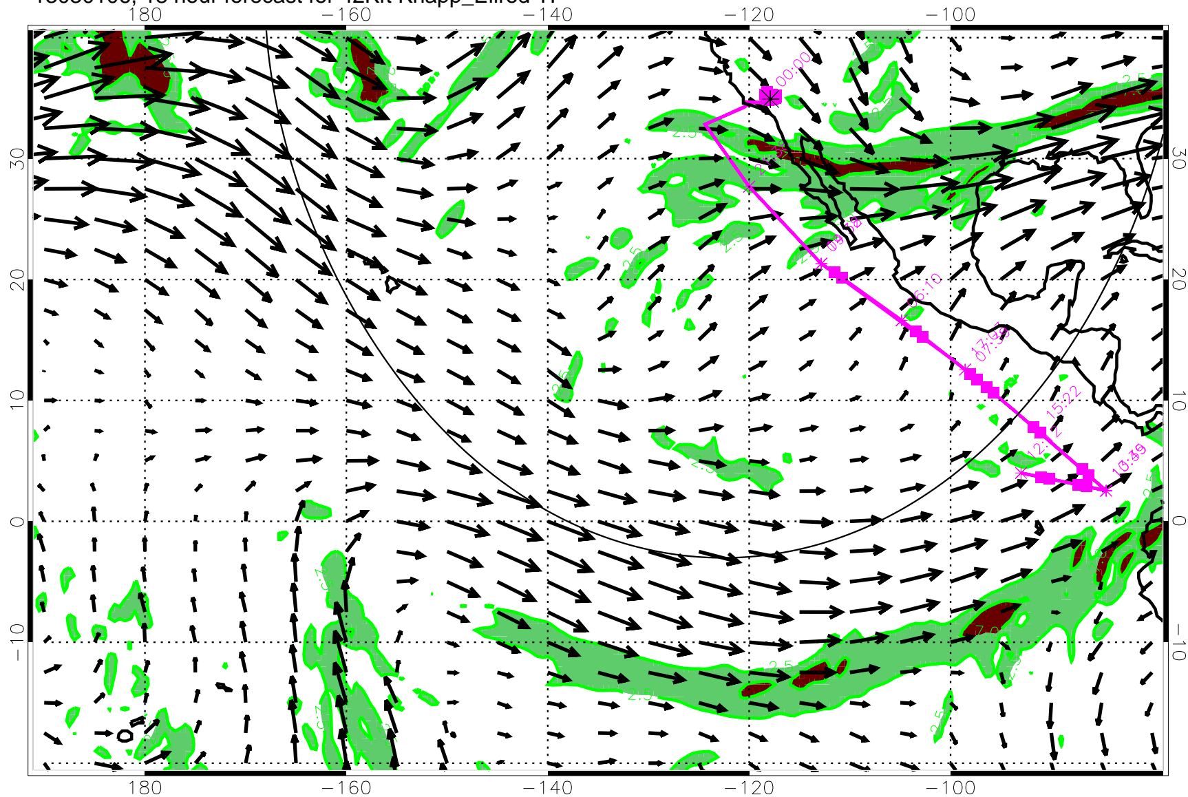
13030106, 18 hour forecast for 42Kft Knapp_Ellrod TI
