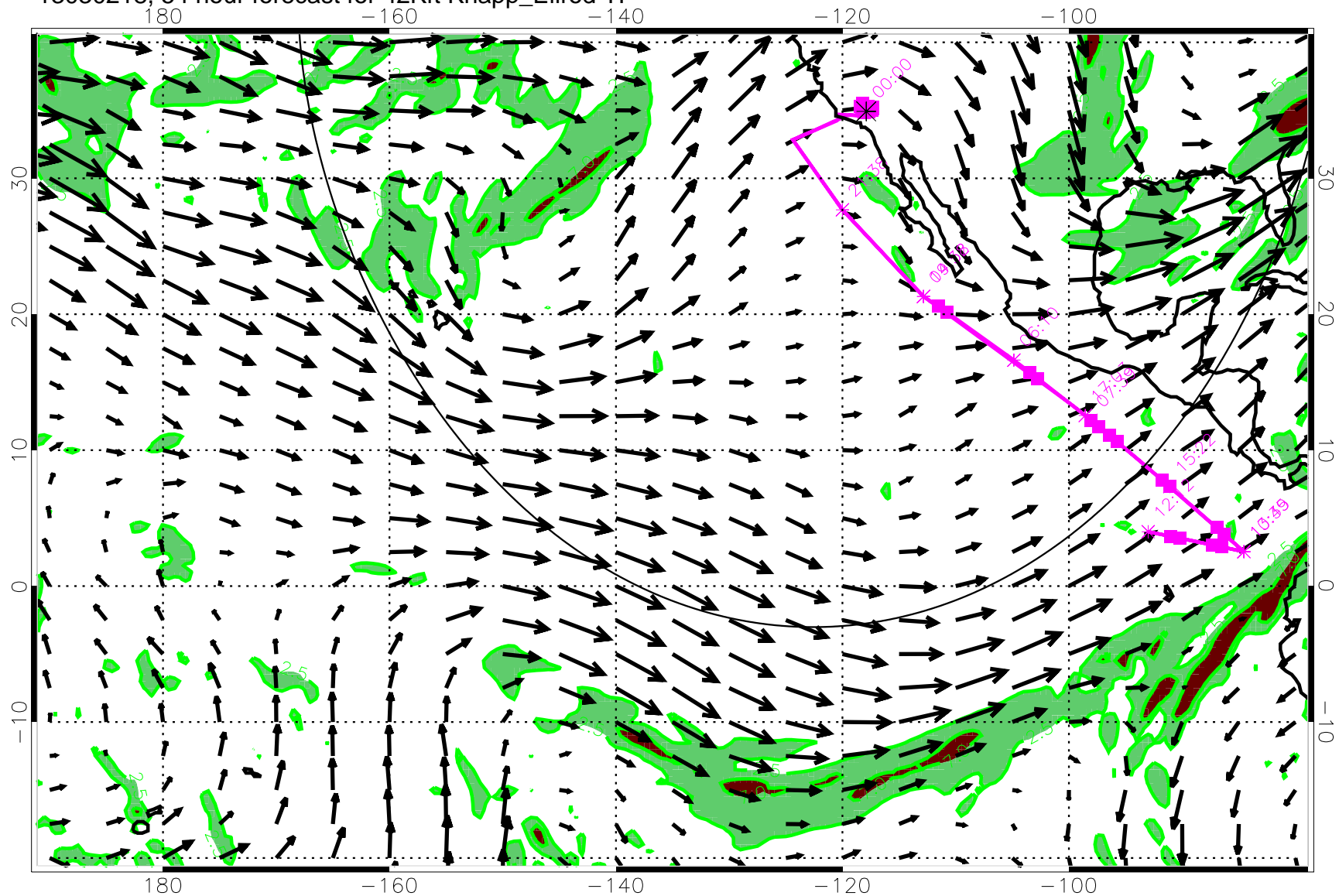
13030218, 54 hour forecast for 42Kft Knapp_Ellrod TI
