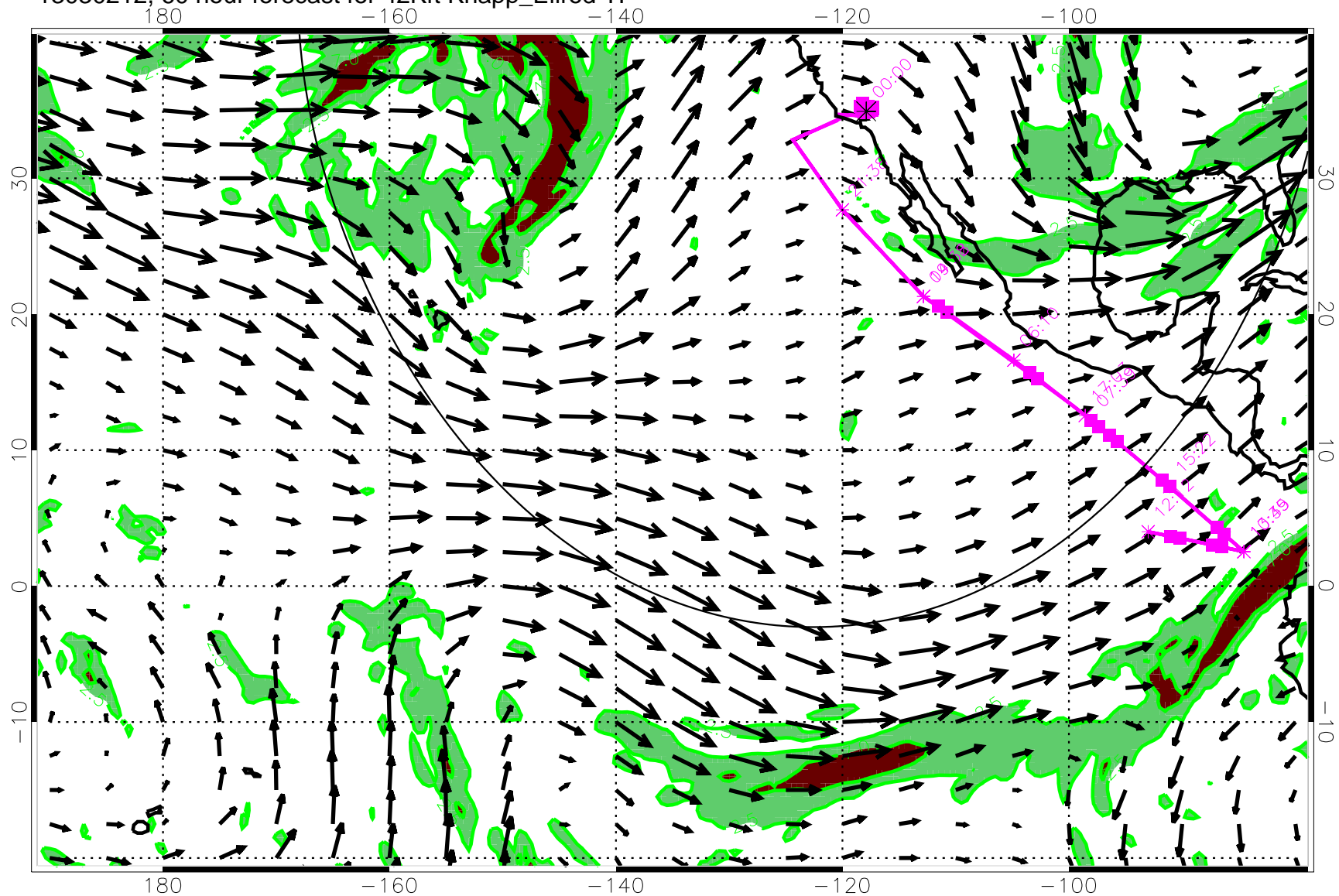
13030212, 60 hour forecast for 42Kft Knapp_Ellrod TI
