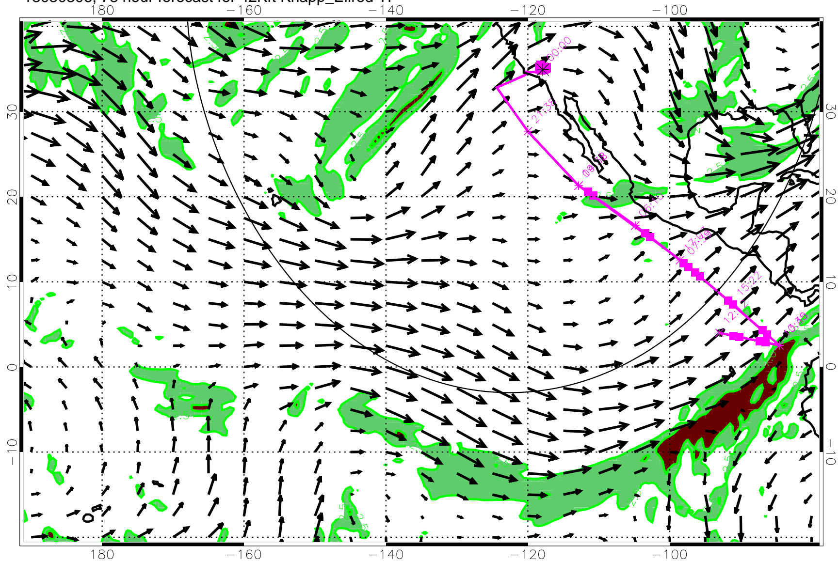
13030306, 78 hour forecast for 42Kft Knapp_Ellrod TI
