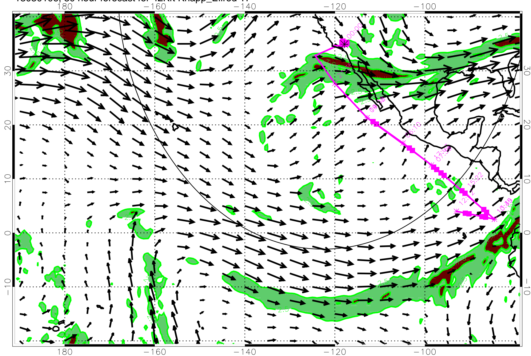
13030106, 30 hour forecast for 42Kft Knapp_Ellrod TI
