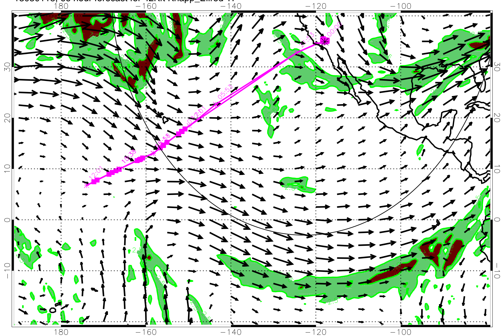
13030118, 66 hour forecast for 42Kft Knapp_Ellrod TI
