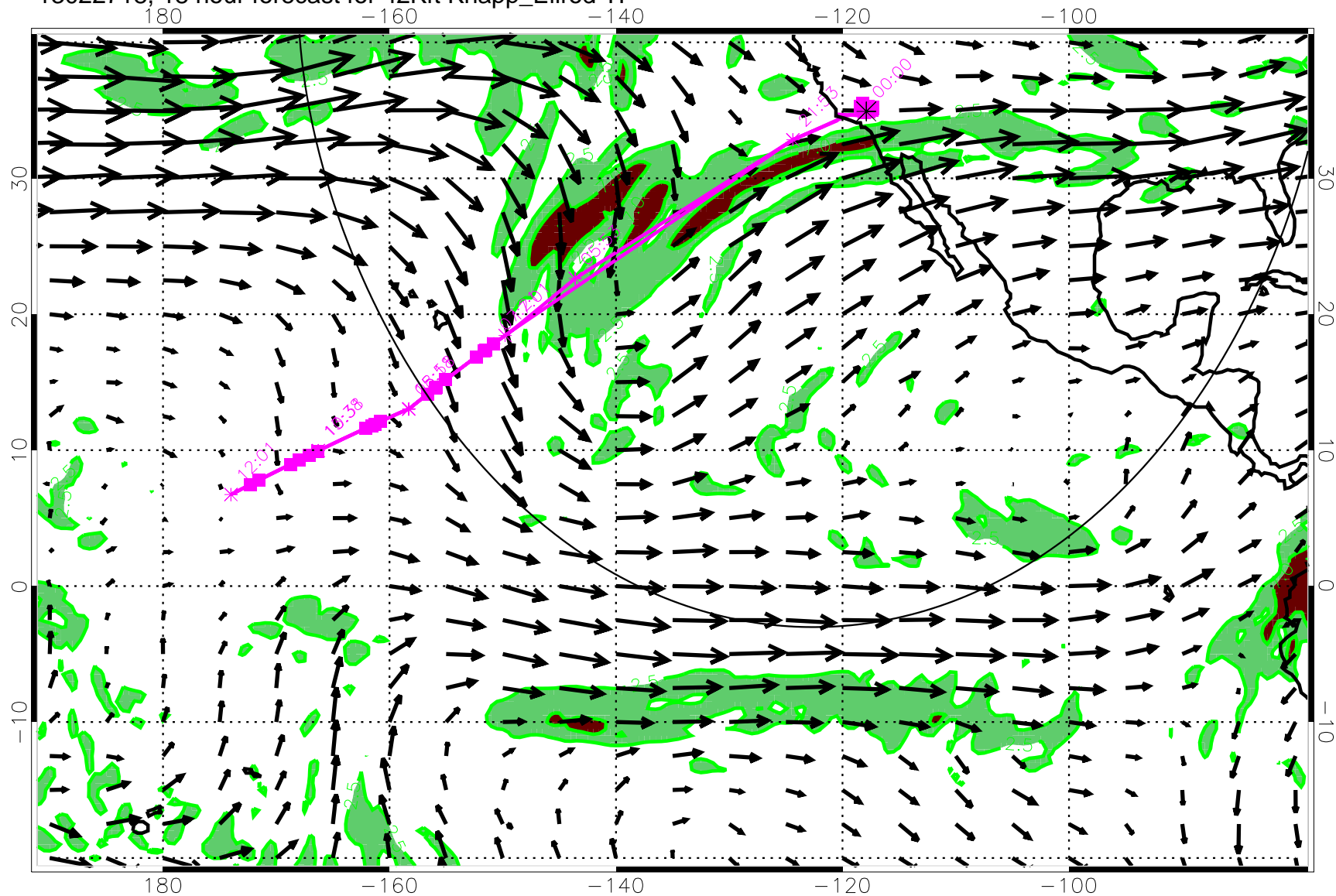
13022718, 18 hour forecast for 42Kft Knapp_Ellrod TI
