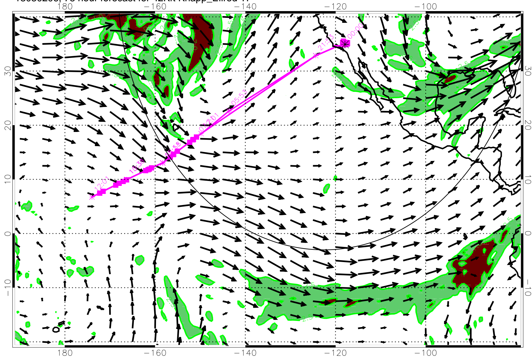
13030206, 78 hour forecast for 42Kft Knapp_Ellrod TI
