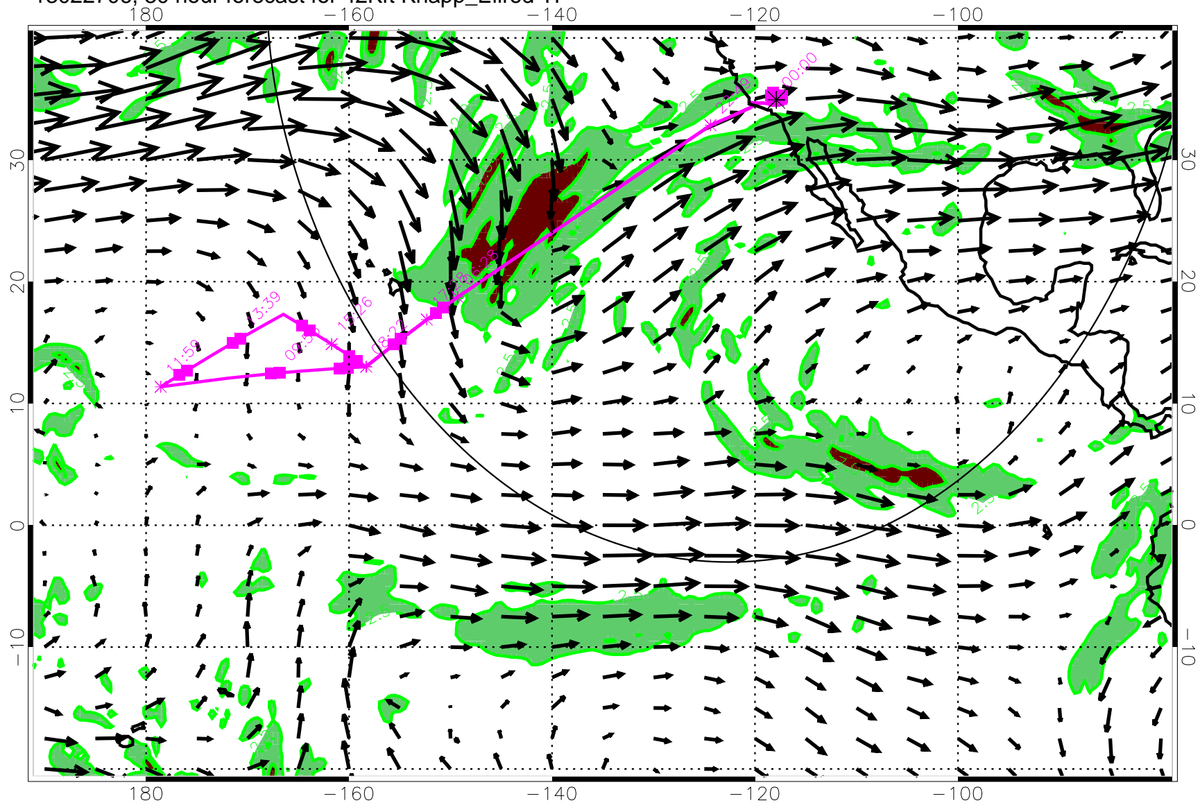
13022706, 30 hour forecast for 42Kft Knapp_Ellrod TI
