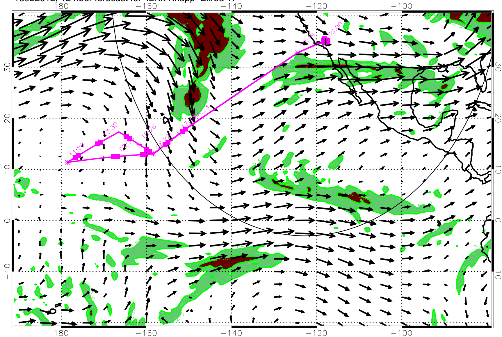
13022612, 12 hour forecast for 42Kft Knapp_Ellrod TI
