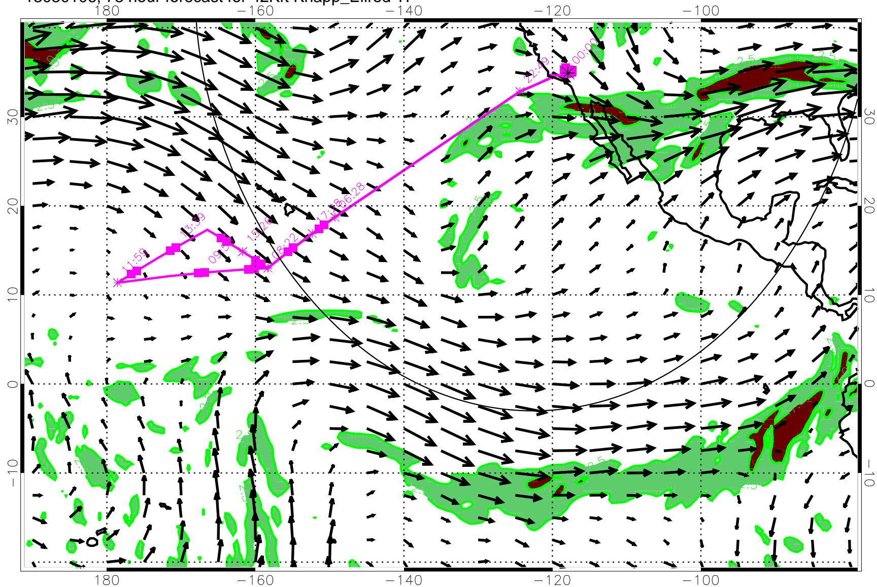
13030106, 78 hour forecast for 42Kft Knapp_Ellrod TI
