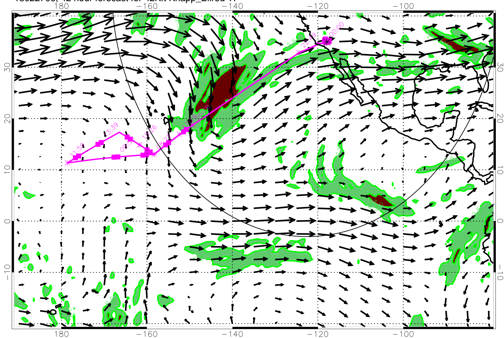
13022706, 42 hour forecast for 42Kft Knapp_Ellrod TI
