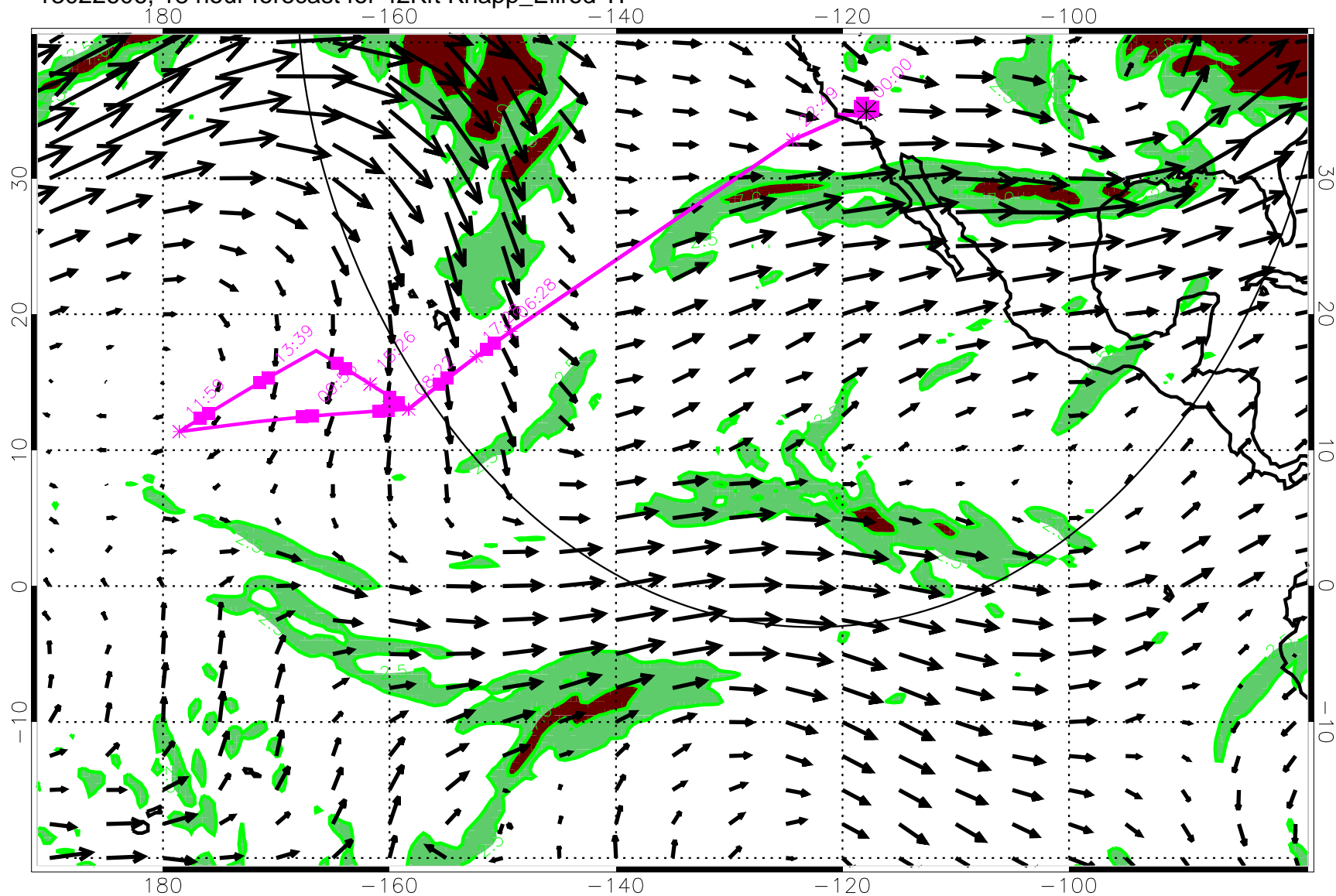
13022606, 18 hour forecast for 42Kft Knapp_Ellrod TI
