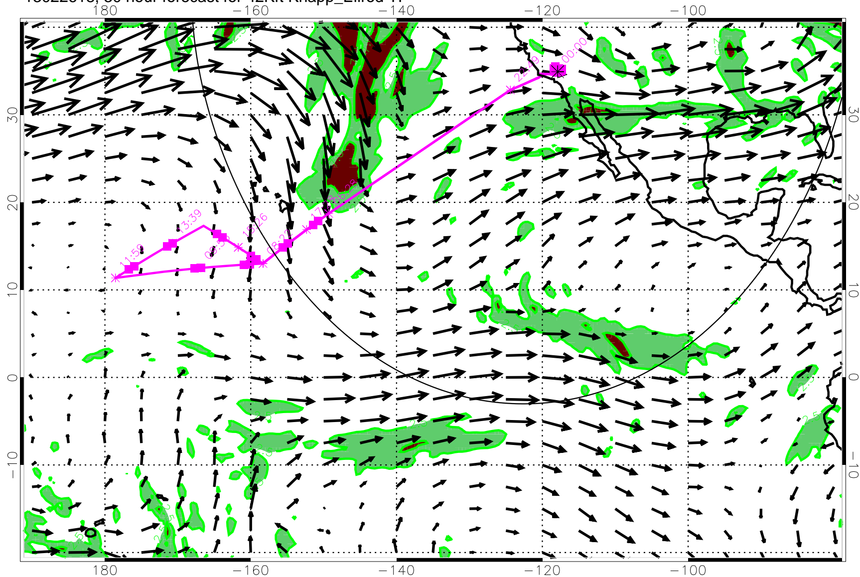
13022618, 30 hour forecast for 42Kft Knapp_Ellrod TI
