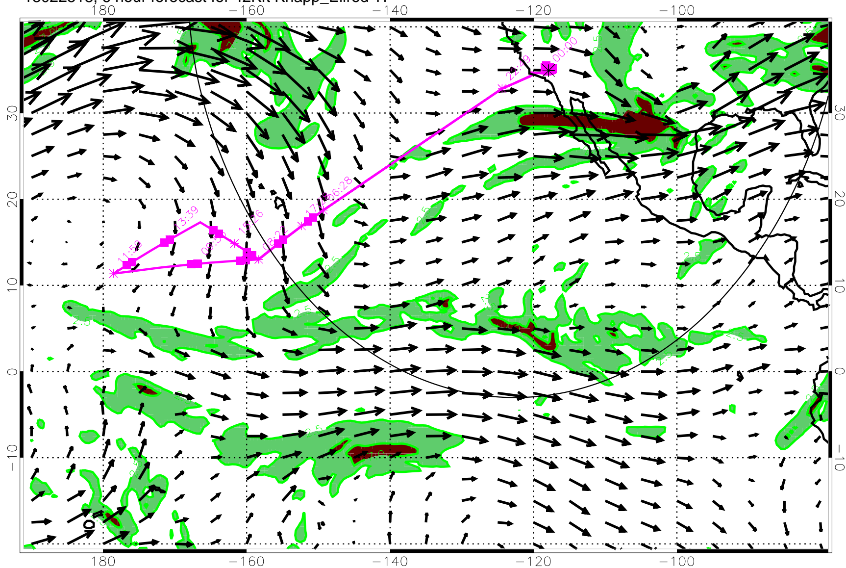
13022518, 6 hour forecast for 42Kft Knapp_Ellrod TI
