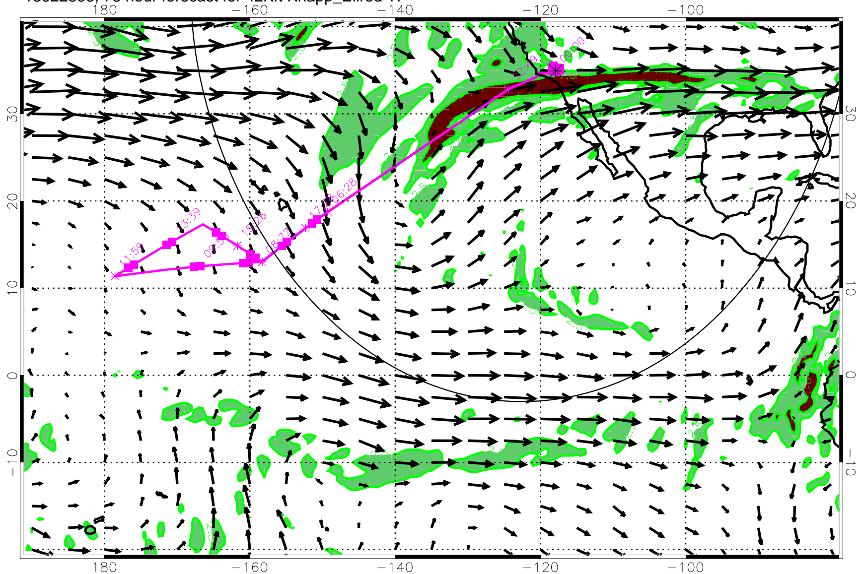
13022806, 78 hour forecast for 42Kft Knapp_Ellrod TI
