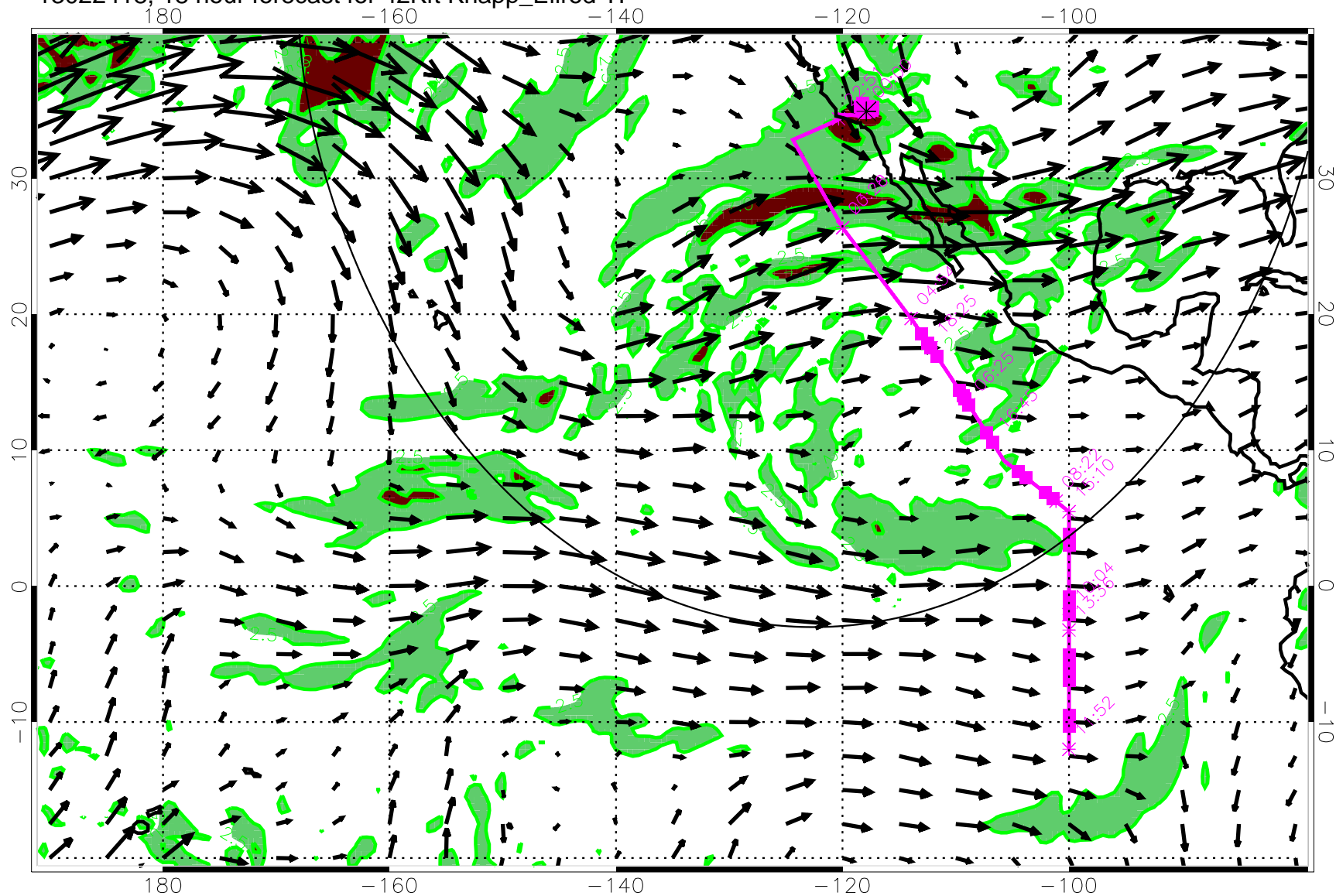
13022418, 18 hour forecast for 42Kft Knapp_Ellrod TI
