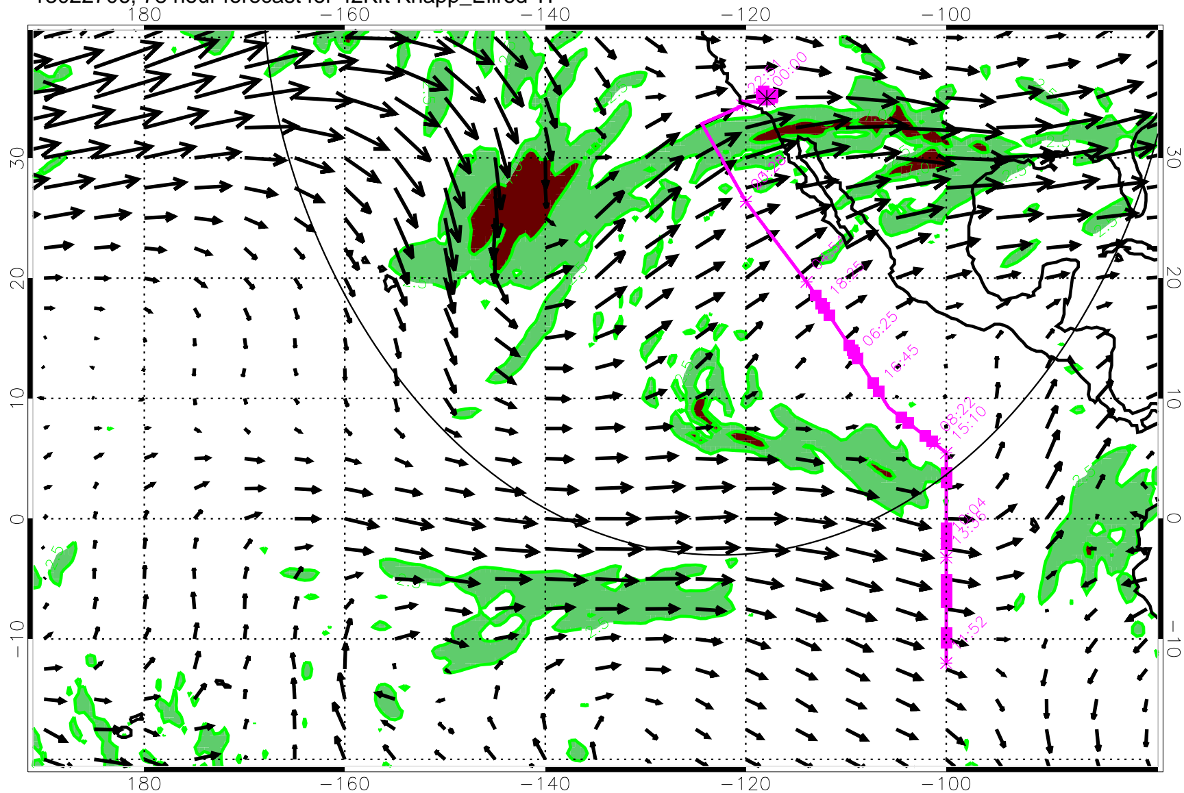
13022706, 78 hour forecast for 42Kft Knapp_Ellrod TI
