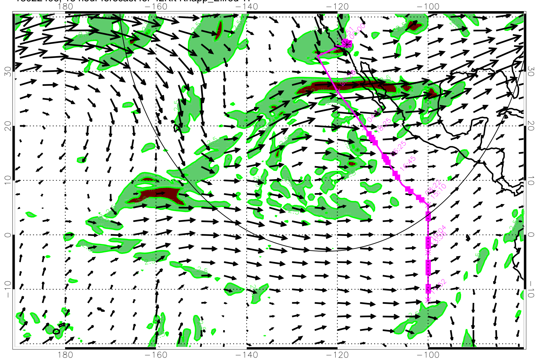
13022406, 18 hour forecast for 42Kft Knapp_Ellrod TI
