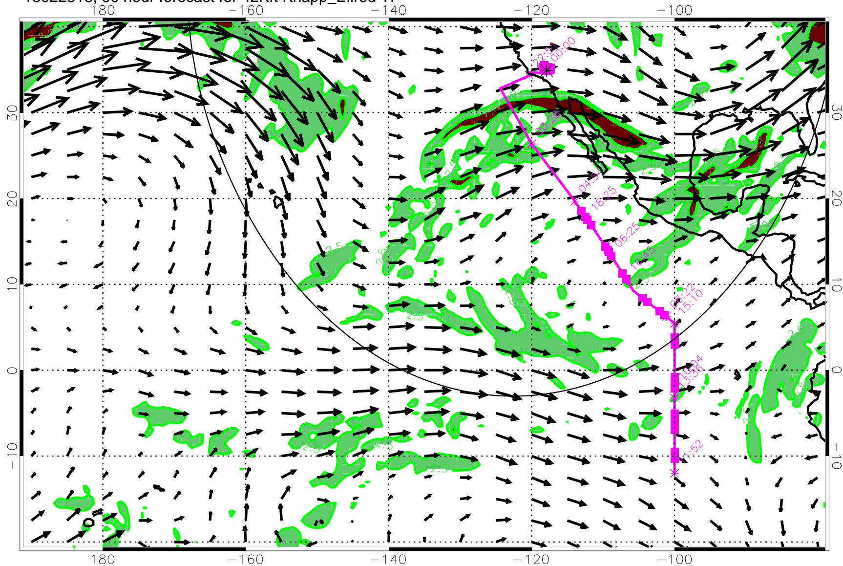
13022518, 90 hour forecast for 42Kft Knapp_Ellrod TI
