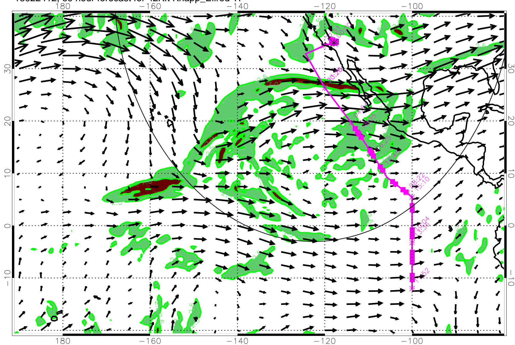
13022412, 60 hour forecast for 42Kft Knapp_Ellrod TI
