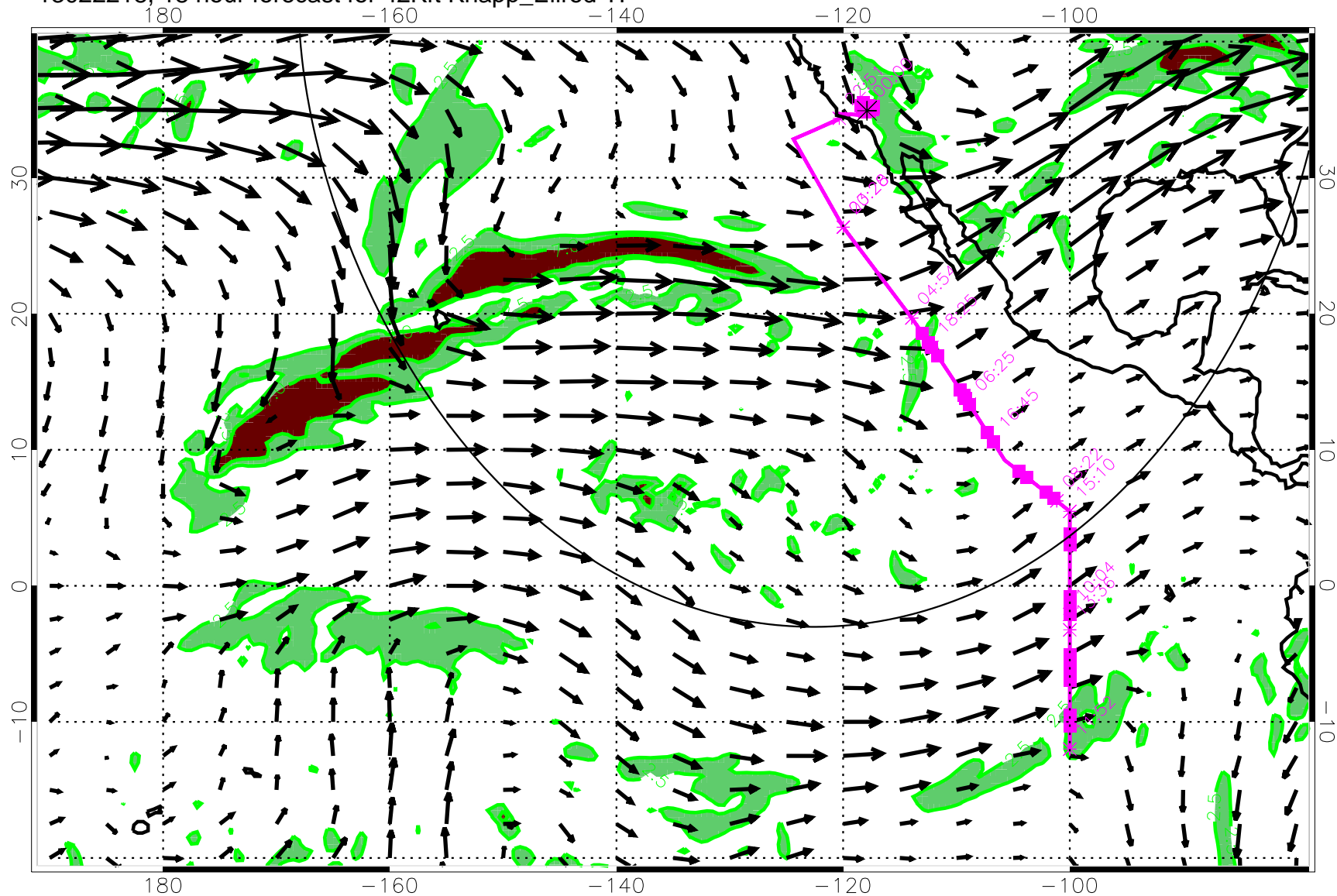
13022218, 18 hour forecast for 42Kft Knapp_Ellrod TI
