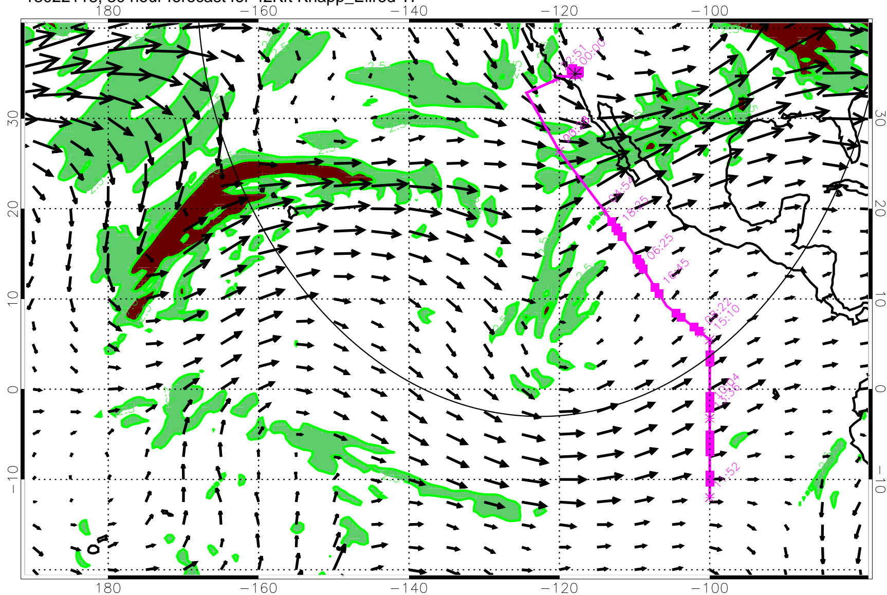
13022118, 30 hour forecast for 42Kft Knapp_Ellrod TI
