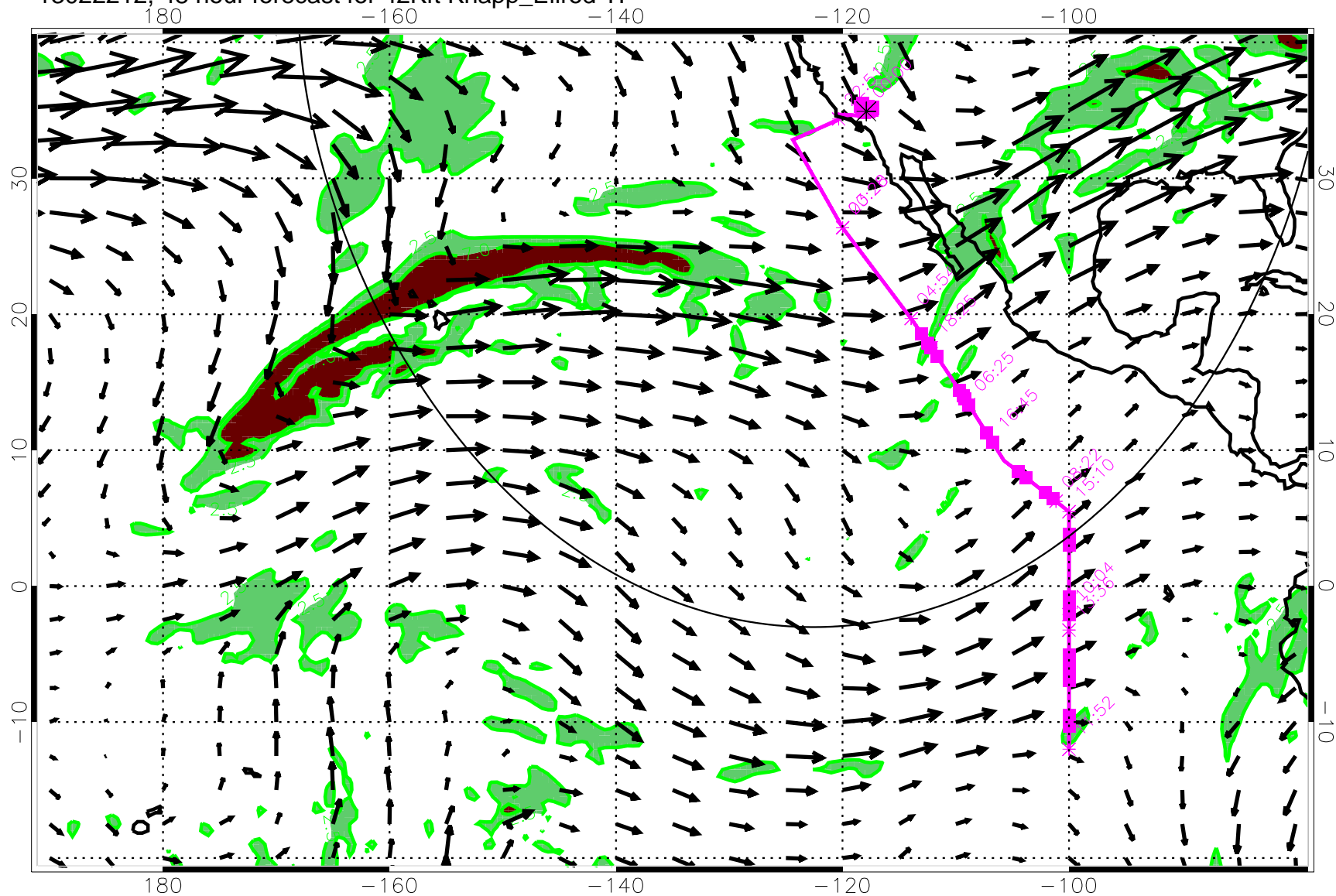
13022212, 48 hour forecast for 42Kft Knapp_Ellrod TI
