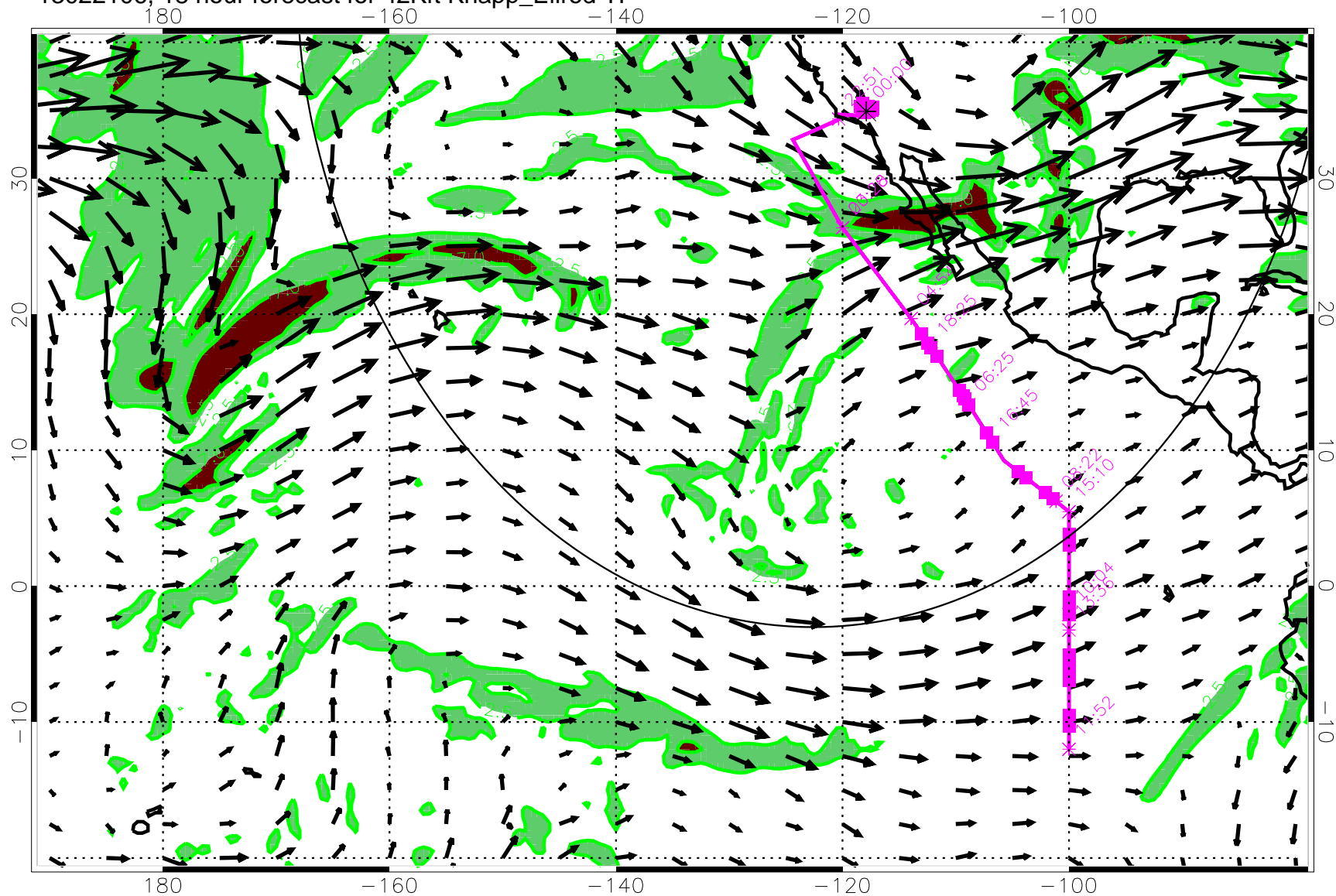
13022106, 18 hour forecast for 42Kft Knapp_Ellrod TI
