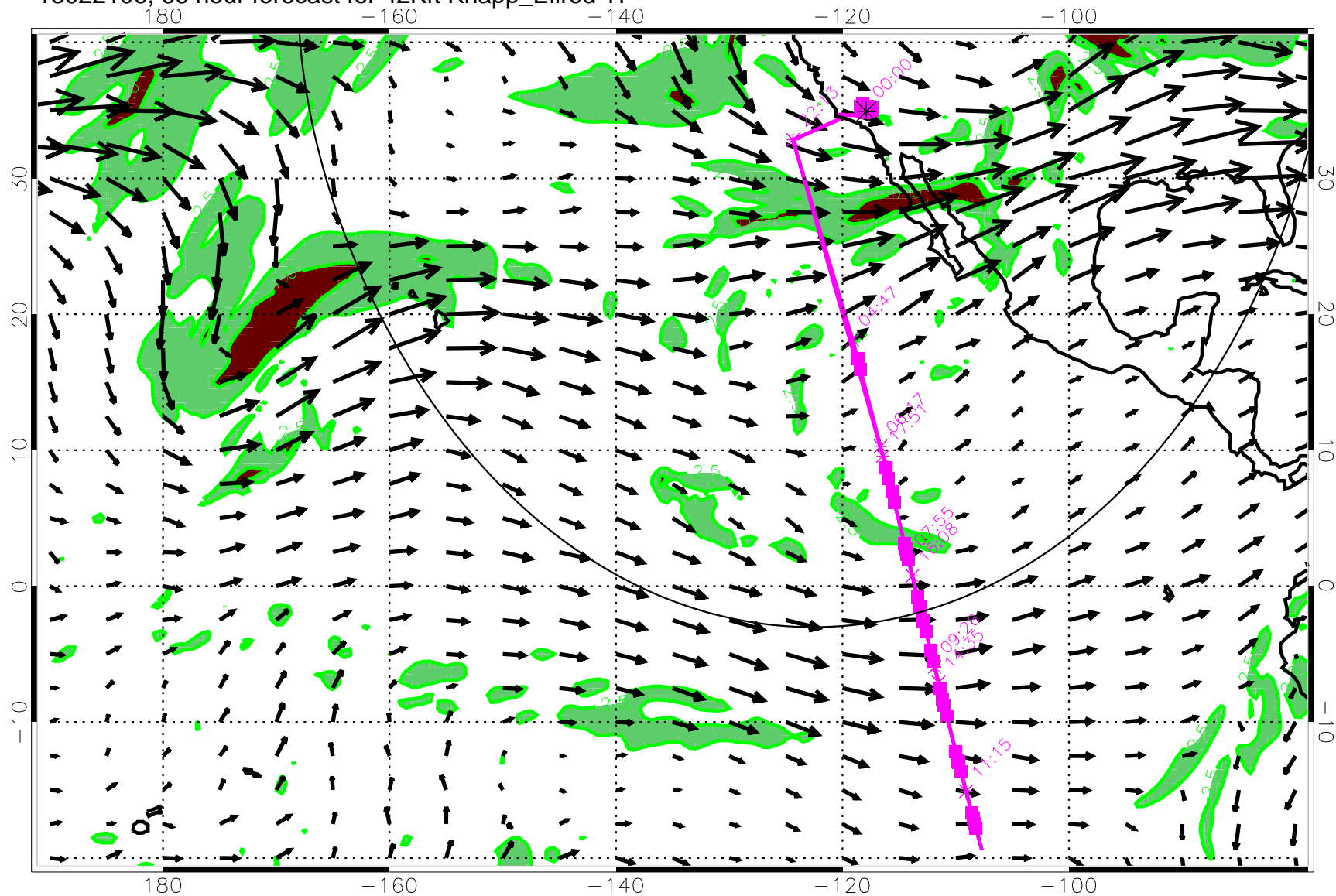
13022106, 66 hour forecast for 42Kft Knapp_Ellrod TI
