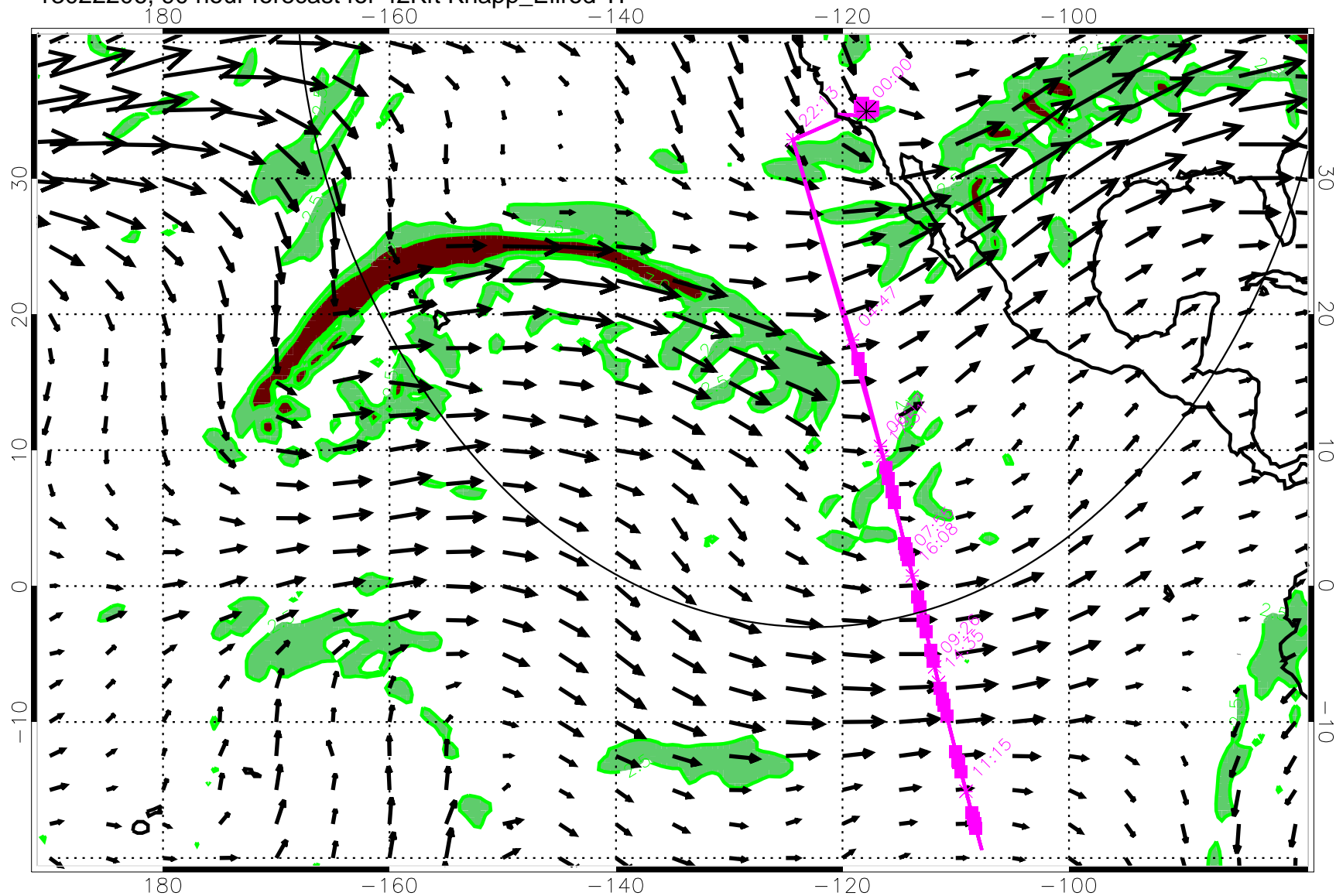
13022206, 90 hour forecast for 42Kft Knapp_Ellrod TI
