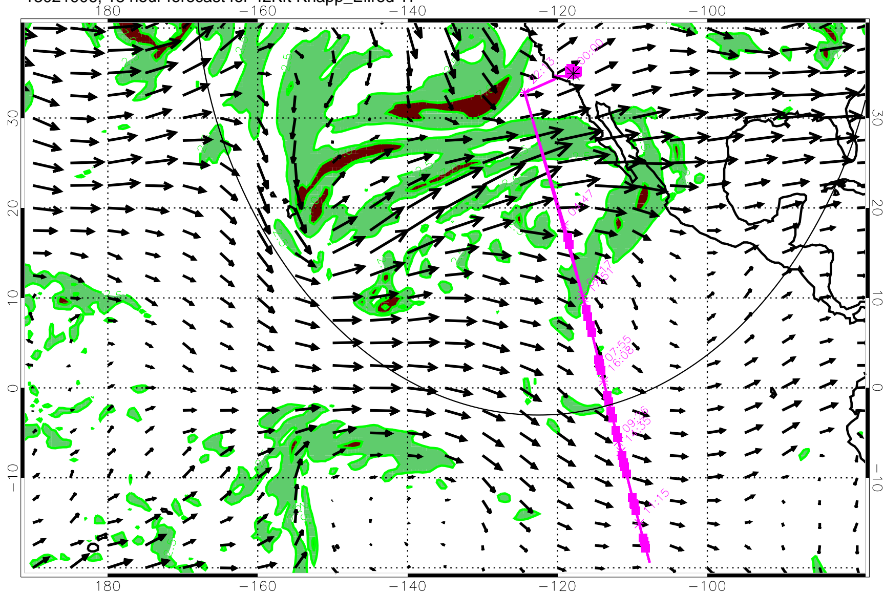
13021906, 18 hour forecast for 42Kft Knapp_Ellrod TI
