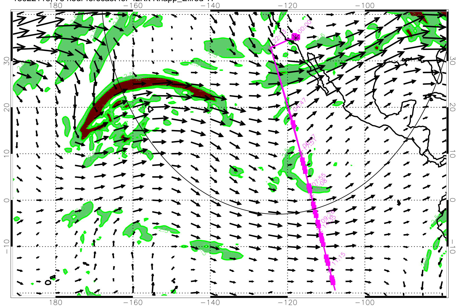
13022118, 78 hour forecast for 42Kft Knapp_Ellrod TI
