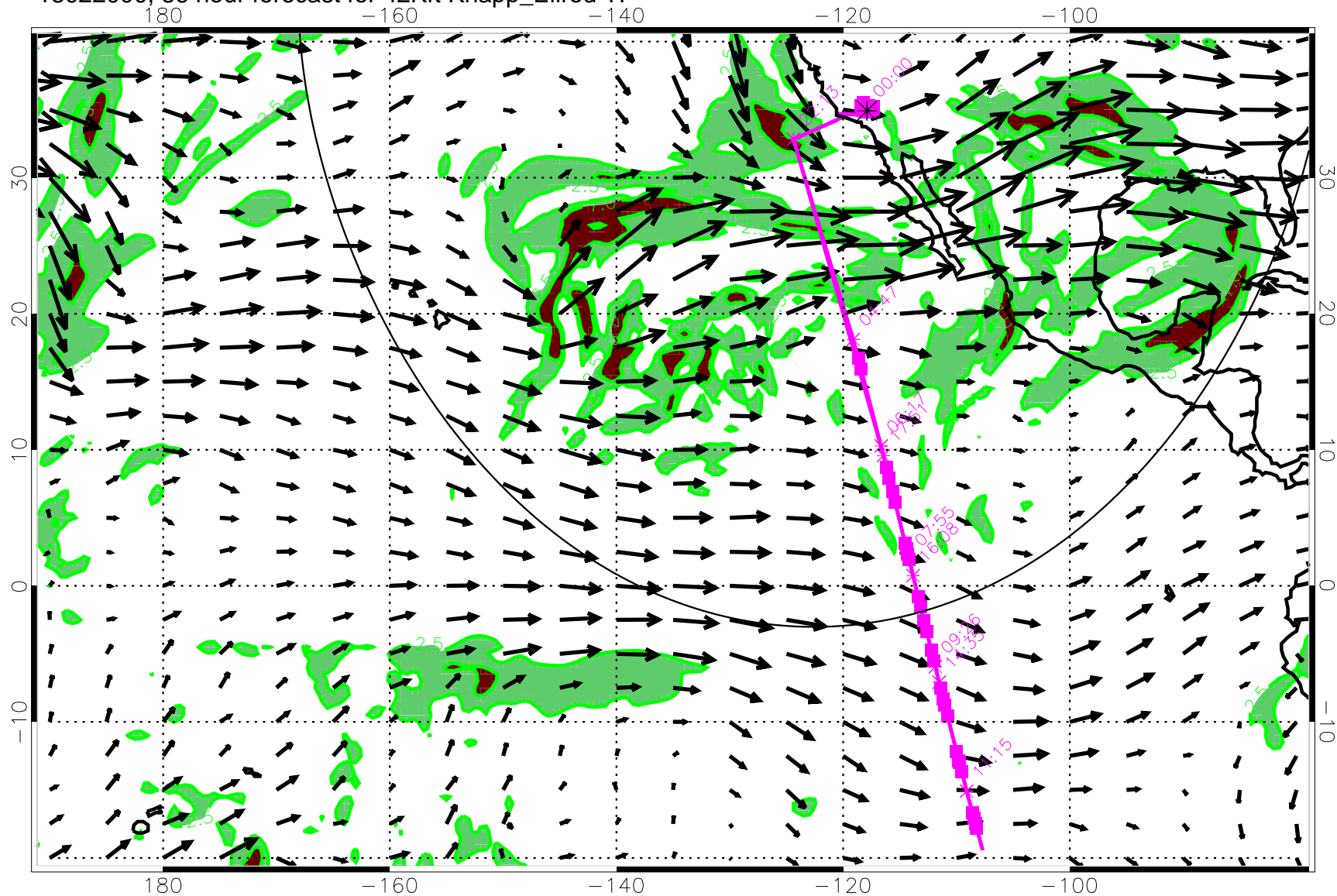
13022000, 36 hour forecast for 42Kft Knapp_Ellrod TI
