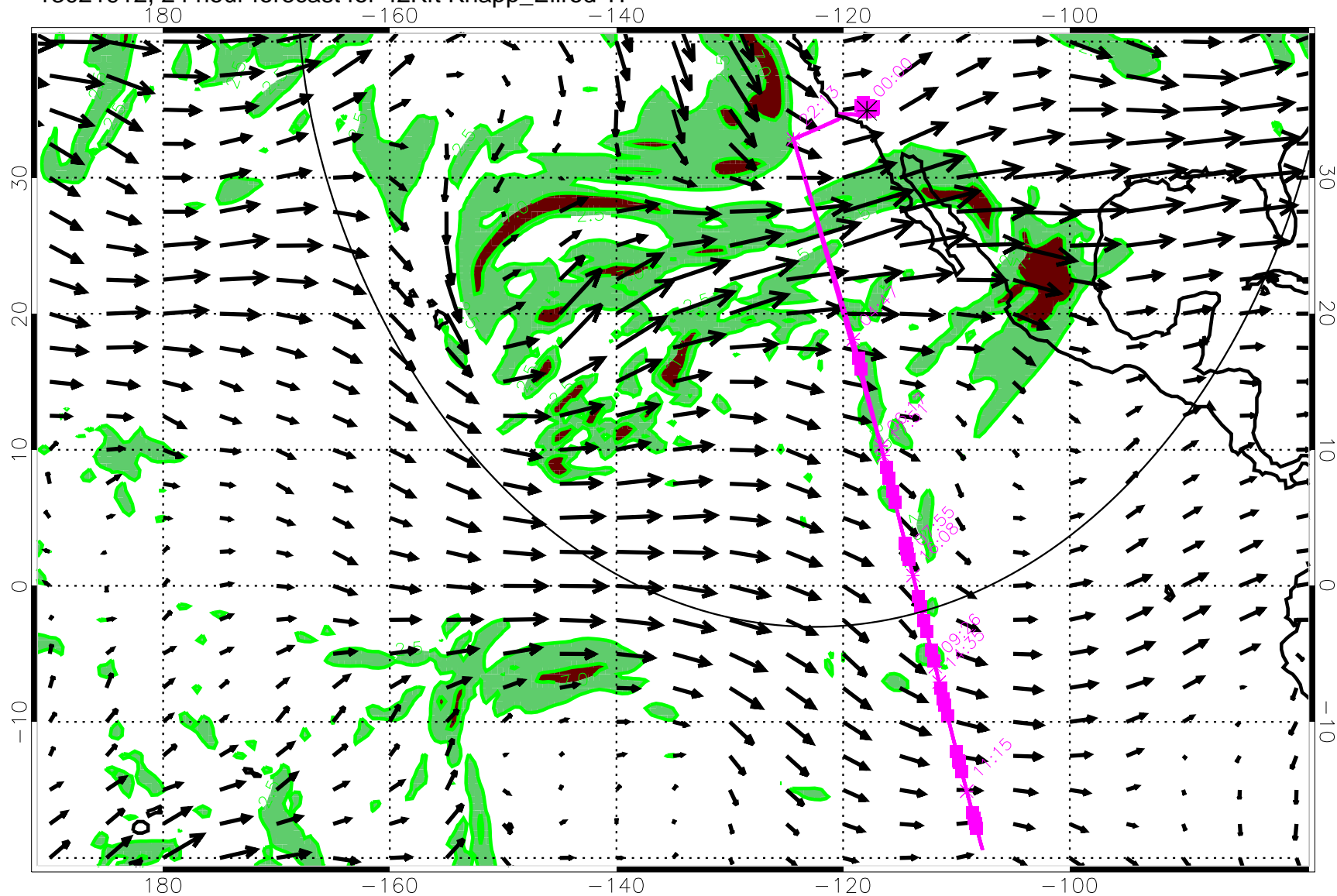
13021912, 24 hour forecast for 42Kft Knapp_Ellrod TI
