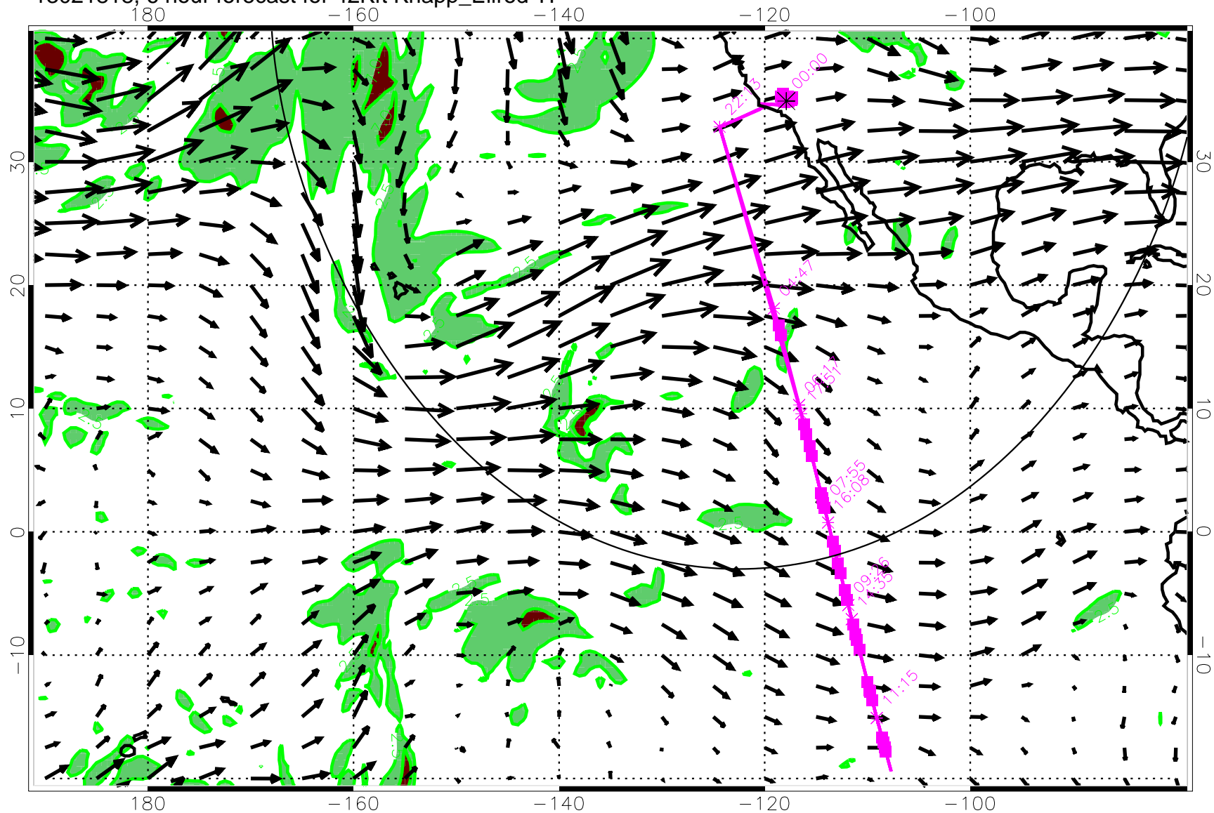
13021818, 6 hour forecast for 42Kft Knapp_Ellrod TI
