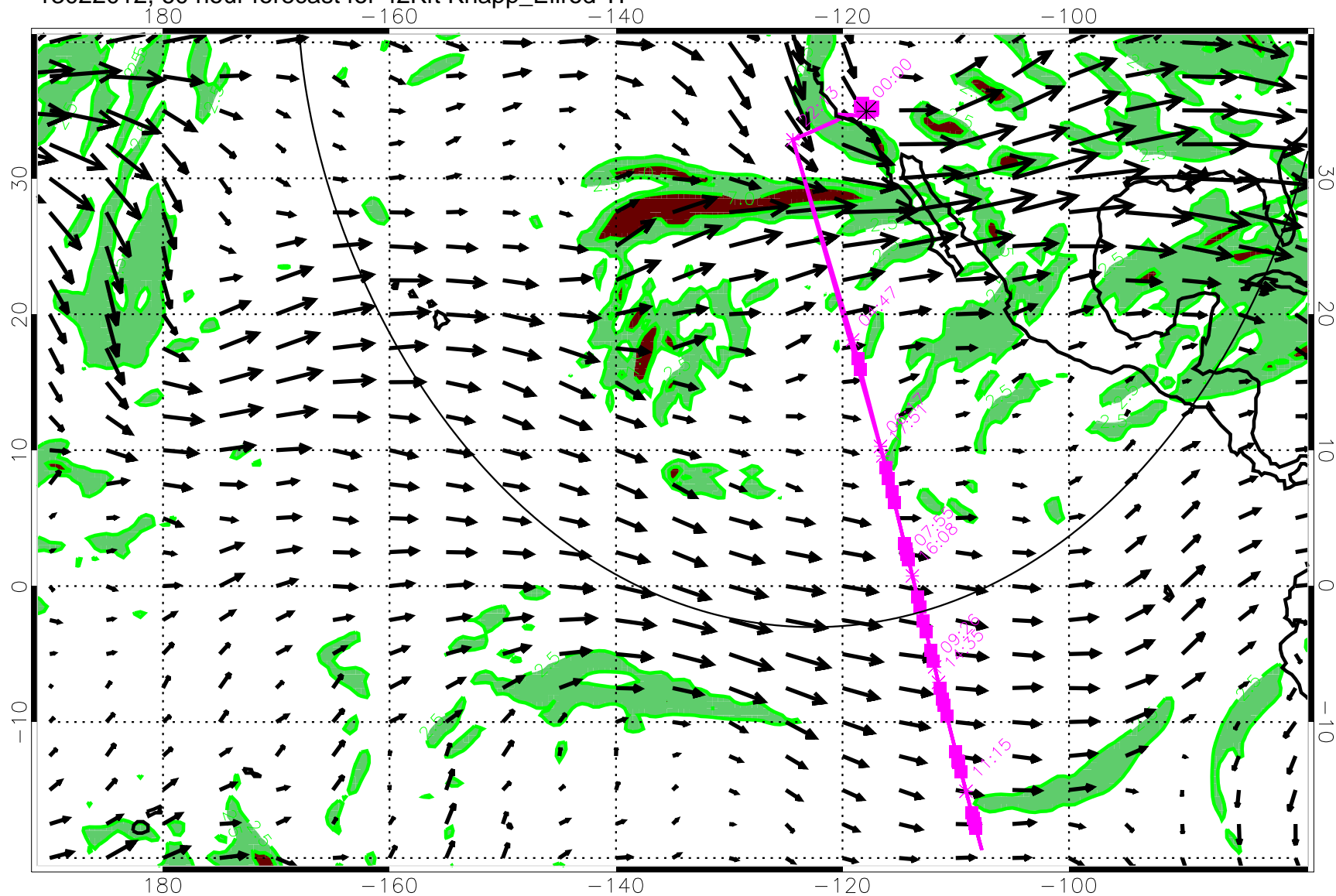
13022012, 60 hour forecast for 42Kft Knapp_Ellrod TI
