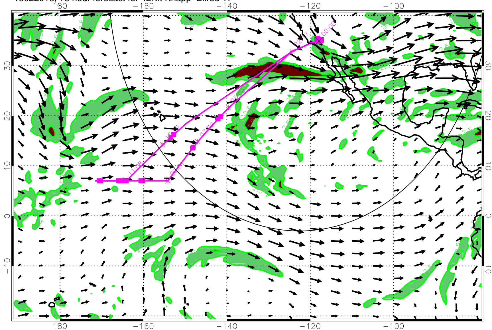
13022018, 78 hour forecast for 42Kft Knapp_Ellrod TI
