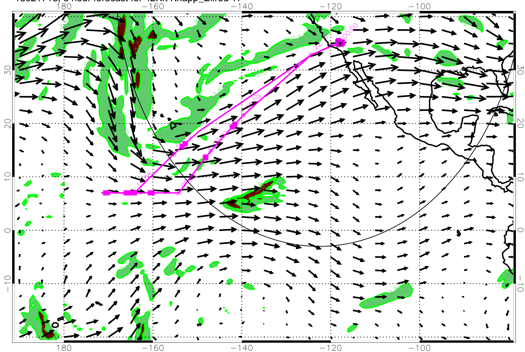
13021718, 6 hour forecast for 42Kft Knapp_Ellrod TI
