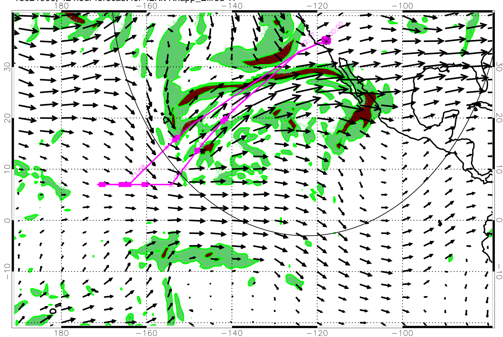
13021906, 42 hour forecast for 42Kft Knapp_Ellrod TI
