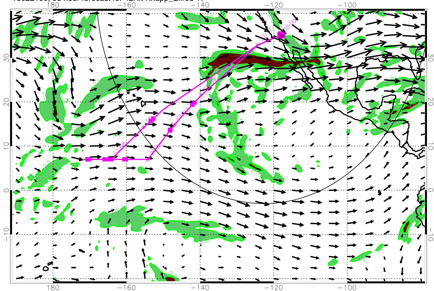
13022100, 96 hour forecast for 42Kft Knapp_Ellrod TI
