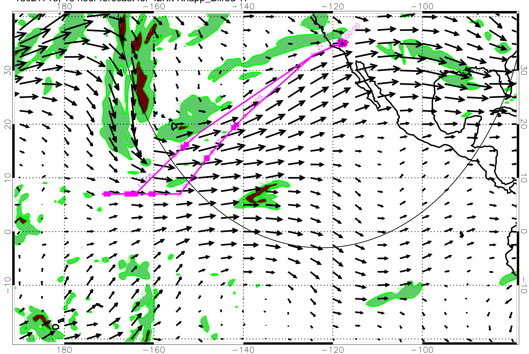
13021718, 18 hour forecast for 42Kft Knapp_Ellrod TI
