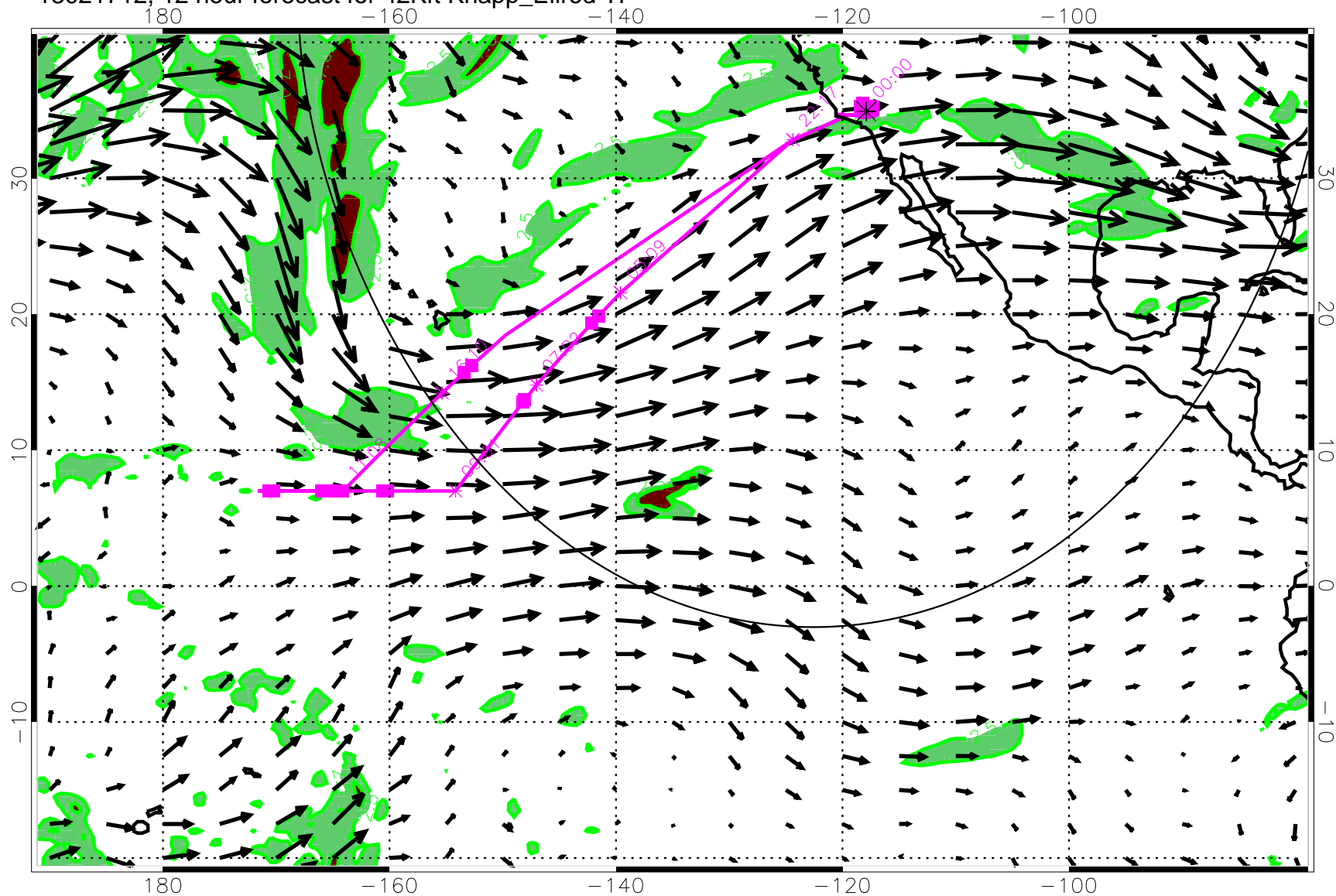
13021712, 12 hour forecast for 42Kft Knapp_Ellrod TI
