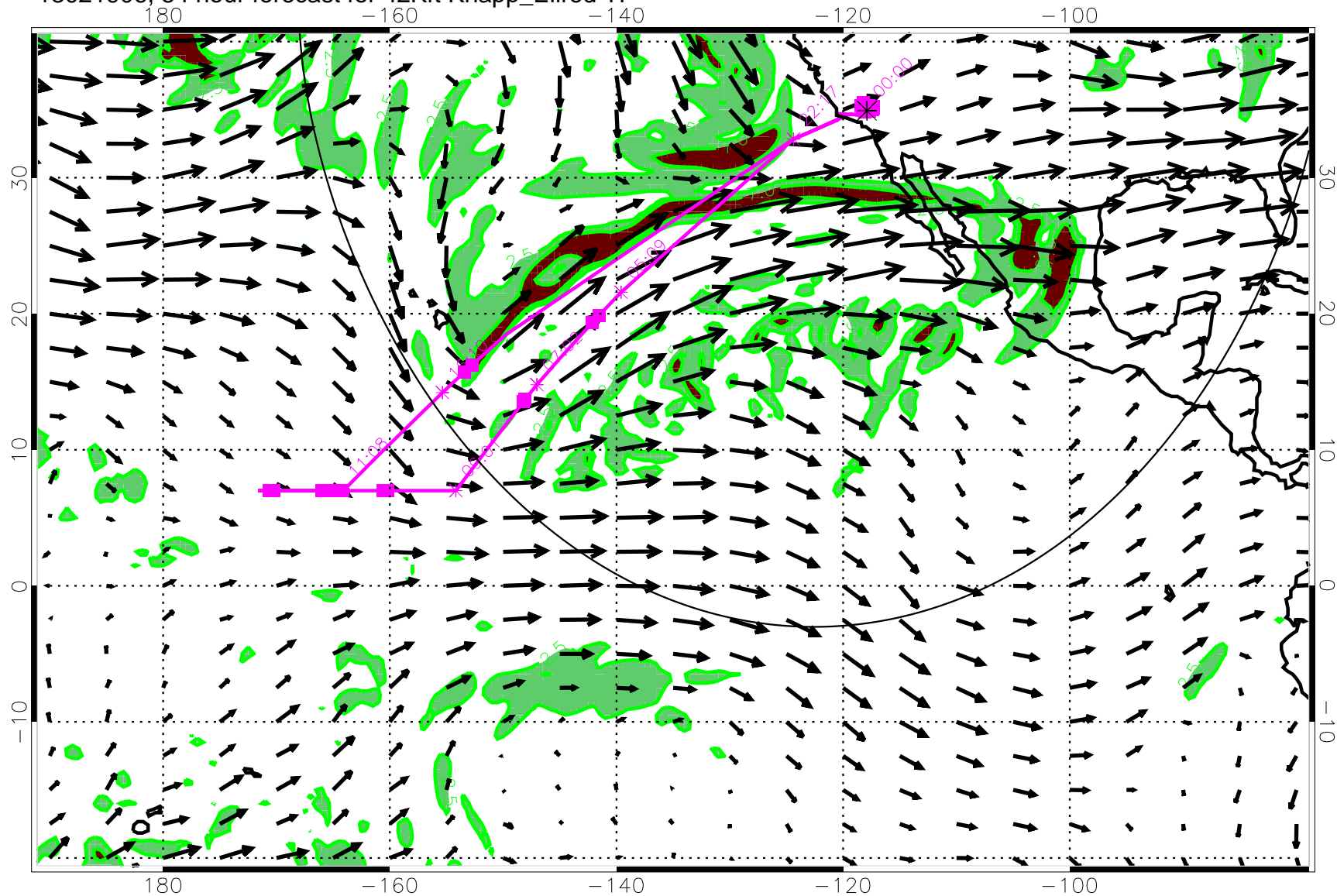
13021906, 54 hour forecast for 42Kft Knapp_Ellrod TI
