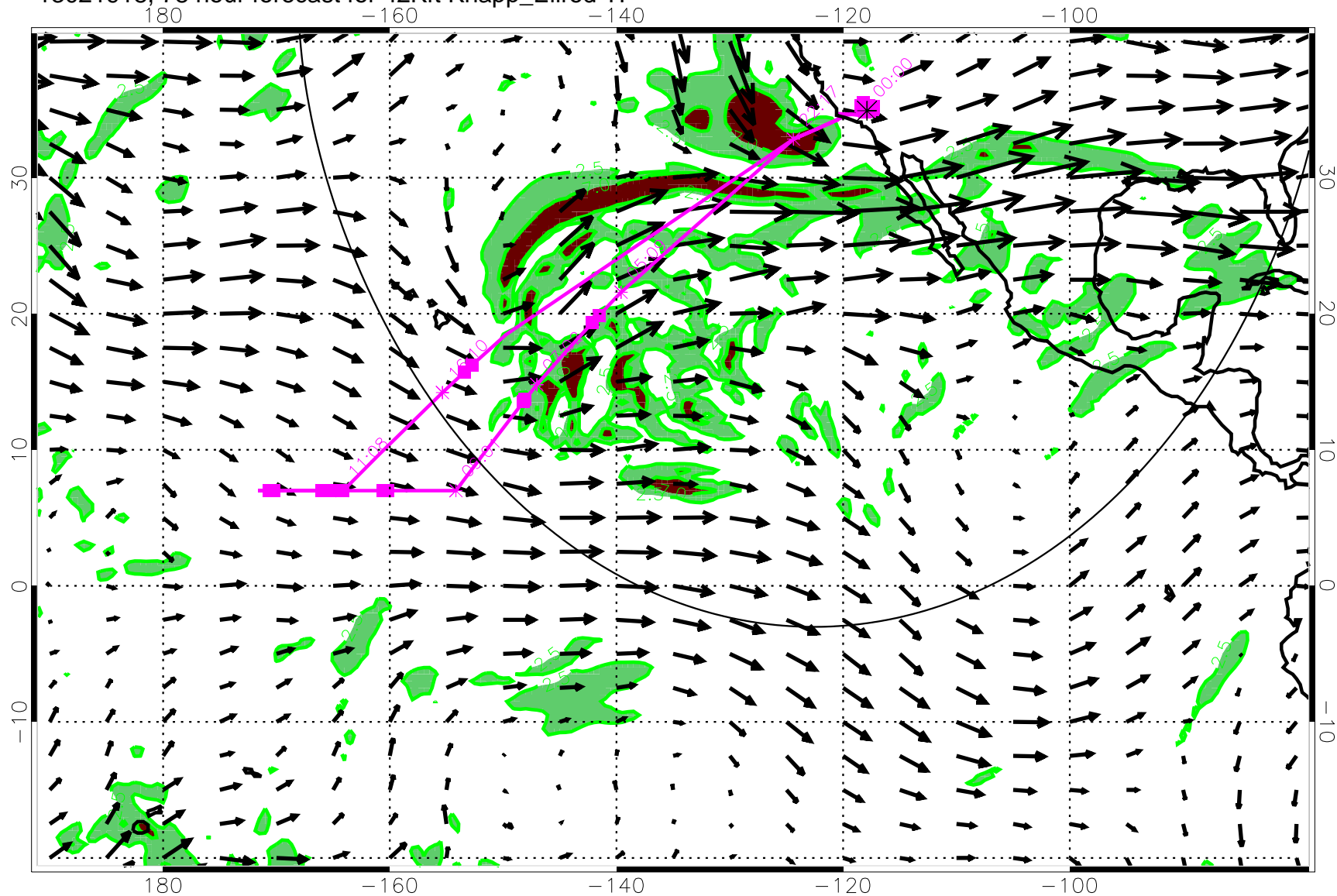
13021918, 78 hour forecast for 42Kft Knapp_Ellrod TI
