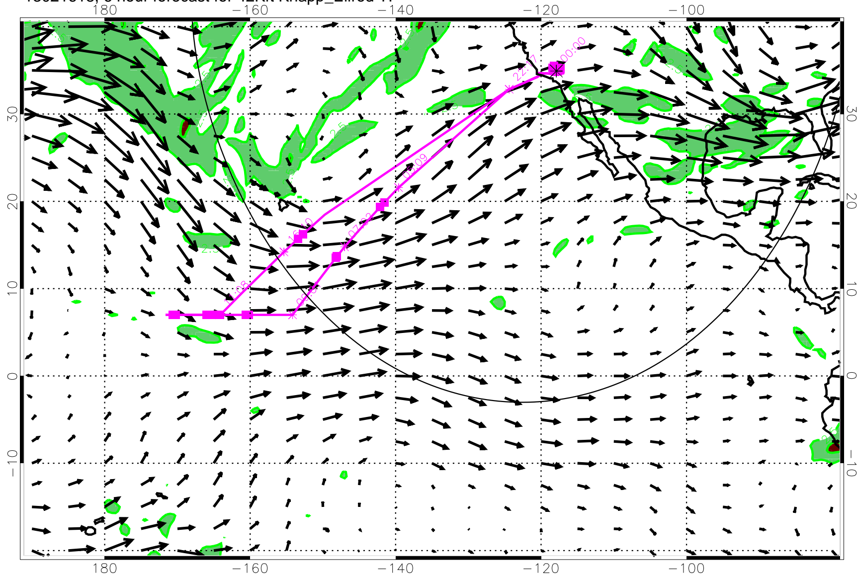
13021618, 6 hour forecast for 42Kft Knapp_Ellrod TI
