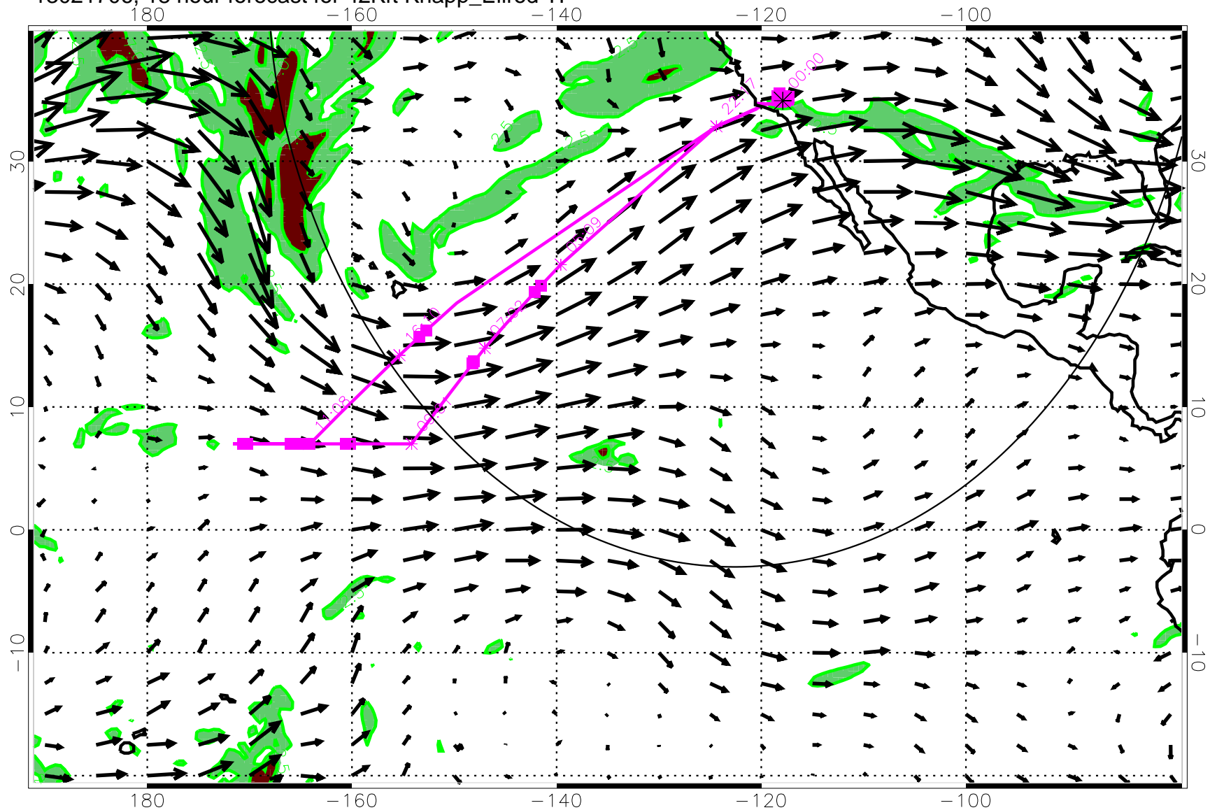
13021706, 18 hour forecast for 42Kft Knapp_Ellrod TI
