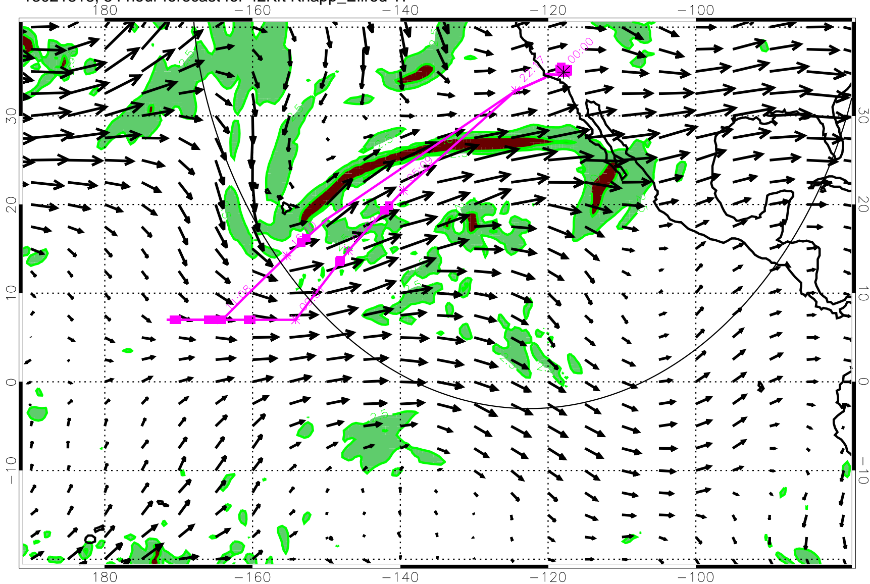
13021818, 54 hour forecast for 42Kft Knapp_Ellrod TI
