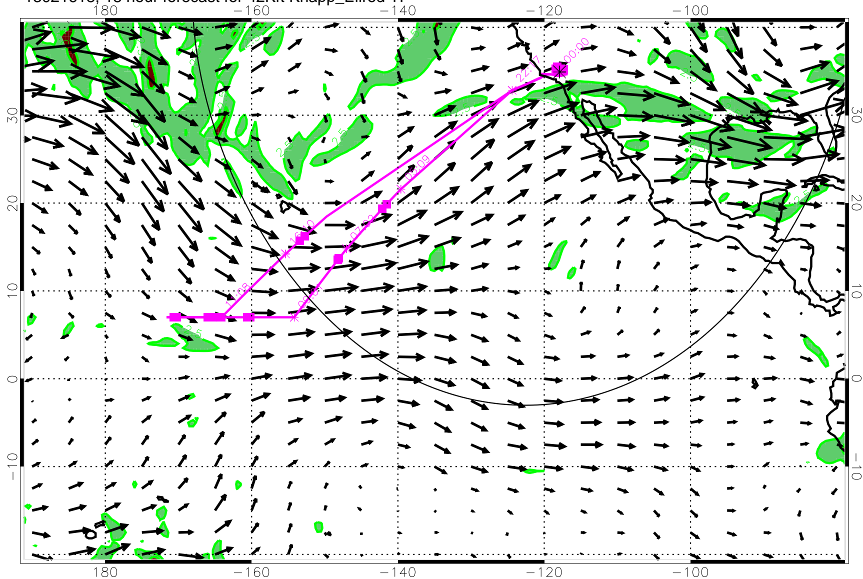
13021618, 18 hour forecast for 42Kft Knapp_Ellrod TI
