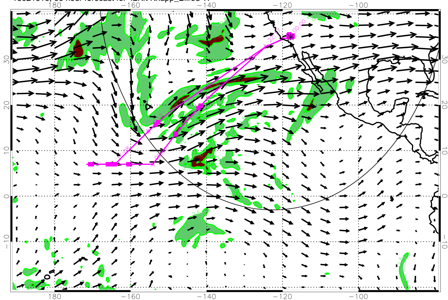
13021818, 66 hour forecast for 42Kft Knapp_Ellrod TI
