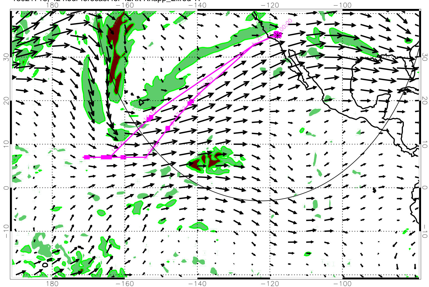
13021718, 42 hour forecast for 42Kft Knapp_Ellrod TI
