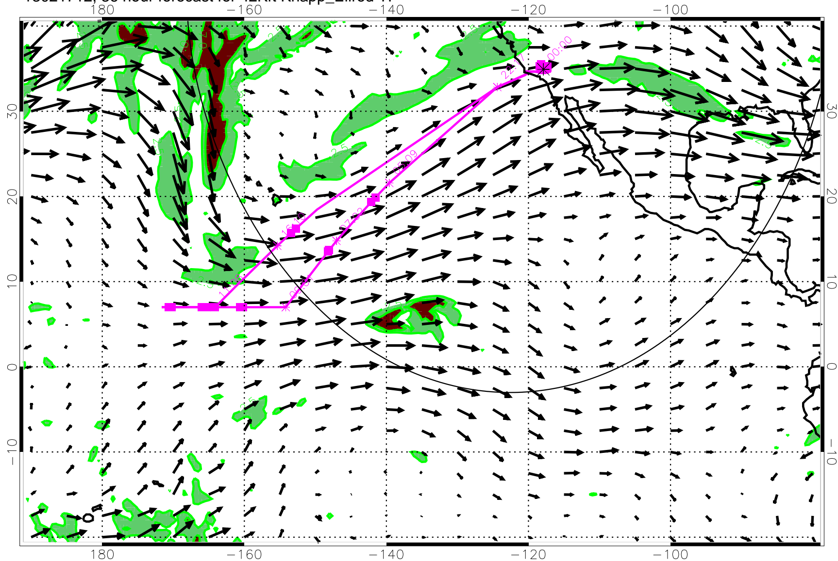
13021712, 36 hour forecast for 42Kft Knapp_Ellrod TI
