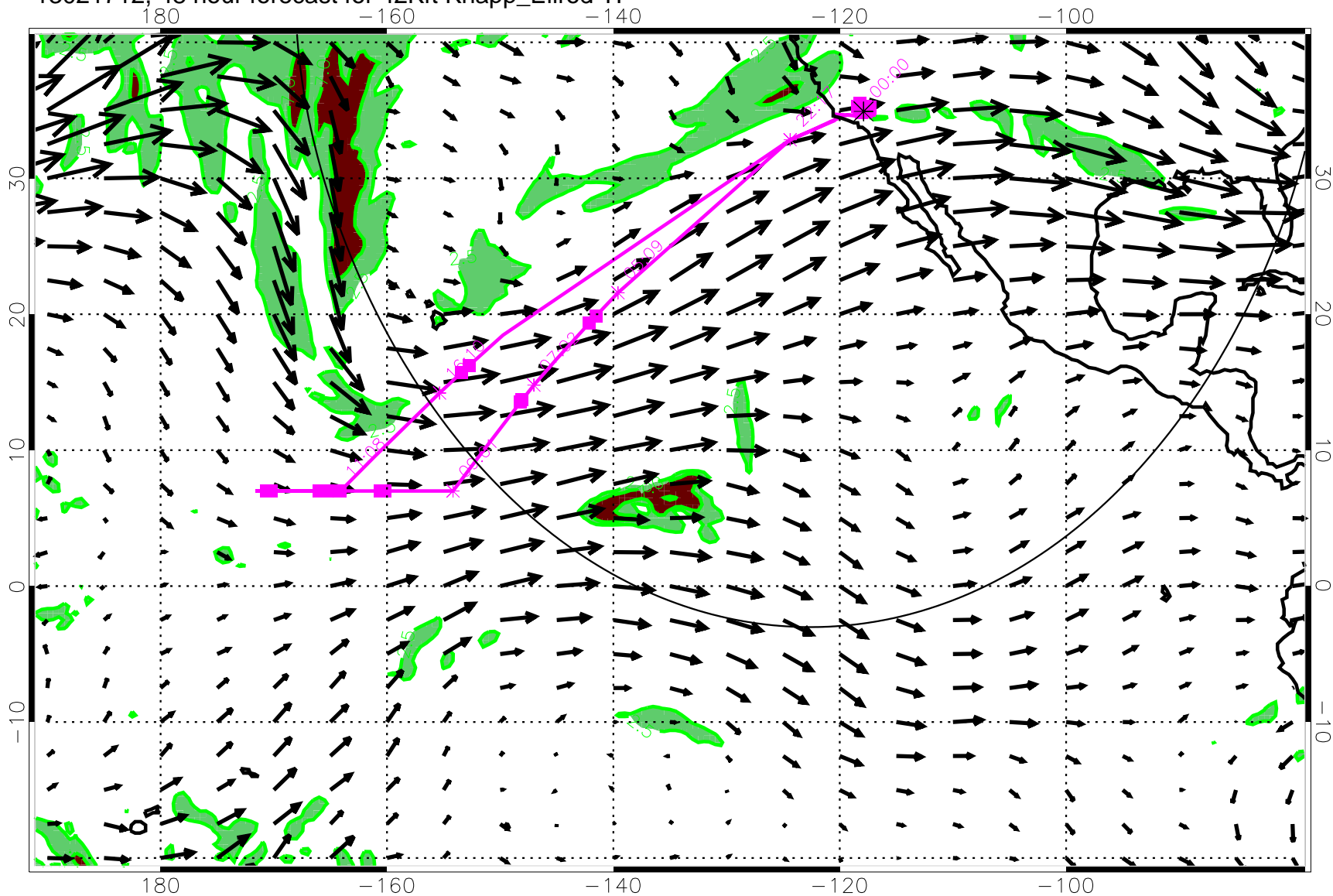
13021712, 48 hour forecast for 42Kft Knapp_Ellrod TI
