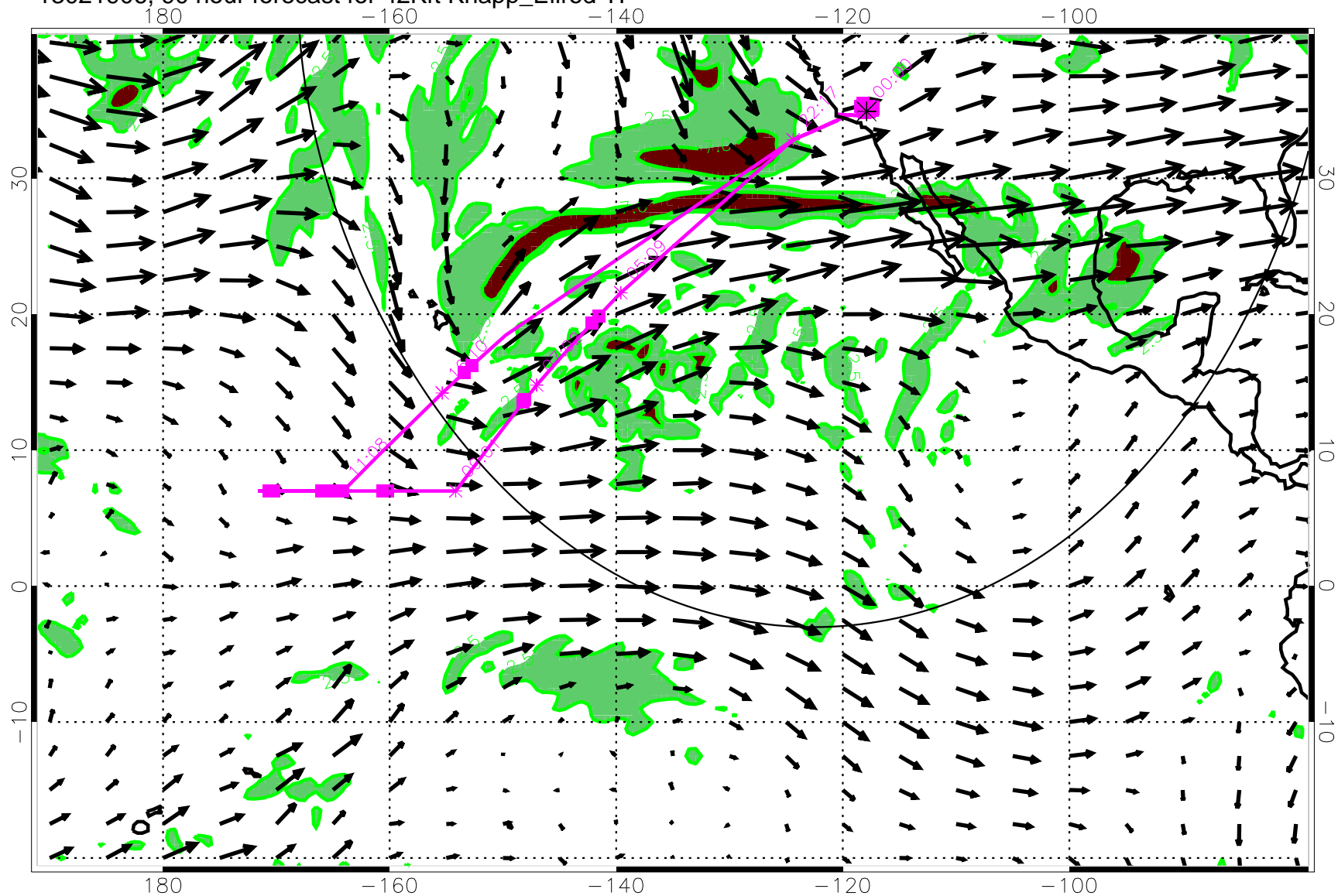
13021906, 90 hour forecast for 42Kft Knapp_Ellrod TI
