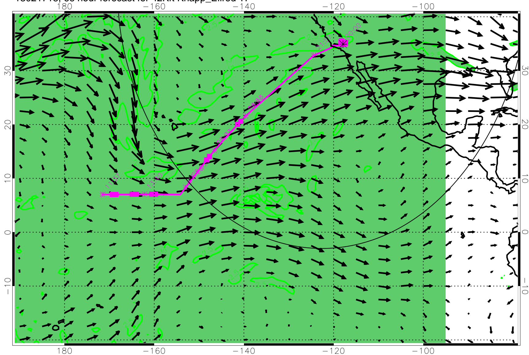
13021718, 66 hour forecast for 42Kft Knapp_Ellrod TI
