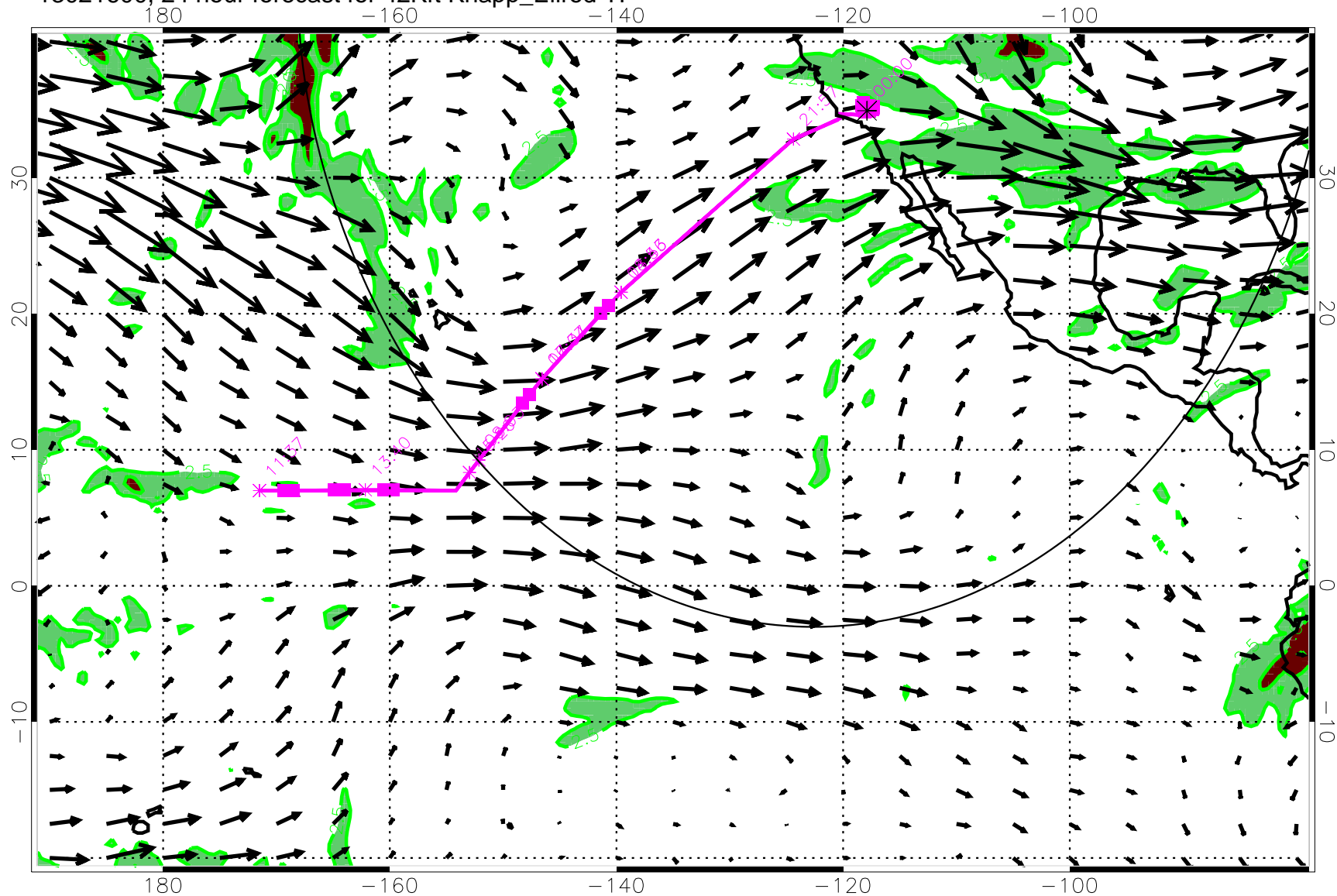
13021600, 24 hour forecast for 42Kft Knapp_Ellrod TI
