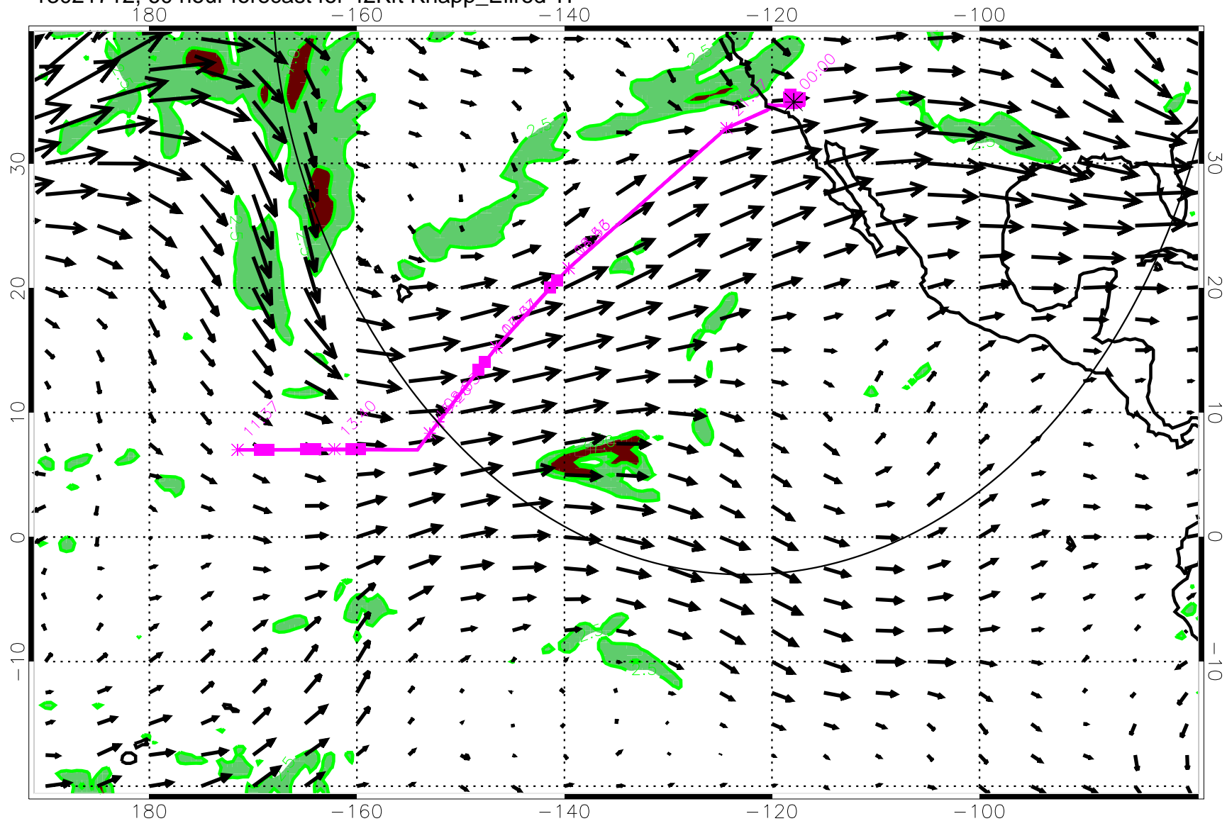
13021712, 60 hour forecast for 42Kft Knapp_Ellrod TI
