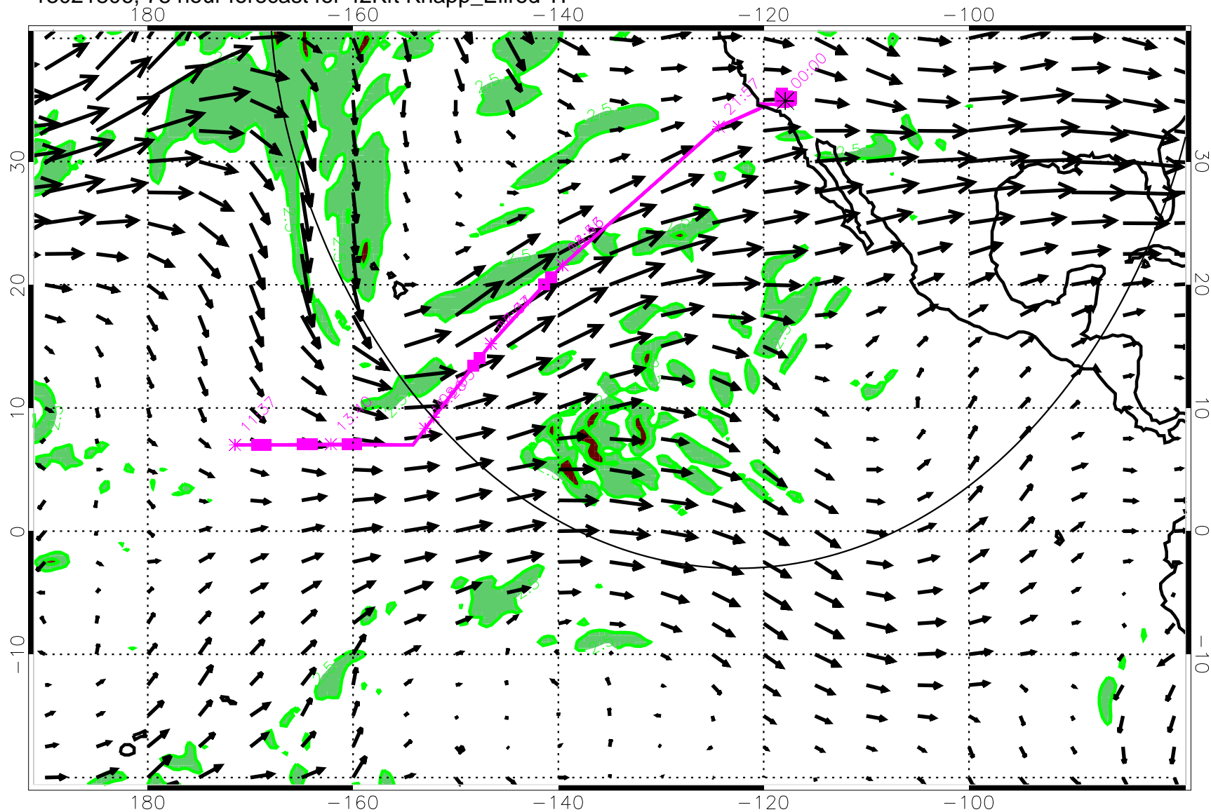
13021806, 78 hour forecast for 42Kft Knapp_Ellrod TI
