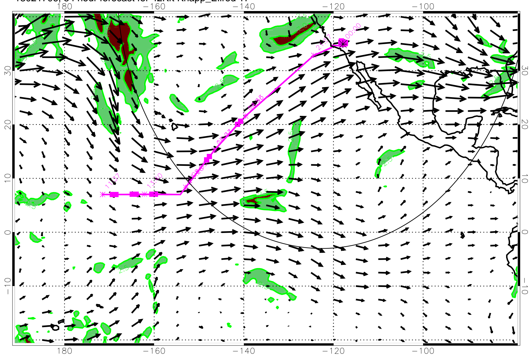
13021706, 54 hour forecast for 42Kft Knapp_Ellrod TI
