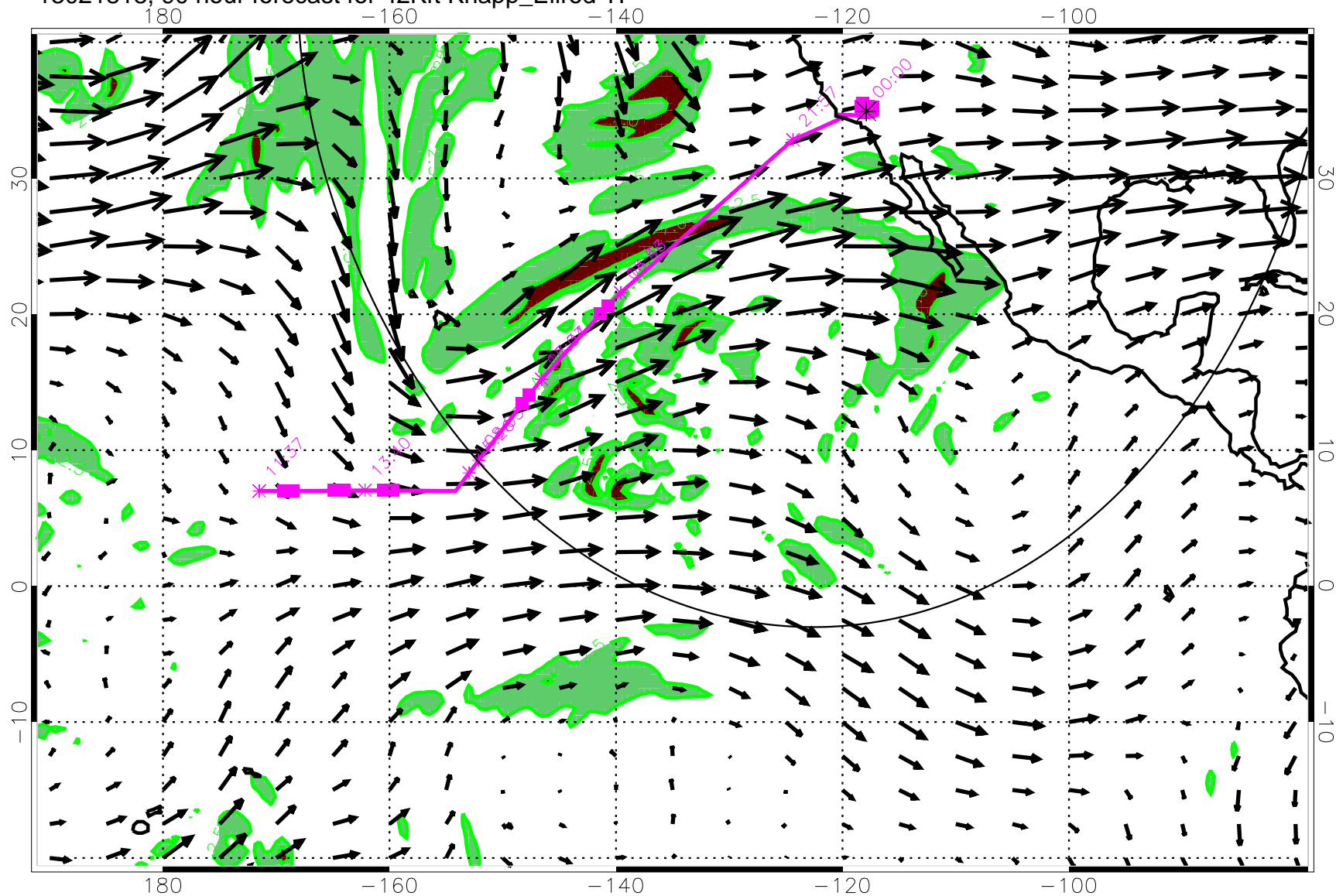
13021818, 90 hour forecast for 42Kft Knapp_Ellrod TI
