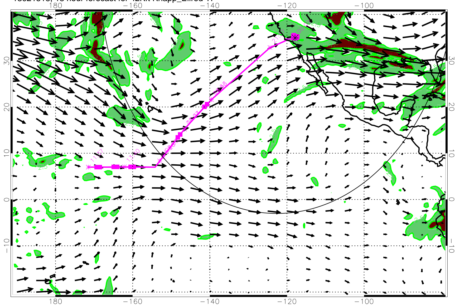
13021518, 18 hour forecast for 42Kft Knapp_Ellrod TI
