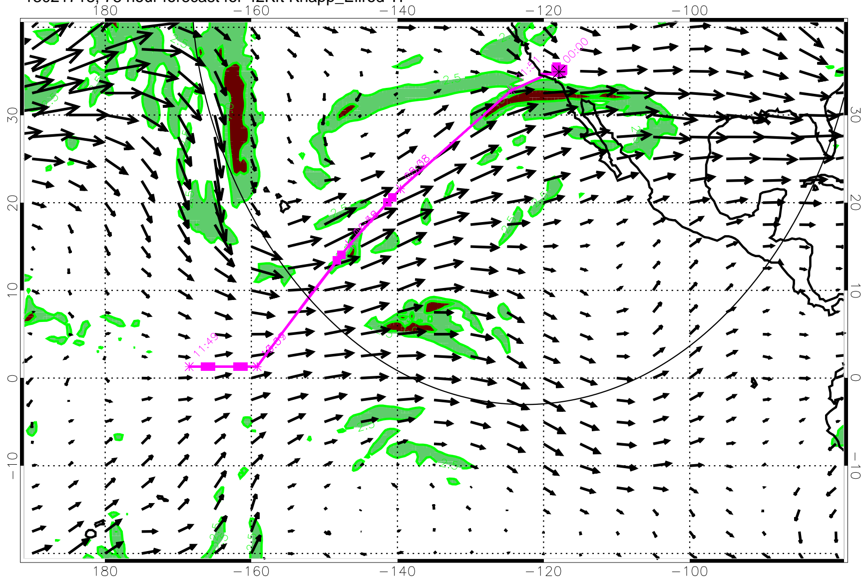
13021718, 78 hour forecast for 42Kft Knapp_Ellrod TI
