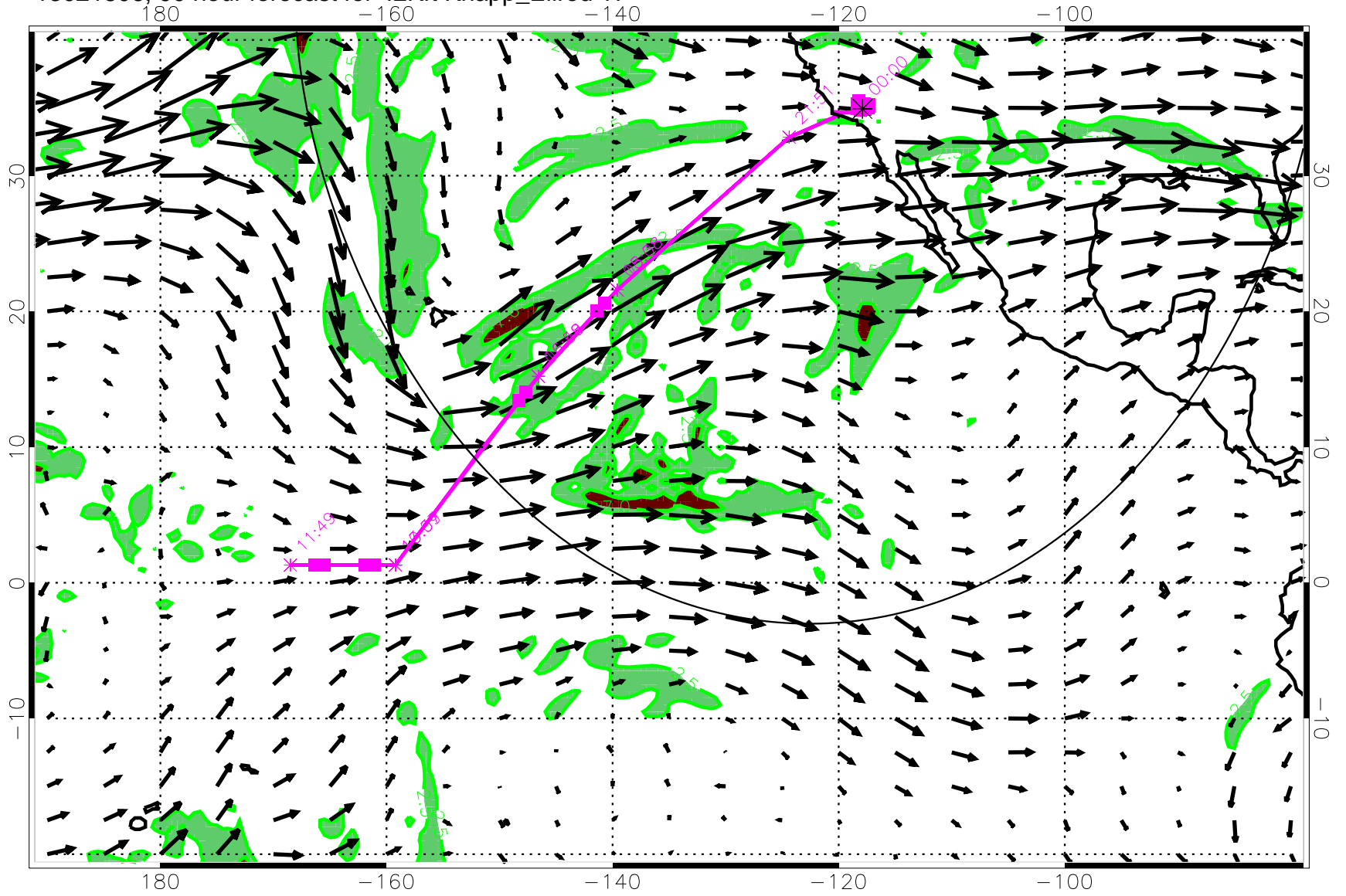
13021806, 90 hour forecast for 42Kft Knapp_Ellrod TI
