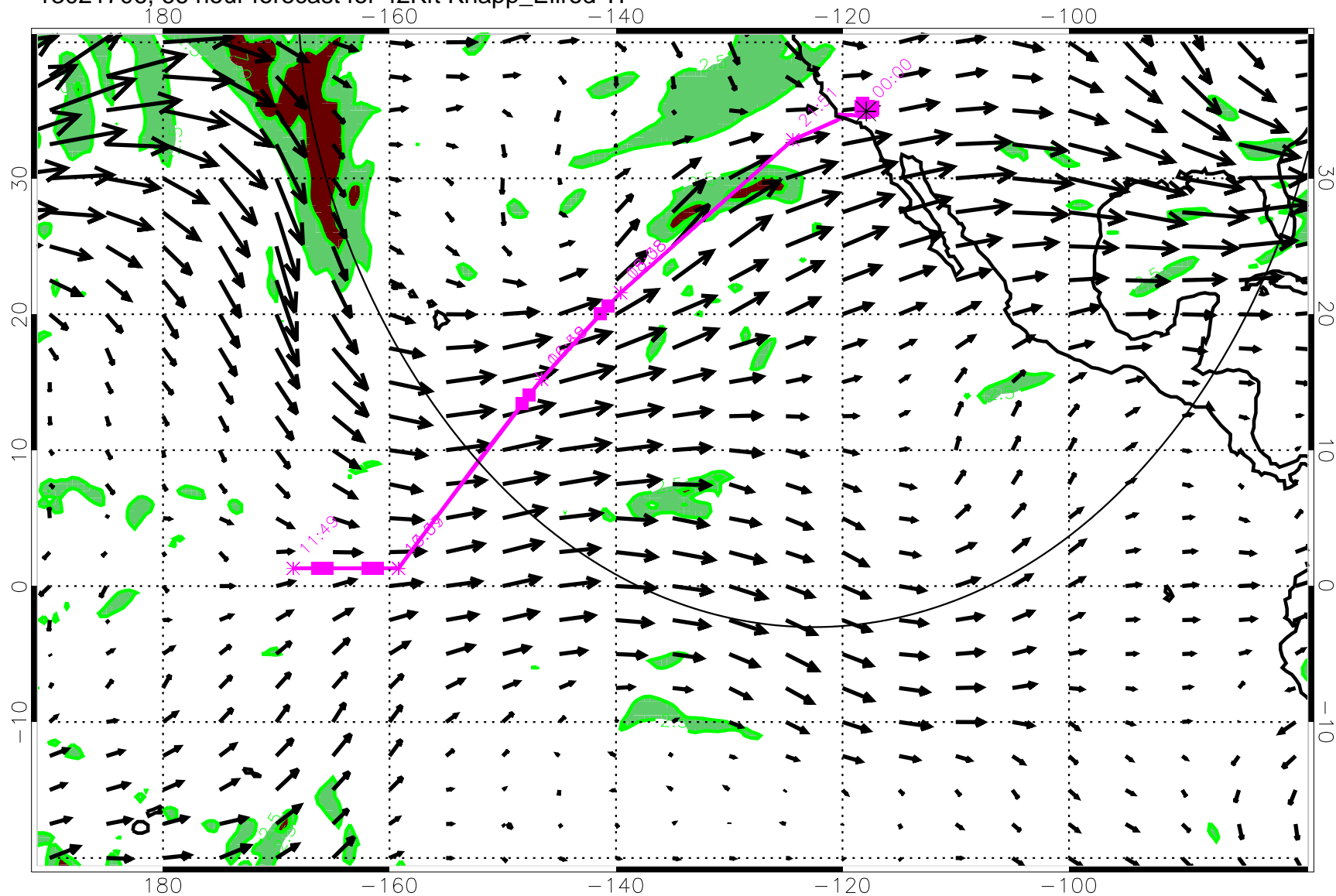
13021706, 66 hour forecast for 42Kft Knapp_Ellrod TI
