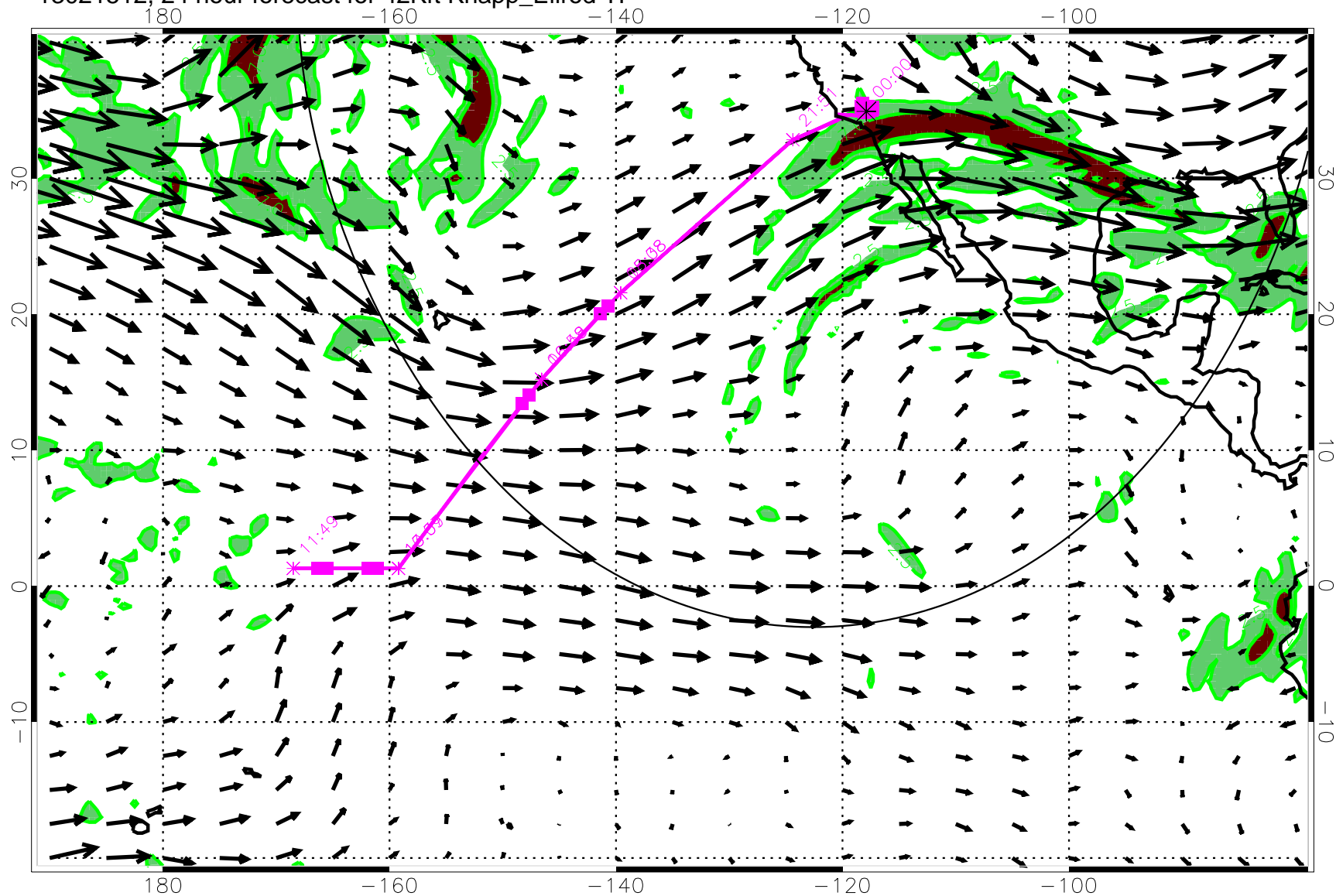
13021512, 24 hour forecast for 42Kft Knapp_Ellrod TI
