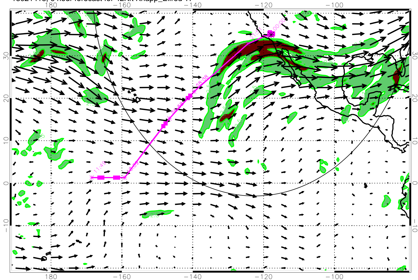
13021418, 6 hour forecast for 42Kft Knapp_Ellrod TI
