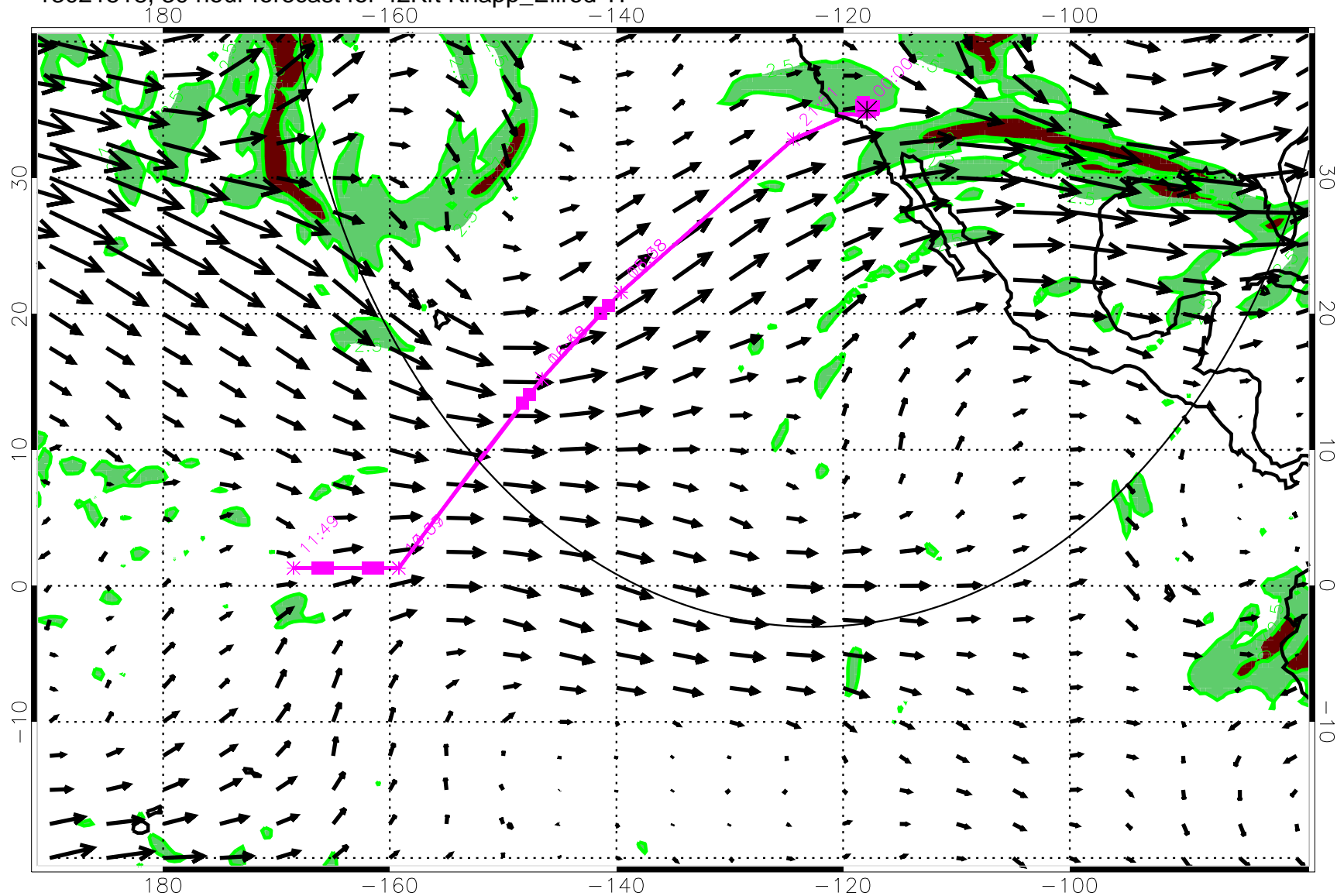
13021518, 30 hour forecast for 42Kft Knapp_Ellrod TI
