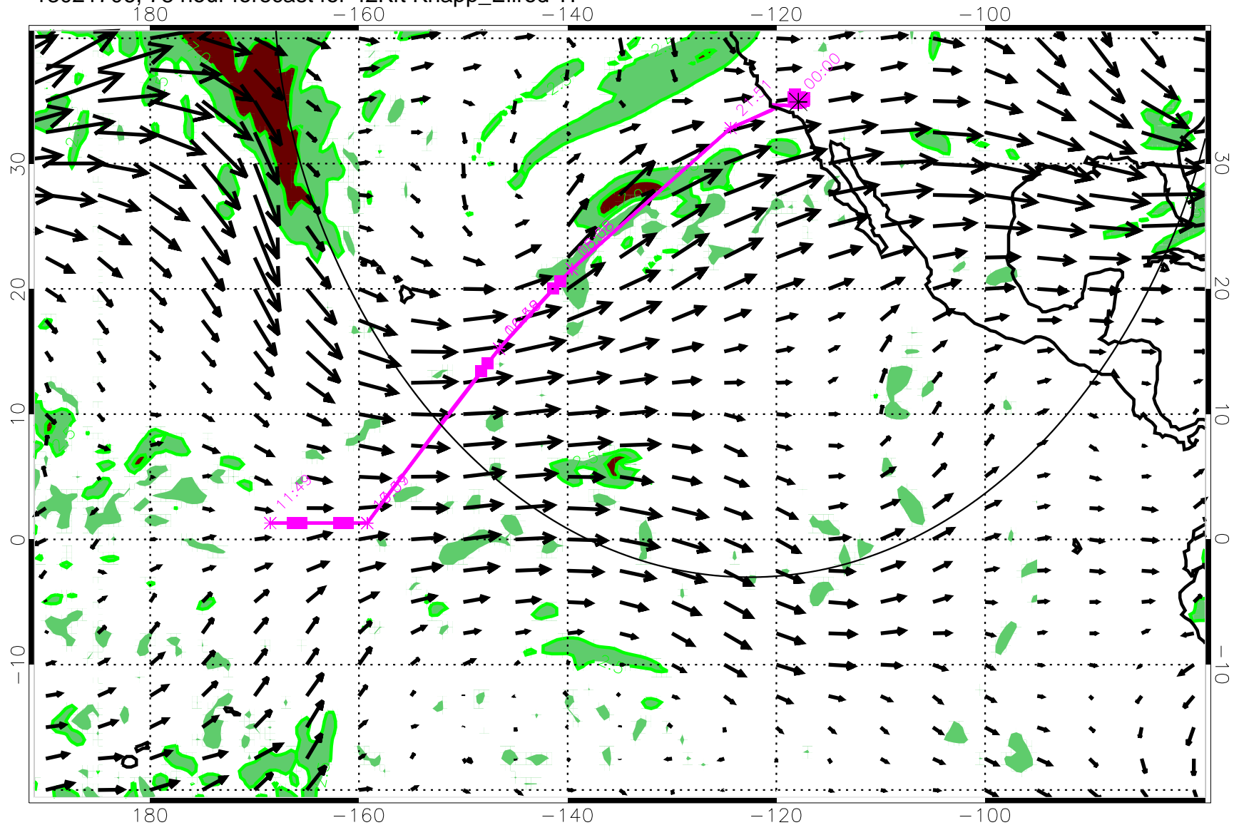
13021706, 78 hour forecast for 42Kft Knapp_Ellrod TI
